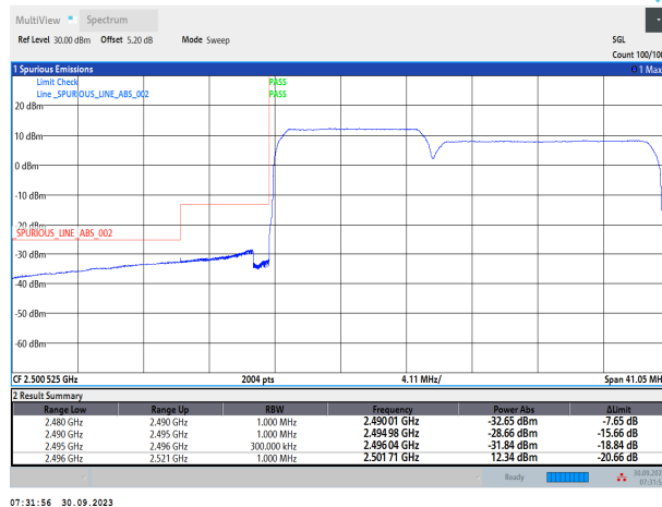
41-41-10MHz-15MHz-QPSK-QPSK-39703-39823-50RB#0-75RB#0
