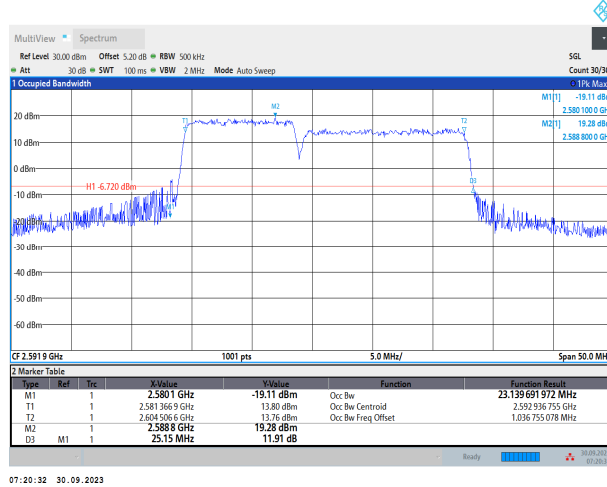
41-41-10MHz-15MHz-16QAM-16QAM-40549-40669-50RB#0-75RB#0
