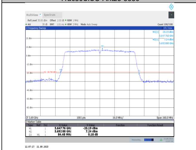
11ac80SISO-Ant23-5690
