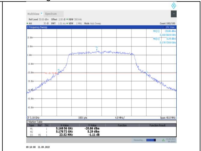
11n20SISO-Ant23-5180
