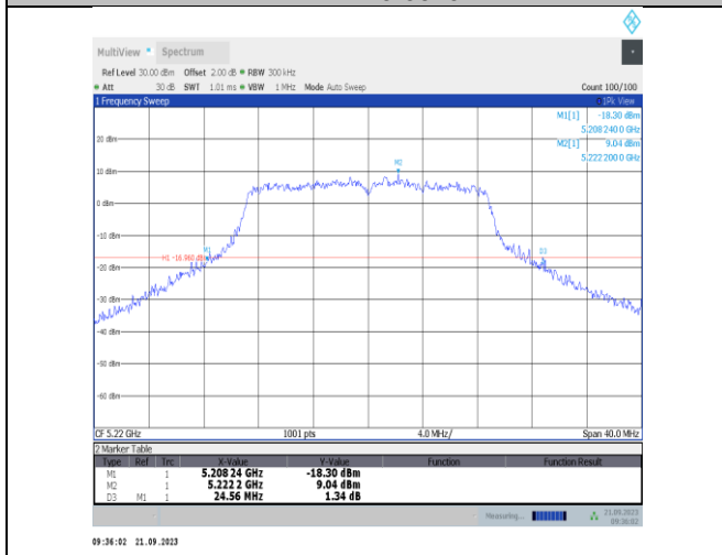
11n20SISO-Ant23-5220
