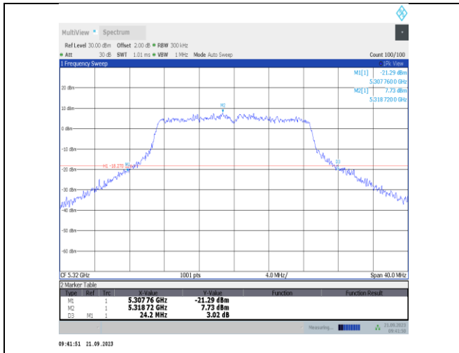
11n20SISO-Ant23-5320
