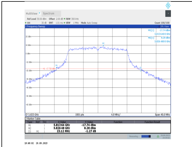
11a-Ant23-5825
