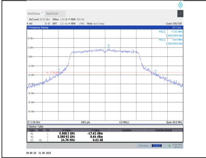
11n20SISO-Ant23-5580
