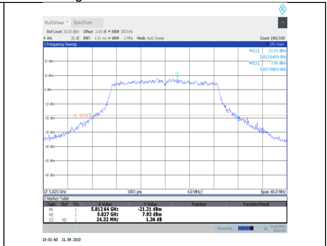
11n20SISO-Ant23-5825
