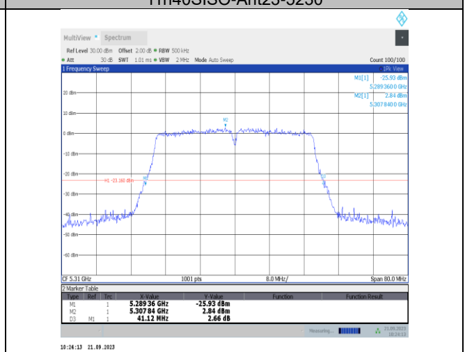
11n40SISO-Ant23-5310
