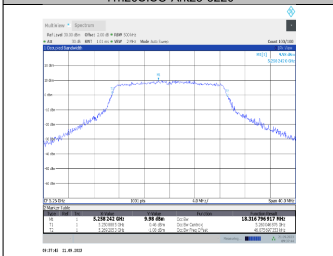
11n20SISO-Ant23-5260
