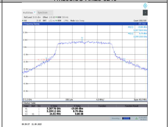
11n20SISO-Ant23-5300
