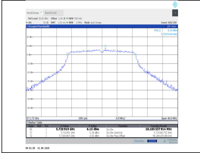
11n20SISO-Ant23-5720
