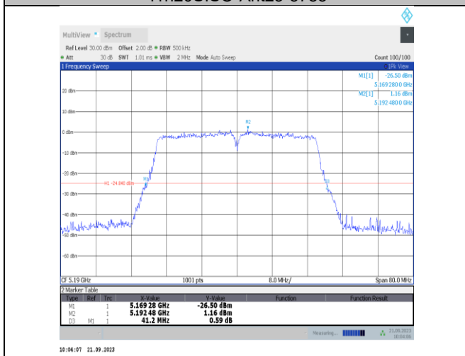
11n40SISO-Ant23-5190
