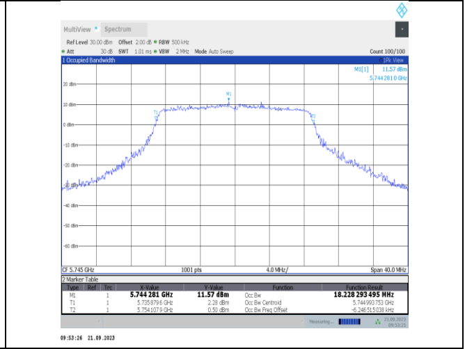
11n20SISO-Ant23-5745
