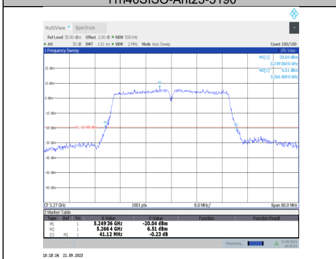
11n40SISO-Ant23-5270
