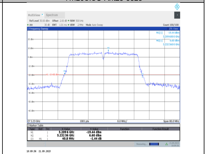
11n40SISO-Ant23-5230
