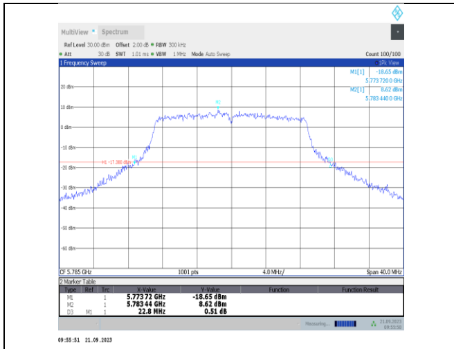
11n20SISO-Ant23-5785
