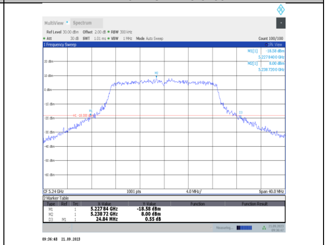
11n20SISO-Ant23-5240
