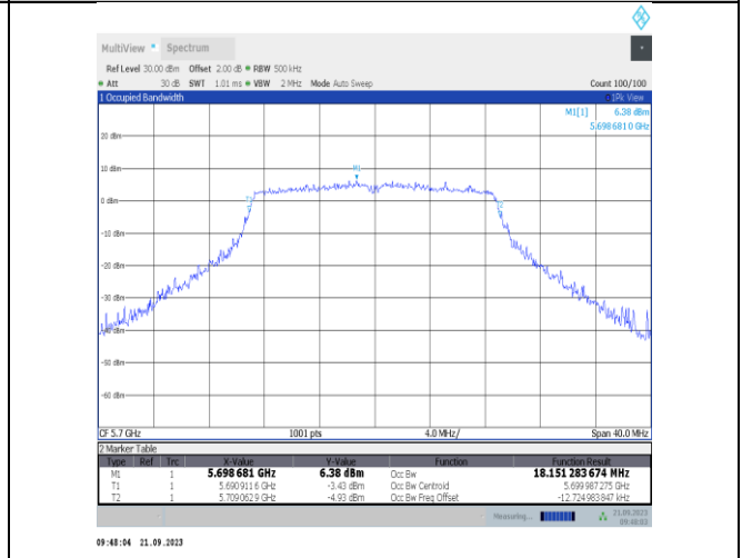
11n20SISO-Ant23-5700
