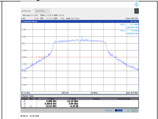
11n20SISO-Ant23-5500
