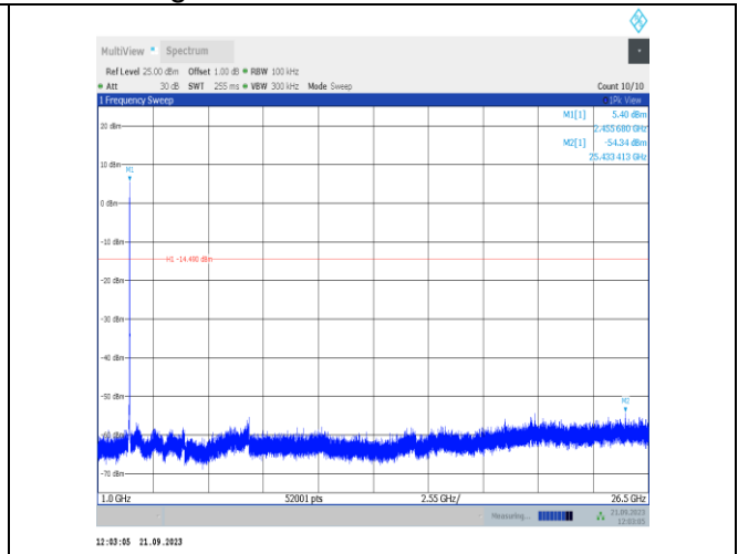
11g-Ant22-2457-1000~26500-PASS
