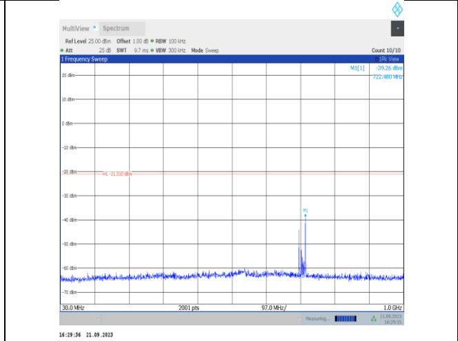
11VHT40SISO-Ant22-2452-30~1000-PASS
