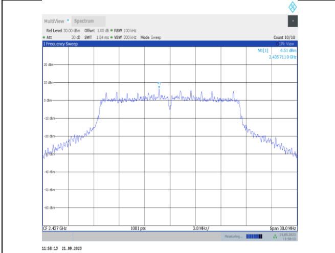
11g-Ant22-2437-0~Reference-PASS
