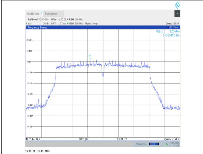
11n40SISO-Ant22-2427-0~Reference-PASS
