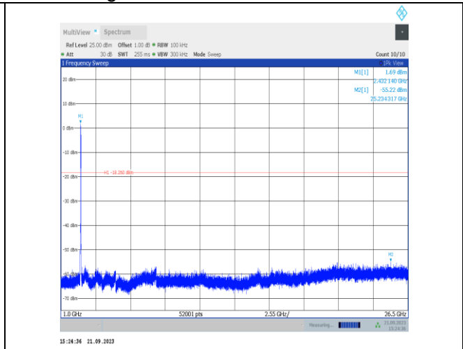
11n40SISO-Ant22-2437-1000~26500-PASS
