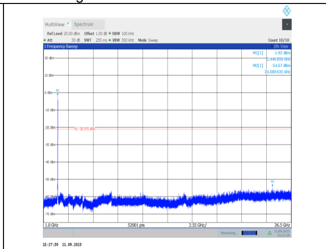
11n40SISO-Ant22-2452-1000~26500-PASS
