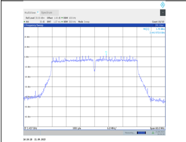
11VHT40SISO-Ant22-2437-0~Reference-PASS
