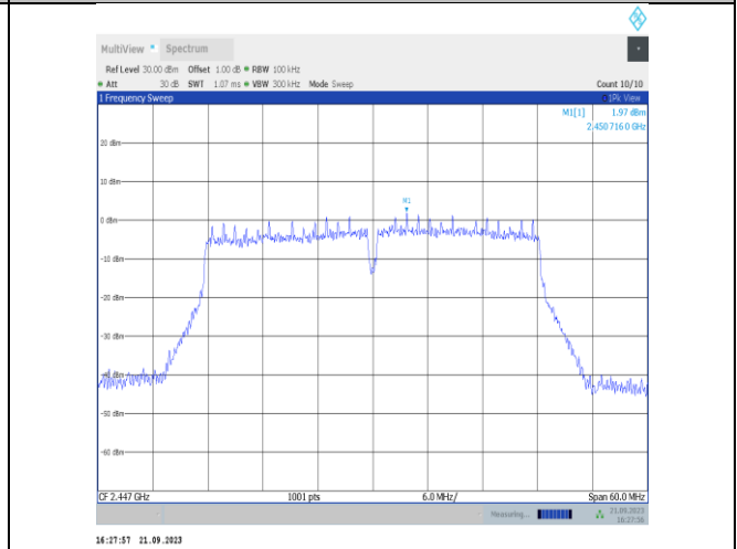
11VHT40SISO-Ant22-2447-0~Reference-PASS
