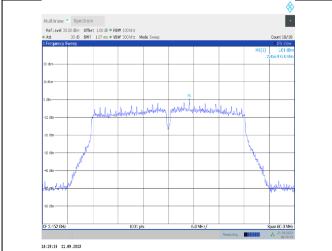
11VHT40SISO-Ant22-2452-0~Reference-PASS
