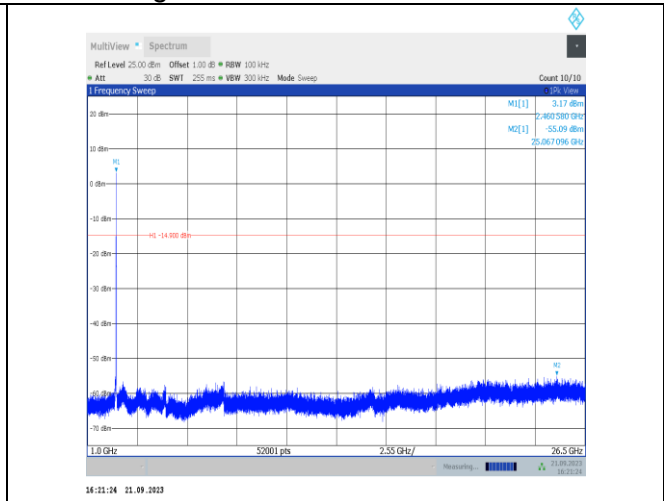
11VHT20SISO-Ant22-2462-1000~26500-PASS
