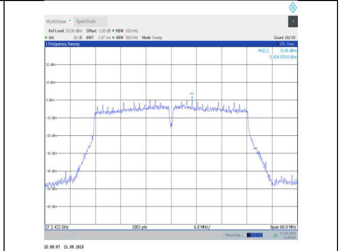
11n40SISO-Ant22-2422-0~Reference-PASS
