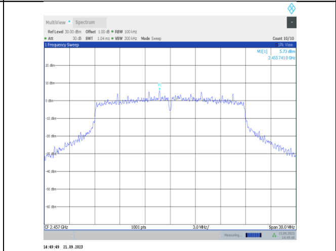
11n20SISO-Ant22-2457-0~Reference-PASS
