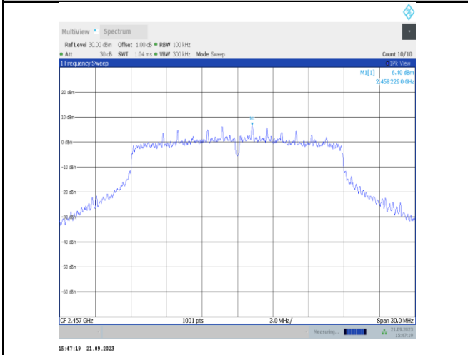
11VHT20SISO-Ant22-2457-0~Reference-PASS
