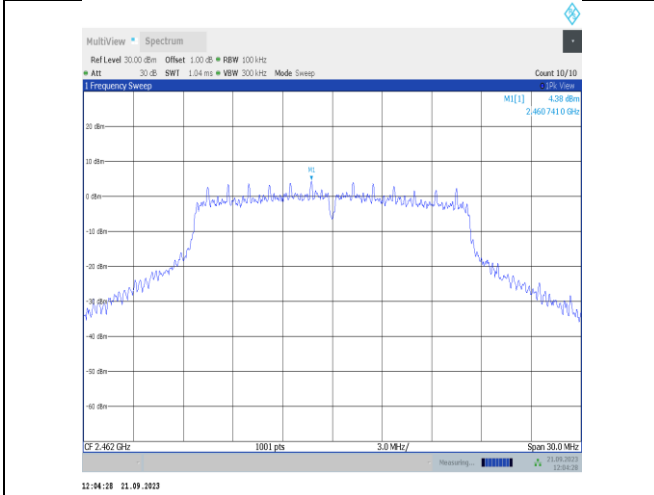
11g-Ant22-2462-0~Reference-PASS
