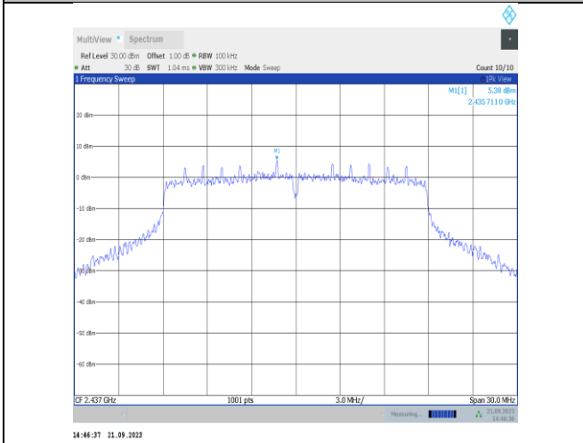
11n20SISO-Ant22-2437-0~Reference-PASS
