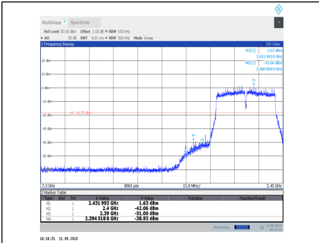
11VHT40SISO-Ant22-2427-PASS
