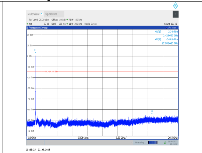
11VHT20SISO-Ant22-2437-1000~26500-PASS
