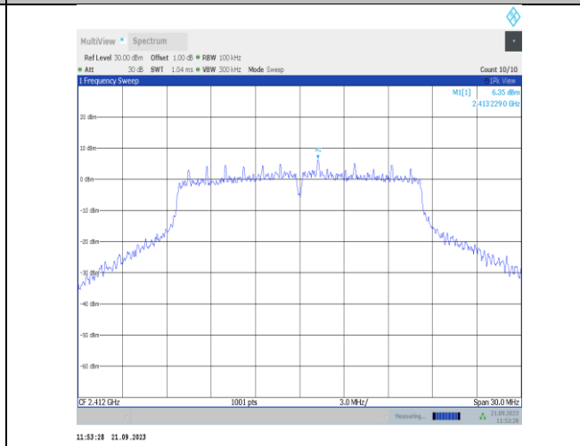
11g-Ant22-2412-0~Reference-PASS
