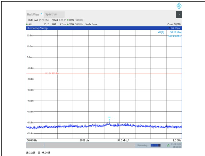
11VHT20SISO-Ant22-2462-30~1000-PASS
