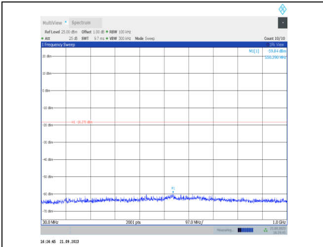
11VHT40SISO-Ant22-2427-30~1000-PASS
