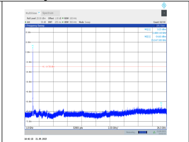
11n20SISO-Ant22-2412-1000~26500-PASS
