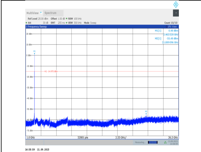
11n20SISO-Ant22-2462-1000~26500-PASS
