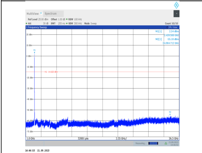
11n20SISO-Ant22-2437-1000~26500-PASS
