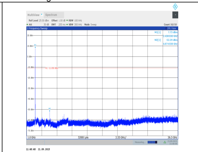
11b-Ant22-2437-1000~26500-PASS
