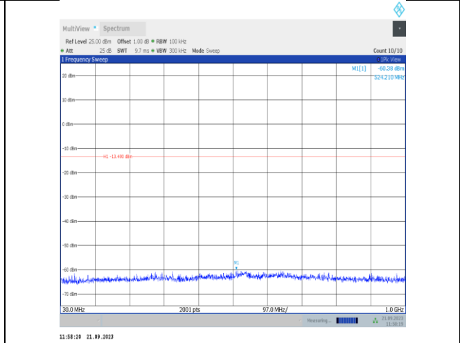
11g-Ant22-2437-30~1000-PASS
