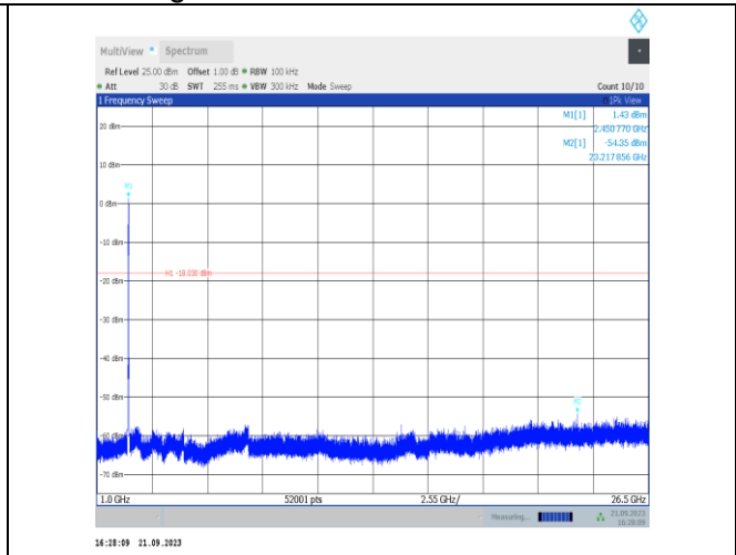
11VHT40SISO-Ant22-2447-1000~26500-PASS
