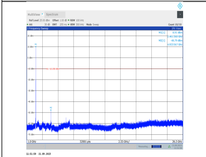
11b-Ant22-2462-1000~26500-PASS
