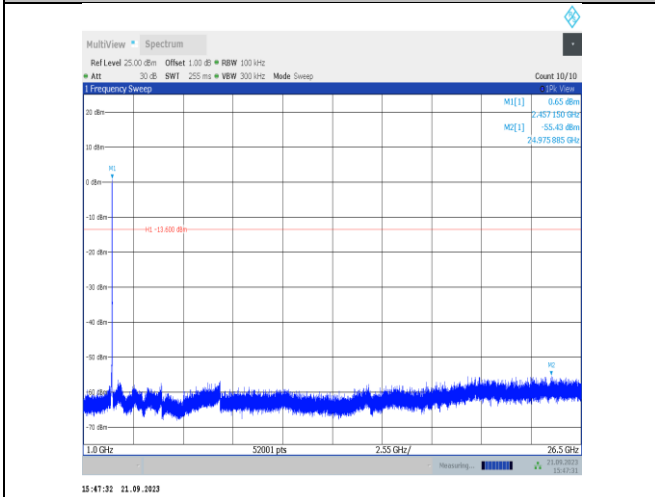
11VHT20SISO-Ant22-2457-1000~26500-PASS
