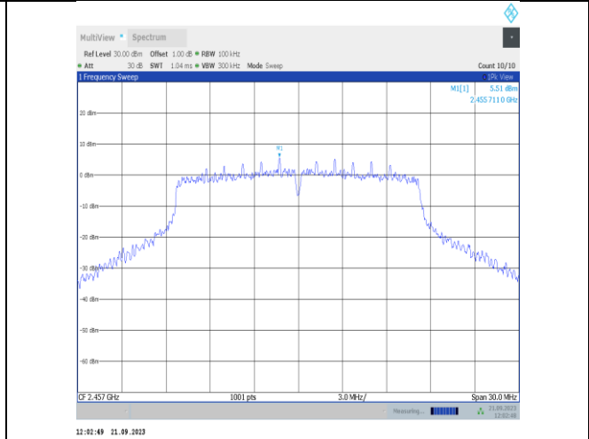
11g-Ant22-2457-0~Reference-PASS
