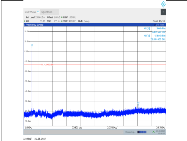
11g-Ant22-2437-1000~26500-PASS
