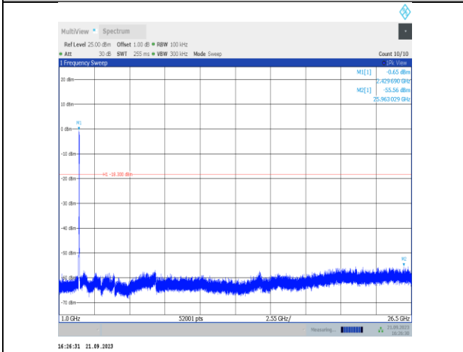
11VHT40SISO-Ant22-2437-1000~26500-PASS
