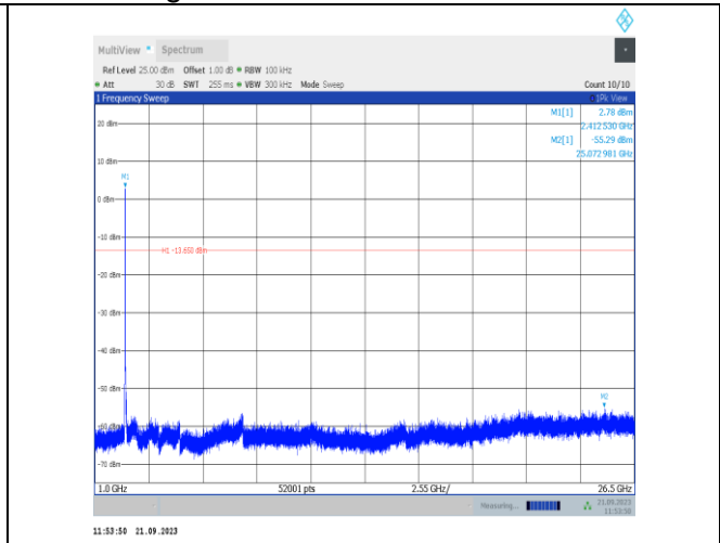
11g-Ant22-2412-1000~26500-PASS
