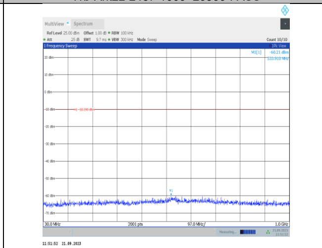
11b-Ant22-2462-30~1000-PASS
