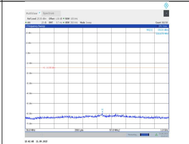
11VHT20SISO-Ant22-2412-30~1000-PASS
