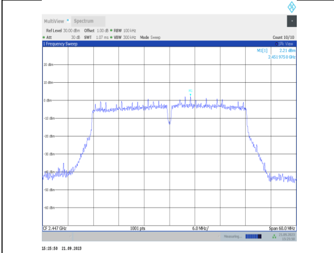
11n40SISO-Ant22-2447-0~Reference-PASS
