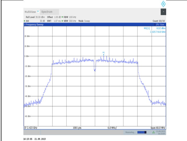
11VHT40SISO-Ant22-2422-0~Reference-PASS
