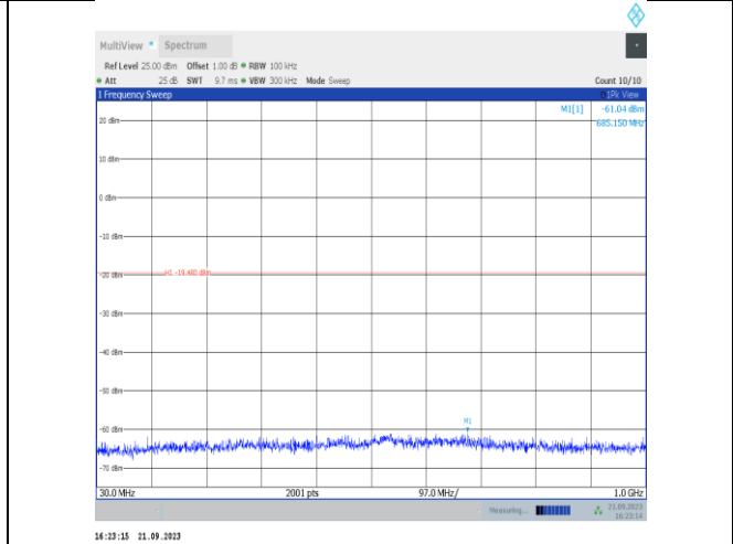
11VHT40SISO-Ant22-2422-30~1000-PASS
