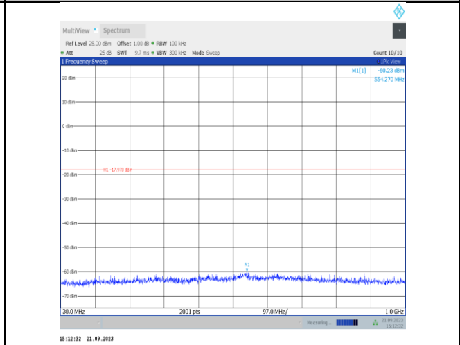
11n40SISO-Ant22-2427-30~1000-PASS
