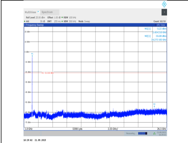
11VHT40SISO-Ant22-2452-1000~26500-PASS
