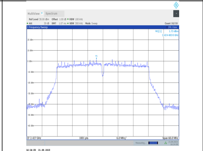
11VHT40SISO-Ant22-2427-0~Reference-PASS
