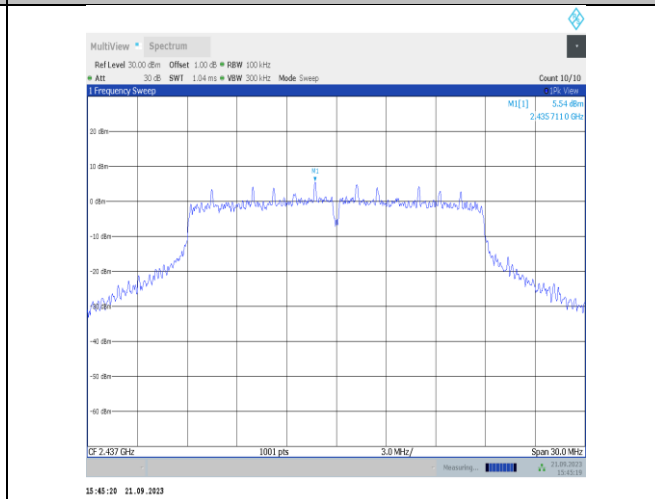
11VHT20SISO-Ant22-2437-0~Reference-PASS
