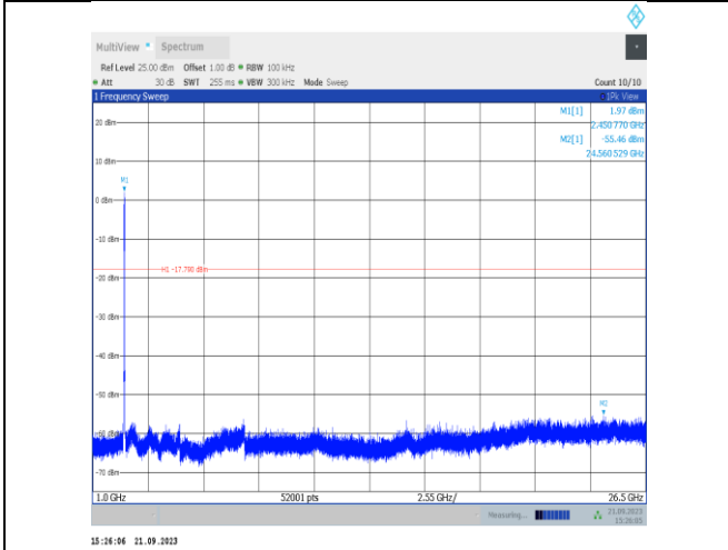
11n40SISO-Ant22-2447-1000~26500-PASS
