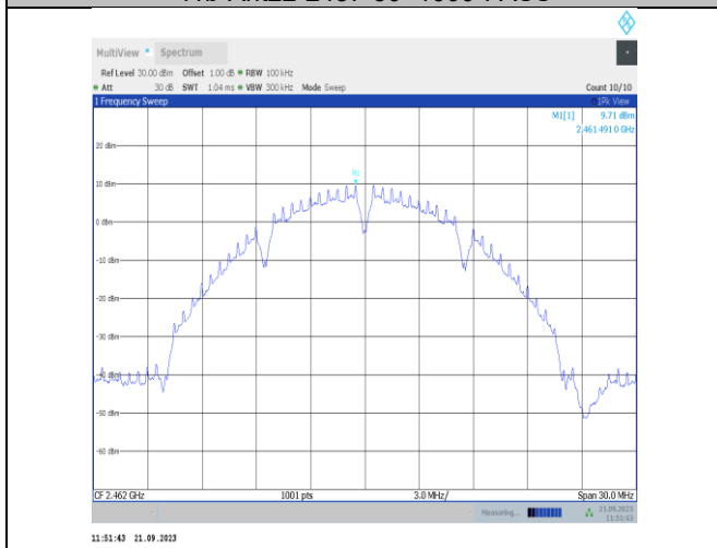
11b-Ant22-2462-0~Reference-PASS
