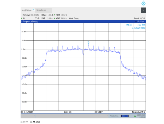
11n20SISO-Ant22-2462-0~Reference-PASS
