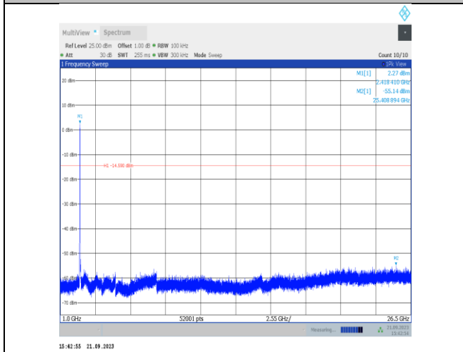
11VHT20SISO-Ant22-2412-1000~26500-PASS
