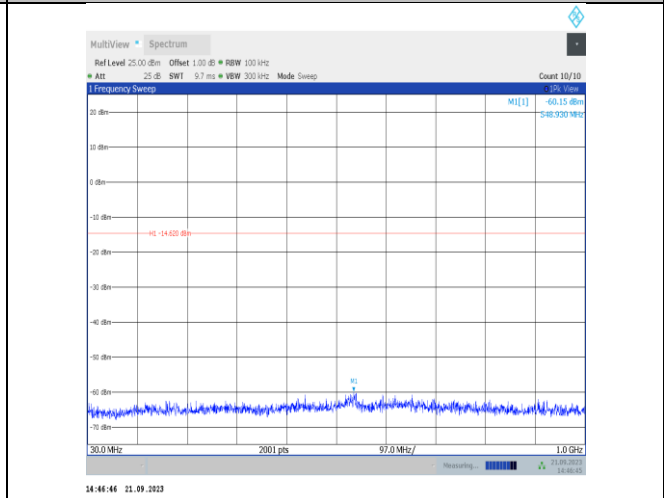
11n20SISO-Ant22-2437-30~1000-PASS
