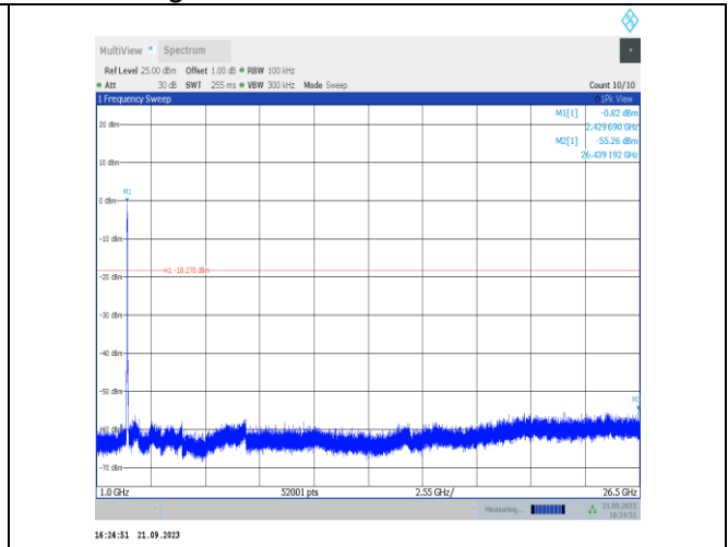
11VHT40SISO-Ant22-2427-1000~26500-PASS
