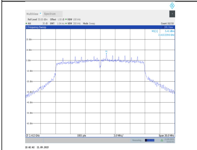
11VHT20SISO-Ant22-2412-0~Reference-PASS
