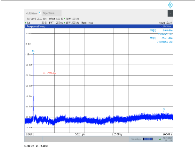
11n40SISO-Ant22-2427-1000~26500-PASS
