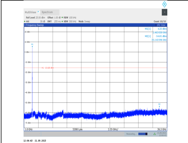
11g-Ant22-2462-1000~26500-PASS
