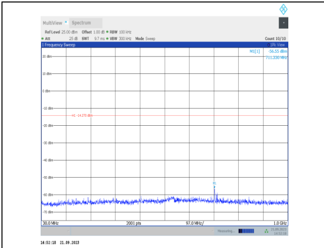
11n20SISO-Ant22-2457-30~1000-PASS
