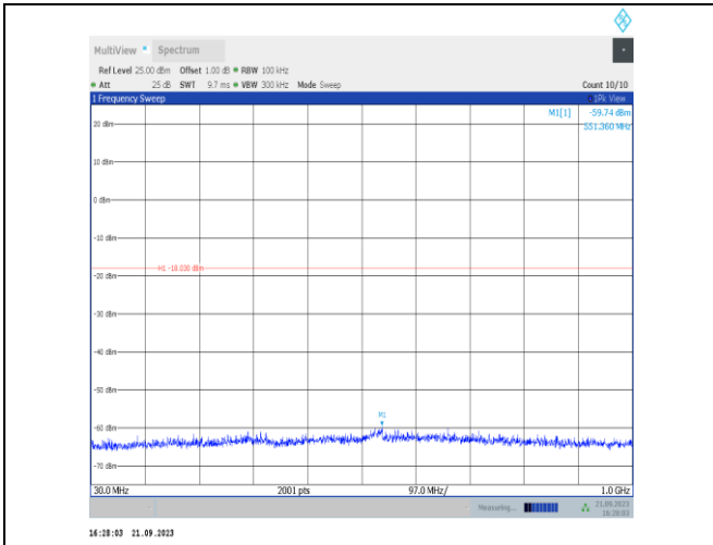
11VHT40SISO-Ant22-2447-30~1000-PASS
