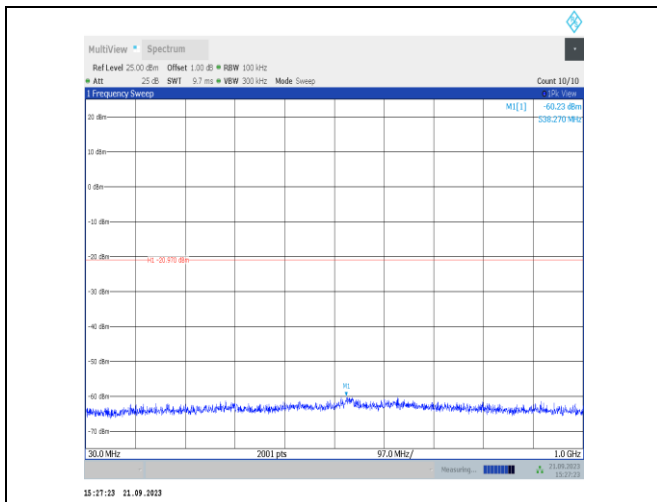
11n40SISO-Ant22-2452-30~1000-PASS
