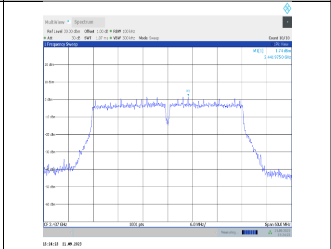
11n40SISO-Ant22-2437-0~Reference-PASS
