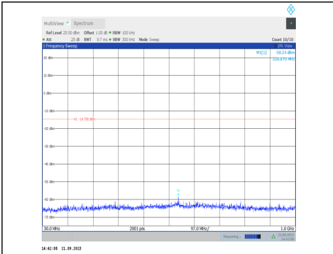
11n20SISO-Ant22-2412-30~1000-PASS
