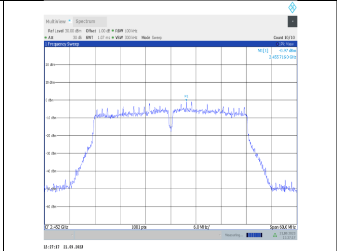
11n40SISO-Ant22-2452-0~Reference-PASS
