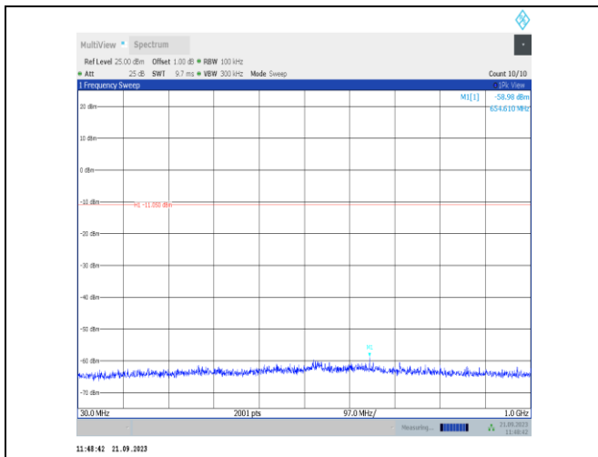
11b-Ant22-2437-30~1000-PASS
