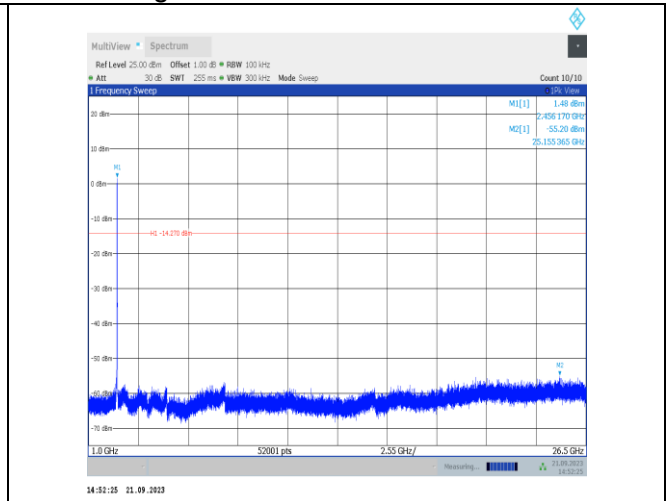
11n20SISO-Ant22-2457-1000~26500-PASS
