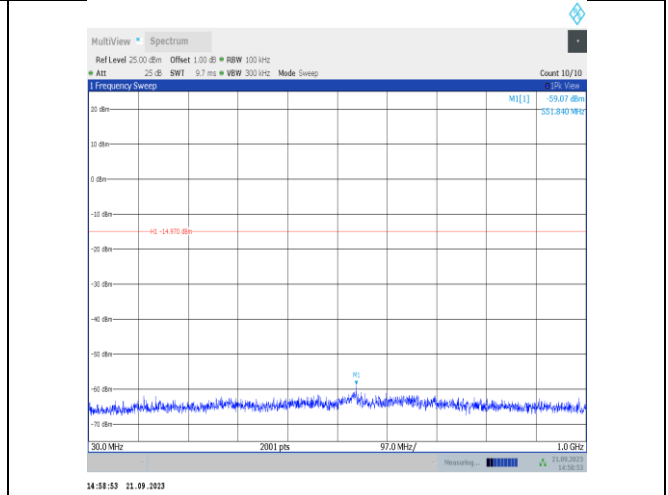
11n20SISO-Ant22-2462-30~1000-PASS
