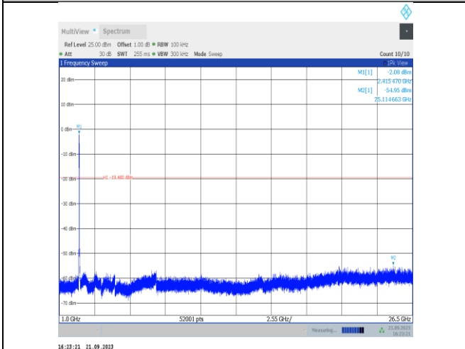
11VHT40SISO-Ant22-2422-1000~26500-PASS
