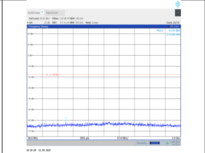
11n40SISO-Ant22-2447-30~1000-PASS
