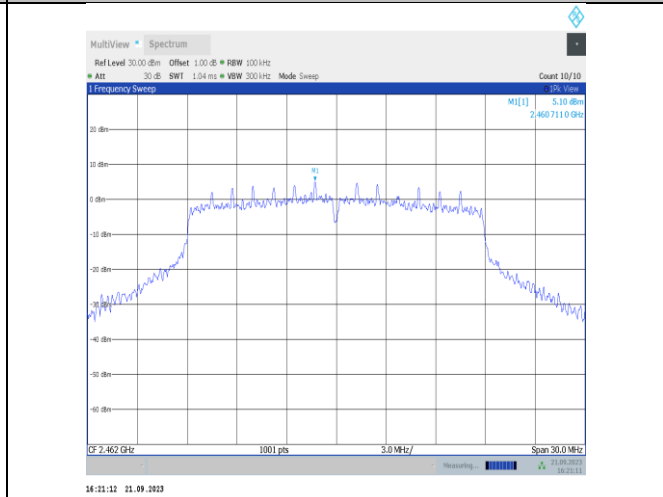
11VHT20SISO-Ant22-2462-0~Reference-PASS
