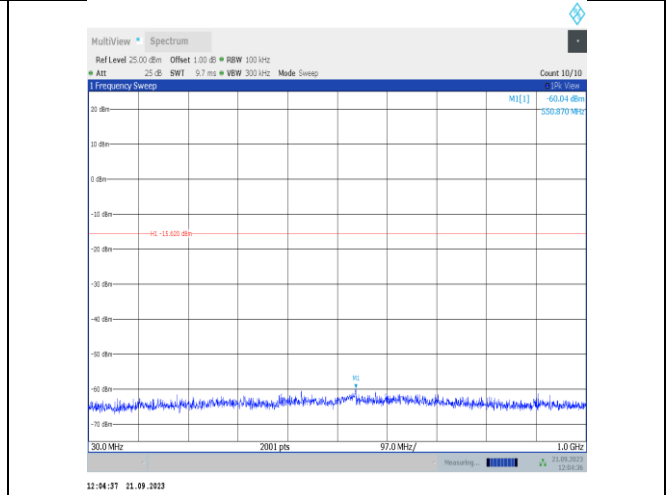
11g-Ant22-2462-30~1000-PASS
