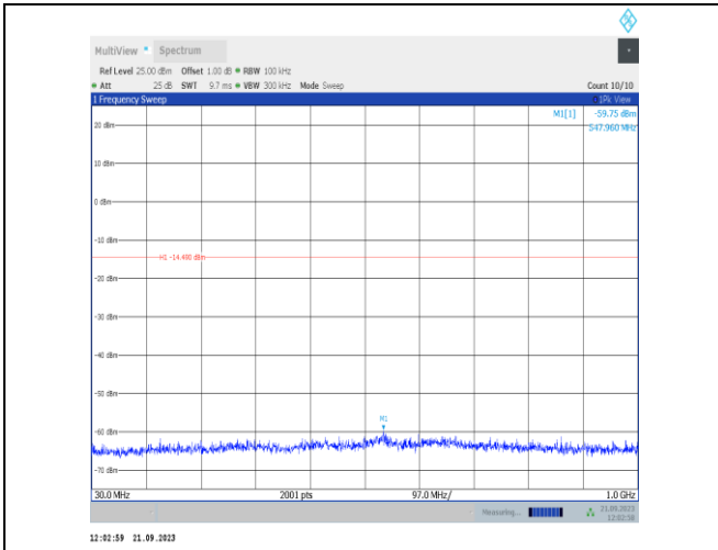
11g-Ant22-2457-30~1000-PASS
