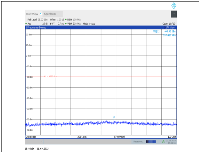
11n40SISO-Ant22-2422-30~1000-PASS
