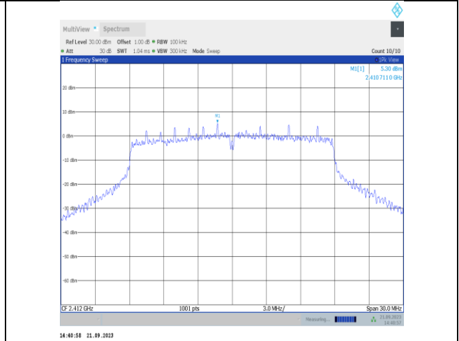
11n20SISO-Ant22-2412-0~Reference-PASS
