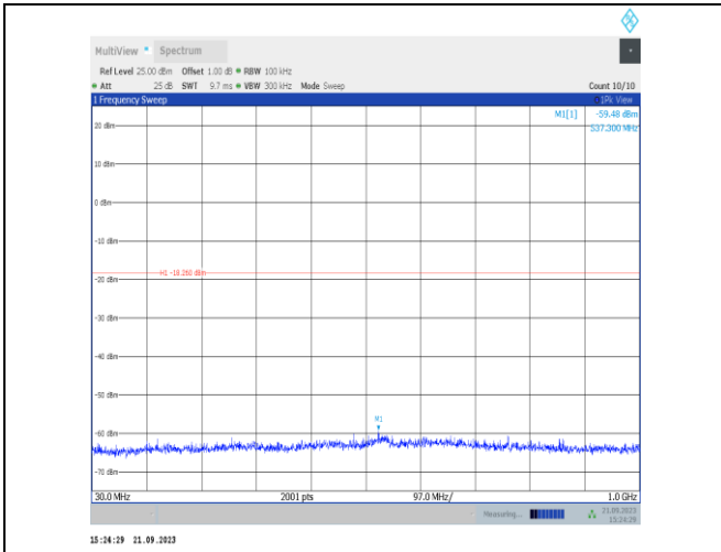
11n40SISO-Ant22-2437-30~1000-PASS
