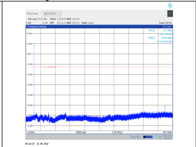
BLE_2M-Ant22-2402-1000~26500-PASS
