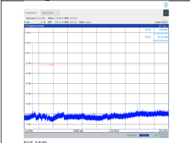
BLE_2M-Ant22-2440-1000~26500-PASS
