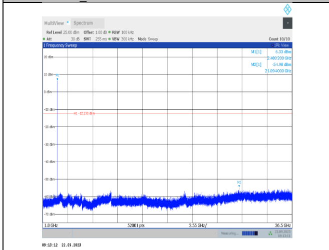
BLE_1M-Ant22-2480-1000~26500-PASS
