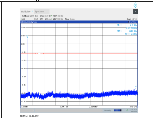
BLE_1M-Ant22-2440-1000~26500-PASS
