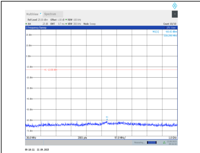
BLE_2M-Ant22-2402-30~1000-PASS
