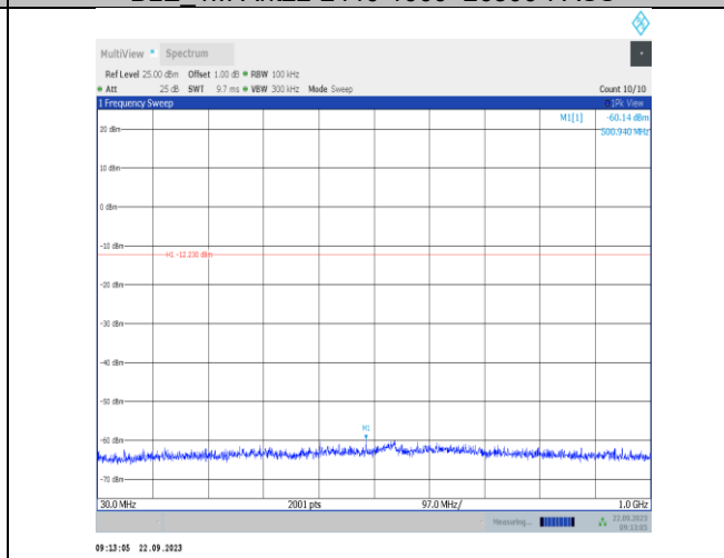
BLE_1M-Ant22-2480-30~1000-PASS
