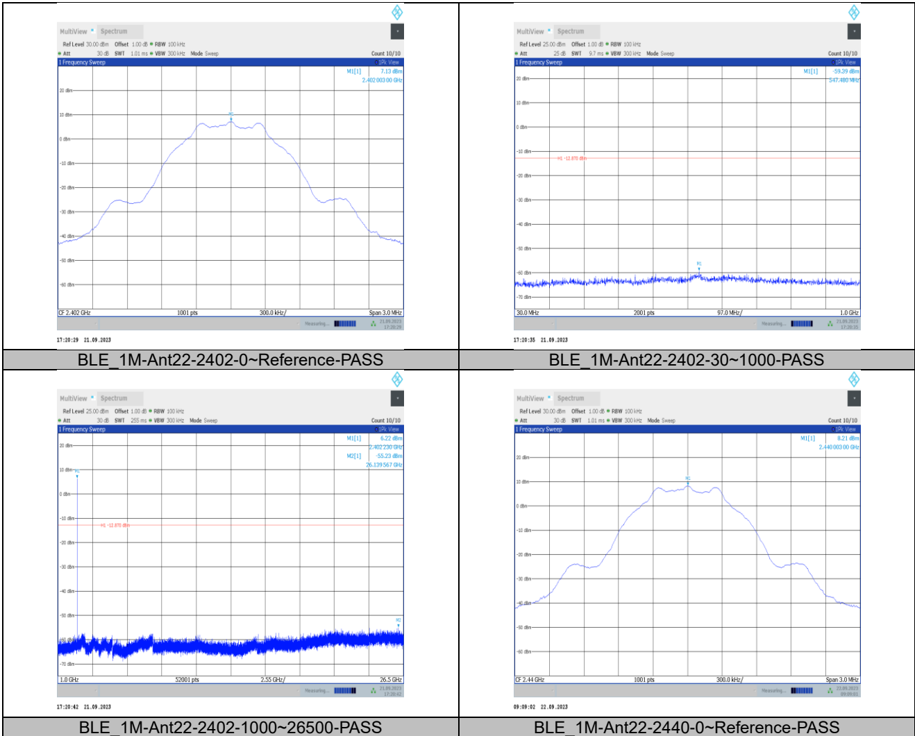
BLE_1M-Ant22-2402-1000~26500-PASS
