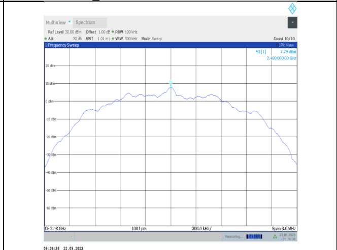
BLE_2M-Ant22-2480-0~Reference-PASS
