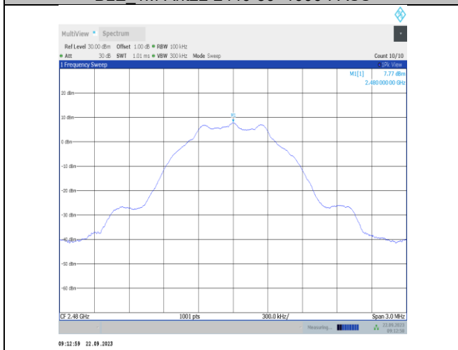
BLE_1M-Ant22-2480-0~Reference-PASS
