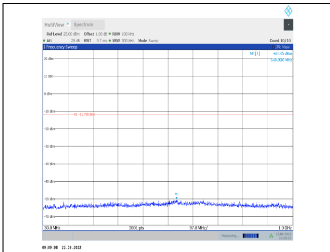
BLE_1M-Ant22-2440-30~1000-PASS
