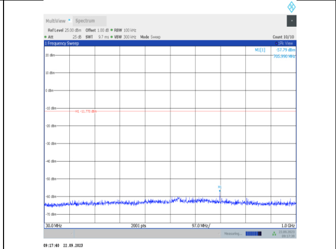
BLE_2M-Ant22-2440-30~1000-PASS
