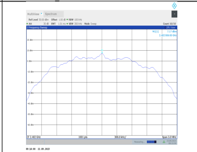
BLE_2M-Ant22-2402-0~Reference-PASS
