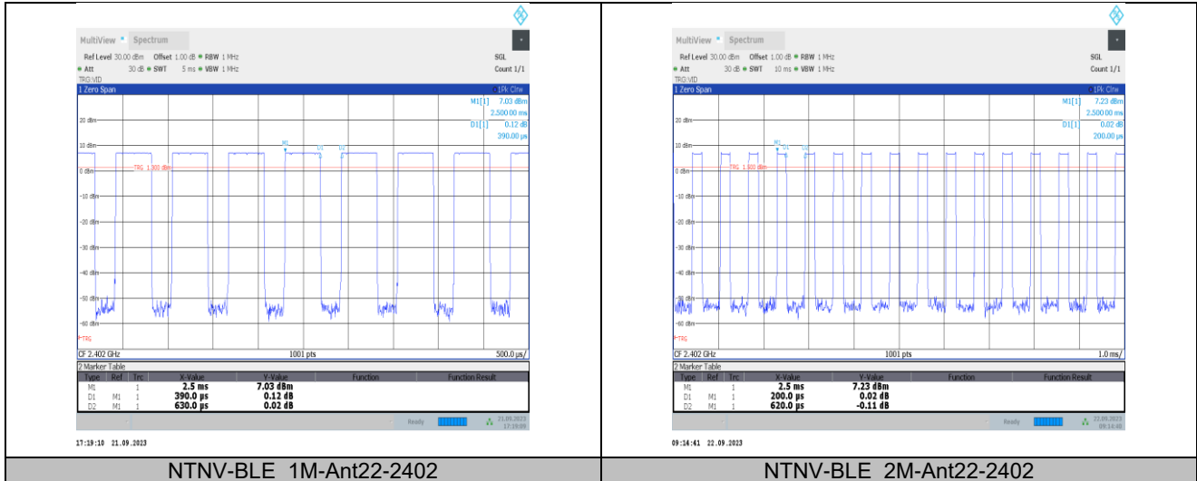
NTNV-BLE 1M-Ant22-2402
