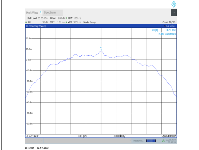
BLE_2M-Ant22-2440-0~Reference-PASS
