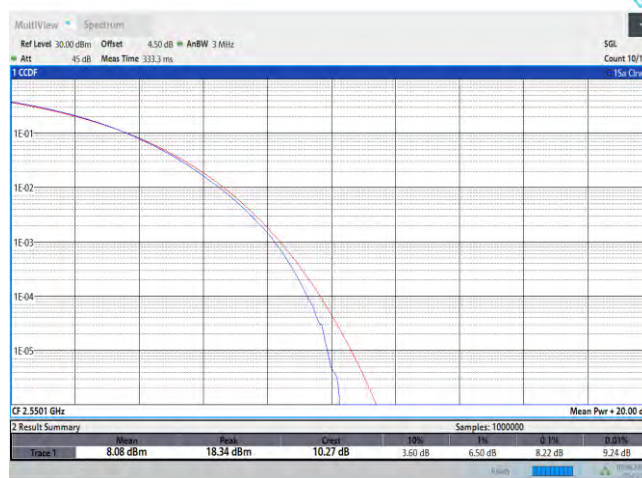
7-7-20MHz-20MHz-QPSK-QPSK-21152-21350-100RB#0-100RB#0
