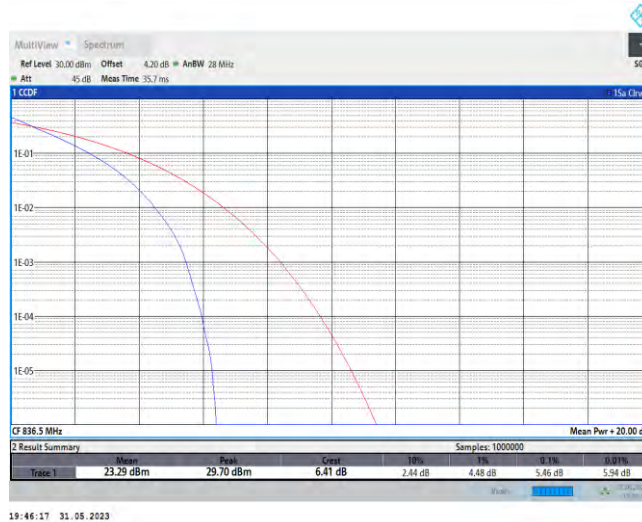
Band26-15MHz-QPSK-26915-75RB#0
