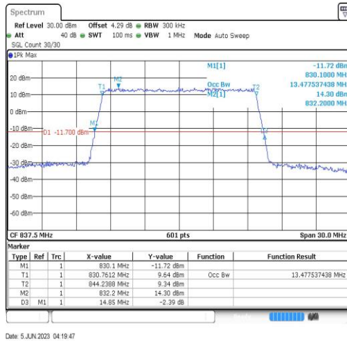
Band19-15MHz-256QAM-24075-75RB#0
