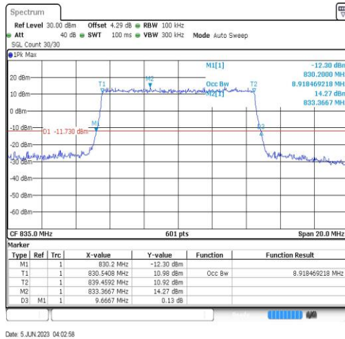
Band19-10MHz-16QAM-24050-50RB#0
