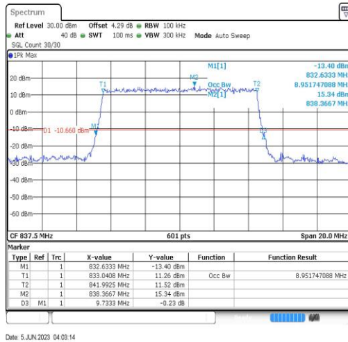
Band19-10MHz-QPSK-24075-50RB#0
