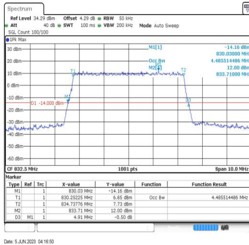
Band19-5MHz-256QAM-24025-25RB#0
