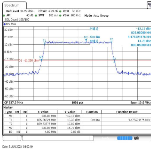
Band19-5MHz-QPSK-24075-25RB#0
