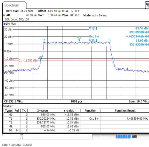
Band19-5MHz-16QAM-24025-25RB#0
