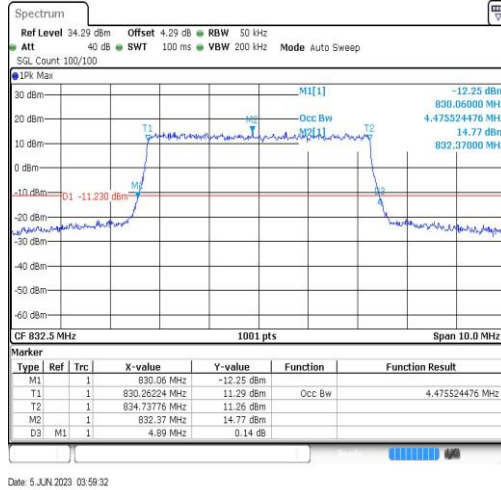
Band19-5MHz-QPSK-24025-25RB#0
