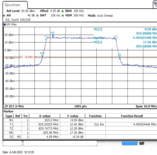
18(824-830)-5MHz-QPSK-23975-25RB#0
