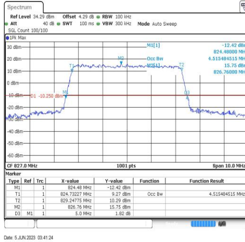
18(824-830)-5MHz-64QAM-23970-25RB#0
