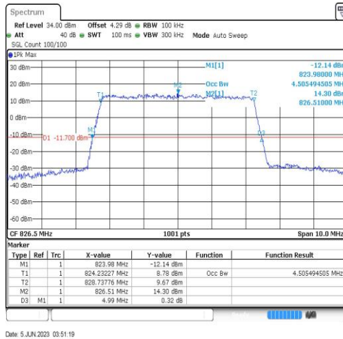
18(824-830)-5MHz-256QAM-23965-25RB#0
