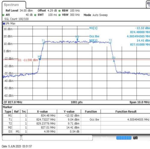
18(824-830)-5MHz-256QAM-23970-25RB#0
