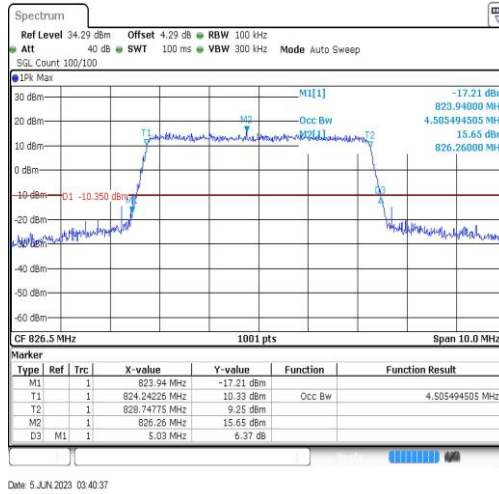
18(824-830)-5MHz-64QAM-23965-25RB#0
