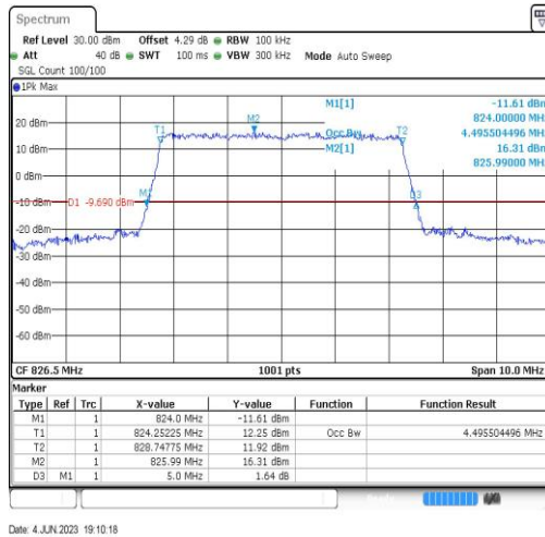
18(824-830)-5MHz-16QAM-23965-25RB#0
