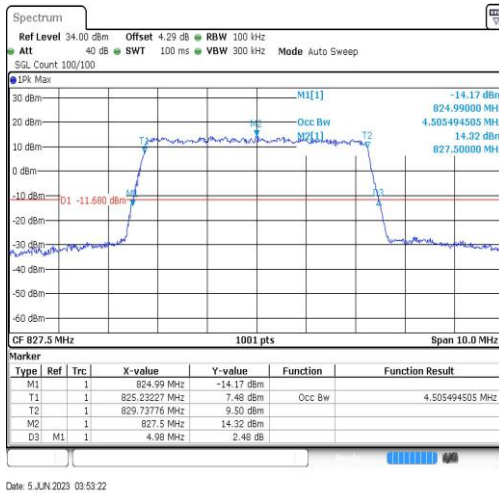
18(824-830)-5MHz-256QAM-23975-25RB#0
