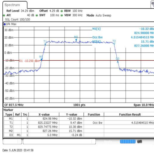
18(824-830)-5MHz-64QAM-23975-25RB#0
