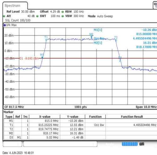
18(815-824)-5MHz-16QAM-23875-25RB#0
