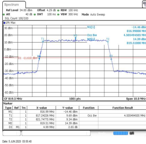
18(815-824)-5MHz-256QAM-23895-25RB#0
