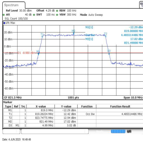
18(815-824)-5MHz-QPSK-23915-25RB#0
