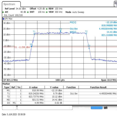
18(815-824)-5MHz-256QAM-23915-25RB#0
