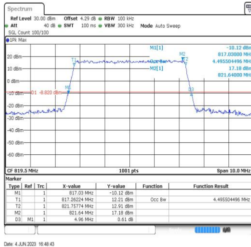
18(815-824)-5MHz-QPSK-23895-25RB#0
