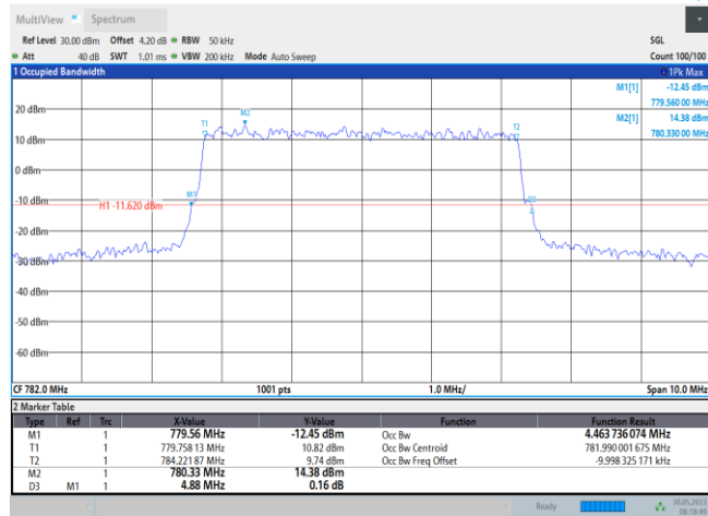
Band13-5MHz-QPSK-23230-25RB#0
