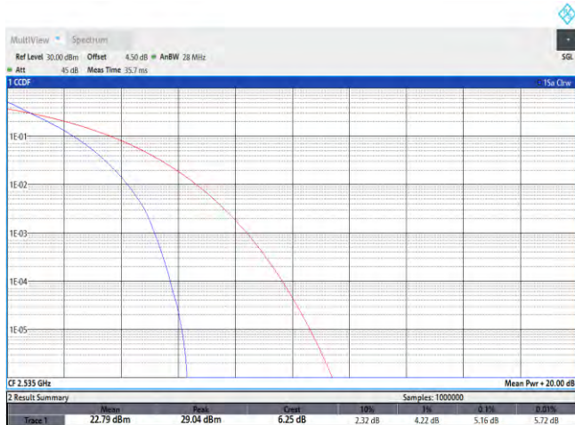
Band7-20MHz-QPSK-21100-100RB#0
