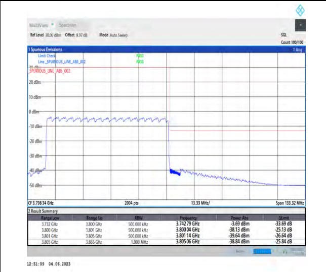
NTNV_N78-3700-3800_PC2_30_60_H_TID6_RID1#1
