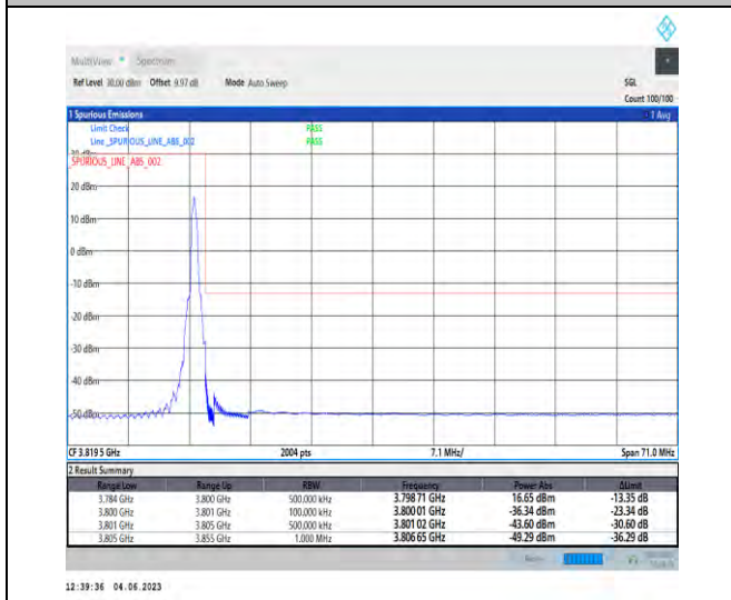
NTNV_N78-3700-3800_PC2_30_50_H_TID5_RID1#1
