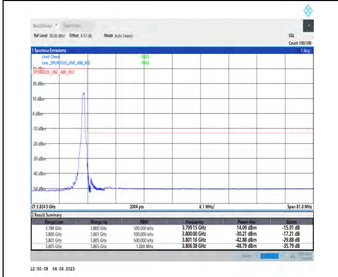
NTNV_N78-3700-3800_PC2_30_60_H_TID5_RID1#1
