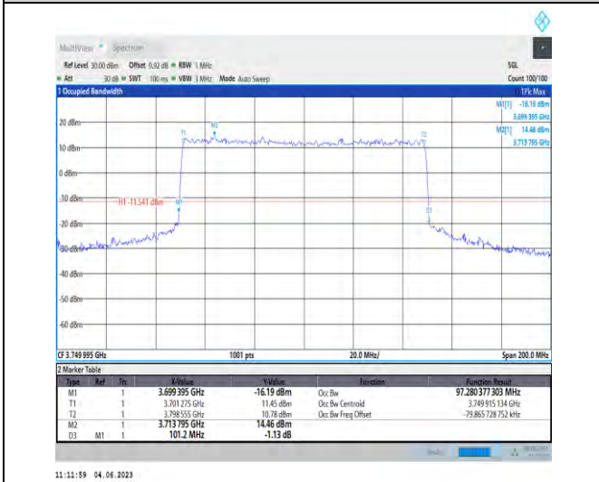
1-N78-3700-3800-PC2-30-100-M-6-CP-QPSK-Outer _Full-273@0-97.28-101.200-≤100-PASS
