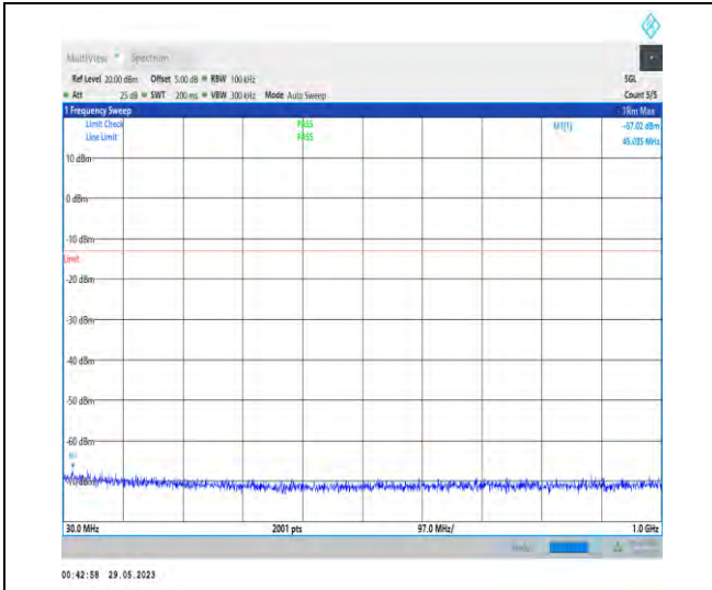
1-N78-3700-3800-PC3-30-100-M-1-N/A-DFT-PI2BP SK-Inner_1RB_Left-1@1-30-1000-45.04--67.02--13- PASS
