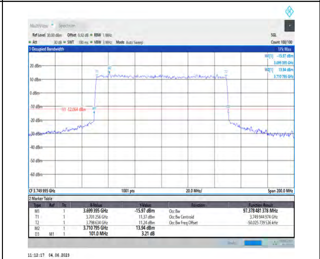
1-N78-3700-3800-PC2-30-100-M-7-CP-16QAM-Out er_Full-273@0-97.378-101.000-≤100-PASS
