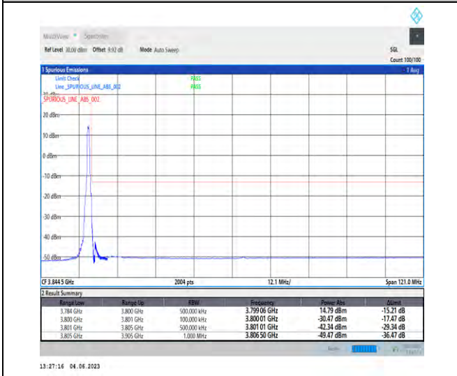
NTNV_N78-3700-3800_PC2_30_100_H_TID5_RID1#1
