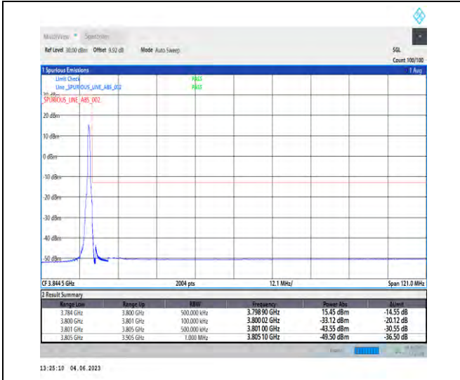
NTNV_N78-3700-3800_PC2_30_100_H_TID2_RID1#1
