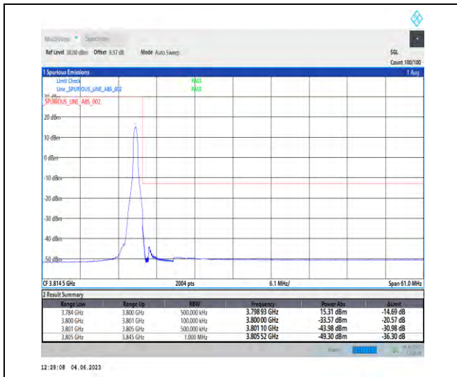
NTNV_N78-3700-3800_PC2_30_40_H_TID2_RID1#1
