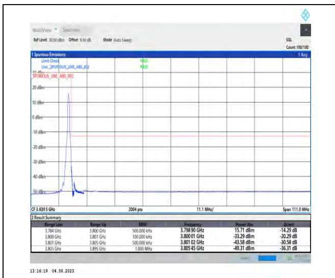
NTNV_N78-3700-3800_PC2_30_90_H_TID2_RID1#1
