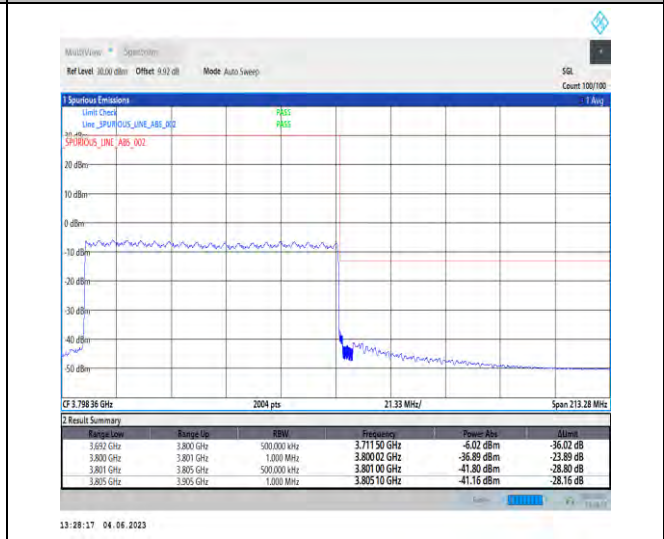
NTNV_N78-3700-3800_PC2_30_100_H_TID6_RID1#1
