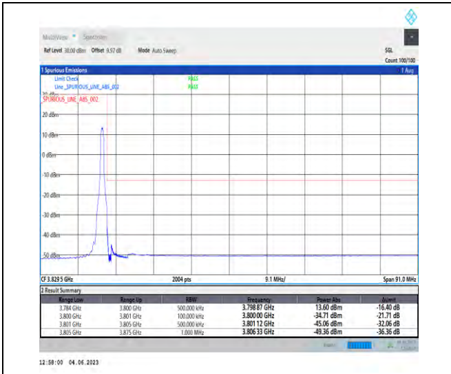
NTNV_N78-3700-3800_PC2_30_70_H_TID2_RID1#1
