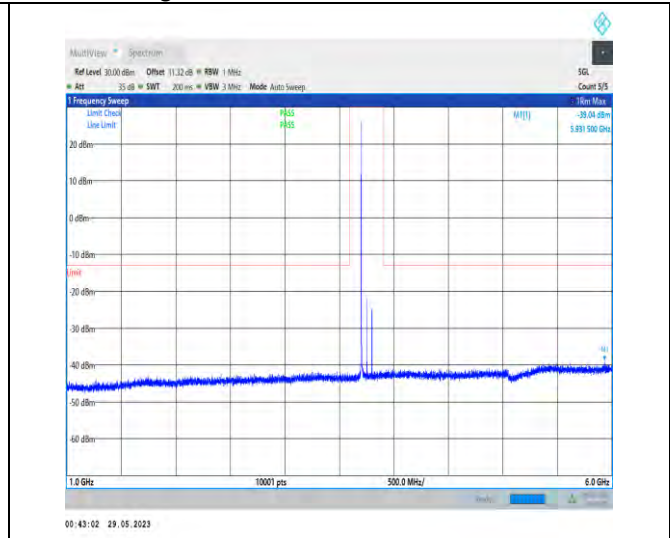
1-N78-3700-3800-PC3-30-100-M-1-N/A-DFT-PI2BPS K-Inner_1RB_Left-1@1-1000-6000-5931.50--39.04-- 13-PASS
