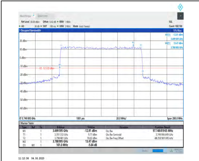
1-N78-3700-3800-PC2-30-100-M-8-CP-64QAM-Outer_Full-273@0-97.149-101.000-≤100-PASS
