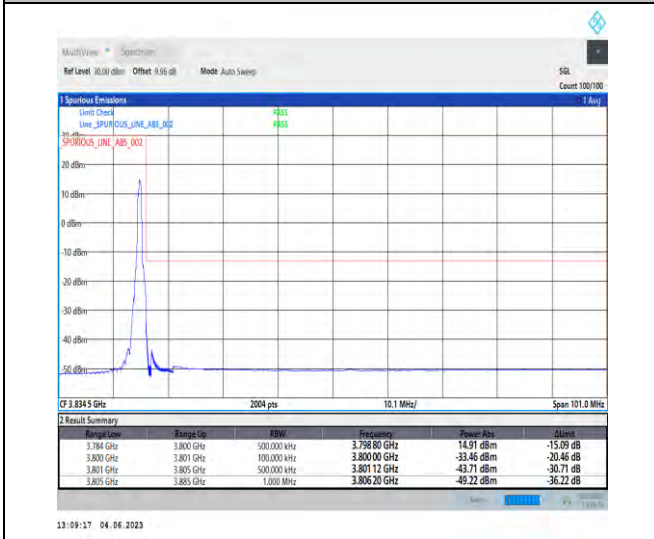
NTNV_N78-3700-3800_PC2_30_80_H_TID5_RID1#1
