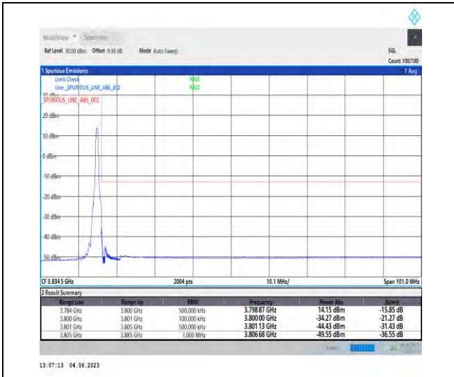
NTNV_N78-3700-3800_PC2_30_80_H_TID2_RID1#1
