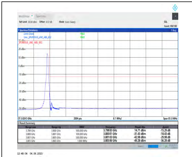
NTNV_N78-3700-3800_PC2_30_60_H_TID2_RID1#1
