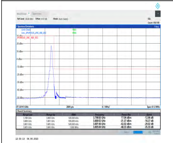
NTNV_N78-3700-3800_PC2_30_40_H_TID5_RID1#1
