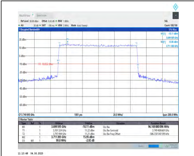
1-N78-3700-3800-PC2-30-100-M-4-DFT-64QAM-Out er_Full-270@0-96.17-99.800-≤100-PASS
