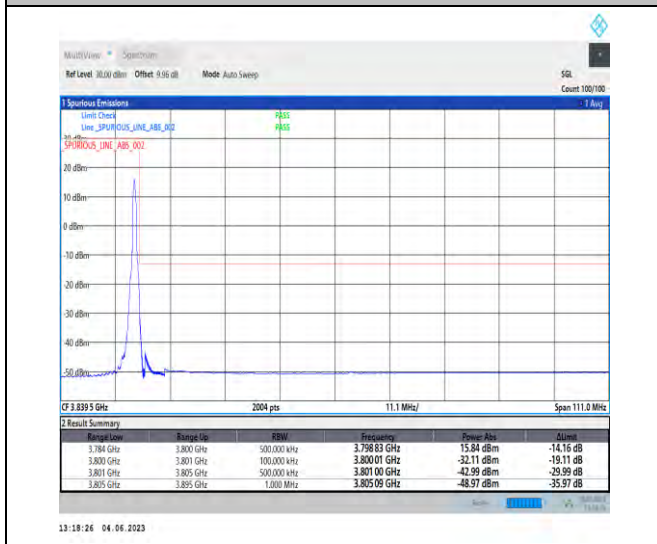
NTNV_N78-3700-3800_PC2_30_90_H_TID5_RID1#1
