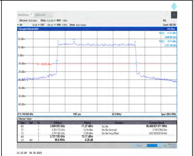
1-N78-3700-3800-PC2-30-100-M-3-DFT-16QAM-Outer_Full-270@0-96.407-99.800-≤100-PASS
