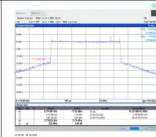
1-N78-3700-3800-PC2-30-70-M-8-CP-64QAM-Outer_Full-189@0-67.558-70.000-≤70-PASS
