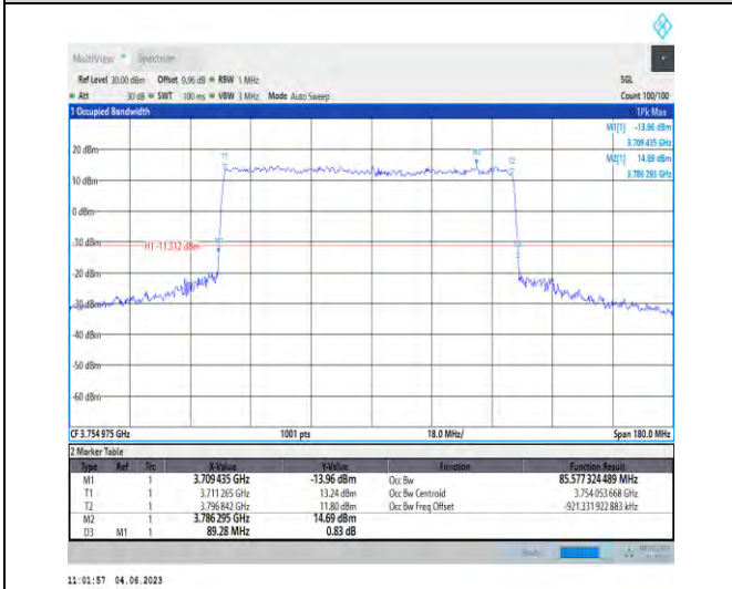
1-N78-3700-3800-PC2-30-90-H-4-DFT-64QAM-Outer _Full-240@0-85.577-89.280-≤90-PASS
