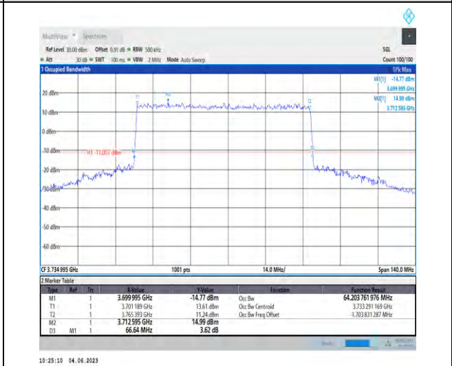
1-N78-3700-3800-PC2-30-70-L-1-DFT-QPSK-Outer _Full-180@0-64.204-66.640-≤70-PASS
