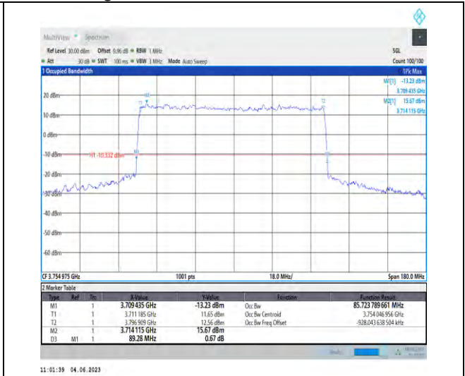
1-N78-3700-3800-PC2-30-90-H-3-DFT-16QAM-Out er_Full-240@0-85.724-89.280-≤90-PASS
