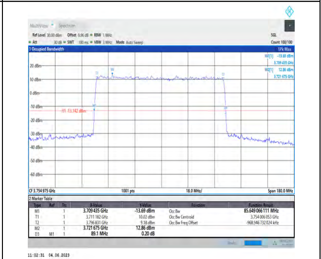
1-N78-3700-3800-PC2-30-90-H-5-DFT-256QAM-Outer _Full-240@0-85.649-89.100-≤90-PASS
