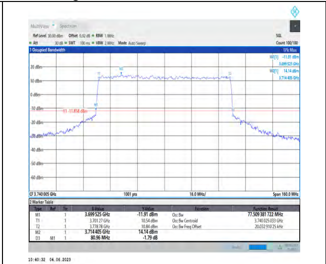
1-N78-3700-3800-PC2-30-80-L-8-CP-64QAM-Outer_Full-217@0-77.509-80.960-≤80-PASS
