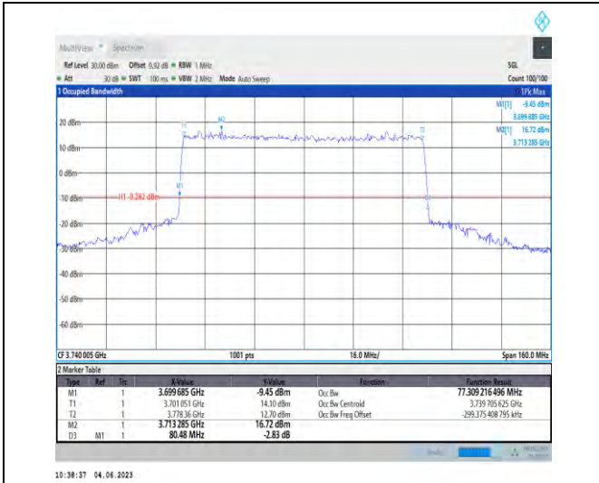
1-N78-3700-3800-PC2-30-80-L-3-DFT-16QAM-Outer_Full-216@0-77.309-80.480-≤80-PASS
