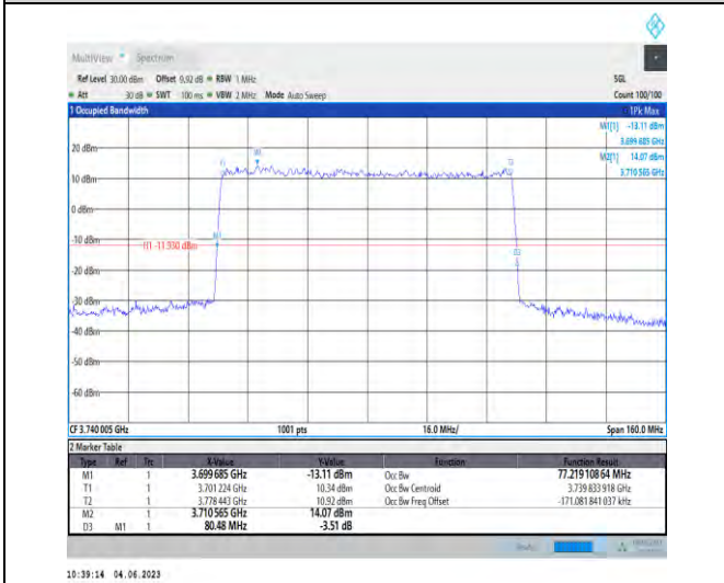
1-N78-3700-3800-PC2-30-80-L-5-DFT-256QAM-Outer_Full-216@0-77.219-80.480-≤80-PASS
