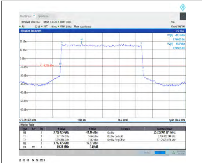
1-N78-3700-3800-PC2-30-90-H-2-DFT-PI2BPSK-Out er_Full-240@0-85.726-89.280-≤90-PASS
