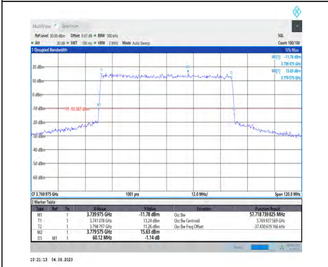
1-N78-3700-3800-PC2-30-60-H-1-DFT-QPSK-Outer_Full-162@0-57.719-60.120-≤60-PASS
