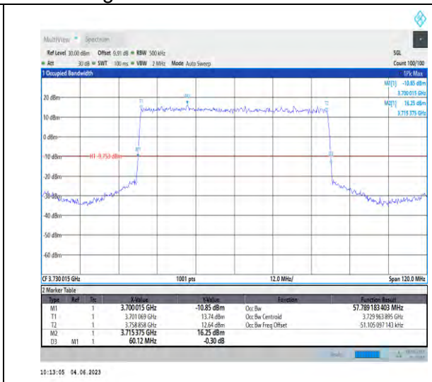
1-N78-3700-3800-PC2-30-60-L-2-DFT-PI2BPSK-Outer_Full-162@0-57.789-60.120-≤60-PASS
