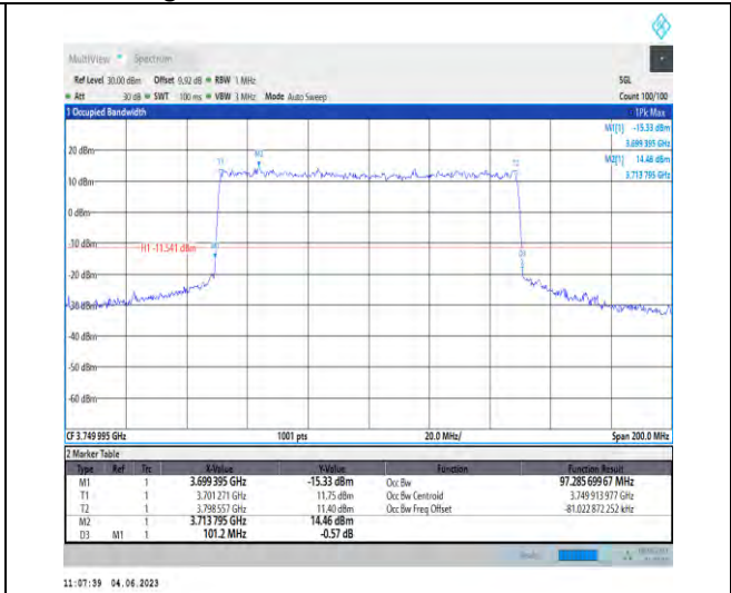
1-N78-3700-3800-PC2-30-100-L-6-CP-QPSK-Outer_Full-273@0-97.286-101.200-≤100-PASS
