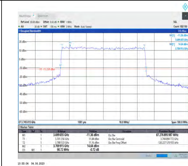
1-N78-3700-3800-PC2-30-90-L-7-CP-16QAM-Outer_Full-245@0-87.277-90.720-≤90-PASS
