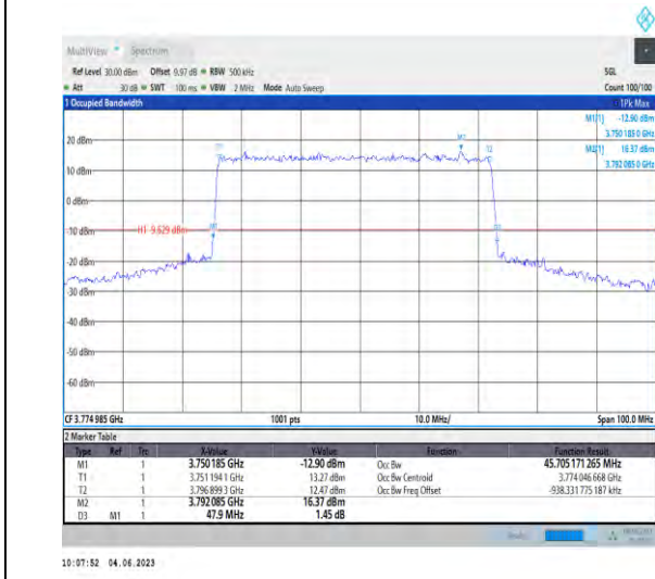
1-N78-3700-3800-PC2-30-50-H-1-DFT-QPSK-Outer_Full-128@0-45.705-47.900-≤50-PASS
