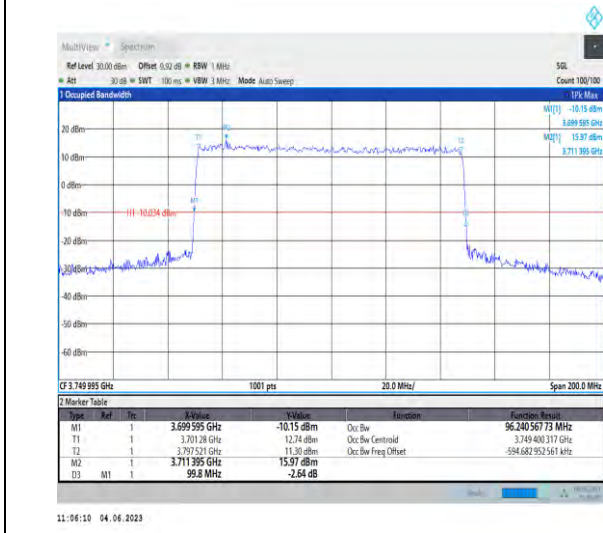
1-N78-3700-3800-PC2-30-100-L-4-DFT-64QAM-Outer_Full-270@0-96.241-99.800-≤100-PASS
