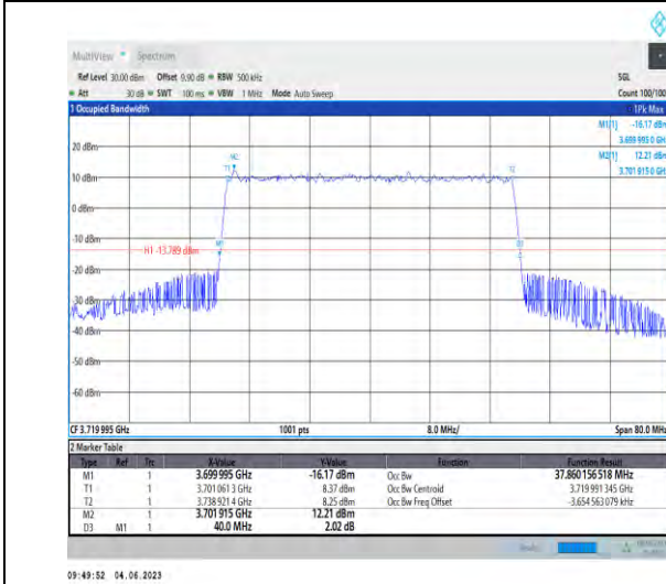
1-N78-3700-3800-PC2-30-40-L-9-CP-256QAM-Outer_Full-106@0-37.86-40.000-≤40-PASS
