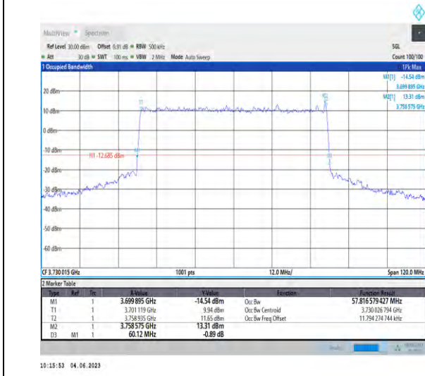
1-N78-3700-3800-PC2-30-60-L-8-CP-64QAM-Outer_Full-162@0-57.817-60.120-≤60-PASS
