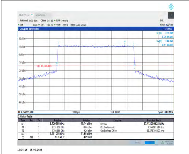
1-N78-3700-3800-PC2-30-70-H-6-CP-QPSK-Outer_Full-189@0-67.412-70.000-≤70-PASS
