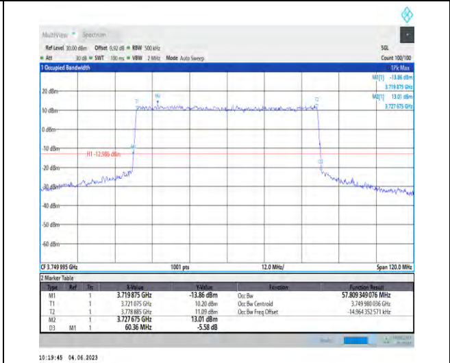
1-N78-3700-3800-PC2-30-60-M-7-CP-16QAM-Outer_Full-162@0-57.809-60.360-≤60-PASS
