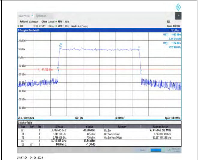
1-N78-3700-3800-PC2-30-80-M-9-CP-256QAM-Outer_Full-217@0-77.417-80.800≤80-PASS
