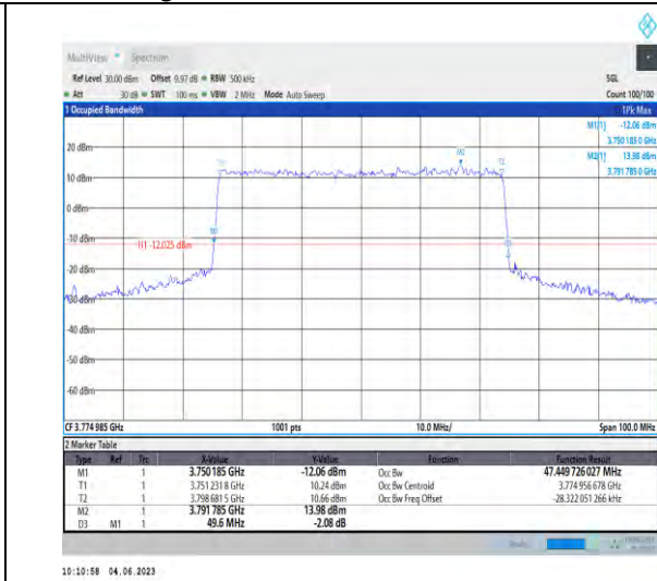
1-N78-3700-3800-PC2-30-50-H-7-CP-16QAM-Outer_Full-133@0-47.45-49.600-≤50-PASS
