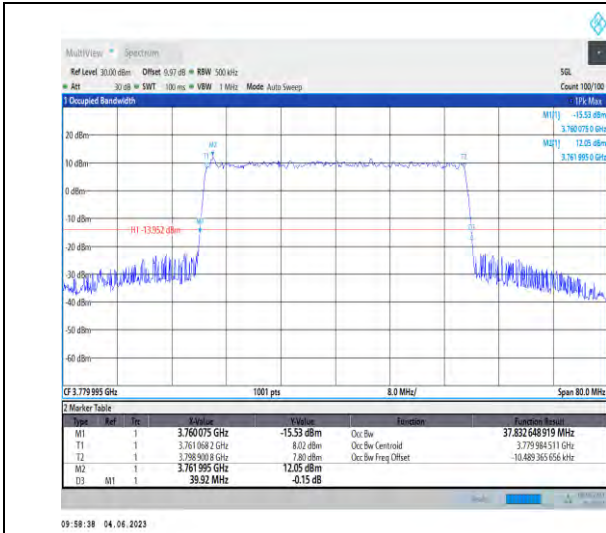
1-N78-3700-3800-PC2-30-40-H-9-CP-256QAM-Outer_Full-106@0-37.833-39.920-≤40-PASS
