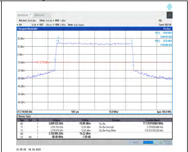
1-N78-3700-3800-PC2-30-80-L-4-DFT-64QAM-Outer_Full-216@0-77.177-80.480-≤80-PASS
