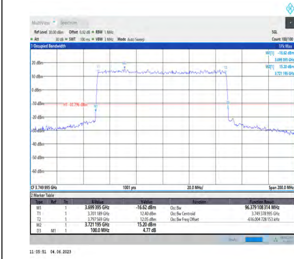
1-N78-3700-3800-PC2-30-100-L-3-DFT-16QAM-Outer_Full-270@0-96.379-100.000-≤100-PASS
