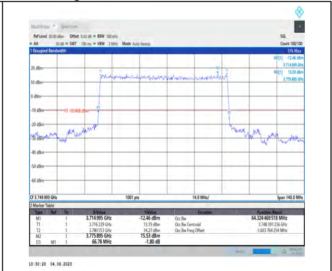
1-N78-3700-3800-PC2-30-70-M-2-DFT-PI2BPSK-Outer_Full-180@0-64.324-66.780-≤70-PASS
