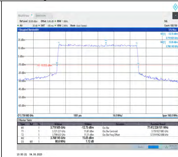
1-N78-3700-3800-PC2-30-80-H-6-CP-QPSK-Outer_Full-217@0-77.412-80.800-≤80-PASS
