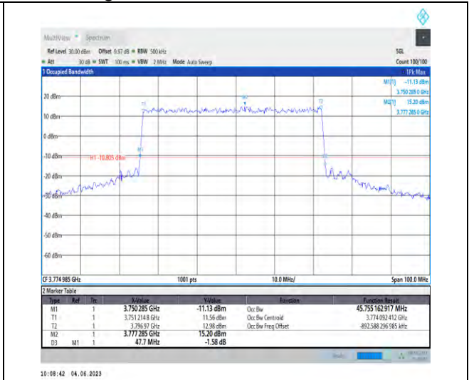
1-N78-3700-3800-PC2-30-50-H-3-DFT-16QAM-Out er_Full-128@0-45.755-47.700-≤50-PASS
