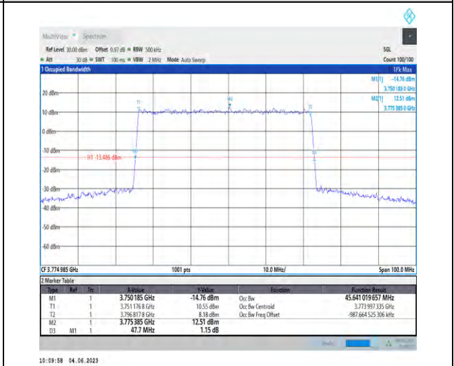
1-N78-3700-3800-PC2-30-50-H-5-DFT-256QAM-Outer _Full-128@0-45.641-47.700-≤50-PASS
