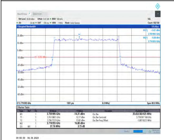
1-N78-3700-3800-PC2-30-40-H-3-DFT-16QAM-Outer_Full-100@0-35.653-37.760-≤40-PASS
