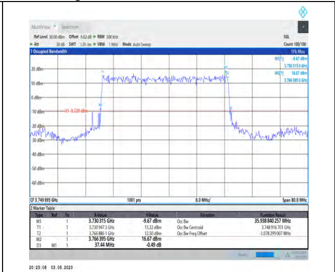
1-N78-3700-3800-PC2-30-40-M-3-DFT-16QAM-Out er_Full-100@0-35.939-37.44-≤40-PASS
