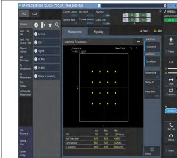
1-N78-3700-3800-30-100-M-7-CP-16QAM-Outer_Full-273@0-see graph-PASS
