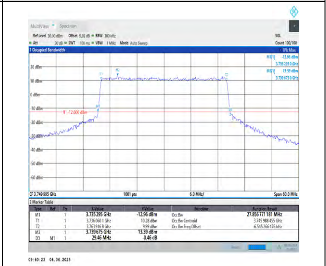
1-N78-3700-3800-PC2-30-30-M-8-CP-64QAM-Outer _Full-78@0-27.857-29.460-≤30-PASS
