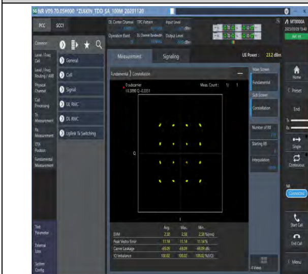
1-N78-3700-3800-30-100-M-3-DFT-16QAM-Outer_Full-270@0-see graph-PASS
