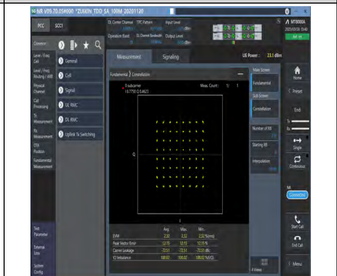
1-N78-3700-3800-30-100-M-4-DFT-64QAM-Outer_Full-270@0-see graph-PASS
