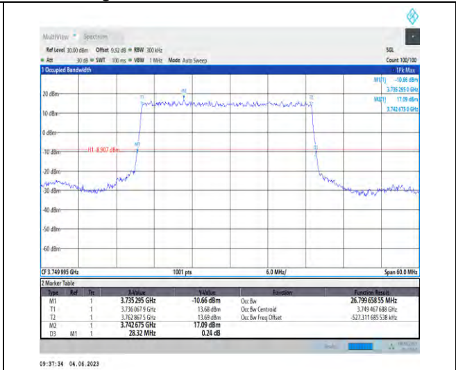
1-N78-3700-3800-PC2-30-30-M-2-DFT-PI2BPSK-Outer_Full-75@0-26.8-28.320-≤30-PASS
