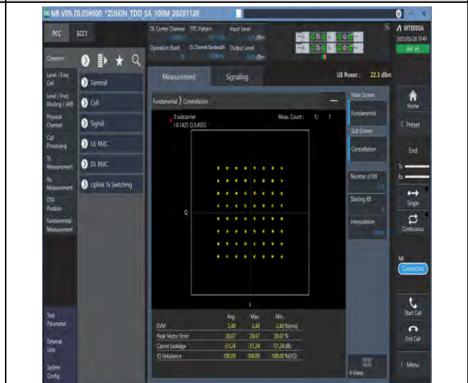
1-N78-3700-3800-30-100-M-8-CP-64QAM-Outer_Full-273@0-see graph-PASS
