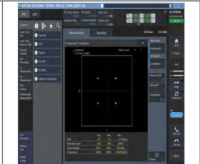
1-N78-3700-3800-30-100-M-2-DFT-QPSK-Outer_Full-270@0-see graph-PASS
