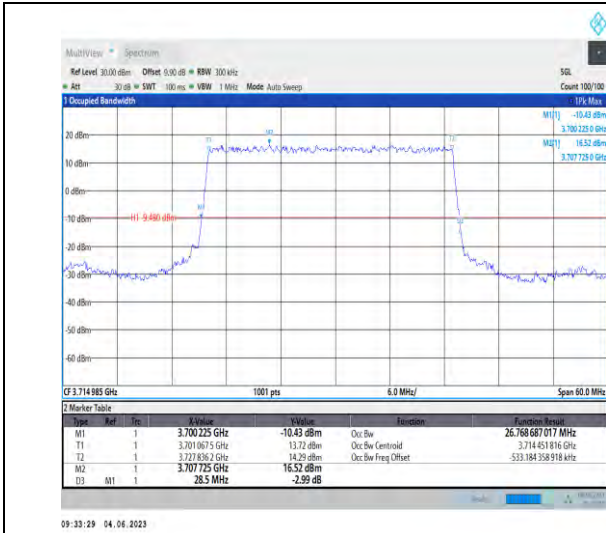
1-N78-3700-3800-PC2-30-30-L-2-DFT-PI2BPSK-Out er_Full-75@0-26.769-28.500-≤30-PASS
