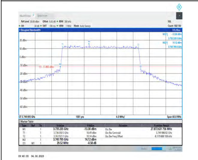
1-N78-3700-3800-PC2-30-30-M-7-CP-16QAM-Outer _Full-78@0-27.873-29.520-≤30-PASS
