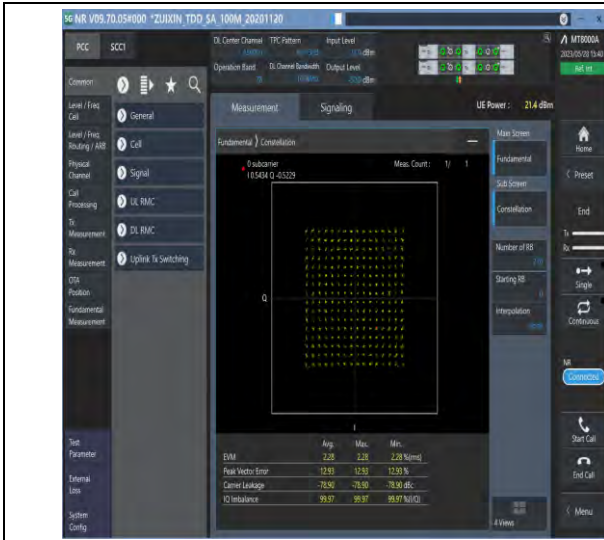
1-N78-3700-3800-30-100-M-5-DFT-256QAM-Outer_Full-270@0-see graph-PASS
