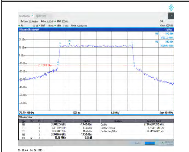
1-N78-3700-3800-PC2-30-30-L-8-CP-64QAM-Outer_Full-78@0-27.865-29.460-≤30-PASS
