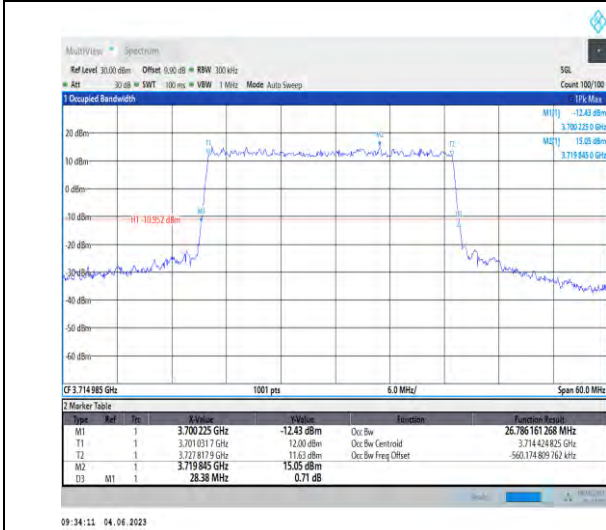
1-N78-3700-3800-PC2-30-30-L-4-DFT-64QAM-Out _Full-75@0-26.786-28.380-≤30-PASS
