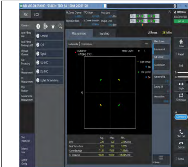
1-N78-3700-3800-30-100-M-1-DFT-PI2BPSK-Outer_Full-270@0-see graph-PASS
