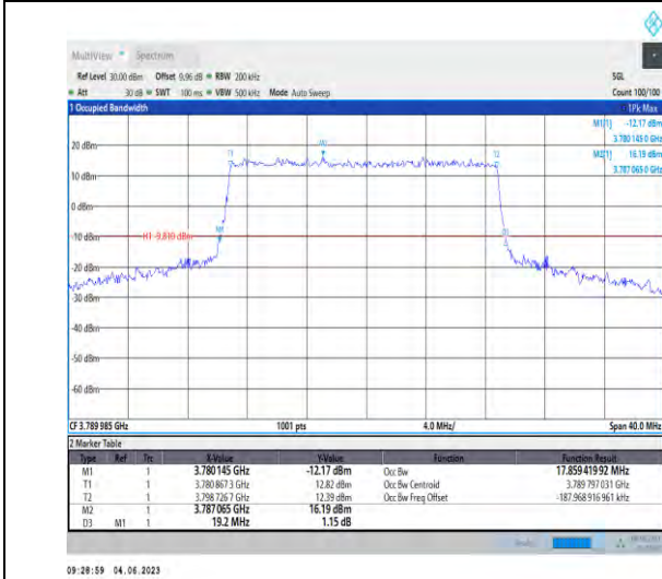
1-N78-3700-3800-PC2-30-20-H-1-DFT-QPSK-Outer_Full-50@0-17.859-19.200-≤20-PASS
