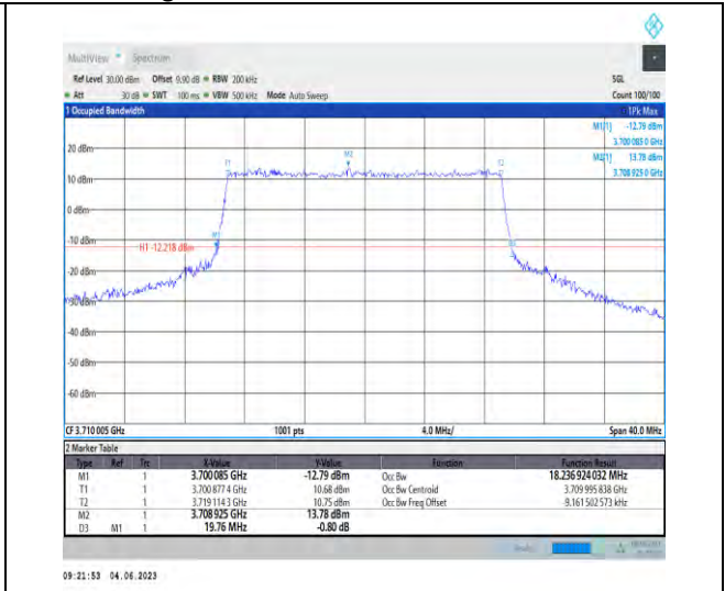
1-N78-3700-3800-PC2-30-20-L-6-CP-QPSK-Outer_Full-51@0-18.237-19.760-≤20-PASS
