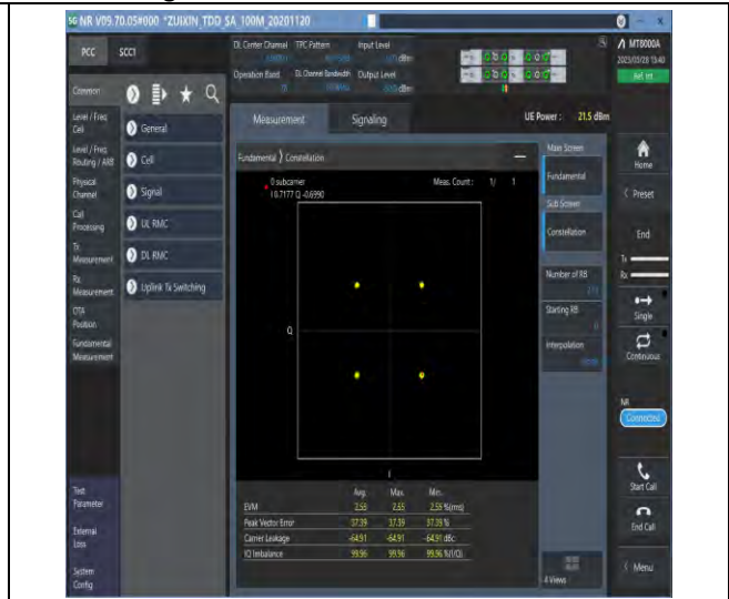
1-N78-3700-3800-30-100-M-6-CP-QPSK-Outer_Full-273@0-see graph-PASS
