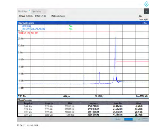
1-N78-3450-3550-PC2-30-50-H-5-CP-QPSK-Edge_1RB_Right-1@132-1--PASS-see graph
