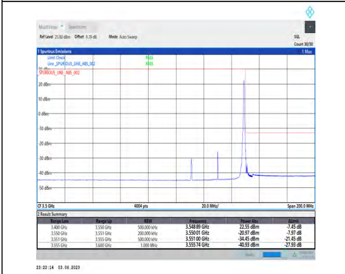
1-N78-3450-3550-PC2-30-40-H-5-CP-QPSK-Edge_1RB_Right-1@105-1--PASS-see graph
