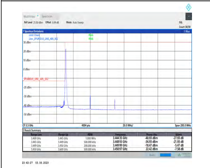
1-N78-3450-3550-PC2-30-60-L-4-CP-QPSK-Edge_1RB_Left-1@0-1--PASS-see graph
