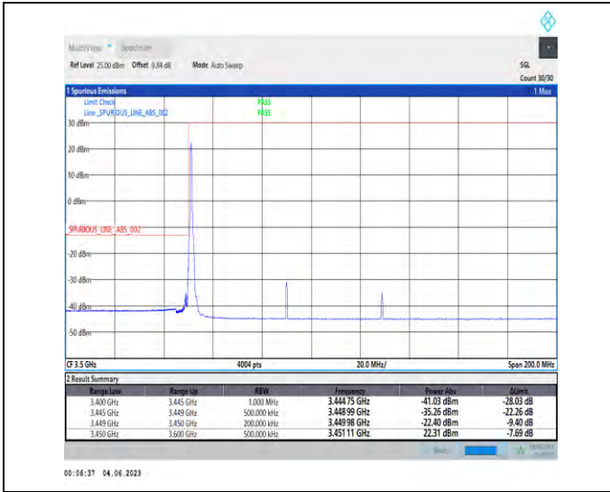
1-N78-3450-3550-PC2-30-80-L-1-DFT-PI2BPSK-Edge_1RB_Left-1@0-1--PASS-see graph
