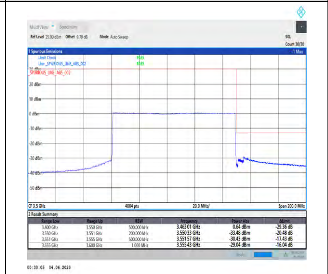
1-N78-3450-3550-PC2-30-90-H-6-CP-QPSK-Outer_Full-245@0-1--PASS-see graph
