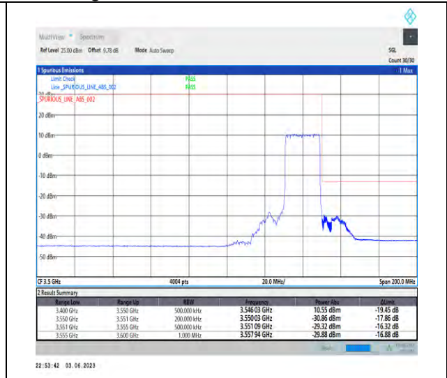
1-N78-3450-3550-PC2-30-20-H-3-DFT-PI2BPSK-Outer_Full-50@0-1--PASS-see graph
