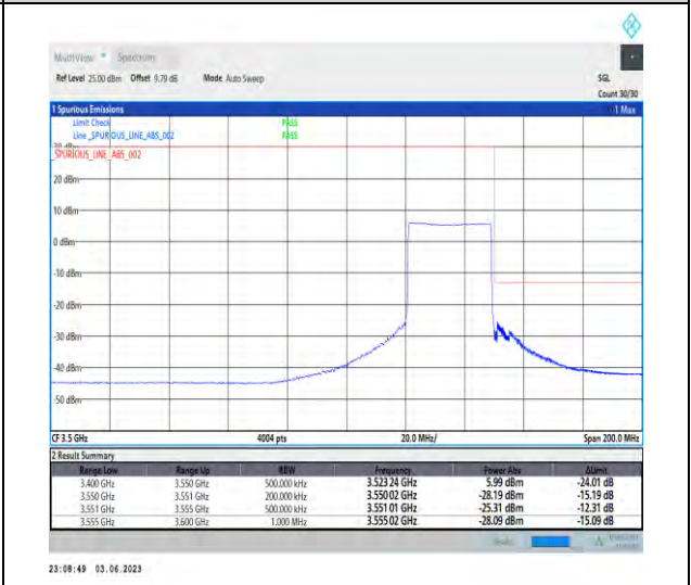
1-N78-3450-3550-PC2-30-30-H-6-CP-QPSK-Outer_Full-78@0-1--PASS-see graph
