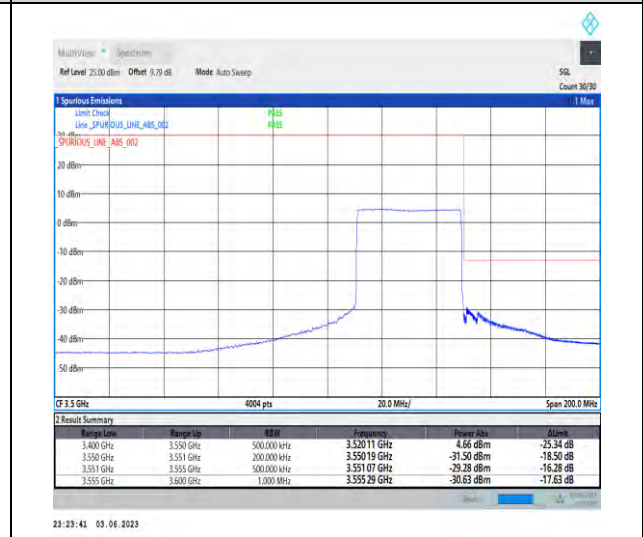
1-N78-3450-3550-PC2-30-40-H-6-CP-QPSK-Outer_Full-106@0-1--PASS-see graph
