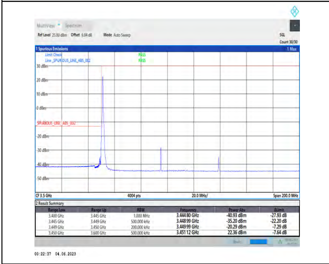
1-N78-3450-3550-PC2-30-90-L-4-CP-QPSK-Edge_1RB_Left-1@0-1--PASS-see graph
