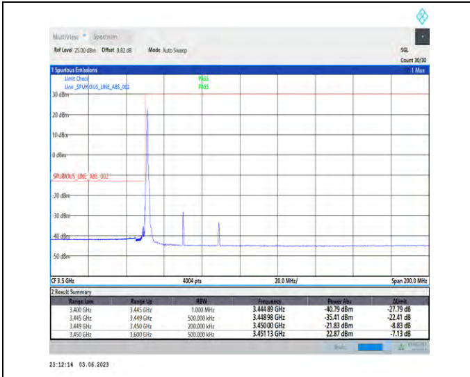
1-N78-3450-3550-PC2-30-40-L-1-DFT-PI2BPSK-Edge_1RB_Left-1@0-1--PASS-see graph
