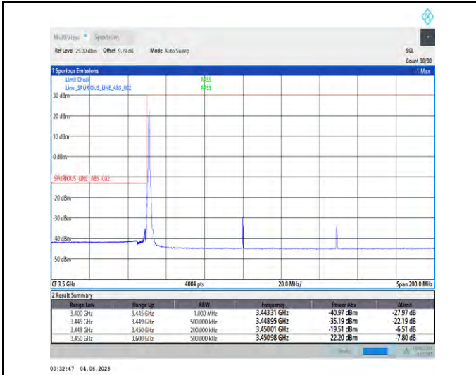
1-N78-3450-3550-PC2-30-100-L-1-DFT-PI2BPSK-Edge_e_1RB_Left-1@0-1--PASS-see graph
