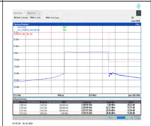
1-N78-3450-3550-PC2-30-70-H-6-CP-QPSK-Outer_Full-189@0-1--PASS-see graph
