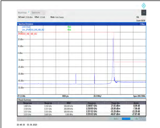
1-N78-3450-3550-PC2-30-60-H-2-DFT-PI2BPSK-Edge_1RB_Right-1@161-1--PASS-see graph
