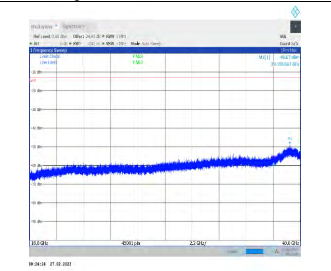
1-N78-3450-3550-PC2-30-100-L-1-N/A-DFT-PI2BPS K-Inner_1RB_Left-1@1-18000-40000-18000.00--62. 71--13-PASS
