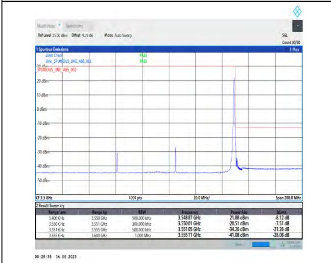
1-N78-3450-3550-PC2-30-90-H-5-CP-QPSK-Edge_1RB_Right-1@244-1--PASS-see graph
