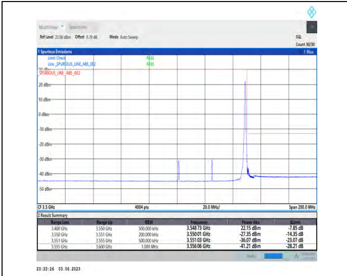
1-N78-3450-3550-PC2-30-50-H-2-DFT-PI2BPSK-Edge_1RB_Right-1@132-1--PASS-see graph
