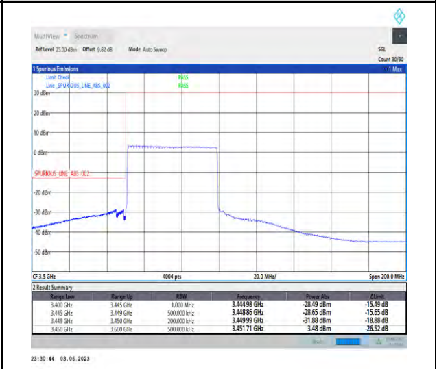
1-N78-3450-3550-PC2-30-50-L-6-CP-QPSK-Outer_Full-133@0-1--PASS-see graph
