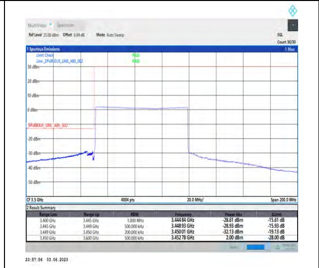
1-N78-3450-3550-PC2-30-70-L-6-CP-QPSK-Outer_Full-189@0-1--PASS-see graph
