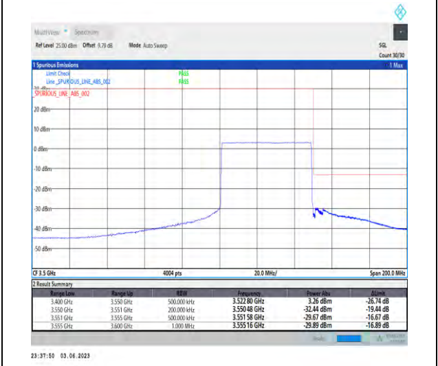
1-N78-3450-3550-PC2-30-50-H-6-CP-QPSK-Outer_Full-133@0-1--PASS-see graph
