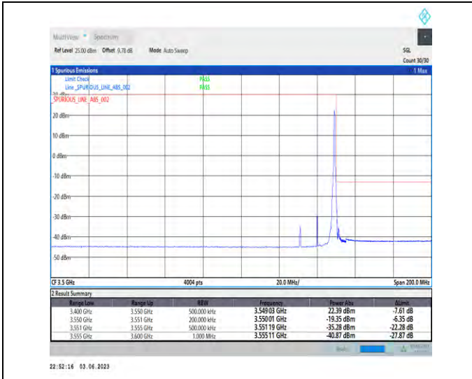
1-N78-3450-3550-PC2-30-20-H-2-DFT-PI2BPSK-Edge_1RB_Right-1@50-1--PASS-see graph
