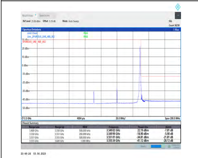
1-N78-3450-3550-PC2-30-60-H-5-CP-QPSK-Edge_1RB_Right-1@161-1--PASS-see graph
