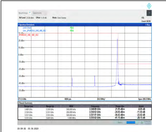
1-N78-3450-3550-PC2-30-70-H-2-DFT-PI2BPSK-Edge_1RB_Right-1@188-1--PASS-see graph
