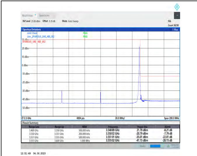
1-N78-3450-3550-PC2-30-100-H-2-DFT-PI2BPSK-Edge_e_1RB_Right-1@272-1--PASS-see graph
