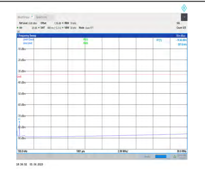
1-N78-3450-3550-PC2-30-100-M-1-N/A-DFT-PI2BPS K-Inner_1RB_Left-1@1-0.15-30-0.60--76.46--33-PAS S
