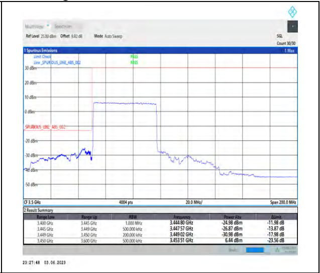
1-N78-3450-3550-PC2-30-50-L-3-DFT-PI2BPSK-Outer_Full-128@0-1--PASS-see graph
