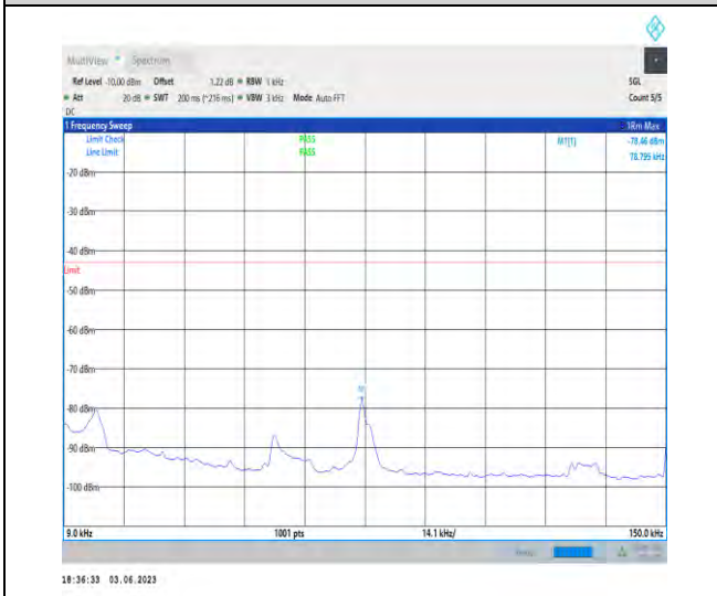
1-N78-3450-3550-PC2-30-100-M-1-N/A-DFT-PI2BP SK-Inner_1RB_Left-1@1-0.009-0.15-0.08--78.46--4 3-PASS
