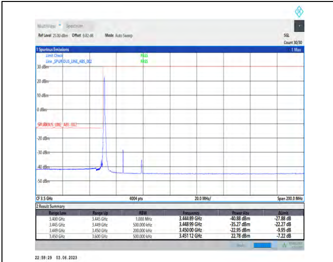
1-N78-3450-3550-PC2-30-30-L-1-DFT-PI2BPSK-Edge_1RB_Left-1@0-1--PASS-see graph
