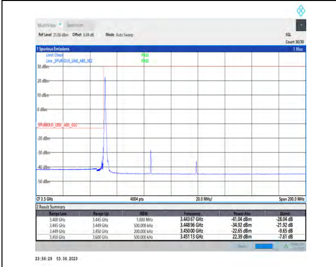
1-N78-3450-3550-PC2-30-70-L-4-CP-QPSK-Edge_1RB_Left-1@0-1--PASS-see graph
