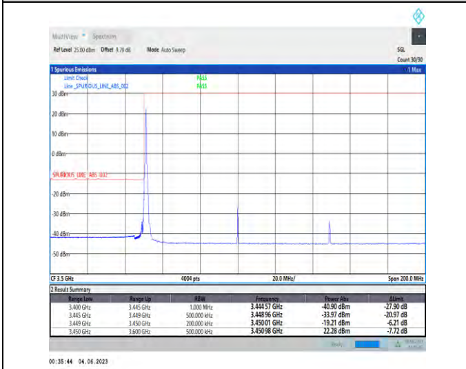
1-N78-3450-3550-PC2-30-100-L-4-CP-QPSK-Edge_1RB_Left-1@0-1--PASS-see graph
