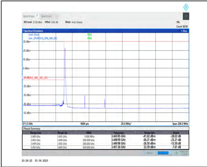
1-N78-3450-3550-PC2-30-50-L-1-DFT-PI2BPSK-Edge_1RB_Left-1@0-1--PASS-see graph
