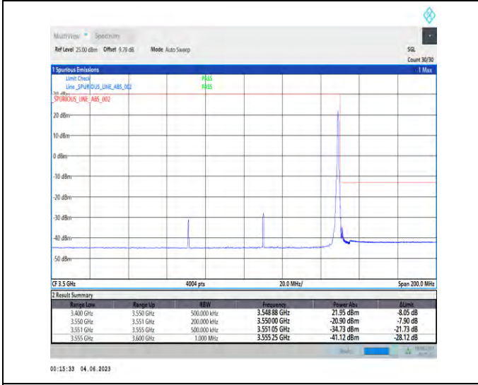
1-N78-3450-3550-PC2-30-80-H-5-CP-QPSK-Edge_1RB_Right-1@216-1--PASS-see graph
