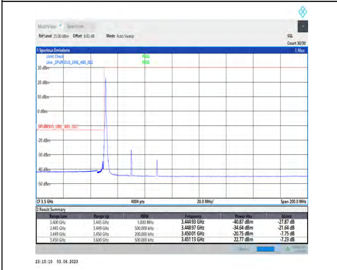
1-N78-3450-3550-PC2-30-40-L-4-CP-QPSK-Edge_1RB_Left-1@0-1--PASS-see graph
