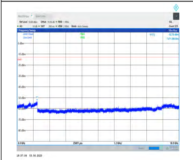
1-N78-3450-3550-PC2-30-100-M-1-N/A-DFT-PI2BP SK-Inner_1RB_Left-1@1-6000-18000-7471.20--52.7 0--13-PASS
