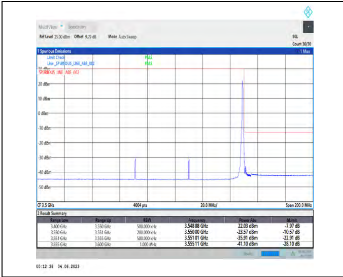
1-N78-3450-3550-PC2-30-80-H-2-DFT-PI2BPSK-Edge_1RB_Right-1@216-1--PASS-see graph
