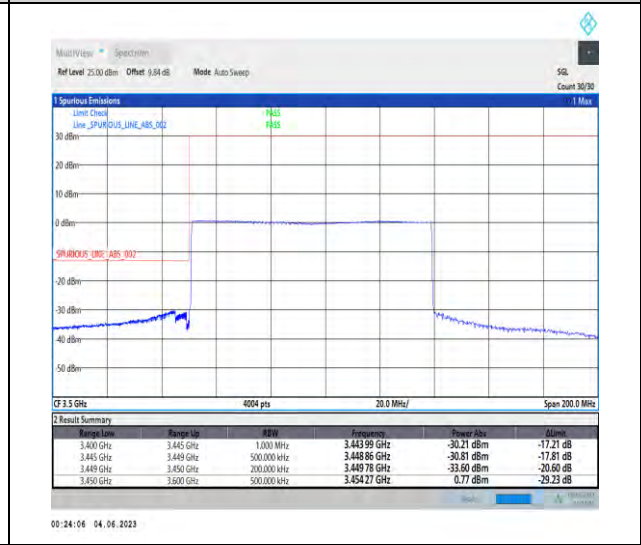
1-N78-3450-3550-PC2-30-90-L-6-CP-QPSK-Outer_Full-245@0-1--PASS-see graph
