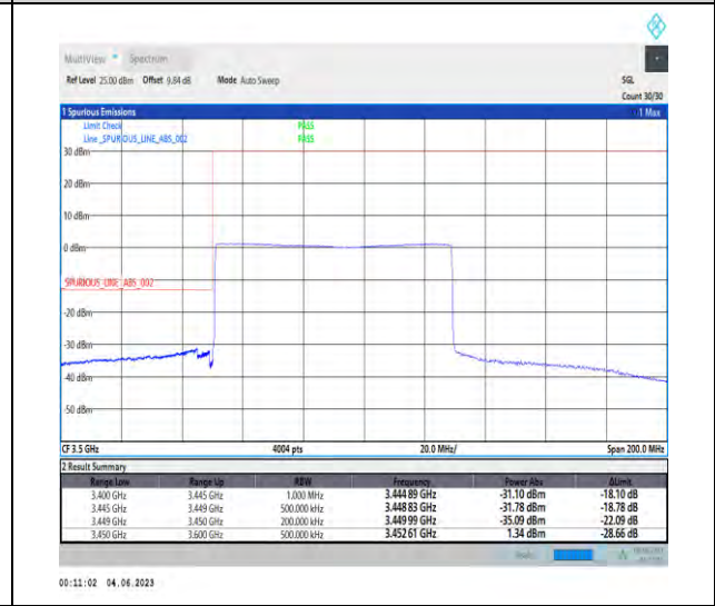
1-N78-3450-3550-PC2-30-80-L-6-CP-QPSK-Outer_Full-217@0-1--PASS-see graph
