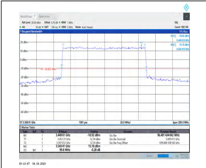
1-N78-3450-3550-PC2-30-100-H-3-DFT-16QAM-Out er_Full-270@0-96.401-99.800-≤100-PASS
