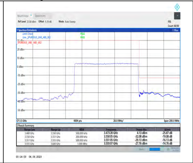
1-N78-3450-3550-PC2-30-80-H-3-DFT-PI2BPSK-Outer_Full-216@0-1--PASS-see graph
