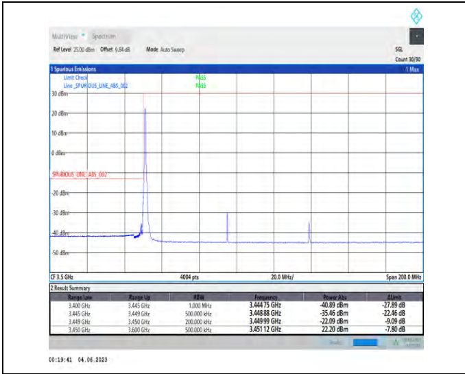
1-N78-3450-3550-PC2-30-90-L-1-DFT-PI2BPSK-Edge_1RB_Left-1@0-1--PASS-see graph
