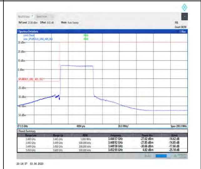
1-N78-3450-3550-PC2-30-40-L-6-CP-QPSK-Outer_Full-106@0-1--PASS-see graph
