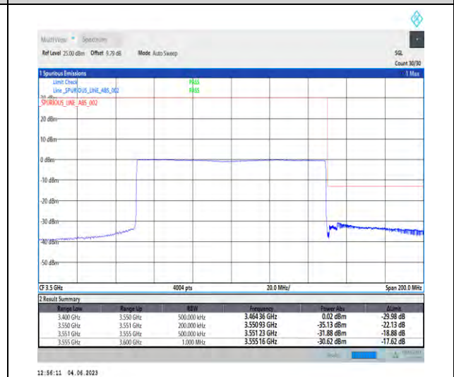
1-N78-3450-3550-PC2-30-100-H-6-CP-QPSK-Outer_Full-273@0-1--PASS-see graph
