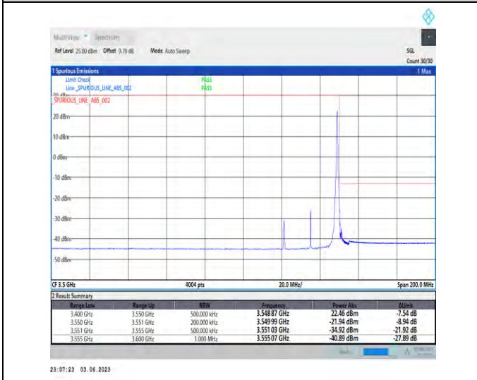
1-N78-3450-3550-PC2-30-30-H-5-CP-QPSK-Edge_1RB_Right-1@77-1--PASS-see graph
