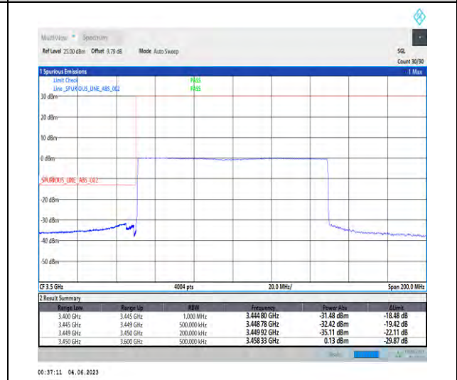
1-N78-3450-3550-PC2-30-100-L-6-CP-QPSK-Outer_Full-273@0-1--PASS-see graph
