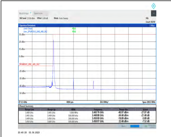
1-N78-3450-3550-PC2-30-60-L-1-DFT-PI2BPSK-Edge_1RB_Left-1@0-1--PASS-see graph
