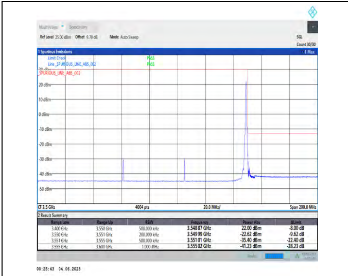
1-N78-3450-3550-PC2-30-90-H-2-DFT-PI2BPSK-Edge_1RB_Right-1@244-1--PASS-see graph
