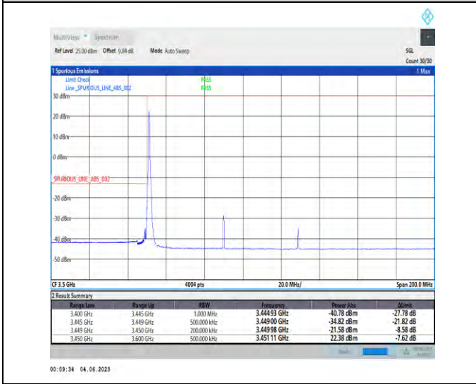
1-N78-3450-3550-PC2-30-80-L-4-CP-QPSK-Edge_1RB_Left-1@0-1--PASS-see graph
