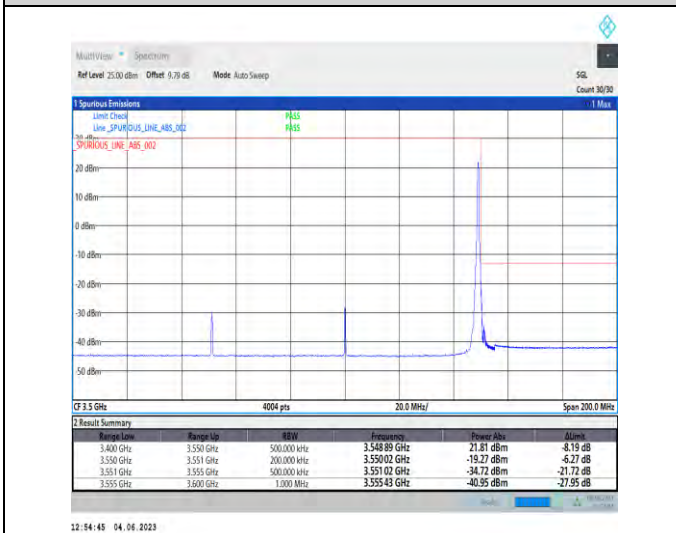
1-N78-3450-3550-PC2-30-100-H-5-CP-QPSK-Edge_1RB_Right-1@272-1--PASS-see graph
