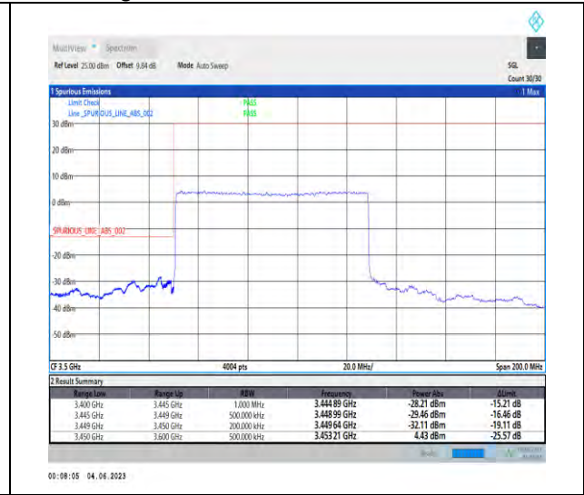
1-N78-3450-3550-PC2-30-80-L-3-DFT-PI2BPSK-Outer_Full-216@0-1--PASS-see graph
