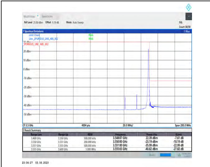
1-N78-3450-3550-PC2-30-30-H-2-DFT-PI2BPSK-Edge_1RB_Right-1@77-1--PASS-see graph
