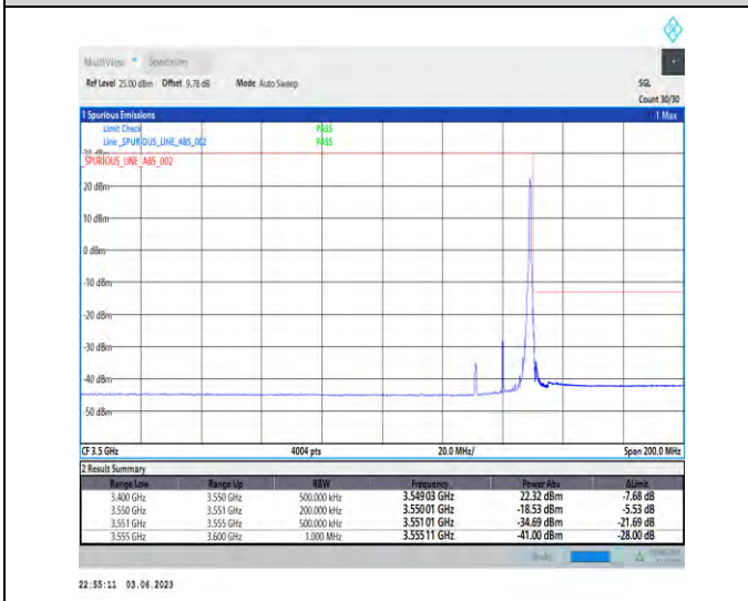
1-N78-3450-3550-PC2-30-20-H-5-CP-QPSK-Edge_1RB_Right-1@50-1--PASS-see graph
