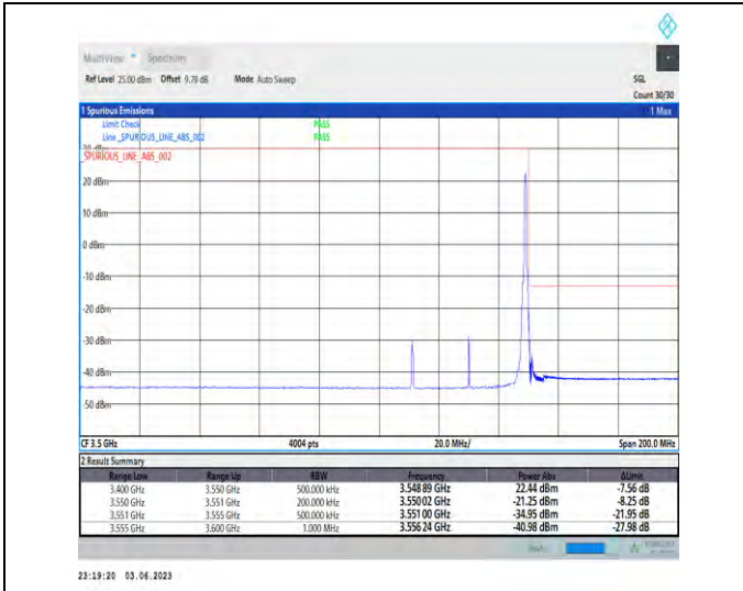
1-N78-3450-3550-PC2-30-40-H-2-DFT-PI2BPSK-Edge_1RB_Right-1@105-1--PASS-see graph
