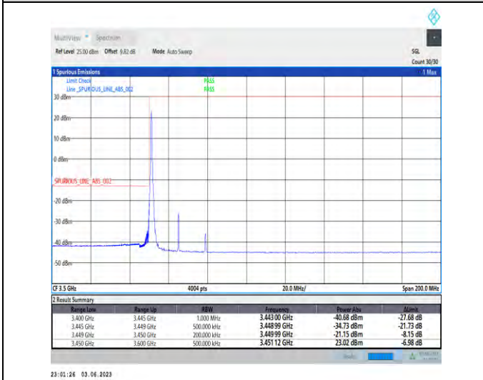
1-N78-3450-3550-PC2-30-30-L-4-CP-QPSK-Edge_1RB_Left-1@0-1--PASS-see graph
