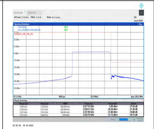
1-N78-3450-3550-PC2-30-60-H-6-CP-QPSK-Outer_Full-162@0-1--PASS-see graph
