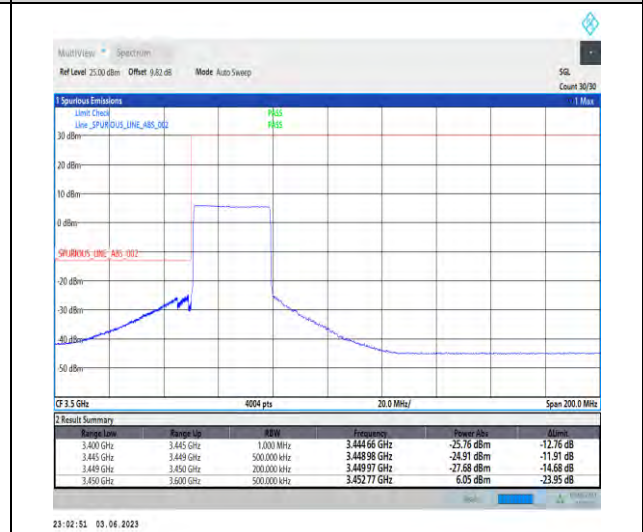
1-N78-3450-3550-PC2-30-30-L-6-CP-QPSK-Outer_Full-78@0-1--PASS-see graph
