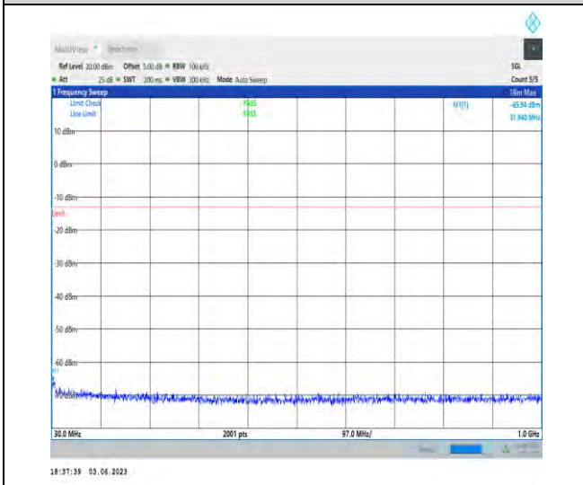
1-N78-3450-3550-PC2-30-100-H-1-N/A-DFT-PI2BP SK-Inner_1RB_Left-1@1-30-1000-31.94--65.94--13- PASS
