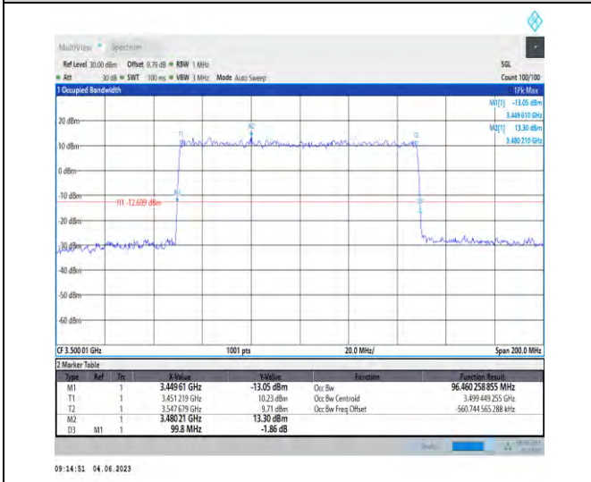
1-N78-3450-3550-PC2-30-100-H-5-DFT-256QAM-Ou ter_Full-270@0-96.46-99.800-≤100-PASS
