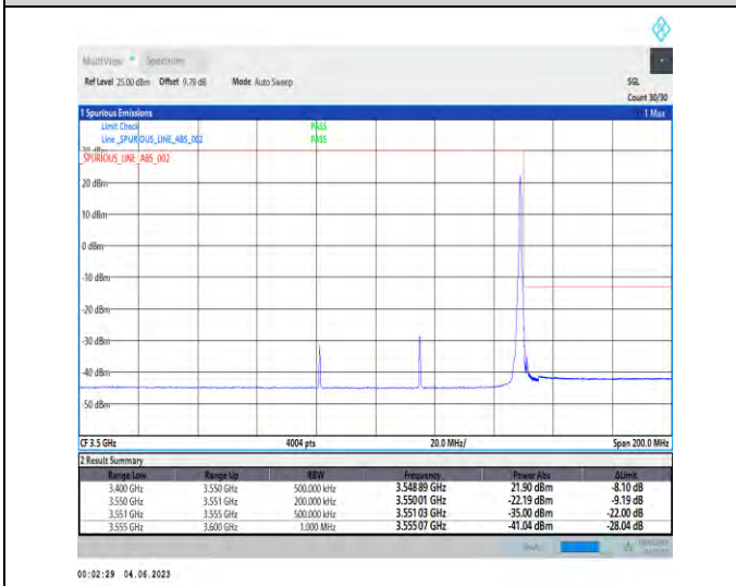
1-N78-3450-3550-PC2-30-70-H-5-CP-QPSK-Edge_1RB_Right-1@188-1--PASS-see graph
