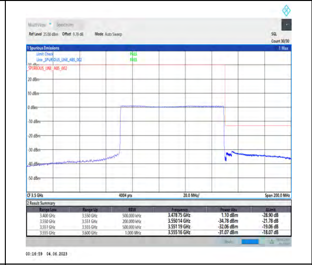
1-N78-3450-3550-PC2-30-80-H-6-CP-QPSK-Outer_Full-217@0-1--PASS-see graph
