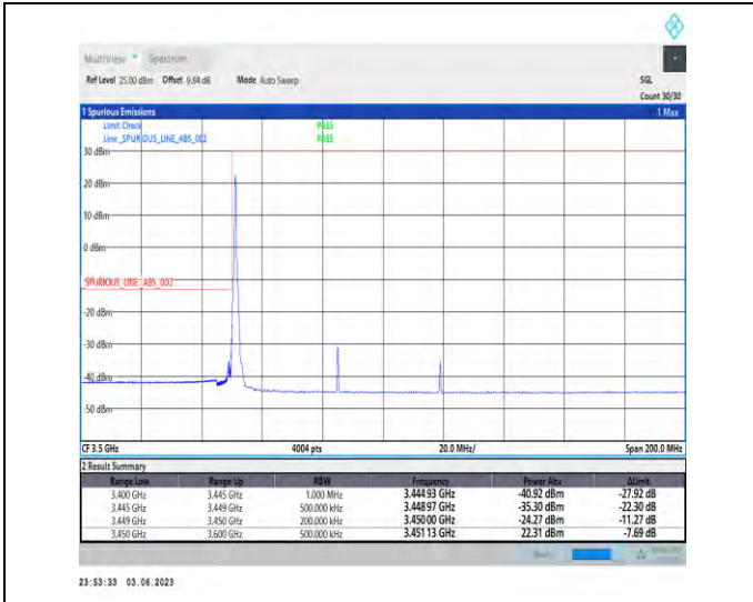
1-N78-3450-3550-PC2-30-70-L-1-DFT-PI2BPSK-Edge_1RB_Left-1@0-1--PASS-see graph
