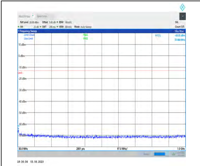
1-N78-3450-3550-PC2-30-100-M-1-N/A-DFT-PI2BP SK-Inner_1RB_Left-1@1-30-1000-33.88--65.03--13- PASS
