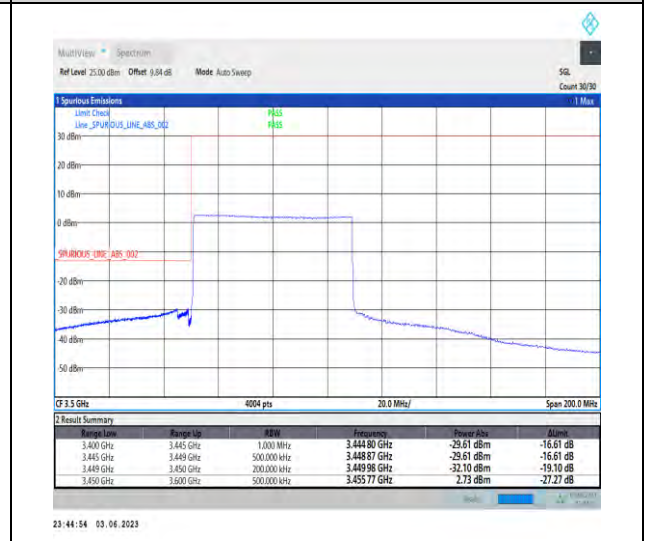
1-N78-3450-3550-PC2-30-60-L-6-CP-QPSK-Outer_Full-162@0-1--PASS-see graph
