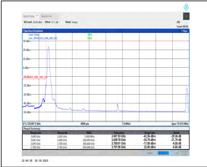
1-N77-3700-3980-PC3-30-60-L-1-DFT-PI2BPSK-Outer_Full-1@0-1--PASS-see graph
