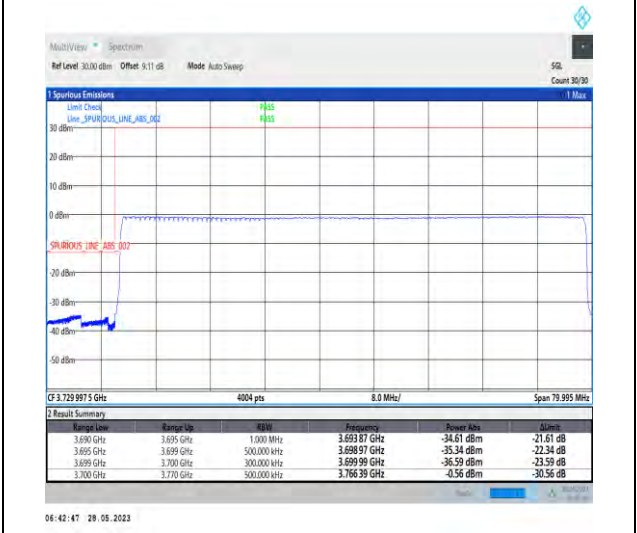
1-N77-3700-3980-PC2-30-70-L-6-CP-QPSK-Outer_Full-189@0-1--PASS-see graph
