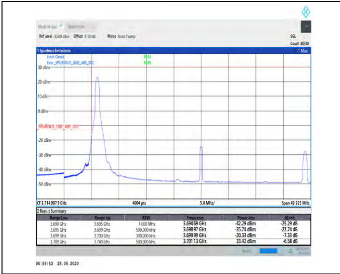
1-N77-3700-3980-PC3-30-40-L-1-DFT-PI2BPSK-Edge_1RB_Left-1@0-1--PASS-see graph
