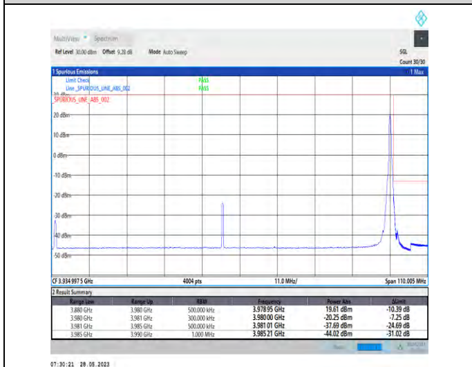
1-N77-3700-3980-PC2-30-100-H-5-CP-QPSK-Edge_1RB_Right-1@272-1--PASS-see graph
