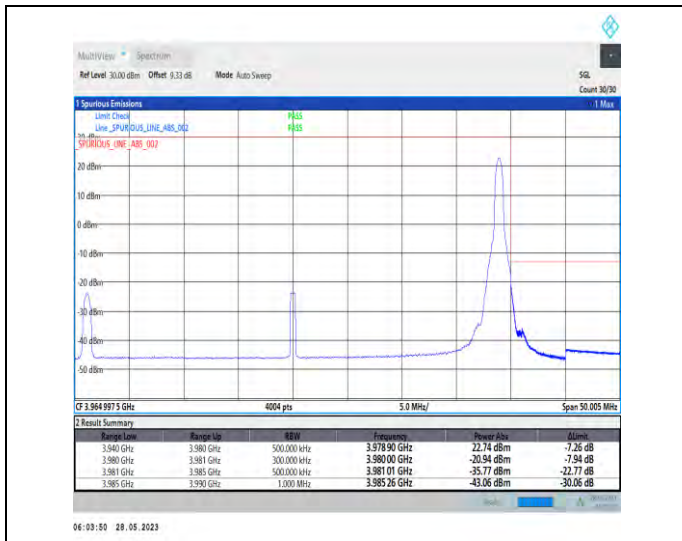
1-N77-3700-3980-PC3-30-40-H-2-DFT-PI2BPSK-Edge_1RB_Right-1@105-1--PASS-see graph
