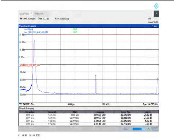
1-N77-3700-3980-PC2-30-90-L-1-DFT-PI2BPSK-Edge_1RB_Left-1@0-1--PASS-see graph
