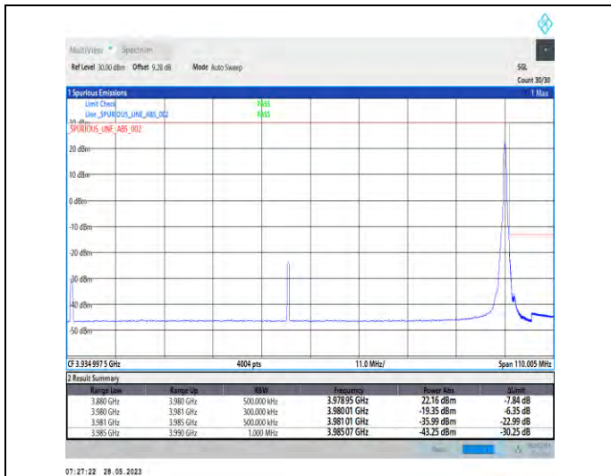
1-N77-3700-3980-PC2-30-100-H-2-DFT-PI2BPSK-Edge_e_1RB_Right-1@272-1--PASS-see graph
