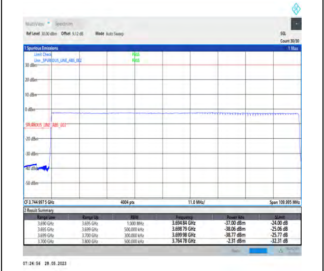
1-N77-3700-3980-PC2-30-100-L-6-CP-QPSK-Outer_Full-273@0-1--PASS-see graph
