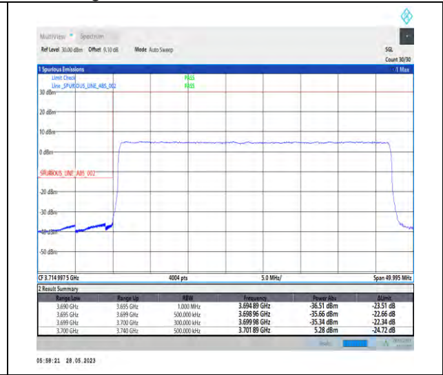
1-N77-3700-3980-PC3-30-40-L-3-DFT-PI2BPSK-Outer_Full-100@0-1--PASS-see graph
