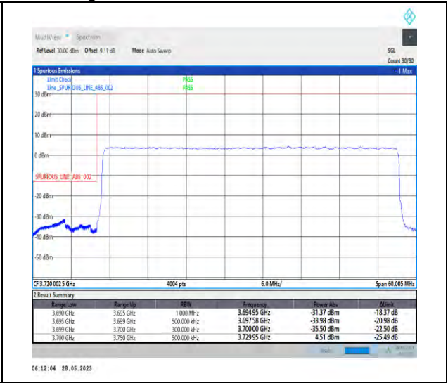
1-N77-3700-3980-PC3-30-50-L-3-DFT-PI2BPSK-Outer_Full-128@0-1--PASS-see graph
