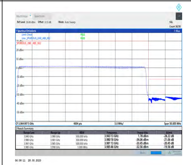
1-N77-3700-3980-PC3-30-40-H-6-CP-QPSK-Outer_Full-106@0-1--PASS-see graph
