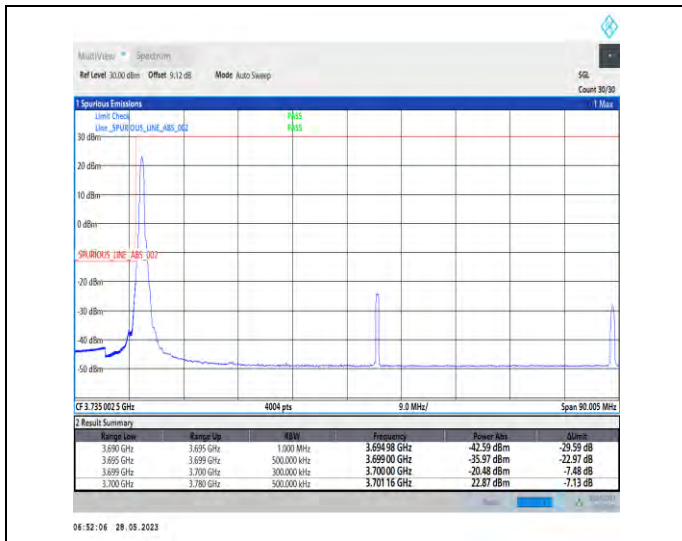
1-N77-3700-3980-PC2-30-80-L-1-DFT-PI2BPSK-Edge_1RB_Left-1@0-1--PASS-see graph
