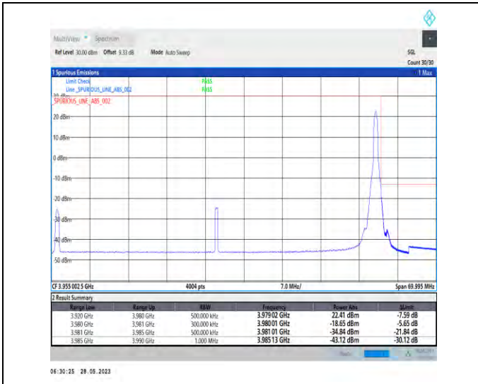
1-N77-3700-3980-PC2-30-60-H-2-DFT-PI2BPSK-Edge_1RB_Right-1@161-1--PASS-see graph
