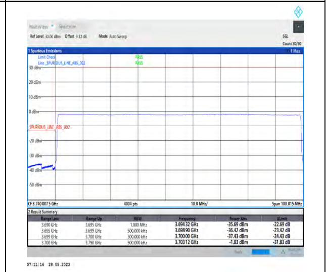
1-N77-3700-3980-PC2-30-90-L-6-CP-QPSK-Outer_Full-245@0-1--PASS-see graph
