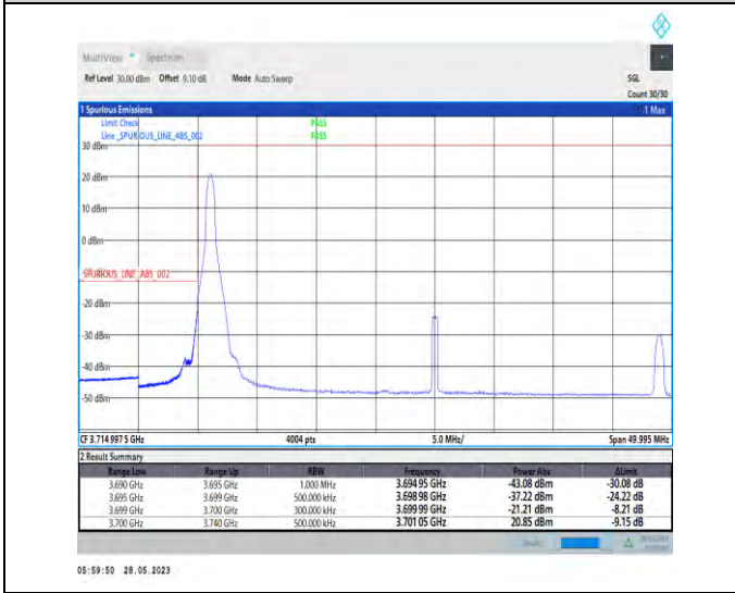
1-N77-3700-3980-PC3-30-40-L-4-CP-QPSK-Edge_1RB_Left-1@0-1--PASS-see graph
