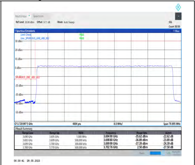
1-N77-3700-3980-PC2-30-70-L-3-DFT-PI2BPSK-Outer_Full-180@0-1--PASS-see graph
