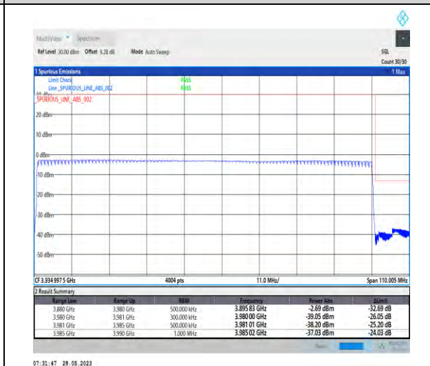
1-N77-3700-3980-PC2-30-100-H-6-CP-QPSK-Outer_Full-273@0-1--PASS-see graph
