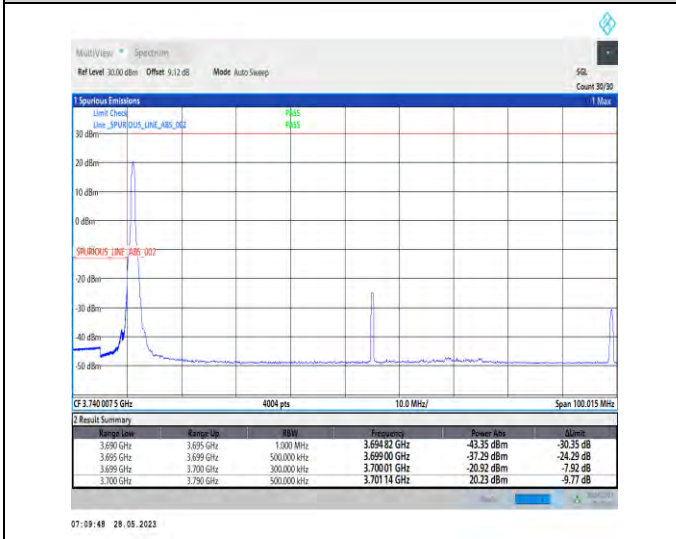
1-N77-3700-3980-PC2-30-90-L-4-CP-QPSK-Edge_1RB_Left-1@0-1--PASS-see graph
