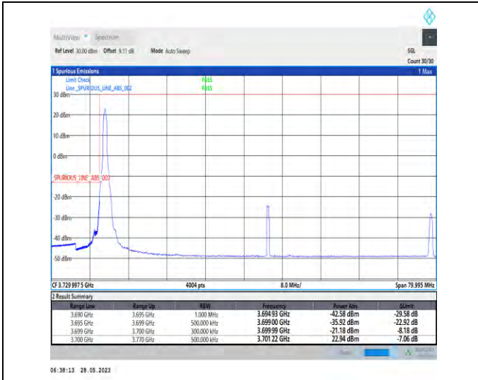
1-N77-3700-3980-PC2-30-70-L-1-DFT-PI2BPSK-Edge_1RB_Left-1@0-1--PASS-see graph
