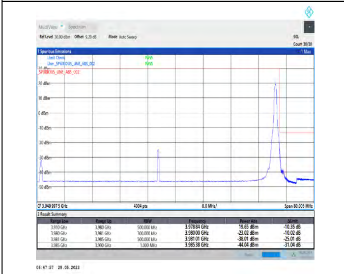
1-N77-3700-3980-PC2-30-70-H-5-CP-QPSK-Edge_1RB_Right-1@188-1--PASS-see graph
