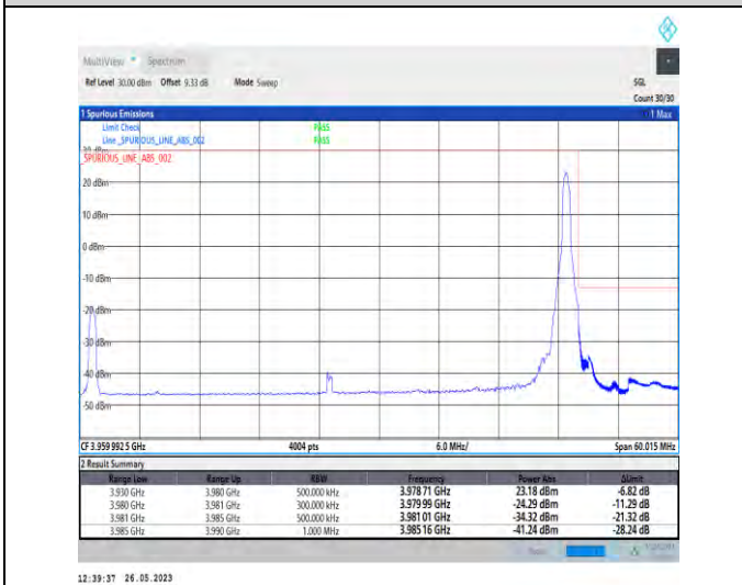
1-N77-3700-3980-PC3-30-50-H-5-CP-QPSK-Edge_1RB_Right-1@132-1--PASS-see graph
