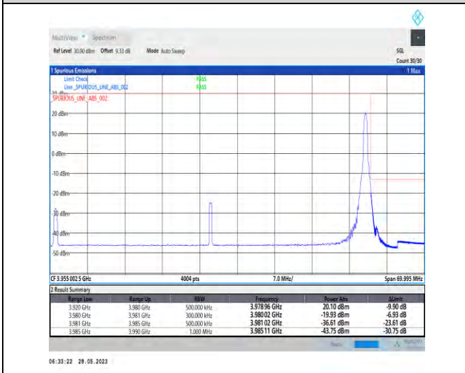
1-N77-3700-3980-PC2-30-60-H-5-CP-QPSK-Edge_1RB_Right-1@161-1--PASS-see graph
