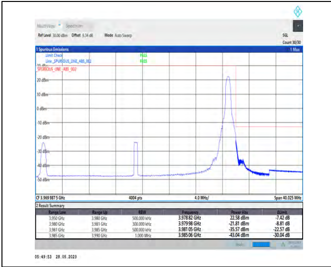
1-N77-3700-3980-PC3-30-30-H-2-DFT-PI2BPSK-Edge_1RB_Right-1@77-1--PASS-see graph
