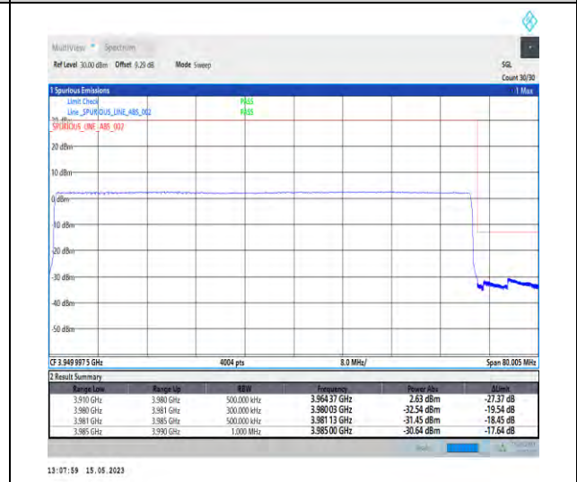
1-N77-3700-3980-PC2-30-70-H-6-CP-QPSK-Outer_Full-189@0-1--PASS-see graph
