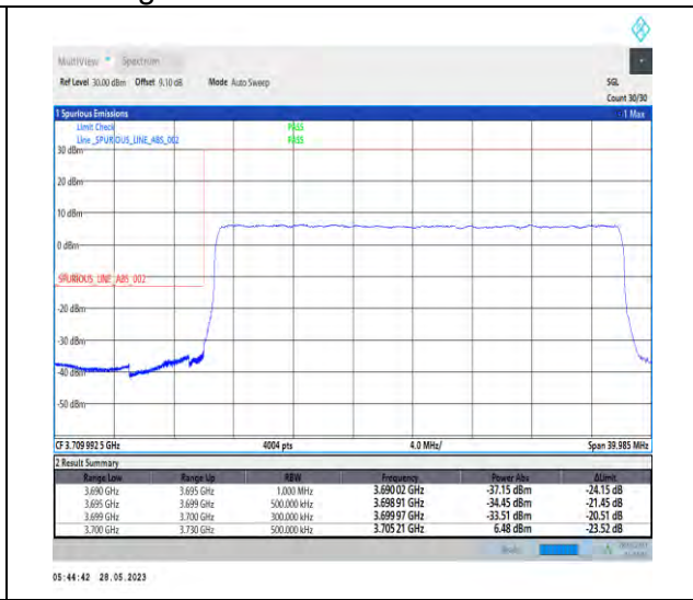
1-N77-3700-3980-PC3-30-30-L-3-DFT-PI2BPSK-Outer_Full-75@0-1--PASS-see graph
