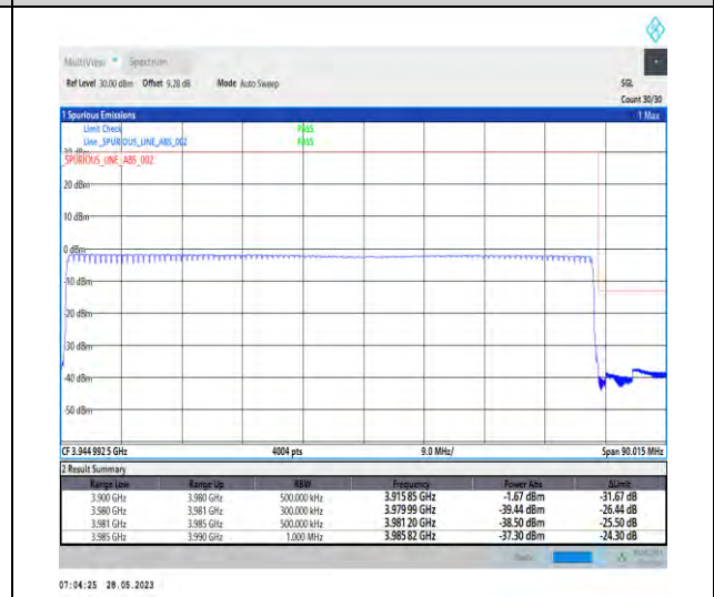
1-N77-3700-3980-PC2-30-80-H-6-CP-QPSK-Outer_Full-217@0-1--PASS-see graph
