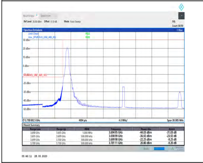
1-N77-3700-3980-PC3-30-30-L-4-CP-QPSK-Edge_1RB_Left-1@0-1--PASS-see graph
