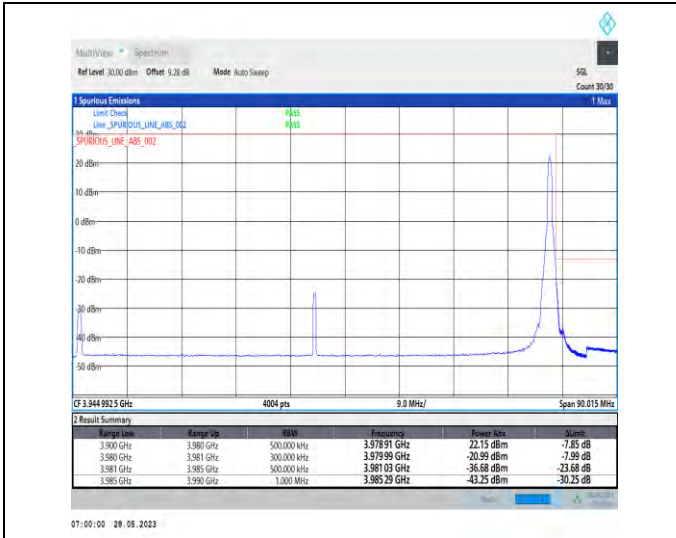
1-N77-3700-3980-PC2-30-80-H-2-DFT-PI2BPSK-Edge_1RB_Right-1@216-1--PASS-see graph
