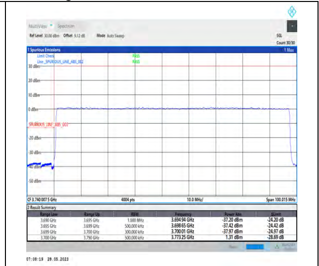
1-N77-3700-3980-PC2-30-90-L-3-DFT-PI2BPSK-Outer_Full-240@0-1--PASS-see graph
