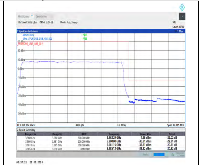
1-N77-3700-3980-PC3-30-20-H-3-DFT-PI2BPSK-Outer_Full-50@0-1--PASS-see graph
