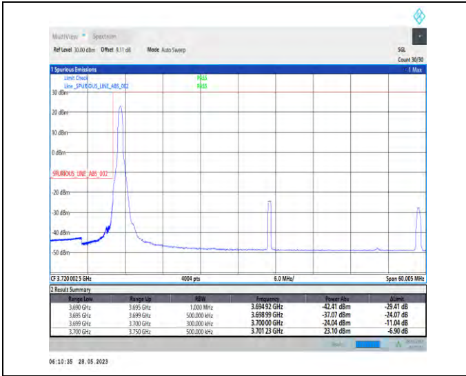
1-N77-3700-3980-PC3-30-50-L-1-DFT-PI2BPSK-Edge_1RB_Left-1@0-1--PASS-see graph
