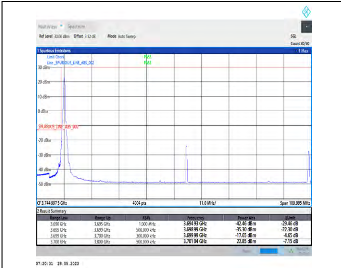
1-N77-3700-3980-PC2-30-100-L-1-DFT-PI2BPSK-Edge_e_1RB_Left-1@0-1--PASS-see graph
