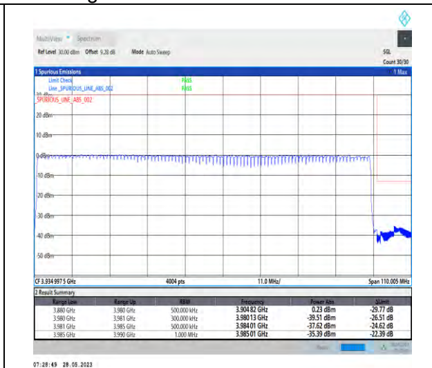
1-N77-3700-3980-PC2-30-100-H-3-DFT-PI2BPSK-Outer_Full-270@0-1--PASS-see graph
