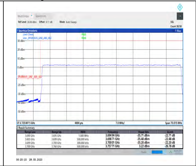
1-N77-3700-3980-PC3-30-60-L-3-DFT-PI2BPSK-Outer_Full-162@0-1--PASS-see graph
