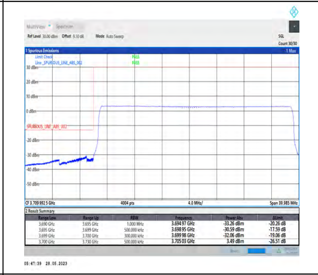
1-N77-3700-3980-PC3-30-30-L-6-CP-QPSK-Outer_Full-78@0-1--PASS-see graph
