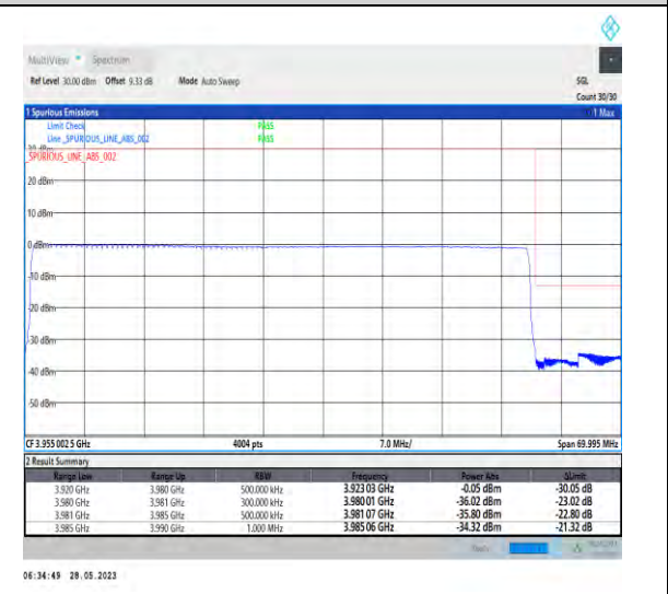
1-N77-3700-3980-PC2-30-60-H-6-CP-QPSK-Outer_Full-162@0-1--PASS-see graph
