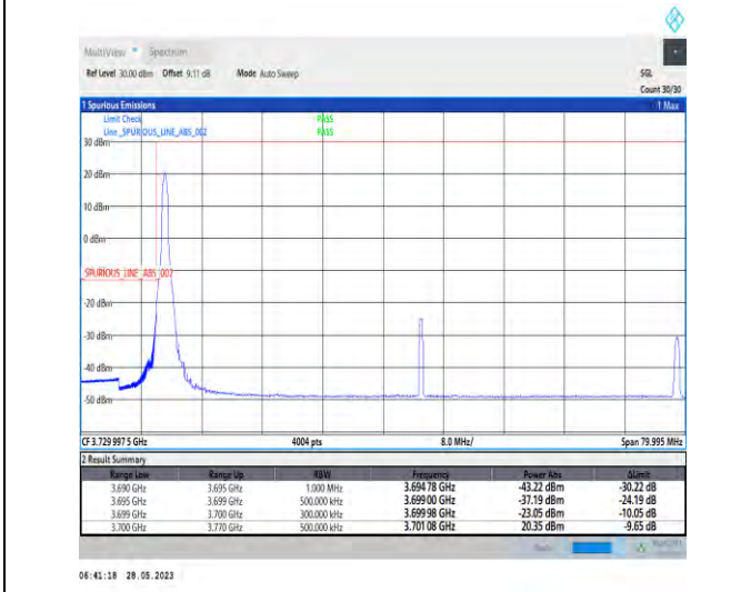
1-N77-3700-3980-PC2-30-70-L-4-CP-QPSK-Edge_1RB_Left-1@0-1--PASS-see graph
