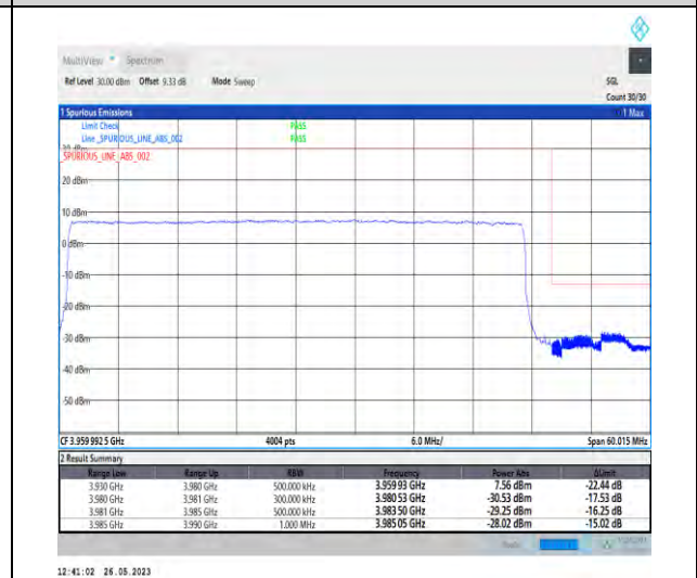
1-N77-3700-3980-PC3-30-50-H-6-CP-QPSK-Outer_Full-133@0-1--PASS-see graph
