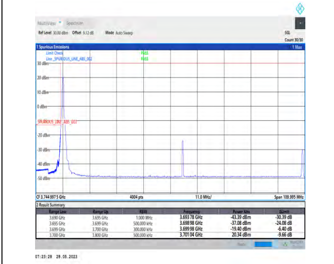
1-N77-3700-3980-PC2-30-100-L-4-CP-QPSK-Edge_1RB_Left-1@0-1--PASS-see graph
