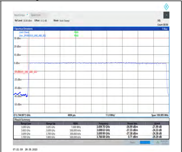
1-N77-3700-3980-PC2-30-100-L-3-DFT-PI2BPSK-Outer_Full-270@0-1--PASS-see graph
