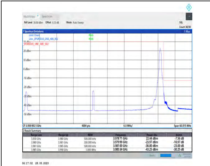
1-N77-3700-3980-PC3-30-50-H-2-DFT-PI2BPSK-Edge_1RB_Right-1@132-1--PASS-see graph
