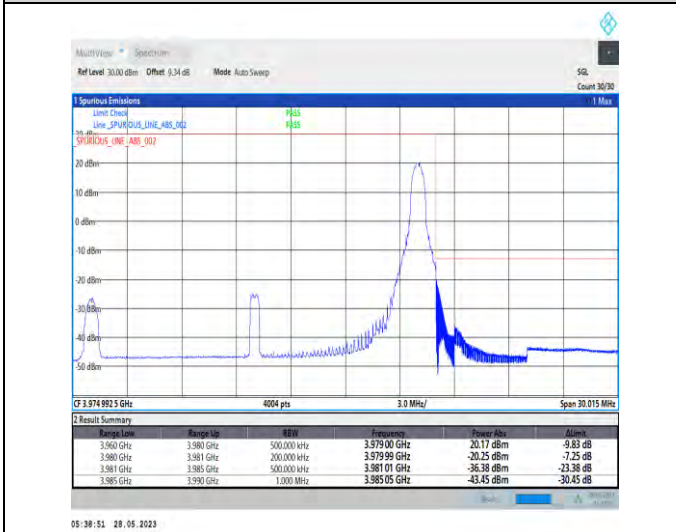
1-N77-3700-3980-PC3-30-20-H-5-CP-QPSK-Edge_1RB_Right-1@50-1--PASS-see graph
