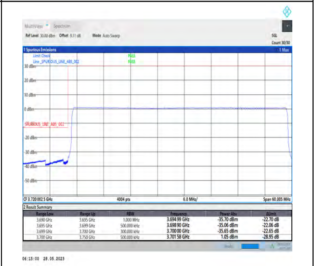
1-N77-3700-3980-PC3-30-50-L-6-CP-QPSK-Outer_Full-133@0-1--PASS-see graph
