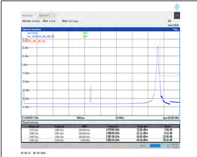
1-N77-3700-3980-PC2-30-70-H-2-DFT-PI2BPSK-Edge_1RB_Right-1@188-1--PASS-see graph
