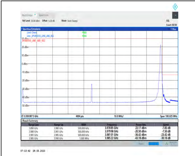
1-N77-3700-3980-PC2-30-90-H-2-DFT-PI2BPSK-Edge_1RB_Right-1@244-1--PASS-see graph
