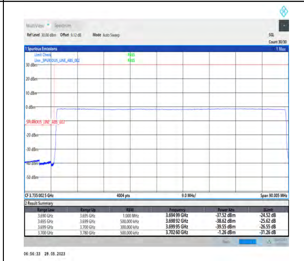
1-N77-3700-3980-PC2-30-80-L-6-CP-QPSK-Outer_Full-217@0-1--PASS-see graph
