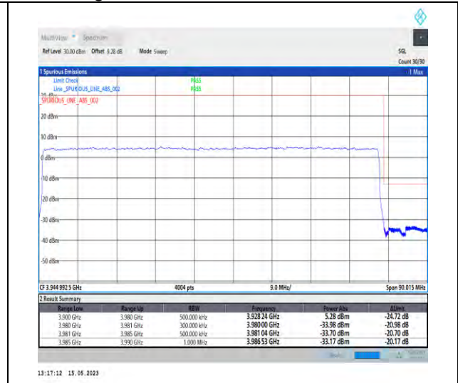
1-N77-3700-3980-PC2-30-80-H-3-DFT-PI2BPSK-Outer_Full-216@0-1--PASS-see graph
