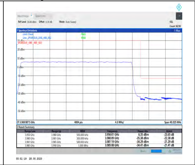
1-N77-3700-3980-PC3-30-30-H-3-DFT-PI2BPSK-Outer_Full-75@0-1--PASS-see graph
