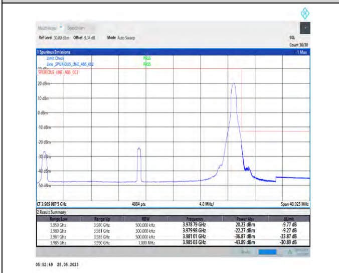
1-N77-3700-3980-PC3-30-30-H-5-CP-QPSK-Edge_1RB_Right-1@77-1--PASS-see graph
