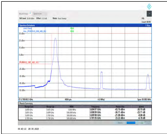
1-N77-3700-3980-PC3-30-30-L-1-DFT-PI2BPSK-Edge_1RB_Left-1@0-1--PASS-see graph
