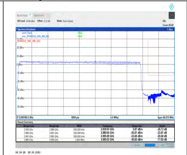
1-N77-3700-3980-PC3-30-50-H-3-DFT-PI2BPSK-Outer_Full-128@0-1--PASS-see graph
