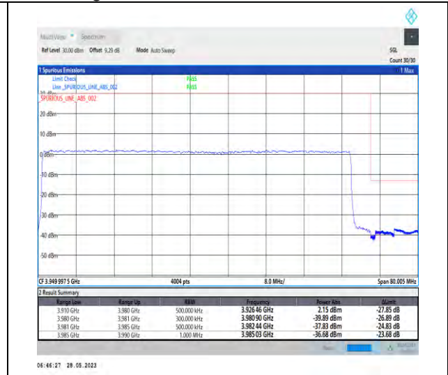
1-N77-3700-3980-PC2-30-70-H-3-DFT-PI2BPSK-Outer_Full-180@0-1--PASS-see graph
