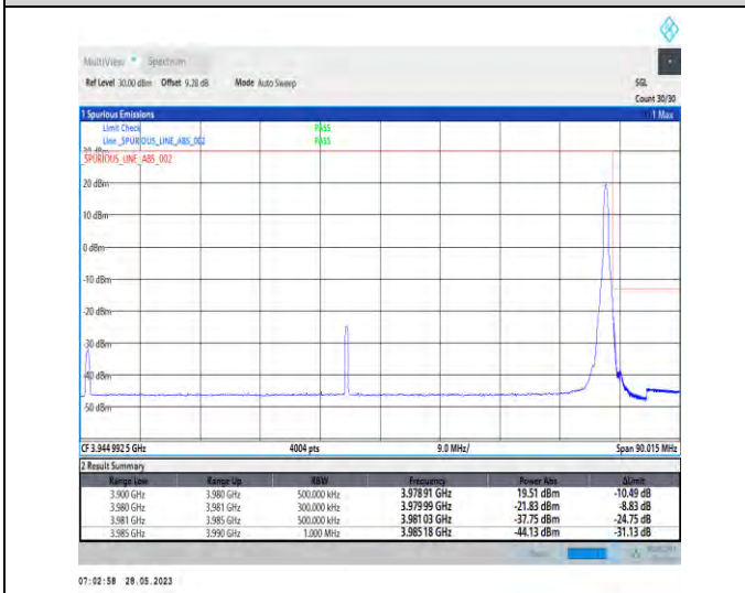
1-N77-3700-3980-PC2-30-80-H-5-CP-QPSK-Edge_1RB_Right-1@216-1--PASS-see graph
