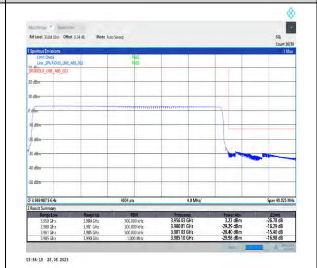
1-N77-3700-3980-PC3-30-30-H-6-CP-QPSK-Outer_Full-78@0-1--PASS-see graph
