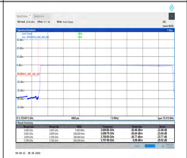
1-N77-3700-3980-PC3-30-60-L-6-CP-QPSK-Outer_Full-162@0-1--PASS-see graph
