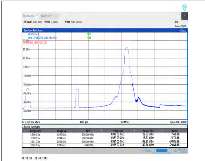
1-N77-3700-3980-PC3-30-20-H-2-DFT-PI2BPSK-Edge_1RB_Right-1@50-1--PASS-see graph
