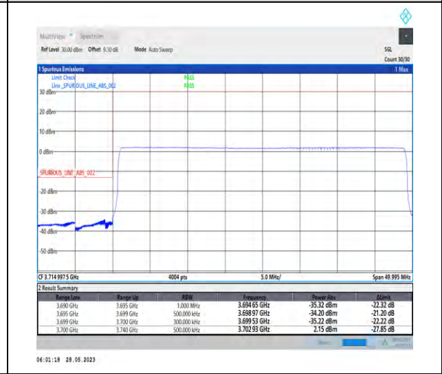
1-N77-3700-3980-PC3-30-40-L-6-CP-QPSK-Outer_Full-106@0-1--PASS-see graph
