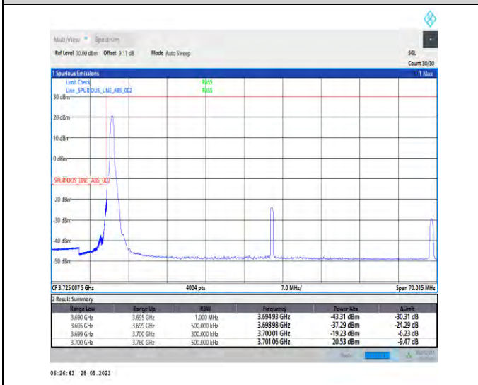
1-N77-3700-3980-PC3-30-60-L-5-CP-QPSK-Outer_Full-1@0-1--PASS-see graph
