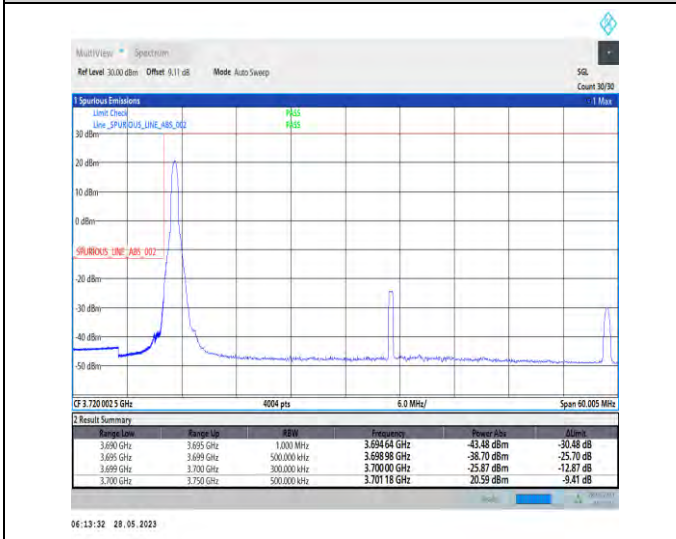
1-N77-3700-3980-PC3-30-50-L-4-CP-QPSK-Edge_1RB_Left-1@0-1--PASS-see graph
