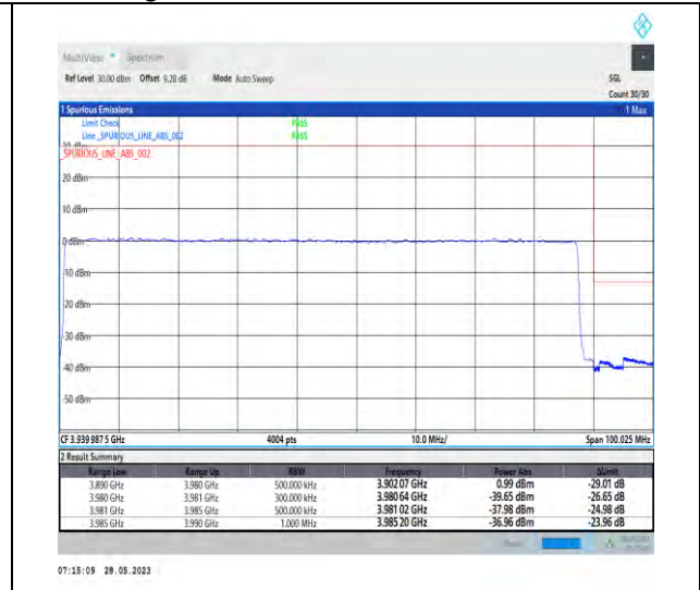
1-N77-3700-3980-PC2-30-90-H-3-DFT-PI2BPSK-Outer_Full-240@0-1--PASS-see graph
