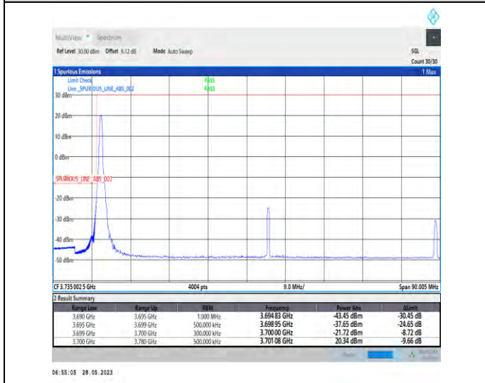
1-N77-3700-3980-PC2-30-80-L-4-CP-QPSK-Edge_1RB_Left-1@0-1--PASS-see graph
