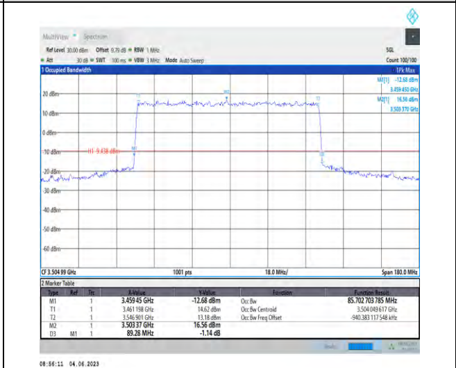
1-N78-3450-3550-PC2-30-90-H-1-DFT-QPSK-Outer _Full-240@0-85.703-89.280-≤90-PASS
