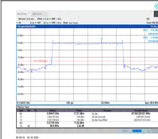
1-N78-3450-3550-PC2-30-90-M-9-CP-256QAM-Outer _Full-245@0-87.593-90.900-≤90-PASS
