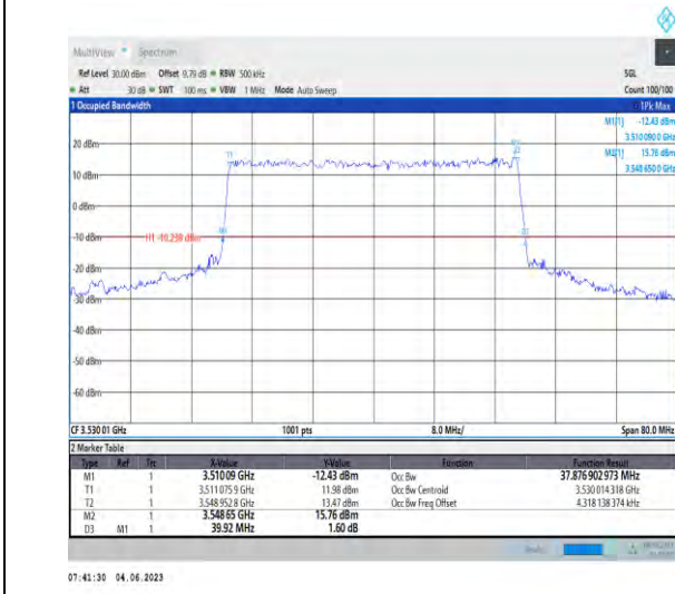
1-N78-3450-3550-PC2-30-40-H-7-CP-16QAM-Outer _Full-106@0-37.877-39.920-≤40-PASS
