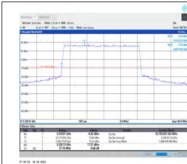
1-N78-3450-3550-PC2-30-40-H-1-DFT-QPSK-Outer_Full-100@0-35.705-37.760-≤40-PASS
