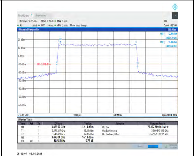
1-N78-3450-3550-PC2-30-80-H-4-DFT-64QAM-Outer_Full-216@0-77.173-80.480-≤80-PASS
