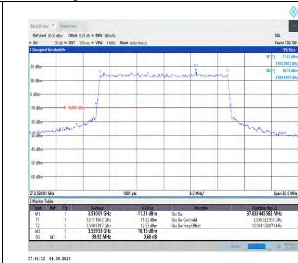
1-N78-3450-3550-PC2-30-40-H-6-CP-QPSK-Outer_ Full-106@0-37.833-39.920-≤40-PASS
