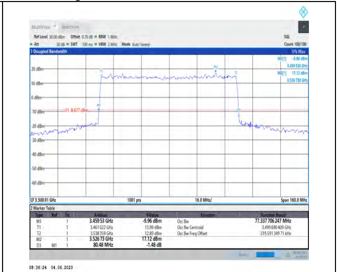
1-N78-3450-3550-PC2-30-80-M-3-DFT-16QAM-Out er_Full-216@0-77.338-80.480-≤80-PASS
