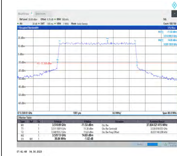
1-N78-3450-3550-PC2-30-40-H-8-CP-64QAM-Outer _Full-106@0-37.834-39.840-≤40-PASS
