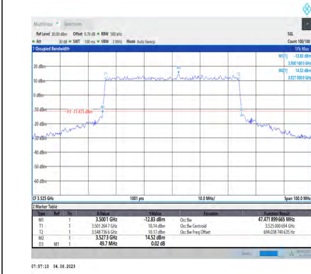
1-N78-3450-3550-PC2-30-50-H-8-CP-64QAM-Outer_Full-133@0-47.472-49.700-≤50-PASS
