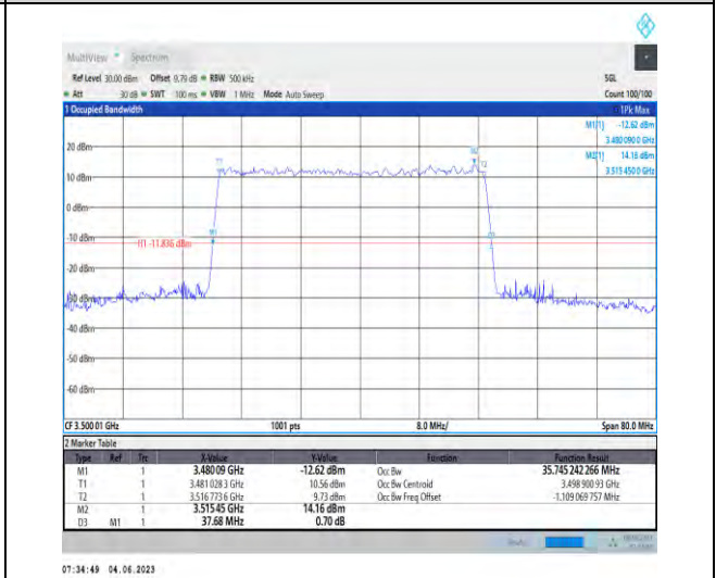
1-N78-3450-3550-PC2-30-40-M-5-DFT-256QAM-Out er_Full-100@0-35.745-37.680-≤40-PASS
