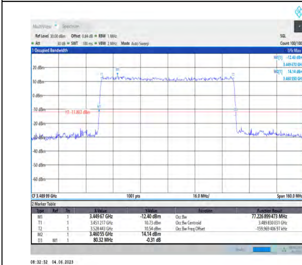
1-N78-3450-3550-PC2-30-80-L-5-DFT-256QAM-Outer_Full-216@0-77.227-80.320-≤80-PASS
