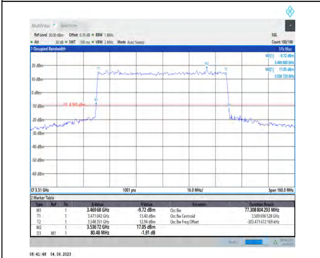
1-N78-3450-3550-PC2-30-80-H-3-DFT-16QAM-Outer_Full-216@0-77.309-80.480-≤80-PASS
