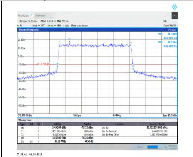
1-N78-3450-3550-PC2-30-40-L-4-DFT-64QAM-Outer_Full-100@0-35.753-37.680-≤40-PASS
