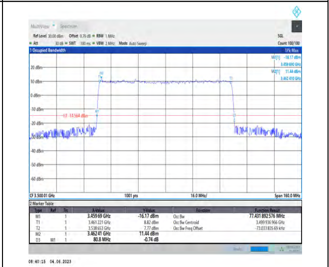
1-N78-3450-3550-PC2-30-80-M-9-CP-256QAM-Outer_Full-217@0-77.432-80.800-≤80-PASS
