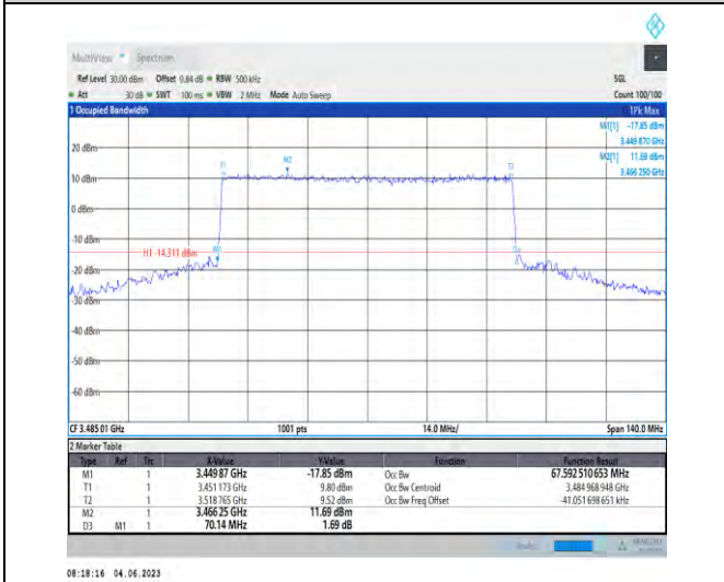
1-N78-3450-3550-PC2-30-70-L-8-CP-64QAM-Outer_Full-189@0-67.593-70.140-≤70-PASS
