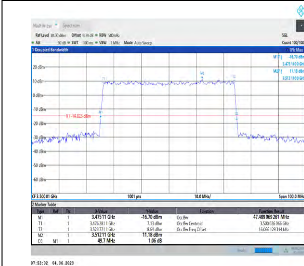
1-N78-3450-3550-PC2-30-50-M-9-CP-256QAM-Outer _Full-133@0-47.49-49.700-≤50-PASS
