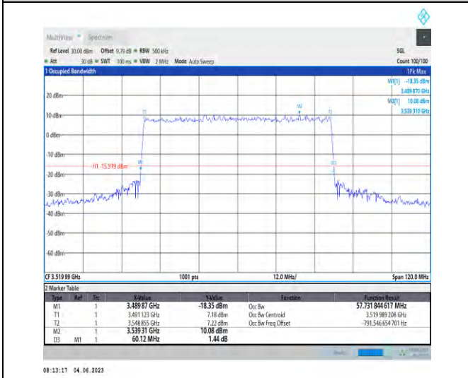
1-N78-3450-3550-PC2-30-60-H-9-CP-256QAM-Outer_Full-162@0-57.732-60.120-≤60-PASS
