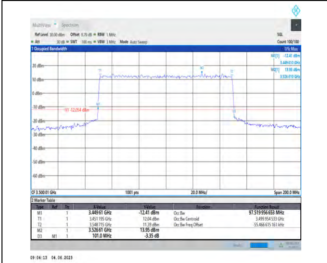
1-N78-3450-3550-PC2-30-100-L-7-CP-16QAM-Outer_Full-273@0-97.52-101.000-≤100-PASS
