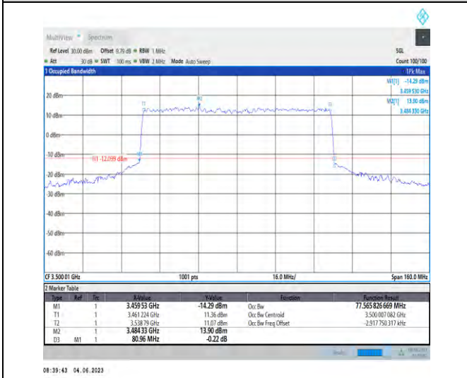
1-N78-3450-3550-PC2-30-80-M-8-CP-64QAM-Outer_Full-217@0-77.566-80.960-≤80-PASS
