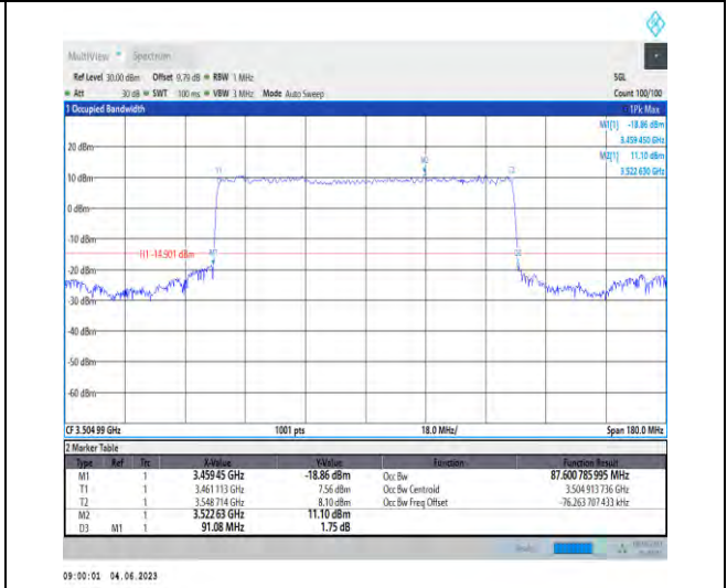
1-N78-3450-3550-PC2-30-90-H-9-CP-256QAM-Outer_Full-245@0-87.601-91.080-≤90-PASS
