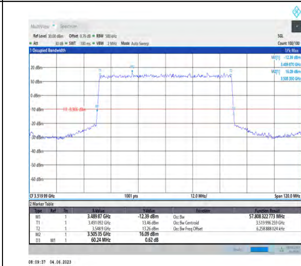
1-N78-3450-3550-PC2-30-60-H-2-DFT-PI2BPSK-Outer_Full-162@0-57.808-60.240-≤60-PASS
