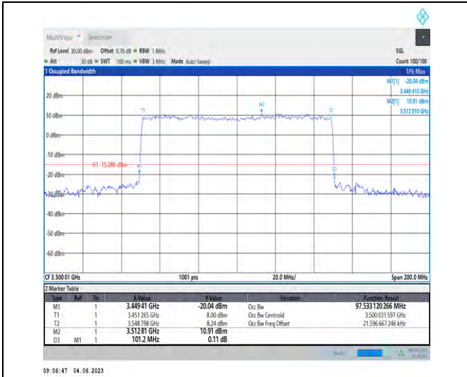
1-N78-3450-3550-PC2-30-100-L-9-CP-256QAM-Out er_Full-273@0-97.533-101.200-≤100-PASS
