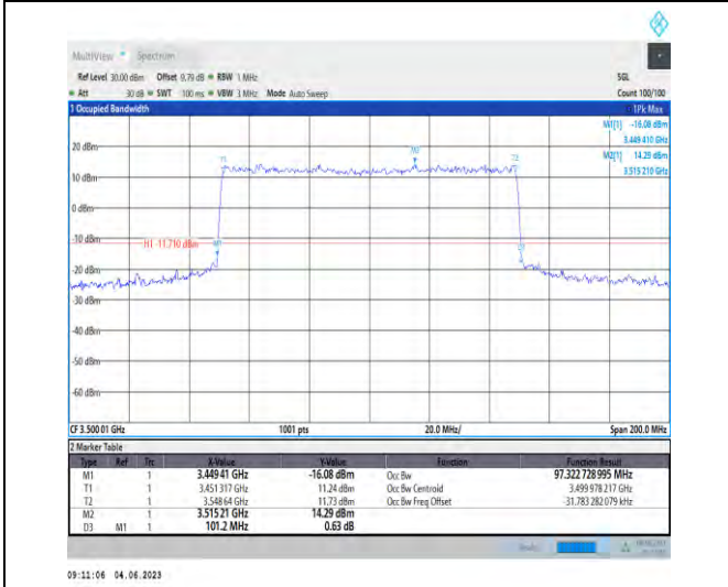
1-N78-3450-3550-PC2-30-100-M-6-CP-QPSK-Outer _Full-273@0-97.323-101.200-≤100-PASS
