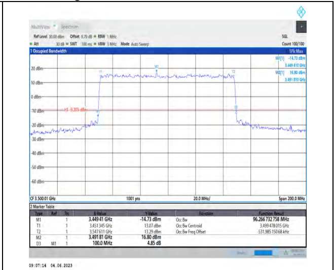
1-N78-3450-3550-PC2-30-100-M-1-DFT-QPSK-Out er_Full-270@0-96.267-100.000-≤100-PASS
