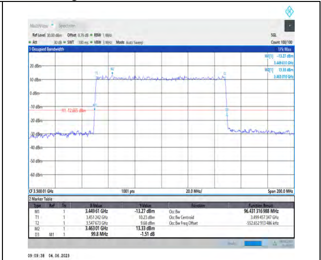
1-N78-3450-3550-PC2-30-100-M-5-DFT-256QAM-O uter_Full-270@0-96.431-99.800-≤100-PASS
