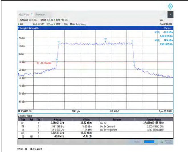
1-N78-3450-3550-PC2-30-40-M-8-CP-64QAM-Outer_Full-106@0-37.866-40.000-≤40-PASS
