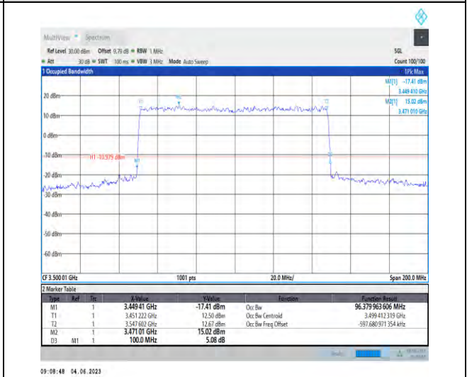
1-N78-3450-3550-PC2-30-100-M-3-DFT-16QAM-Ou ter_Full-270@0-96.38-100.000-≤100-PASS
