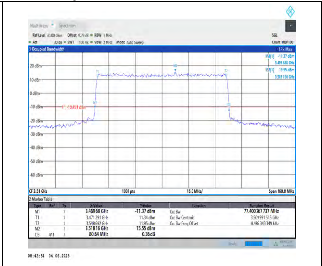
1-N78-3450-3550-PC2-30-80-H-6-CP-QPSK-Outer_Full-217@0-77.4-80.640-≤80-PASS
