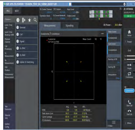
1-N78-3450-3550-PC2-30-100-M-2-DFT-QPSK-Out_Full-270@0-see graph-PASS
