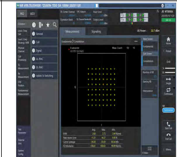
1-N78-3450-3550-PC2-30-100-M-8-CP-64QAM-Outer_Full-273@0-see graph-PASS
