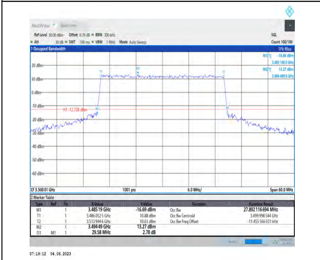
1-N78-3450-3550-PC2-30-30-M-7-CP-16QAM-Outer _Full-78@0-27.892-29.580-≤30-PASS
