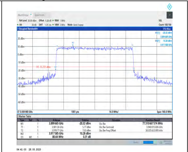
1-N77-3700-3980-PC3-30-80-H-8-CP-64QAM-Outer_Full-217@0-77.511-80.640-≤80-PASS
