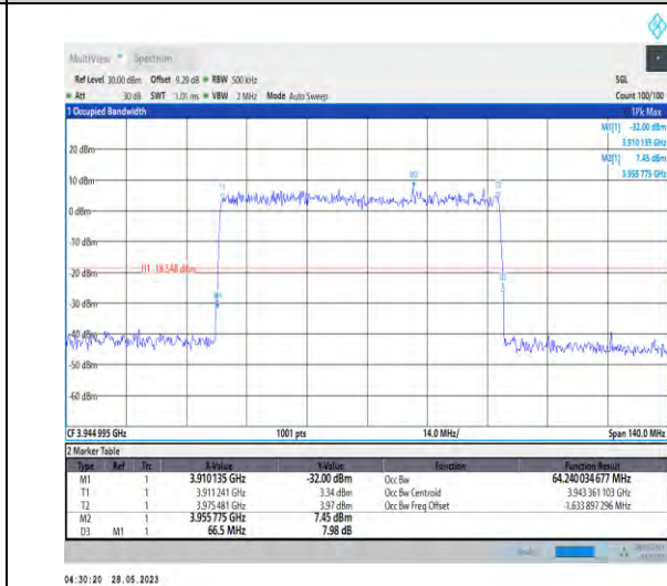
1-N77-3700-3980-PC3-30-70-H-5-DFT-256QAM-Outer _Full-180@0-64.24-66.500-≤70-PASS
