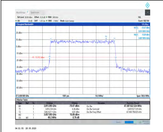
1-N77-3700-3980-PC3-30-50-M-7-CP-16QAM-Outer _Full-133@0-47.387-49.200-≤50-PASS
