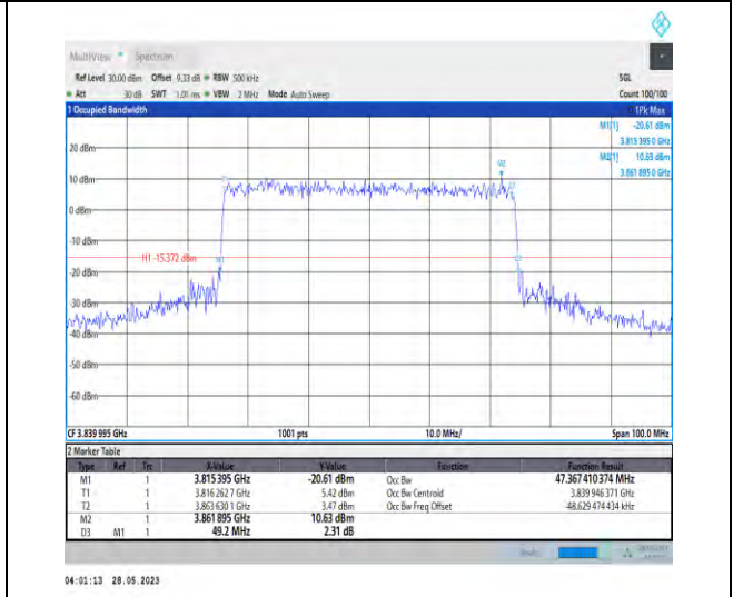
1-N77-3700-3980-PC3-30-50-M-8-CP-64QAM-Outer r_Full-133@0-47.367-49.200-≤50-PASS
