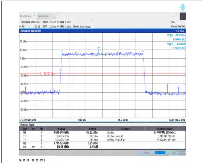
1-N77-3700-3980-PC3-30-80-L-9-CP-256QAM-Outer_Full-217@0-77.402-80.480-≤80-PASS
