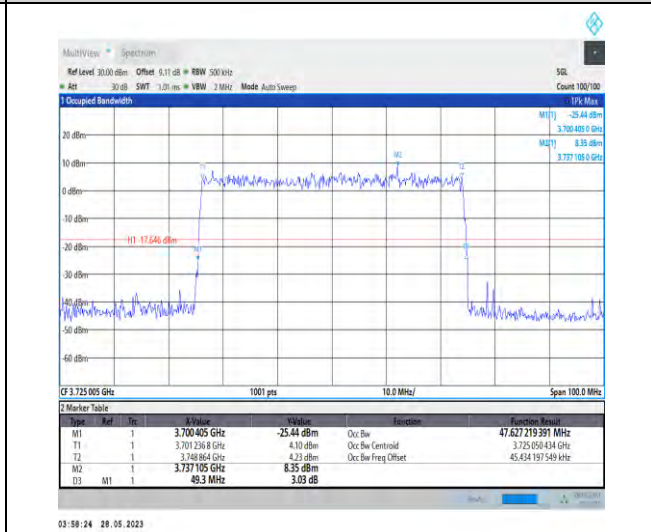
1-N77-3700-3980-PC3-30-50-L-9-CP-256QAM-Outer_Full-133@0-47.627-49.300-≤50-PASS
