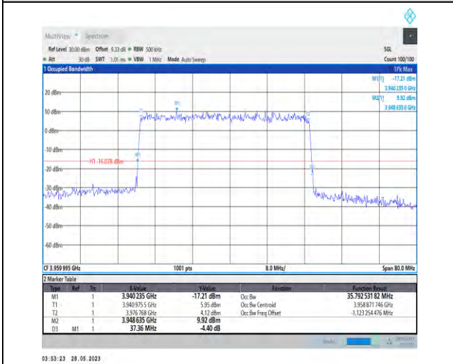
1-N77-3700-3980-PC3-30-40-H-5-DFT-256QAM-Outer_Full-100@0-35.793-37.360-≤40-PASS
