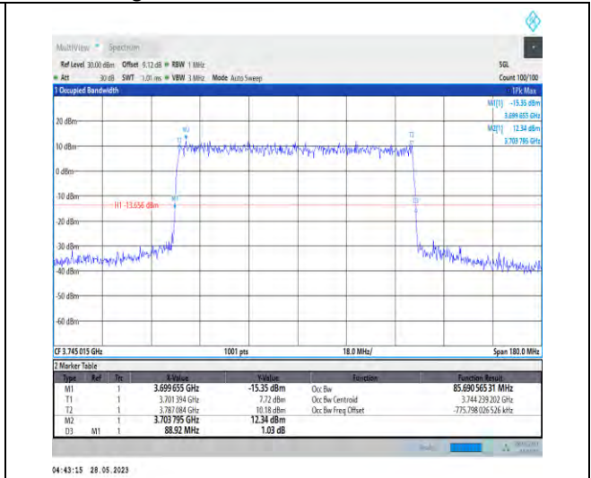
1-N77-3700-3980-PC3-30-90-L-3-DFT-16QAM-Out r_Full-240@0-85.691-88.920-≤90-PASS
