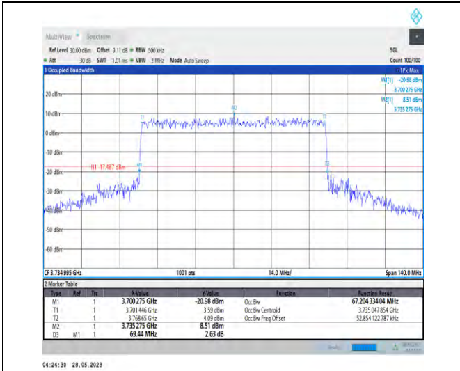
1-N77-3700-3980-PC3-30-70-L-8-CP-64QAM-Outer_Full-189@0-67.204-69.440-≤70-PASS
