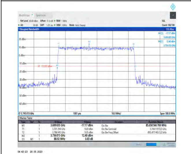
1-N77-3700-3980-PC3-30-90-L-4-DFT-64QAM-Out _Full-240@0-85.651-88.920-≤90-PASS
