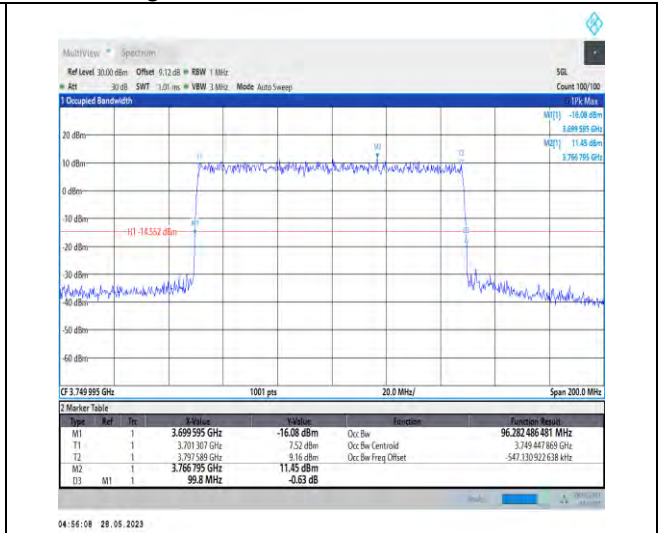
1-N77-3700-3980-PC3-30-100-L-4-DFT-64QAM-Out er_Full-270@0-96.282-99.800-≤100-PASS
