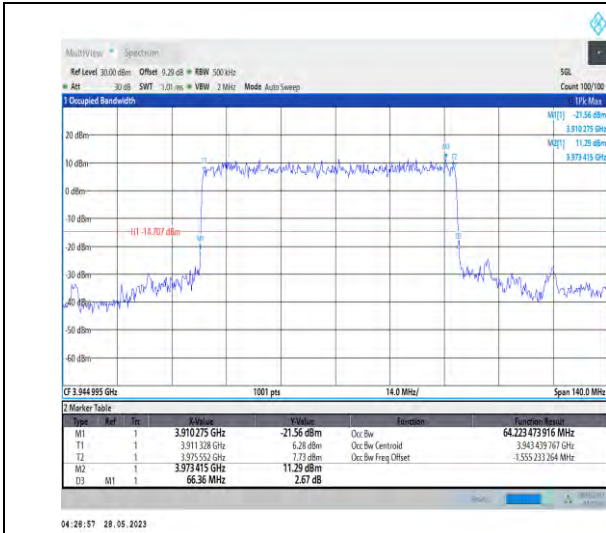
1-N77-3700-3980-PC3-30-70-H-2-DFT-PI2BPSK-Out er_Full-180@0-64.223-66.360-≤70-PASS
