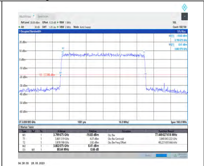
1-N77-3700-3980-PC3-30-80-M-9-CP-256QAM-Outer_Full-217@0-77.449-80.640-≤80-PASS
