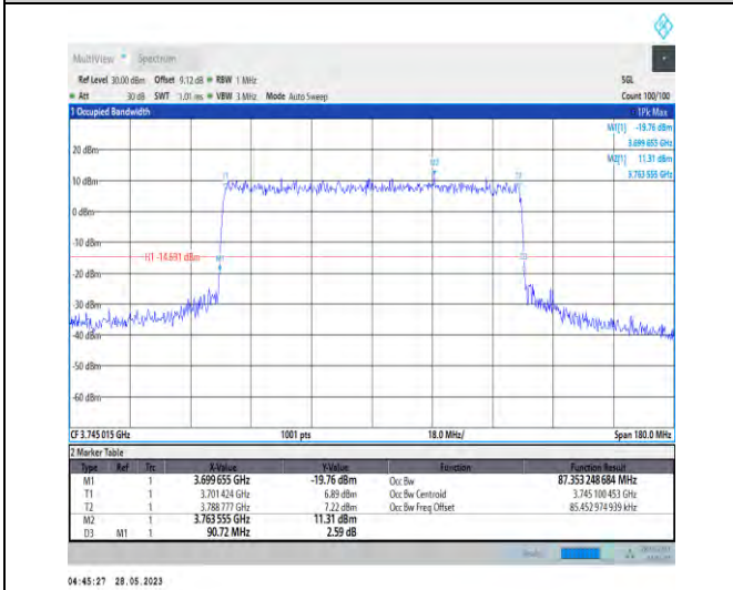
1-N77-3700-3980-PC3-30-90-L-8-CP-64QAM-Outer_Full-245@0-87.353-90.720-≤90-PASS
