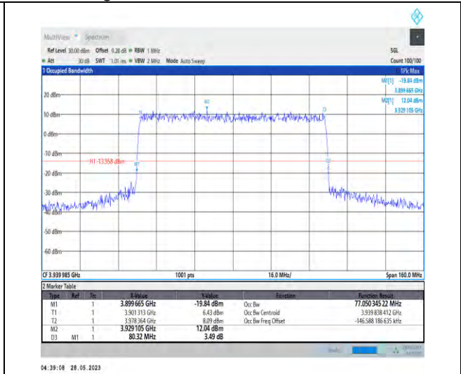
1-N77-3700-3980-PC3-30-80-H-4-DFT-64QAM-Outer_Full-216@0-77.05-80.320-≤80-PASS
