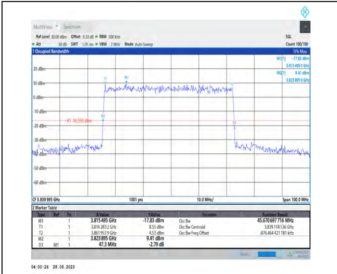
1-N77-3700-3980-PC3-30-50-M-5-DFT-256QAM-Out er_Full-128@0-45.671-47.300-≤50-PASS
