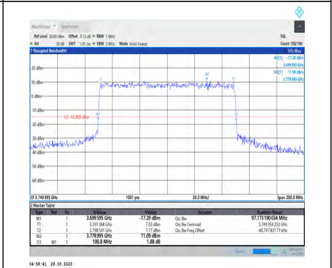
1-N77-3700-3980-PC3-30-100-L-6-CP-QPSK-Outer _Full-273@0-97.173-100.800-≤100-PASS
