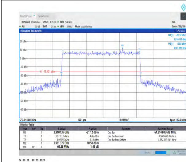
1-N77-3700-3980-PC3-30-70-H-4-DFT-64QAM-Outer _Full-180@0-64.215-66.360-≤70-PASS
