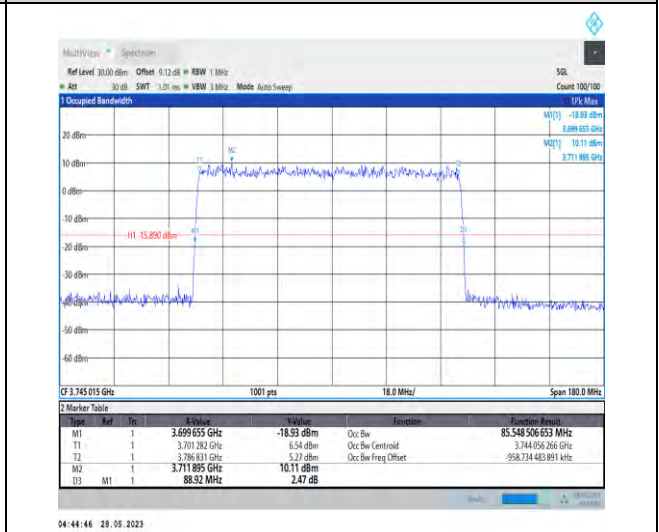
1-N77-3700-3980-PC3-30-90-L-5-DFT-256QAM-Out er_Full-240@0-85.549-88.920-≤90-PASS
