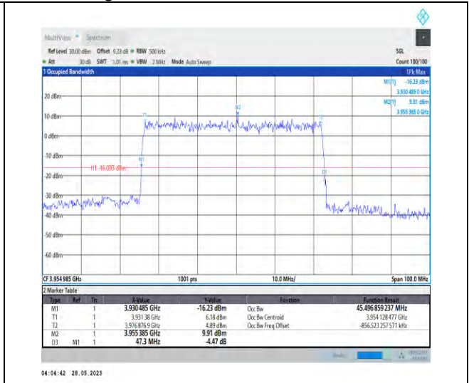
1-N77-3700-3980-PC3-30-50-H-5-DFT-256QAM-Outer_Full-128@0-45.497-47.300-≤50-PASS
