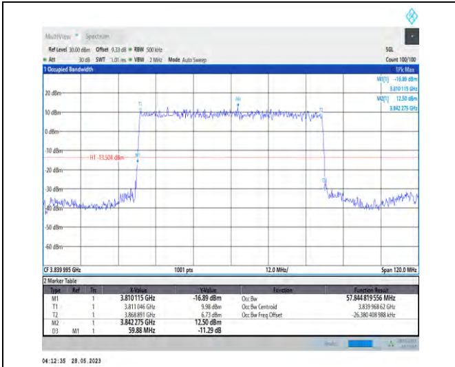
1-N77-3700-3980-PC3-30-60-M-2-DFT-PI2BPSK-Out er_Full-162@0-57.845-59.880-≤60-PASS
