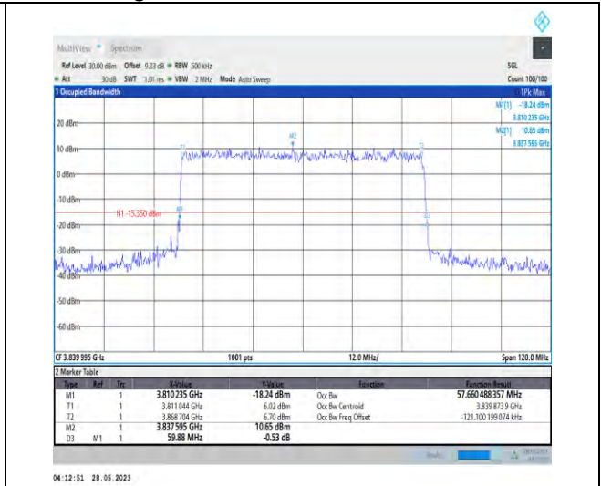
1-N77-3700-3980-PC3-30-60-M-3-DFT-16QAM-Out er_Full-162@0-57.66-59.880-≤60-PASS
