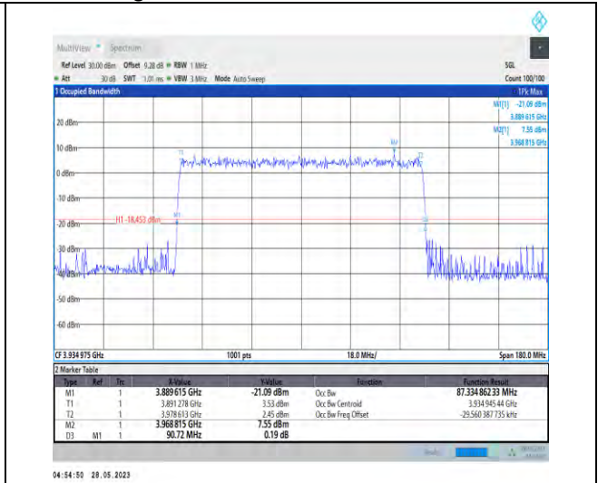
1-N77-3700-3980-PC3-30-90-H-9-CP-256QAM-Outer_Full-245@0-87.335-90.720-≤90-PASS
