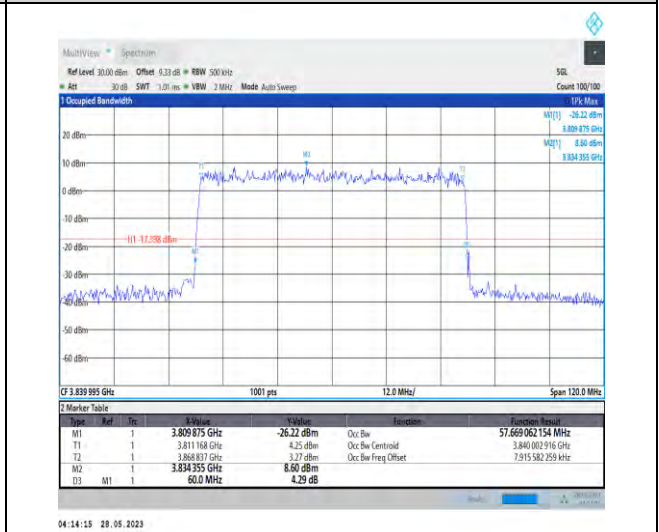
1-N77-3700-3980-PC3-30-60-M-5-DFT-256QAM-Out er_Full-162@0-57.669-60.000-≤60-PASS
