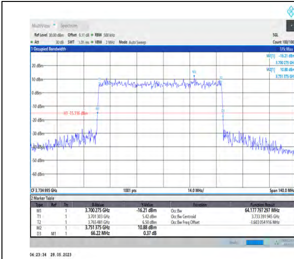
1-N77-3700-3980-PC3-30-70-L-4-DFT-64QAM-Outer_Full-180@0-64.178-66.220-≤70-PASS
