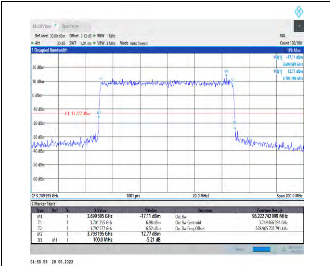
1-N77-3700-3980-PC3-30-100-L-3-DFT-16QAM-Out er_Full-270@0-96.223-100.000-≤100-PASS
