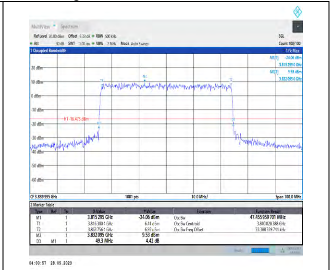
1-N77-3700-3980-PC3-30-50-M-6-CP-QPSK-Outer Full-133@0-47.456-49.300-≤50-PASS
