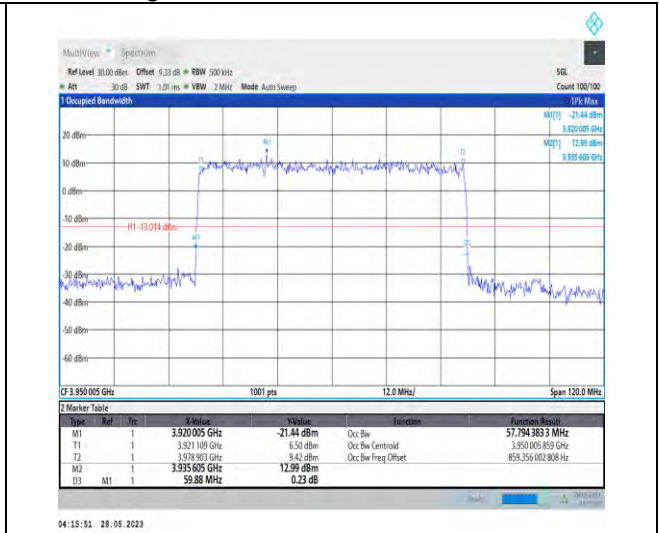
1-N77-3700-3980-PC3-30-60-H-2-DFT-PI2BPSK-Outer_Full-162@0-57.794-59.880-≤60-PASS
