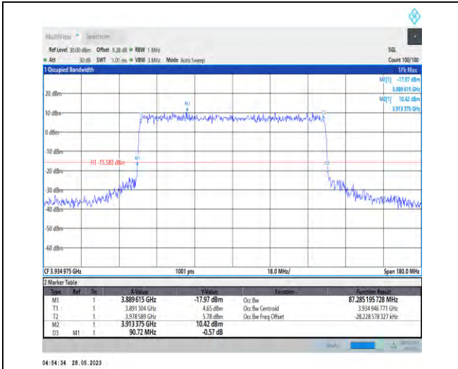
1-N77-3700-3980-PC3-30-90-H-8-CP-64QAM-Outer_Full-245@0-87.285-90.720-≤90-PASS
