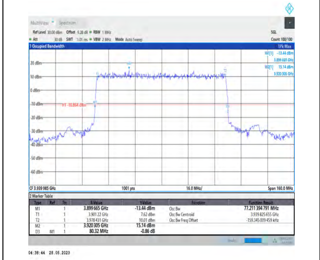
1-N77-3700-3980-PC3-30-80-H-2-DFT-PI2BPSK-Outer_Full-216@0-77.211-80.320-≤80-PASS
