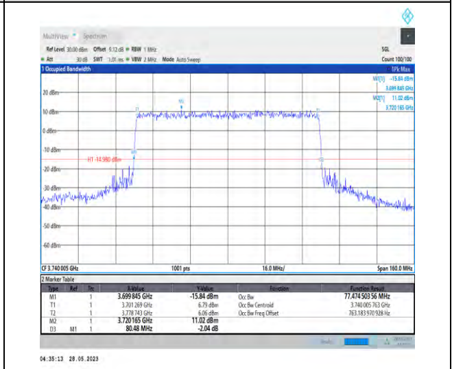
1-N77-3700-3980-PC3-30-80-L-8-CP-64QAM-Outer_Full-217@0-77.475-80.480-≤80-PASS
