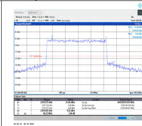
1-N77-3700-3980-PC3-30-70-H-3-DFT-16QAM-Out er_Full-180@0-64.019-66.220-≤70-PASS
