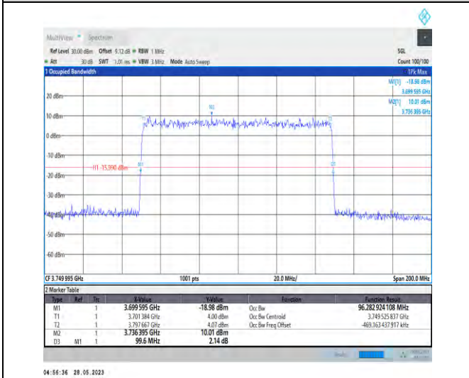
1-N77-3700-3980-PC3-30-100-L-5-DFT-256QAM-Out er_Full-270@0-96.283-99.600-≤100-PASS
