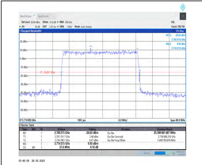
1-N77-3700-3980-PC3-30-40-L-5-DFT-256QAM-Out er_Full-100@0-35.589-37.600-≤40-PASS
