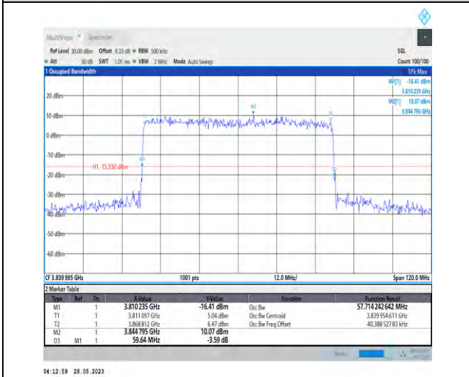
1-N77-3700-3980-PC3-30-60-M-4-DFT-64QAM-Out er_Full-162@0-57.714-59.640-≤60-PASS
