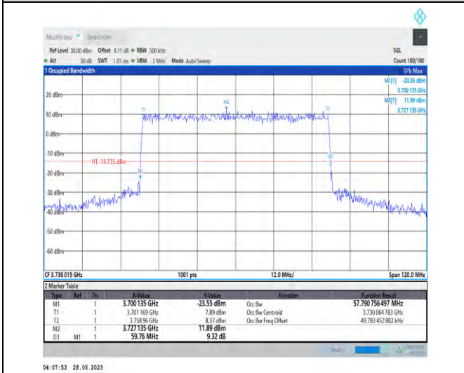
1-N77-3700-3980-PC3-30-60-L-1-DFT-QPSK-Outer_Full-162@0-57.791-59.760-≤60-PASS
