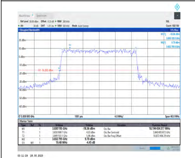
1-N77-3700-3980-PC3-30-20-M-6-CP-QPSK-Outer_Full-51@0-18.194-19.480-≤20-PASS
