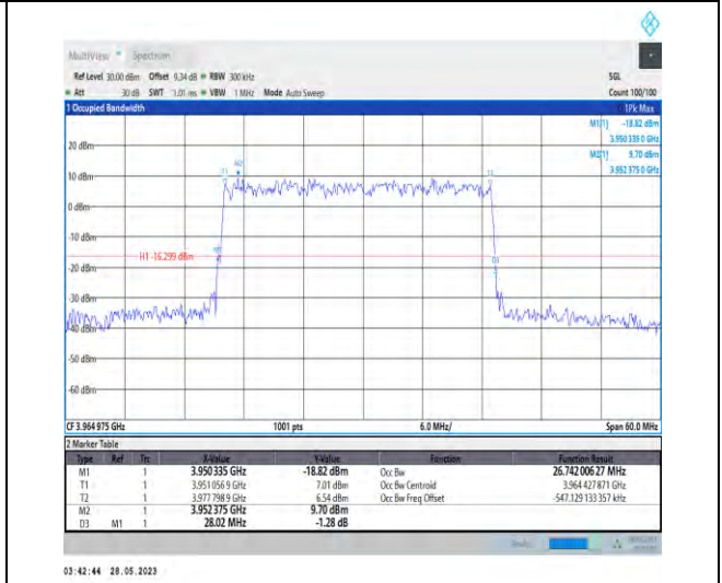
1-N77-3700-3980-PC3-30-30-H-5-DFT-256QAM-Outer _Full-75@0-26.742-28.020-≤30-PASS
