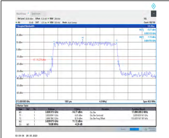
1-N77-3700-3980-PC3-30-20-M-4-DFT-64QAM-Outer_Full-50@0-17.89-18.880-≤20-PASS
