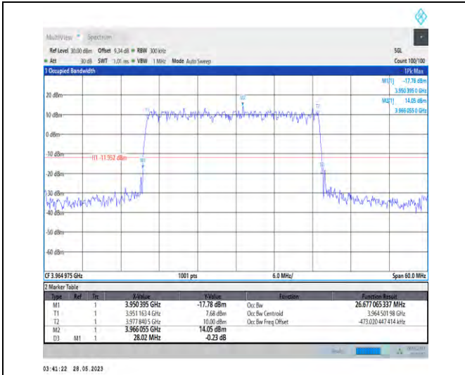
1-N77-3700-3980-PC3-30-30-H-2-DFT-PI2BPSK-Out er_Full-75@0-26.677-28.020-≤30-PASS
