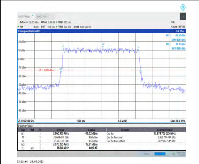
1-N77-3700-3980-PC3-30-20-H-2-DFT-PI2BPSK-Outer_Full-50@0-17.875-18.880-≤20-PASS
