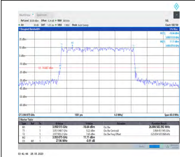
1-N77-3700-3980-PC3-30-30-H-4-DFT-64QAM-Outer _Full-75@0-26.807-27.960-≤30-PASS
