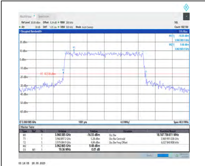
1-N77-3700-3980-PC3-30-20-H-8-CP-64QAM-Outer_Full-51@0-18.188-19.360-≤20-PASS
