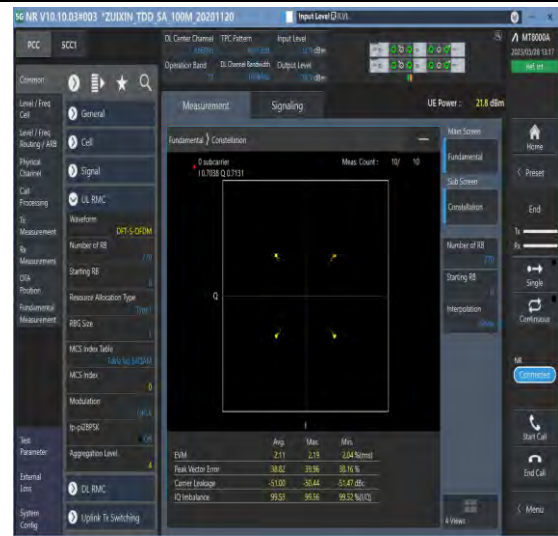
1-N77-3700-3980-PC3-30-100-M-2-DFT-QPSK-Out_er_Full-270@0-see graph-PASS
