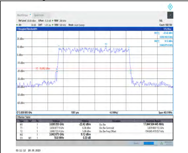
1-N77-3700-3980-PC3-30-20-M-5-DFT-256QAM-Outer_Full-50@0-17.845-18.800-≤20-PASS
