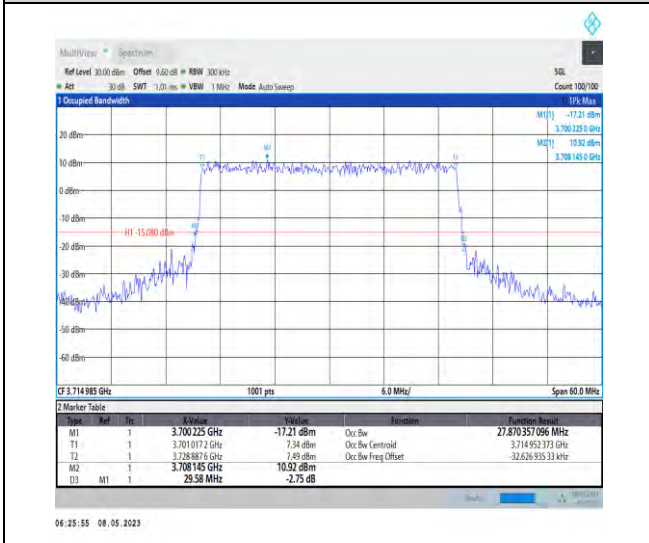
1-N77-3700-3980-PC2-30-30-L-4-DFT-256QAM-Outer_Full-75@0-27.87-29.580-≤30-PASS
