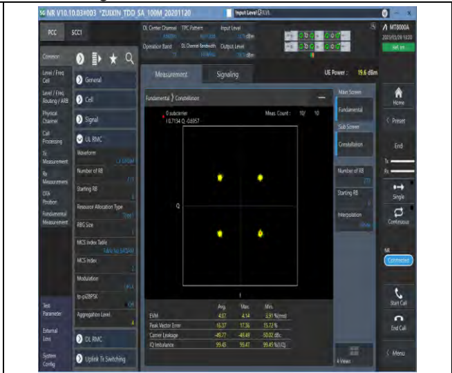
1-N77-3700-3980-PC3-30-100-M-6-CP-QPSK-Outer_Full-273@0-see graph-PASS
