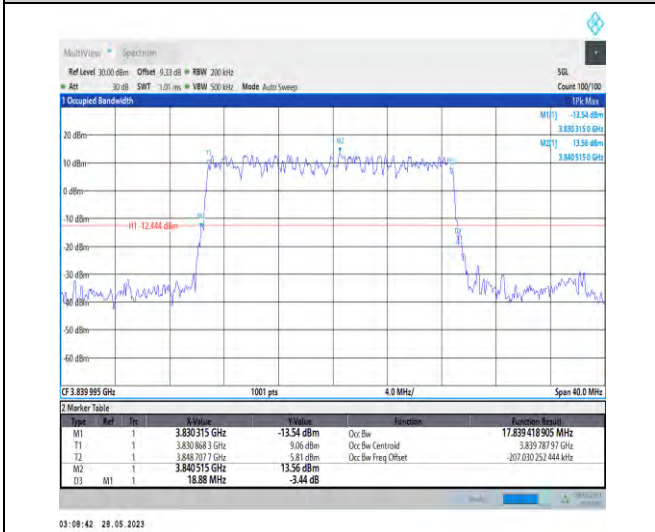
1-N77-3700-3980-PC3-30-20-M-2-DFT-PI2BPSK-Outer_Full-50@0-17.839-18.880-≤20-PASS
