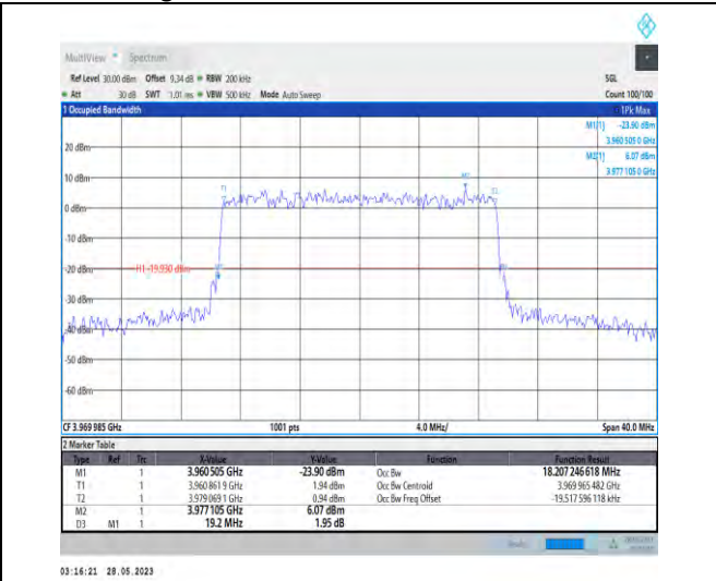
1-N77-3700-3980-PC3-30-20-H-9-CP-256QAM-Outer_Full-51@0-18.207-19.200-≤20-PASS
