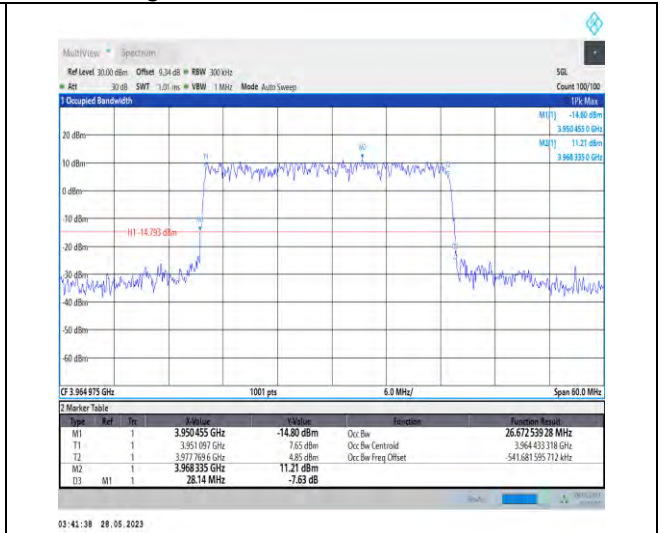
1-N77-3700-3980-PC3-30-30-H-3-DFT-16QAM-Out er_Full-75@0-26.673-28.140-≤30-PASS
