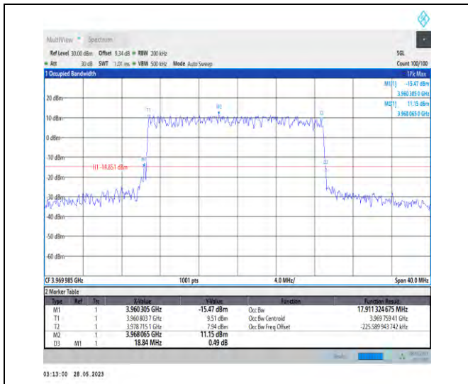
1-N77-3700-3980-PC3-30-20-H-3-DFT-16QAM-Outer_Full-50@0-17.911-18.840-≤20-PASS
