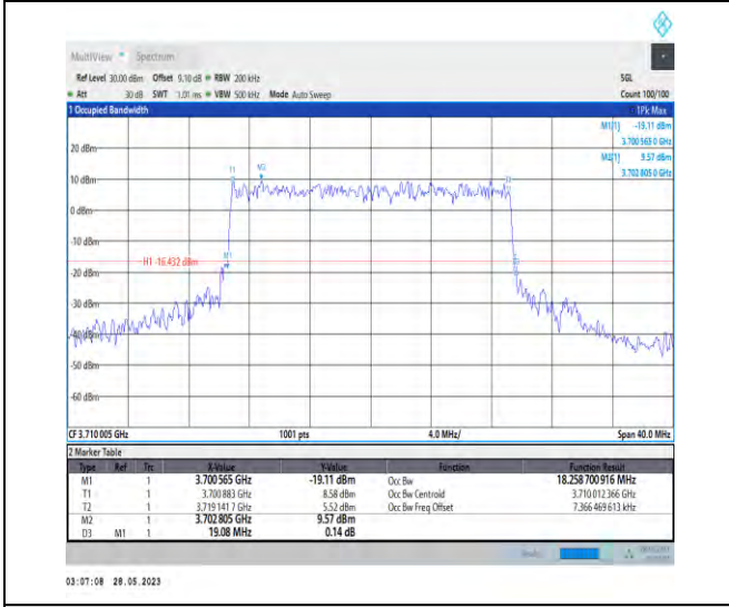
1-N77-3700-3980-PC3-30-20-L-7-CP-16QAM-Outer _Full-51@0-18.259-19.080-≤20-PASS
