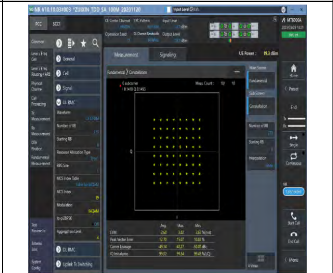
1-N77-3700-3980-PC3-30-100-M-8-CP-64QAM-Outer_Full-273@0-see graph-PASS
