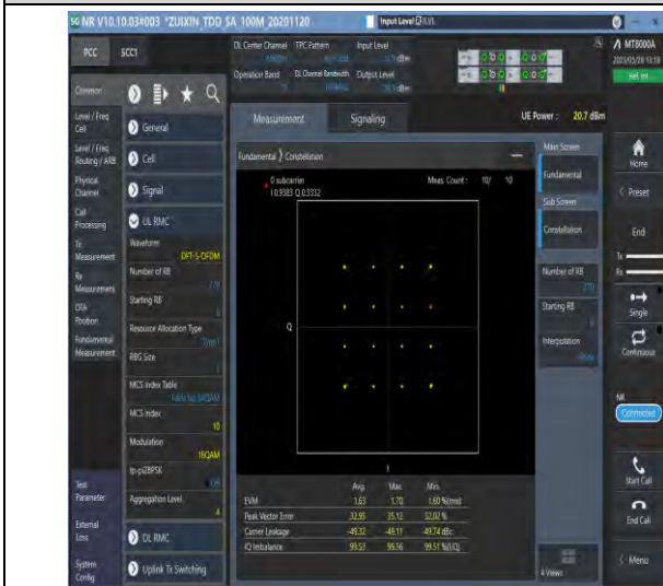
1-N77-3700-3980-PC3-30-100-M-3-DFT-16QAM-Out_er_Full-270@0-see graph-PASS
