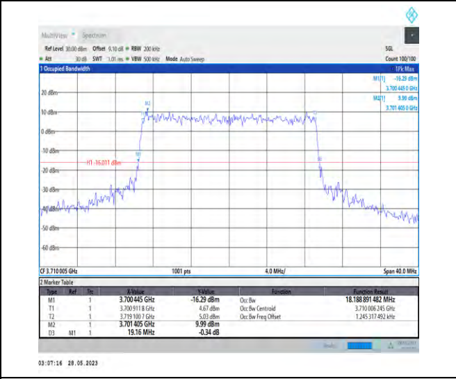
1-N77-3700-3980-PC3-30-20-L-8-CP-64QAM-Outer _Full-51@0-18.189-19.160-≤20-PASS
