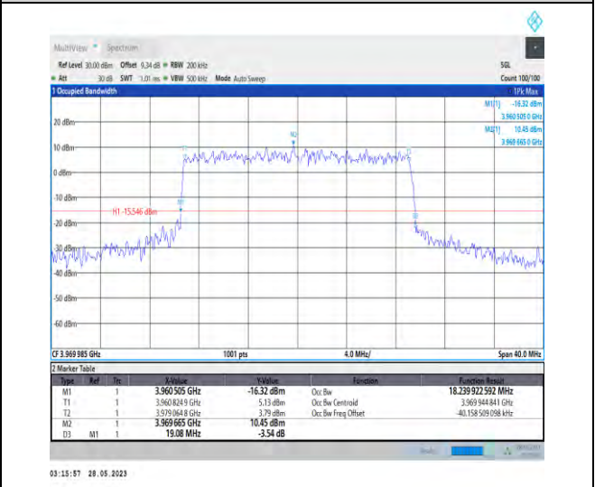
1-N77-3700-3980-PC3-30-20-H-7-CP-16QAM-Outer_Full-51@0-18.24-19.080-≤20-PASS
