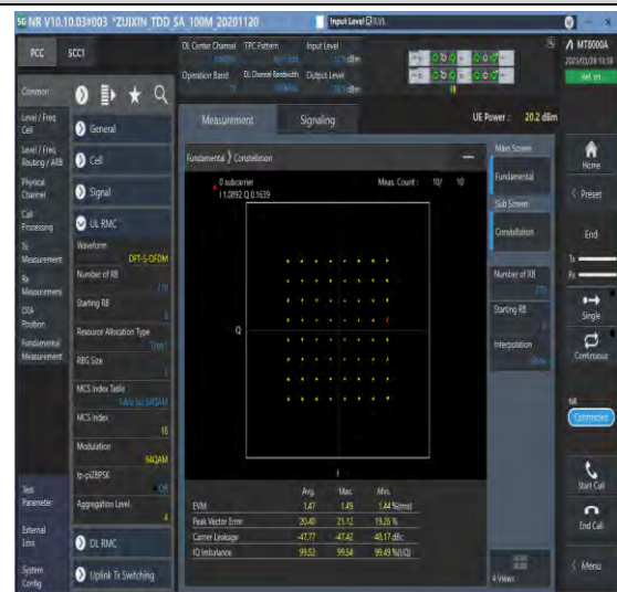
1-N77-3700-3980-PC3-30-100-M-4-DFT-64QAM-Out_er_Full-270@0-see graph-PASS
