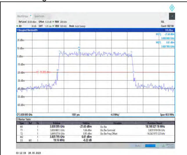
1-N77-3700-3980-PC3-30-20-M-9-CP-256QAM-Outer_Full-51@0-18.19-19.160-≤20-PASS
