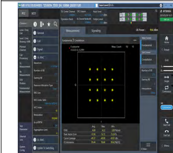
1-N77-3700-3980-PC3-30-100-M-7-CP-16QAM-Outer_Full-273@0-see graph-PASS
