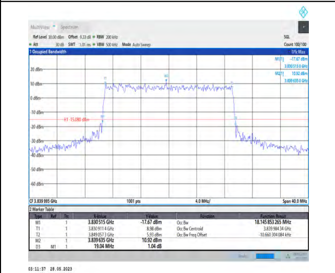
1-N77-3700-3980-PC3-30-20-M-7-CP-16QAM-Outer_Full-51@0-18.146-19.040-≤20-PASS
