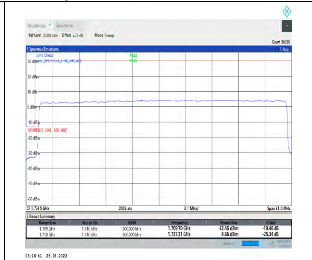
1-N66-PC3-15-30-L-3-DFT-PI2BPSK-Outer_Full-160@0-1-seegraph-PASS-see graph
