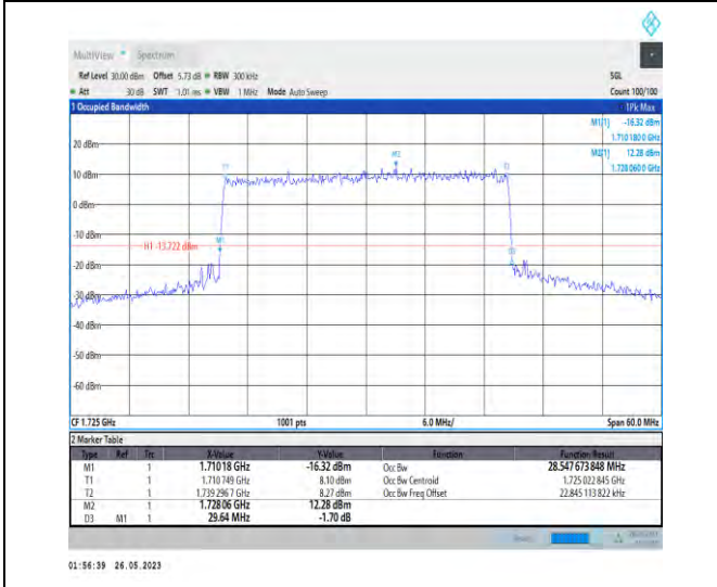
1-N66-PC3-15-30-L-7-CP-16QAM-Outer_Full-160@0 -28.548-29.640-≤30-PASS
