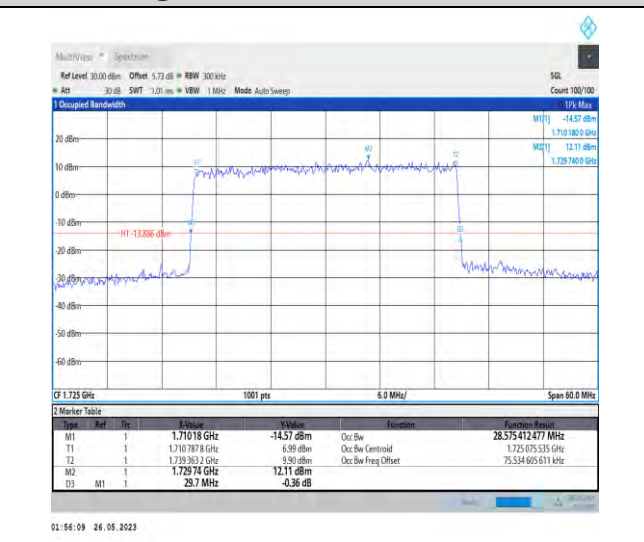
1-N66-PC3-15-30-L-4-DFT-64QAM-Outer_Full-160@ 0-28.575-29.700-≤30-PASS
