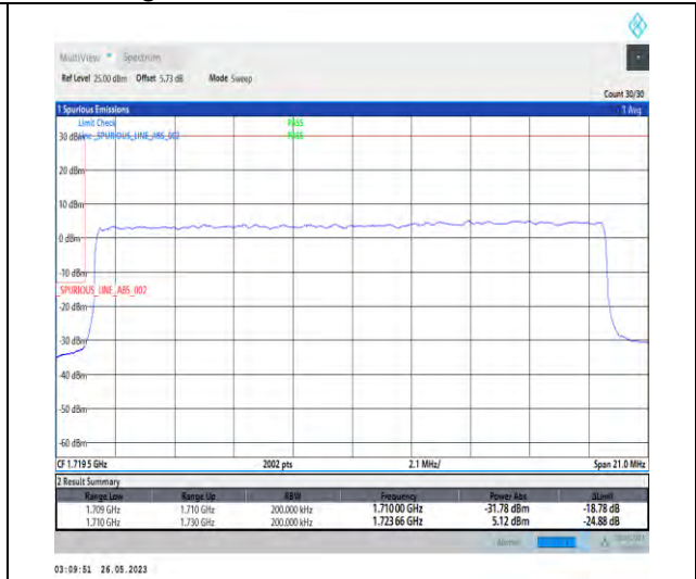
1-N66-PC3-15-20-L-3-DFT-PI2BPSK-Outer_Full-100@0-1-seegraph-PASS-see graph
