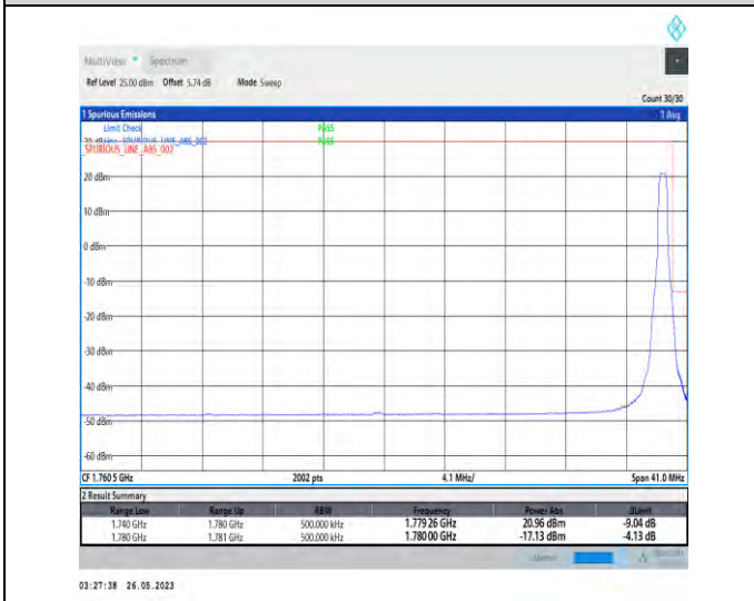
1-N66-PC3-15-40-H-5-CP-QPSK-Edge_1RB_Right-1@215-1-seegraph-PASS-see graph
