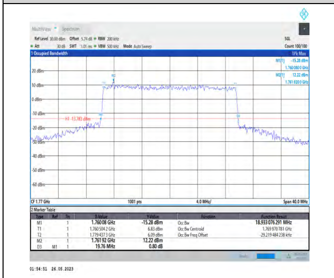
1-N66-PC3-15-20-H-8-CP-64QAM-Outer_Full-106@0 -18.933-19.760-<20-PASS
