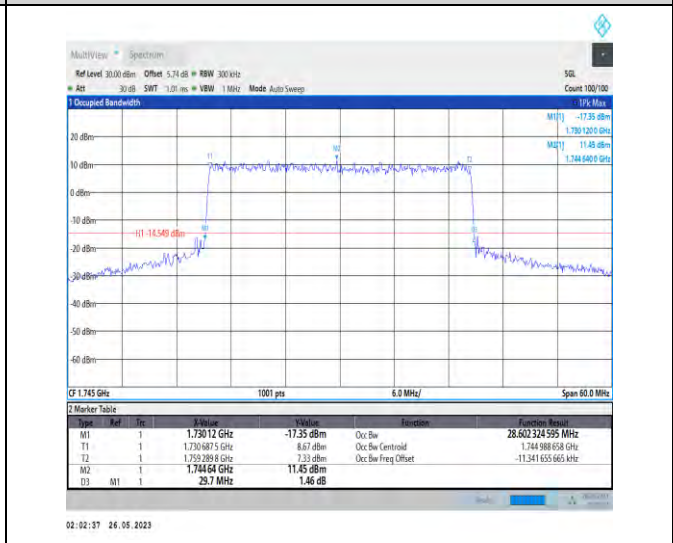
1-N66-PC3-15-30-M-7-CP-16QAM-Outer_Full-160@ 0-28.602-29.700-<30-PASS
