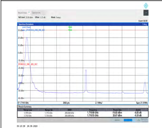
1-N66-PC3-15-20-L-4-CP-QPSK-Edge_1RB_Left-1@0-1-seegraph-PASS-see graph
