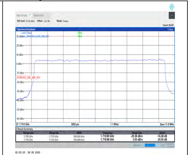
1-N66-PC3-15-10-L-3-DFT-PI2BPSK-Outer_Full-50@0-1-seegraph-PASS-see graph
