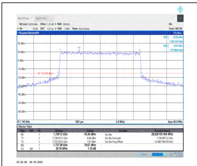
1-N66-PC3-15-30-M-8-CP-64QAM-Outer_Full-160 @0-28.63-29.760-<30-PASS
