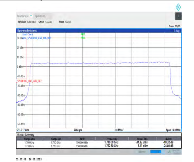
1-N66-PC3-15-15-L-3-DFT-PI2BPSK-Outer_Full-75@0-1-seegraph-PASS-see graph
