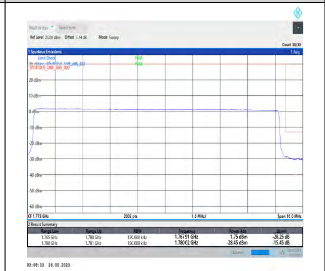
1-N66-PC3-15-15-H-6-CP-QPSK-Outer_Full-79@0-1-seegraph-PASS-see graph
