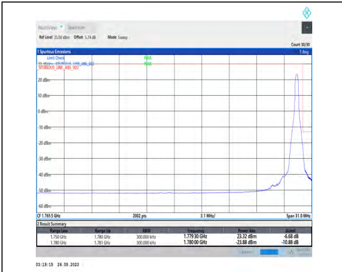
1-N66-PC3-15-30-H-2-DFT-PI2BPSK-Edge_1RB_Right-t-1@159-1-seegraph-PASS-see graph
