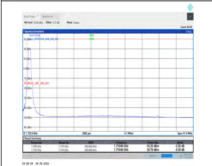
1-N66-PC3-15-40-L-4-CP-QPSK-Edge_1RB_Left-1@0-1-seegraph-PASS-see graph
