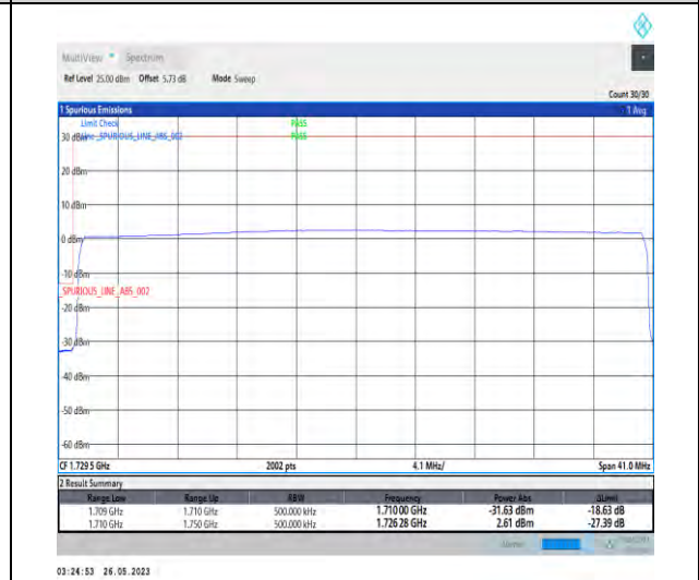
1-N66-PC3-15-40-L-6-CP-QPSK-Outer_Full-216@0-1-seegraph-PASS-see graph
