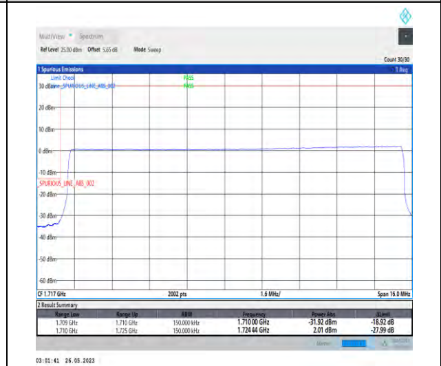
1-N66-PC3-15-15-L-6-CP-QPSK-Outer_Full-79@0-1-seegraph-PASS-see graph
