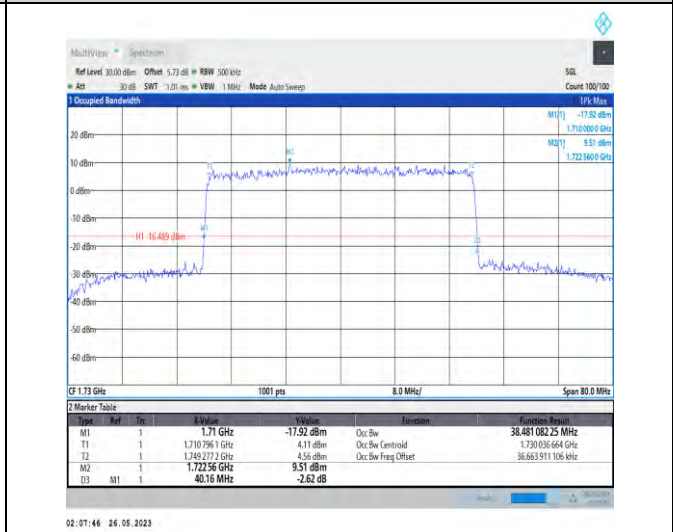
1-N66-PC3-15-40-L-9-CP-256QAM-Outer_Full-216@0 0-38.481-40.160-≤40-PASS
