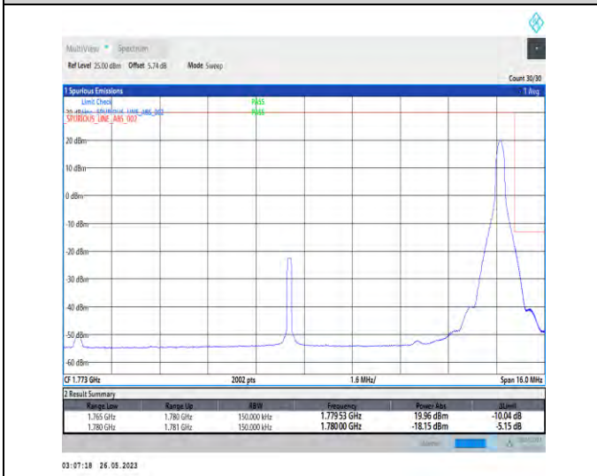
1-N66-PC3-15-15-H-5-CP-QPSK-Edge_1RB_Right-1@78-1-seegraph-PASS-see graph
