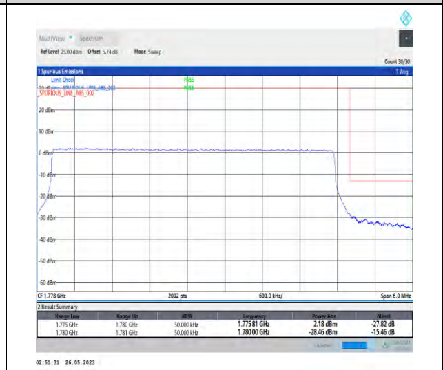
1-N66-PC3-15-5-H-6-CP-QPSK-Outer_Full-25@0-1-seegraph-PASS-see graph
