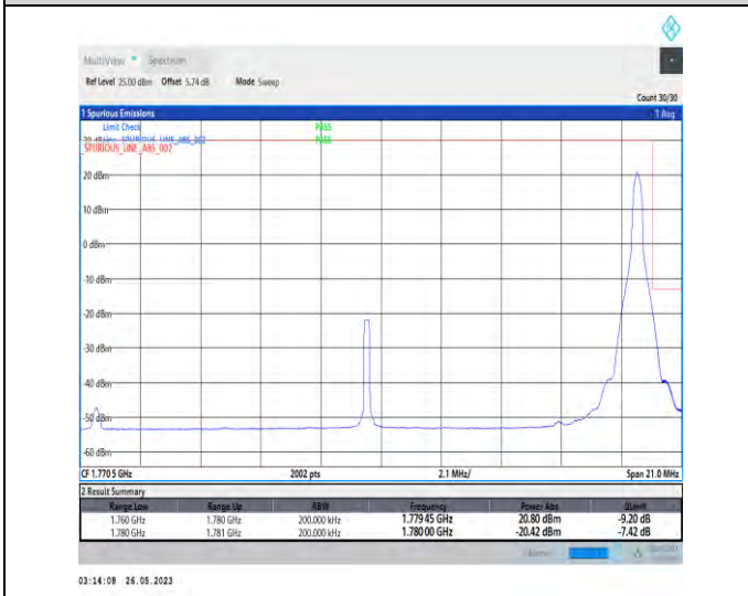
1-N66-PC3-15-20-H-5-CP-QPSK-Edge_1RB_Right-1@105-1-seegraph-PASS-see graph
