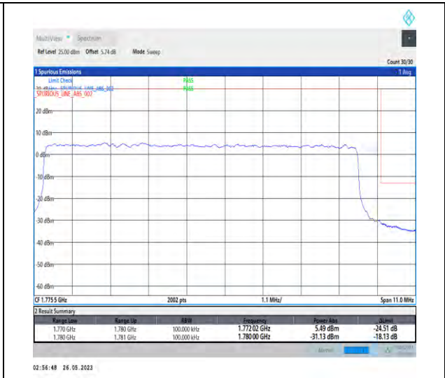
1-N66-PC3-15-10-H-3-DFT-PI2BPSK-Outer_Full-50@0-1-seegraph-PASS-see graph
