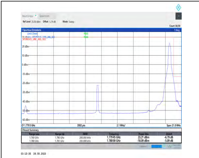
1-N66-PC3-15-20-H-2-DFT-PI2BPSK-Edge_1RB_Right-t-1@105-1-seegraph-PASS-see graph
