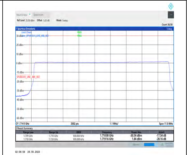
1-N66-PC3-15-10-L-6-CP-QPSK-Outer_Full-52@0-1-seegraph-PASS-see graph
