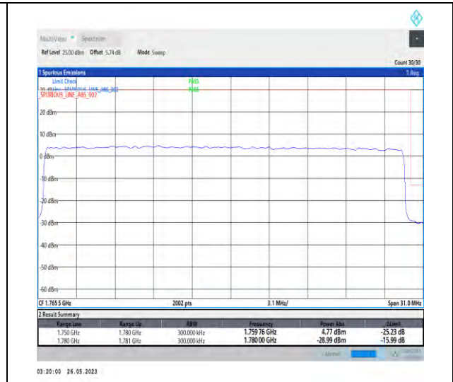
1-N66-PC3-15-30-H-3-DFT-PI2BPSK-Outer_Full-160@0-1-seegraph-PASS-see graph
