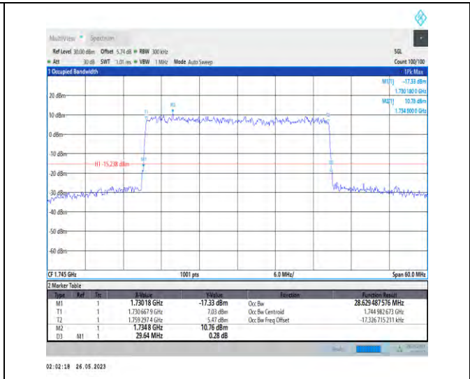
1-N66-PC3-15-30-M-5-DFT-256QAM-Outer_Full-160 @0-28.629-29.640-<30-PASS
