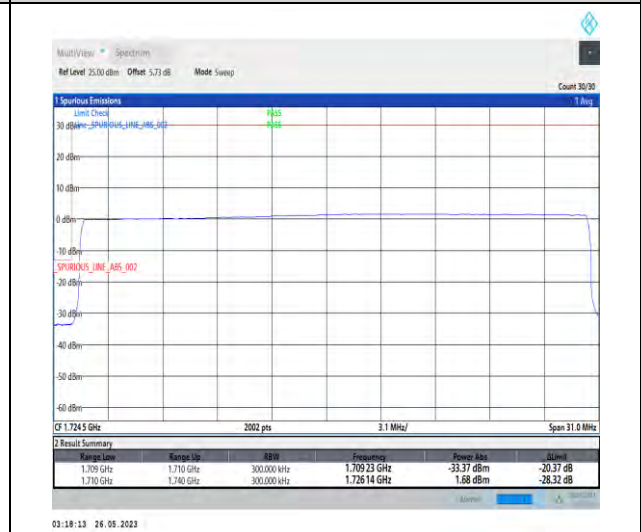
1-N66-PC3-15-30-L-6-CP-QPSK-Outer_Full-160@0-1-seegraph-PASS-see graph
