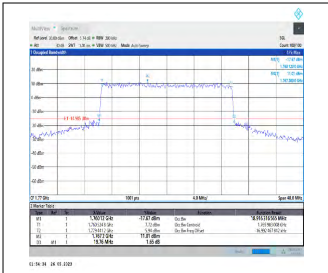
1-N66-PC3-15-20-H-6-CP-QPSK-Outer_Full-106@0 -18.916-19.760-<20-PASS
