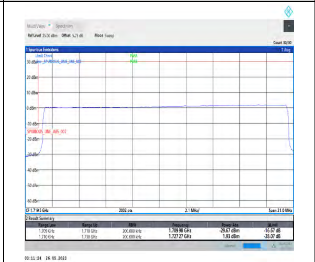
1-N66-PC3-15-20-L-6-CP-QPSK-Outer_Full-106@0-1-seegraph-PASS-see graph
