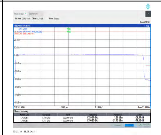
1-N66-PC3-15-30-H-6-CP-QPSK-Outer_Full-160@0-1-seegraph-PASS-see graph
