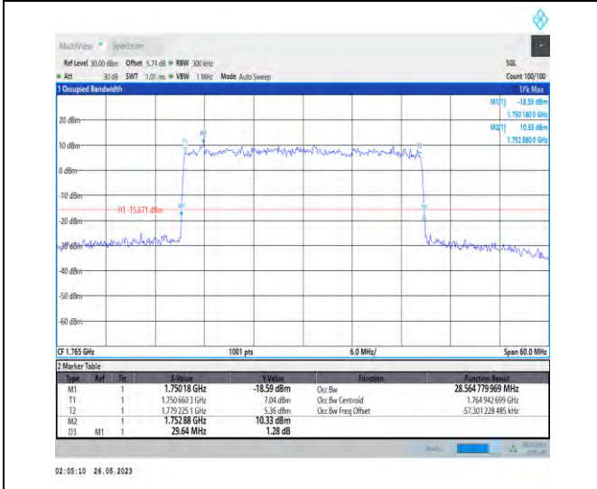
1-N66-PC3-15-30-H-5-DFT-256QAM-Outer_Full-160 @0-28.565-29.640-<=30-PASS
