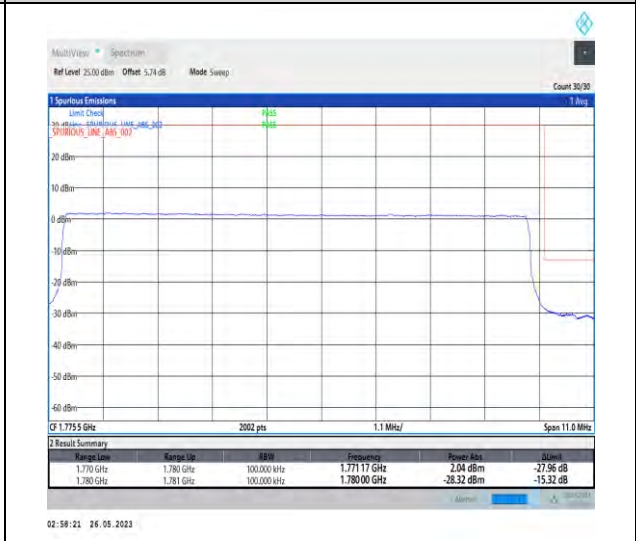
1-N66-PC3-15-10-H-6-CP-QPSK-Outer_Full-52@0-1-seegraph-PASS-see graph
