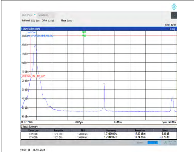
1-N66-PC3-15-15-L-4-CP-QPSK-Edge_1RB_Left-1@0-1-seegraph-PASS-see graph
