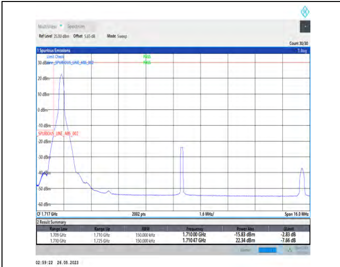
1-N66-PC3-15-15-L-1-DFT-PI2BPSK-Edge_1RB_Left-1@0-1-seegraph-PASS-see graph
