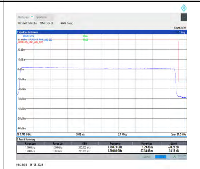
1-N66-PC3-15-20-H-6-CP-QPSK-Outer_Full-106@0-1-seegraph-PASS-see graph
