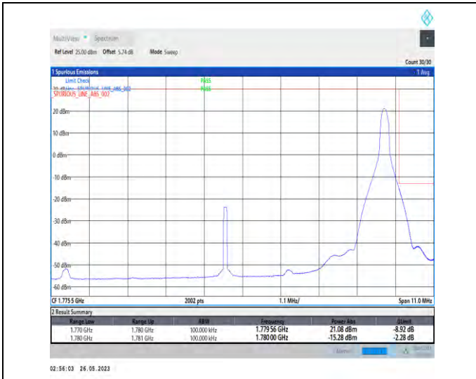
1-N66-PC3-15-10-H-2-DFT-PI2BPSK-Edge_1RB_Right-t1@51-1-seegraph-PASS-see graph
