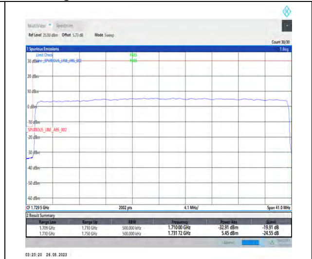
1-N66-PC3-15-40-L-3-DFT-PI2BPSK-Outer_Full-216@0-1-seegraph-PASS-see graph
