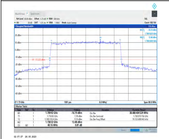
1-N66-PC3-15-40-L-8-CP-64QAM-Outer_Full-216@0 0-38.48-40.160-≤40-PASS
