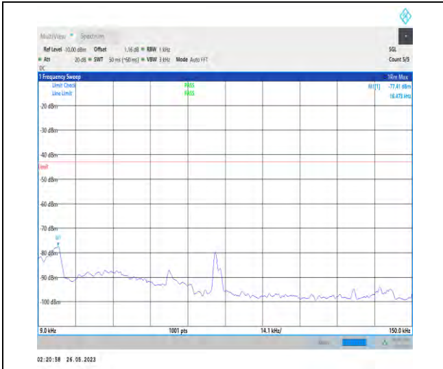
1-N66-PC3-15-40-H-1-DFT-PI2BPSK-Inner_1RB_L eft-1@1-0.009-0.15-0.13--93.43--43-PASS
