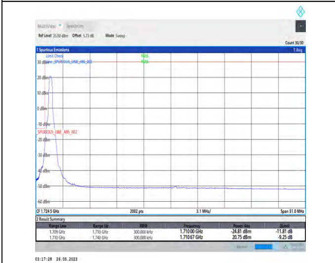
1-N66-PC3-15-30-L-4-CP-QPSK-Edge_1RB_Left-1@0-1-seegraph-PASS-see graph
