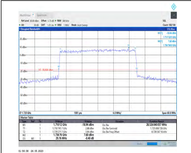
1-N66-PC3-15-30-L-9-CP-256QAM-Outer_Full-160@ 0-28.526-29.760-<30-PASS
