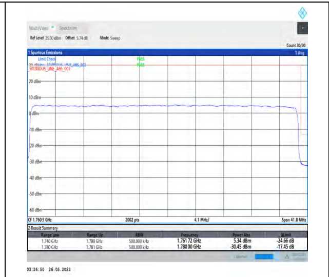
1-N66-PC3-15-40-H-3-DFT-PI2BPSK-Outer_Full-216@0-1-seegraph-PASS-see graph
