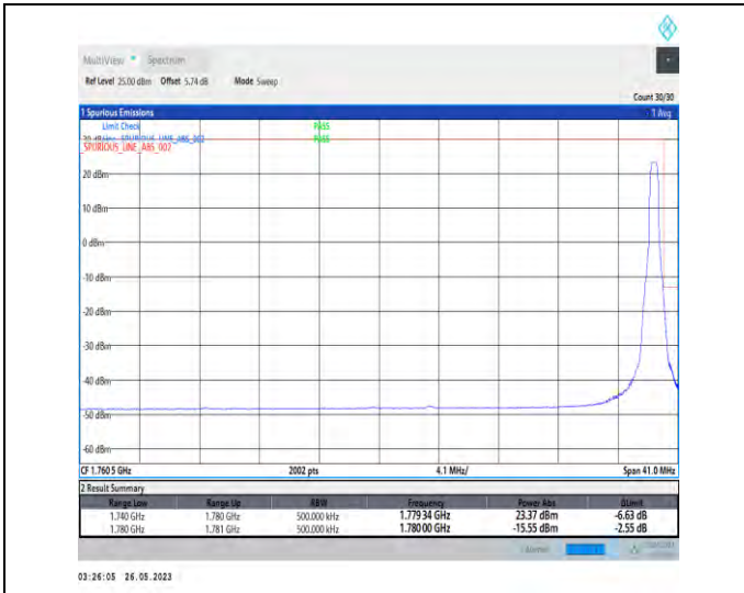
1-N66-PC3-15-40-H-2-DFT-PI2BPSK-Edge_1RB_Right-t-1@215-1-seegraph-PASS-see graph
