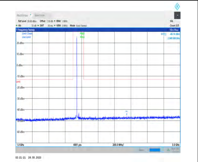
1-N66-PC3-15-40-H-1-DFT-PI2BPSK-Inner_1RB_Lef t-1@1-1000-3000-2904.00--44.35--13-PASS
