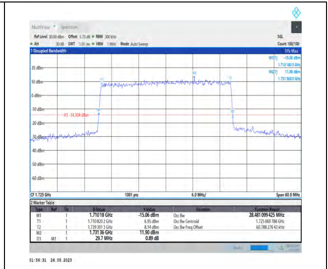
1-N66-PC3-15-30-L-6-CP-QPSK-Outer_Full-160@0 -28.481-29.700-≤30-PASS
