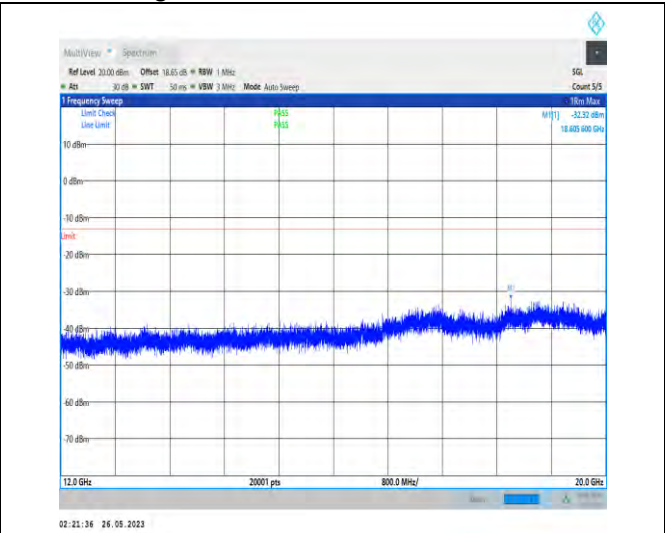
1-N66-PC3-15-40-H-1-DFT-PI2BPSK-Inner_1RB_Lef t-1@1-12000-20000-17324.00--33.24--13-PASS
