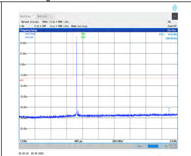
1-N66-PC3-15-40-M-1-DFT-PI2BPSK-Inner_1RB_Lef t-1@1-1000-3000-2657.00--44.79--13-PASS
