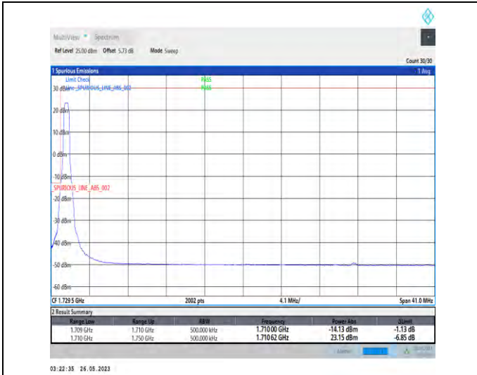
1-N66-PC3-15-40-L-1-DFT-PI2BPSK-Edge_1RB_Left-1@0-1-seegraph-PASS-see graph
