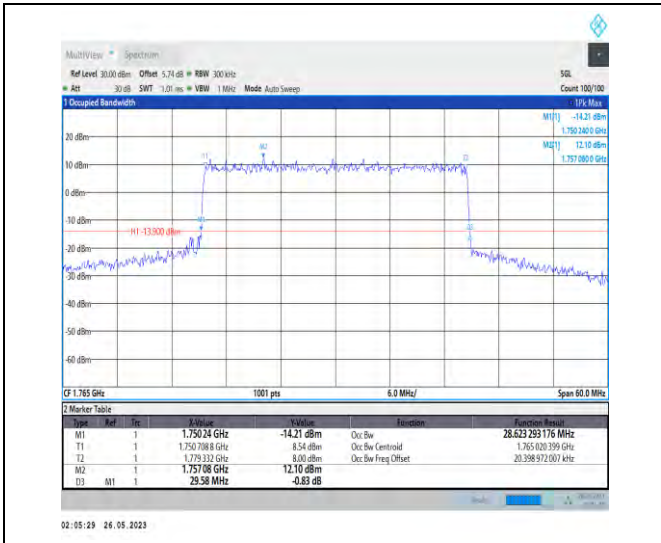
1-N66-PC3-15-30-H-7-CP-16QAM-Outer_Full-160@ 0-28.623-29.580-≤30-PASS
