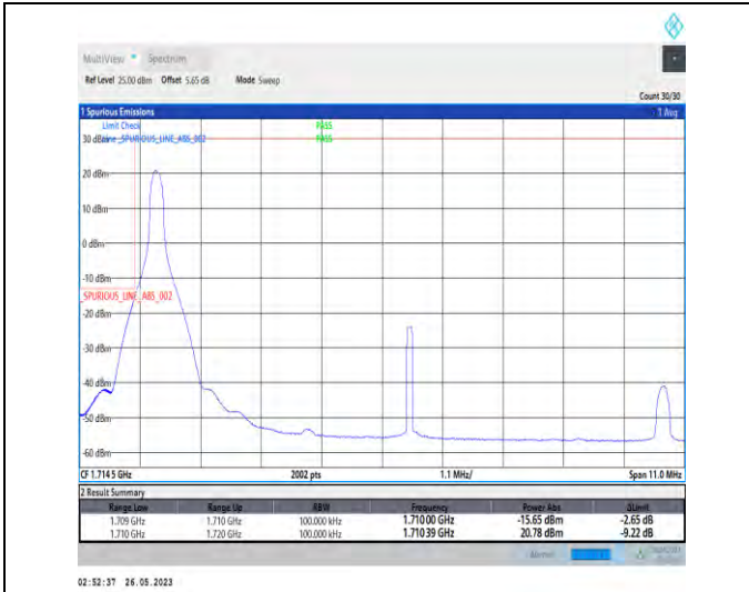
1-N66-PC3-15-10-L-1-DFT-PI2BPSK-Edge_1RB_Left-1@0-1-seegraph-PASS-see graph
