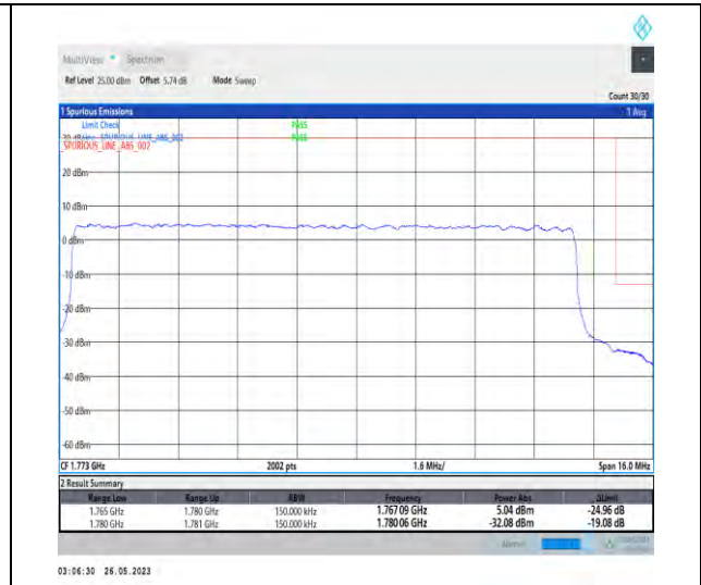
1-N66-PC3-15-15-H-3-DFT-PI2BPSK-Outer_Full-75@0-1-seegraph-PASS-see graph
