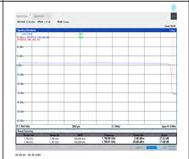
1-N66-PC3-15-40-H-6-CP-QPSK-Outer_Full-216@0-1-seegraph-PASS-see graph
