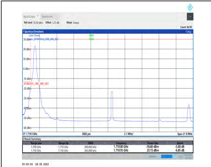
1-N66-PC3-15-20-L-1-DFT-PI2BPSK-Edge_1RB_Left-1@0-1-seegraph-PASS-see graph
