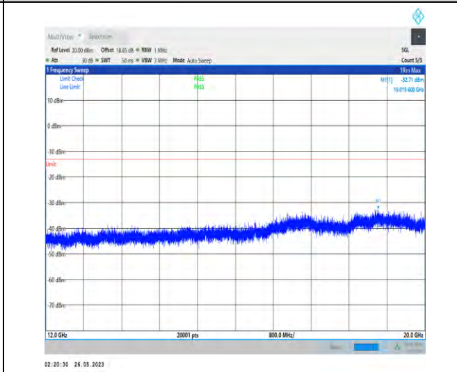
1-N66-PC3-15-40-M-1-DFT-PI2BPSK-Inner_1RB_Lef t-1@1-12000-20000-17533.20--33.17--13-PASS
