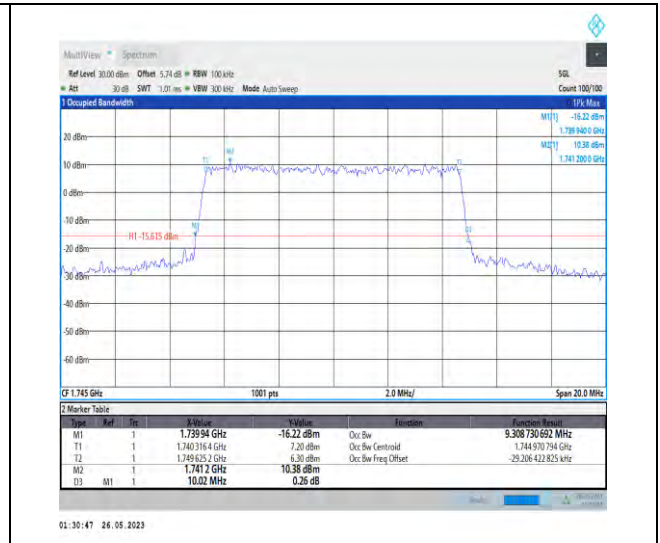
1-N66-PC3-15-10-M-6-CP-QPSK-Outer_Full-52@0- 9.309-10.020-≤10-PASS
