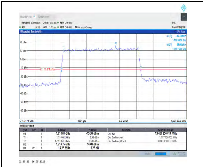
1-N66-PC3-15-15-L-3-DFT-16QAM-Outer_Full-75@0 -13.456-14.250-≤15-PASS
