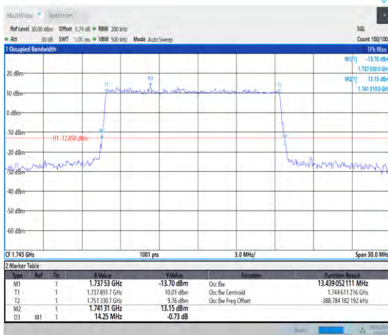
1-N66-PC3-15-15-M-4-DFT-64QAM-Outter_Full-75@ 0-13.439-14.250-≤15-PASS
