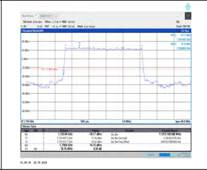
1-N66-PC3-15-20-M-2-DFT-PI2BPSK-Outer_Full-100 @0-17.915-18.760-<=20-PASS
