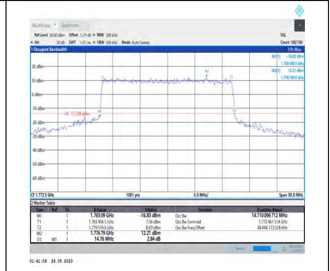
1-N66-PC3-15-15-H-8-CP-64QAM-Outer_Full-79@ 0-14.11-14.760-≤15-PASS
