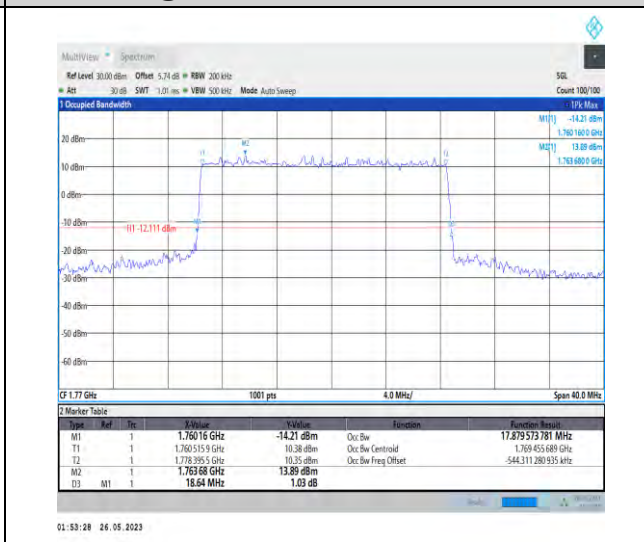
1-N66-PC3-15-20-H-1-DFT-QPSK-Outer_Full-100@ 0-17.88-18.640-<20-PASS
