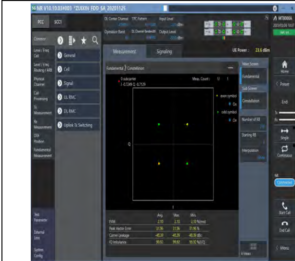
1-N66-PC3-15-40-M-1-DFT-PI2BPSK-Outer_Full-216 @0-see graph-PASS
