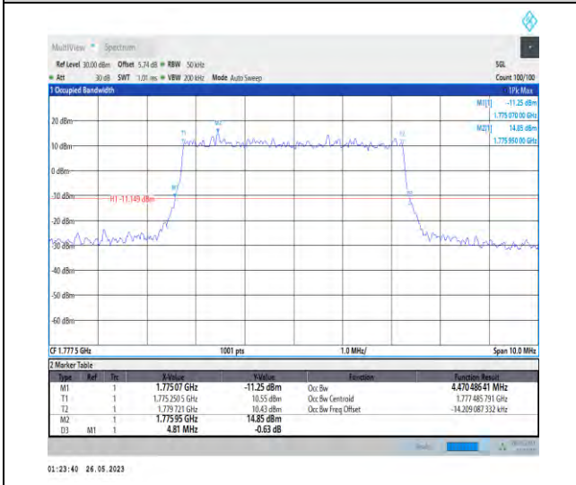
1-N66-PC3-15-5-H-1-DFT-QPSK-Outer_Full-25@0- 4.47-4.810-≤5-PASS
