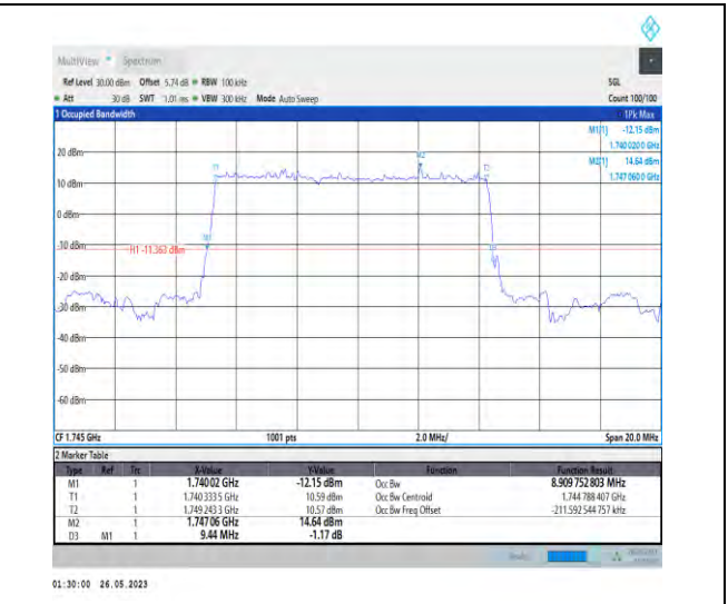
1-N66-PC3-15-10-M-2-DFT-PI2BPSK-Outter_Full-50@ @0-8.91-9.440-≤10-PASS
