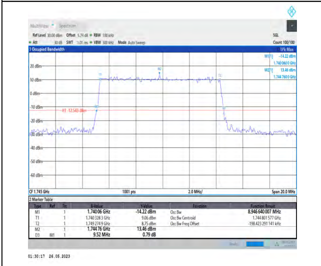
1-N66-PC3-15-10-M-3-DFT-16QAM-Outter_Full-50@ 0-8.947-9.520-≤10-PASS
