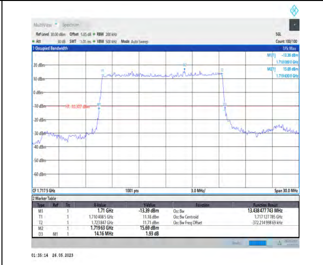
1-N66-PC3-15-15-L-2-DFT-PI2BPSK-Outer_Full-75@ 0-13.438-14.160-≤15-PASS
