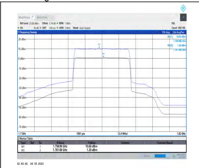
1-N66-PC3-15-40-H-2-CP-256QAM-Outer_Full-216 @0-9.40-100%-0.00-9.40-PASS-≤13
