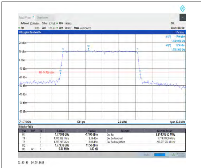
1-N66-PC3-15-10-H-4-DFT-64QAM-Outer_Full-50@ 0-8.914-9.540-≤10-PASS
