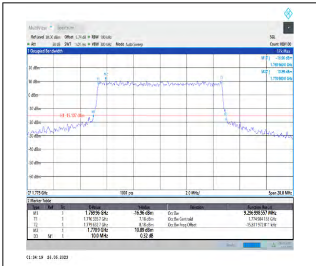
1-N66-PC3-15-10-H-8-CP-64QAM-Outer_Full-52@ 0-9.297-10.000-≤10-PASS
