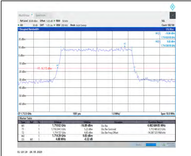
1-N66-PC3-15-5-L-5-DFT-256QAM-Outer_Full-25@0 -4.483-4.880-≤5-PASS
