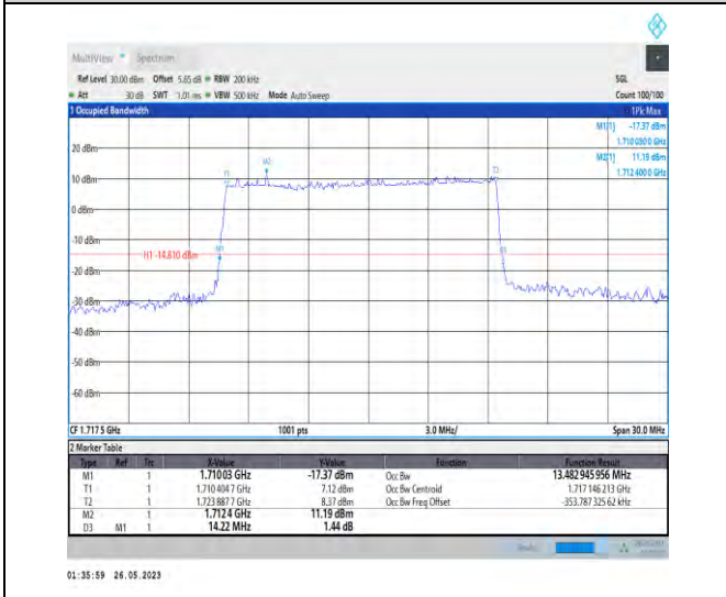
1-N66-PC3-15-15-L-5-DFT-256QAM-Outer_Full-75@0 0-13.483-14.220-≤15-PASS
