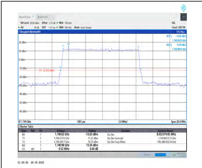
1-N66-PC3-15-10-M-1-DFT-QPSK-Outter_Full-50@ -8.932-9.520-≤10-PASS
