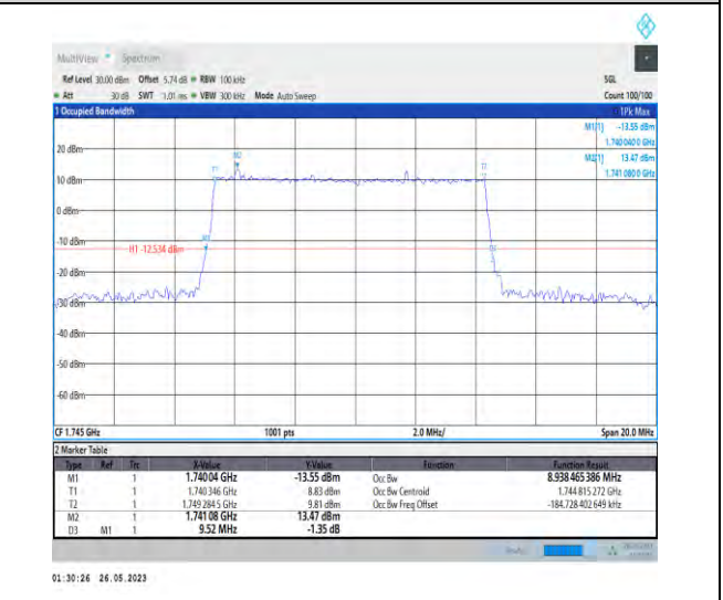
1-N66-PC3-15-10-M-4-DFT-64QAM-Outter_Full-50@ 0-8.938-9.520-≤10-PASS
