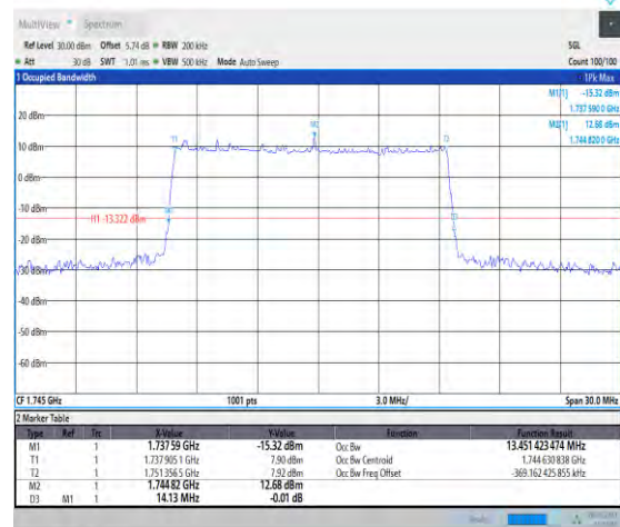
1-N66-PC3-15-15-M-5-DFT-256QAM-Outter_Full-75 @0-13.451-14.130-≤15-PASS
