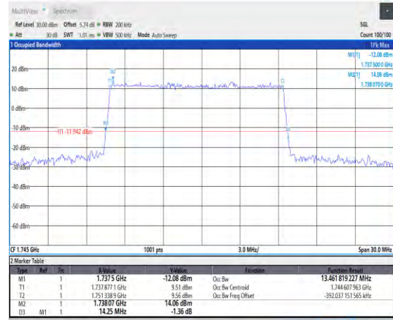
1-N66-PC3-15-15-M-3-DFT-16QAM-Outter_Full-75@ 0-13.462-14.250-≤15-PASS
