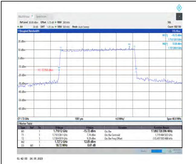
1-N66-PC3-15-20-L-4-DFT-64QAM-Outer_Full-100 @0-17.893-18.720-≤20-PASS
