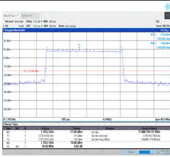
1-N66-PC3-15-20-M-3-DFT-16QAM-Outer_Full-100 @0-17.891-18.720-<20-PASS
