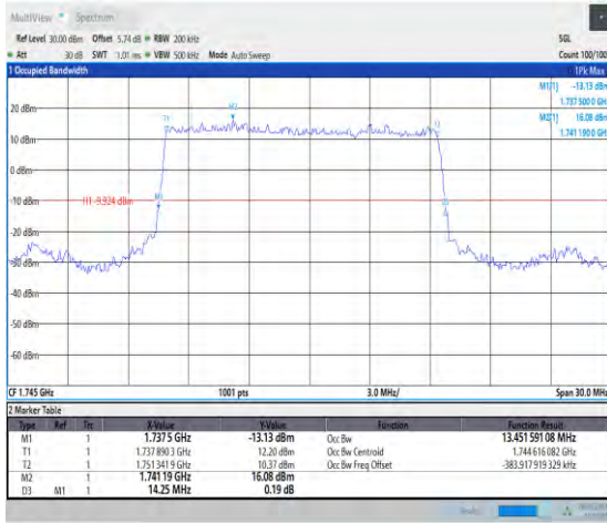
1-N66-PC3-15-15-M-2-DFT-PI2BPSK-Outter_Full-75 @0-13.452-14.250-≤15-PASS
