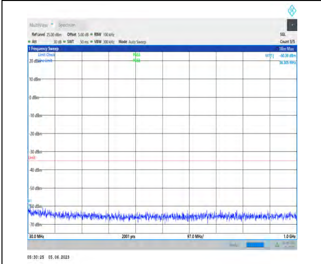
1-N41-PC3-30-100-M-1-N/A-DFT-PI2BPSK-Inner_1 RB_Left-1@1-30-1000-36.31--60.39--35-PASS
