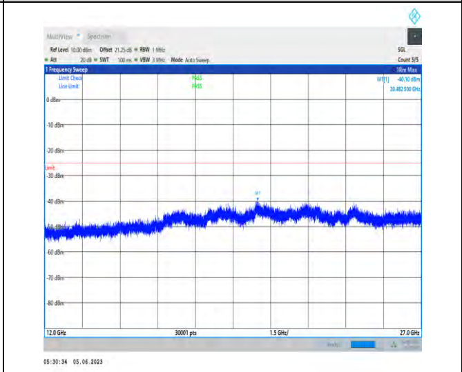
1-N41-PC3-30-100-M-1-N/A-DFT-PI2BPSK-Inner_1R B_Left-1@1-12000-27000-20482.50--40.10--25-PAS
