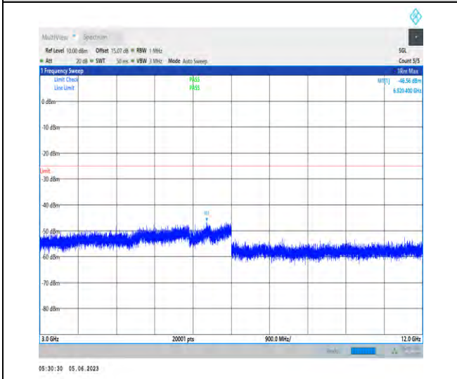
1-N41-PC3-30-100-M-1-N/A-DFT-PI2BPSK-Inner_1 RB_Left-1@1-3000-12000-6920.40--46.56--25-PAS
