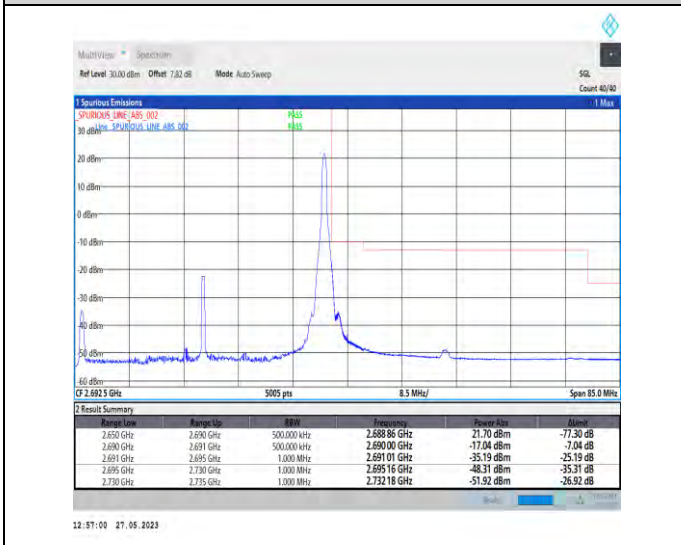
1-N41-PC3-30-40-H-5-CP-QPSK-Edge_1RB_Right-1@105-1--PASS-see graph
