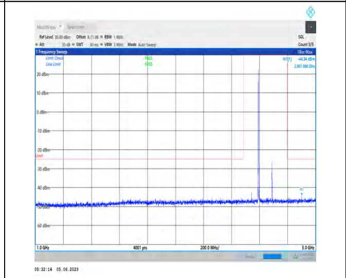
1-N41-PC3-30-100-H-1-N/A-DFT-PI2BPSK-Inner_1R B_Left-1@1-1000-3000-2901.00--44.34--25-PASS
