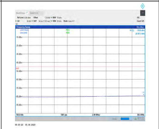
1-N41-PC3-30-100-M-1-N/A-DFT-PI2BPSK-Inner_1R B_Left-1@1-0.15-30-29.70--78.83--45-PASS
