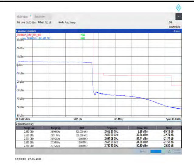
1-N41-PC3-30-40-H-6-CP-QPSK-Outer_Full-100@0-1--PASS-see graph
