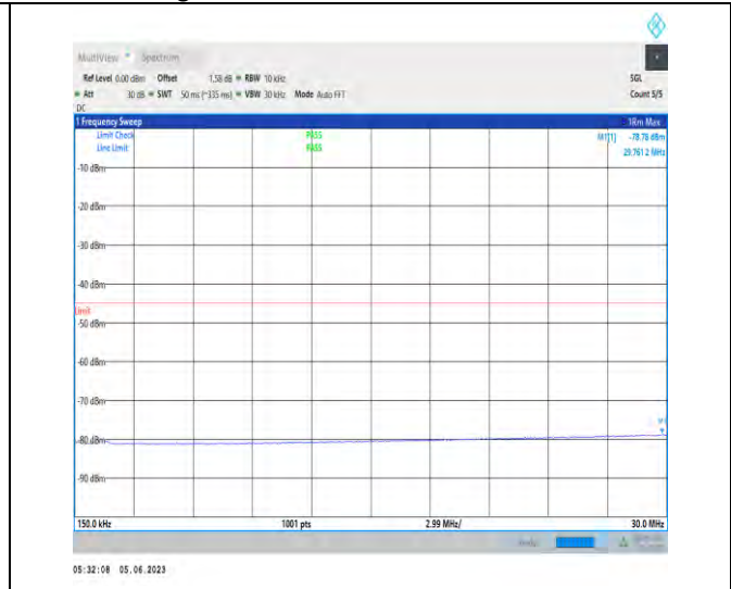
1-N41-PC3-30-100-H-1-N/A-DFT-PI2BPSK-Inner_1R B_Left-1@1-0.15-30-29.76--78.78--45-PASS
