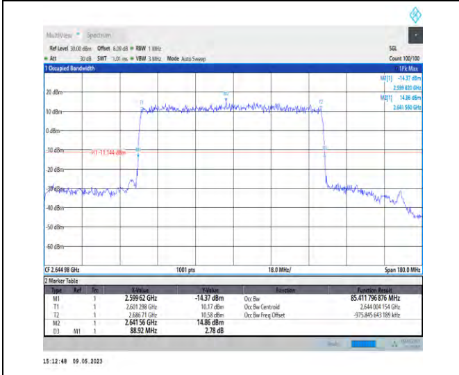
1-N41-PC3-30-90-H-2-DFT-PI2BPSK-Outer_Full-240 @0-85.412-88.920-<90-PASS
