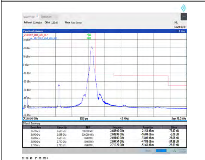
1-N41-PC3-30-20-H-5-CP-QPSK-Edge_1RB_Right-1@50-1--PASS-see graph
