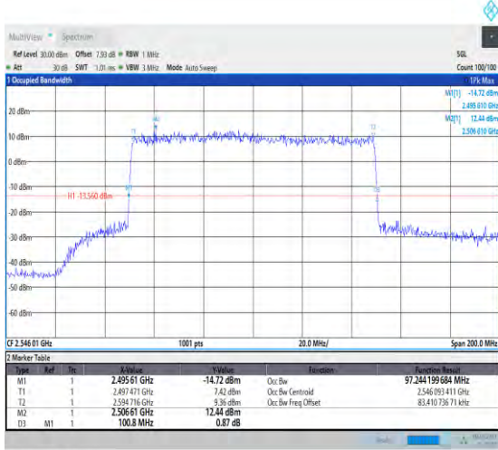
1-N41-PC3-30-100-L-7-CP-16QAM-Outer_Full-273 @0-97.244-100.800-≤100-PASS
