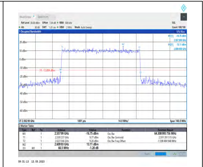
1-N41-PC3-30-70-M-4-DFT-64QAM-Outer_Full-180 @0-64.309-66.50-≤70-PASS
