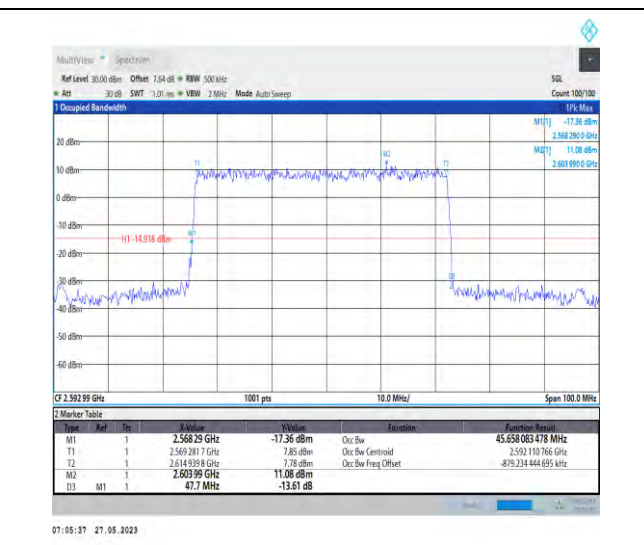
1-N41-PC3-30-50-M-5-DFT-256QAM-Outer_Full-128 @0-45.658-47.700-<50-PASS
