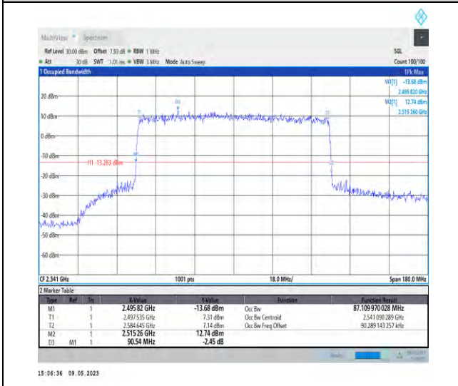
1-N41-PC3-30-90-L-8-CP-64QAM-Outer_Full-245@0 0-87.11-90.540-<=90-PASS
