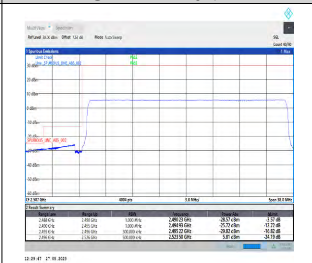
1-N41-PC3-30-30-L-6-CP-QPSK-Outer_Full-78@0-1--PASS-see graph
