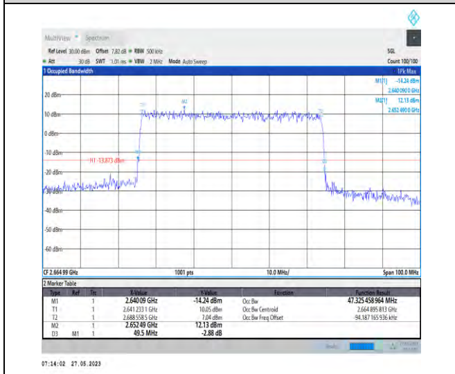
1-N41-PC3-30-50-H-7-CP-16QAM-Outer_Full-133@ 0-47.325-49.500-<=50-PASS
