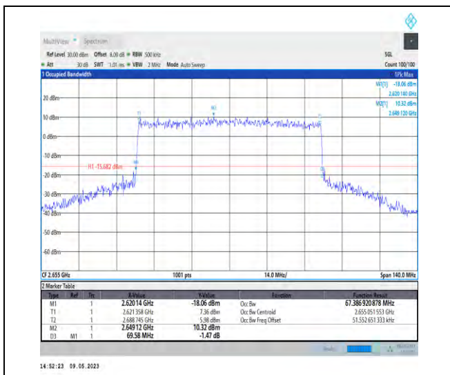
1-N41-PC3-30-70-H-6-CP-QPSK-Outer_Full-189@0 -67.387-69.580-<=70-PASS
