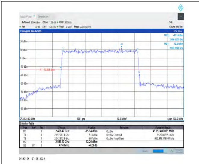
1-N41-PC3-30-50-L-5-DFT-256QAM-Outer_Full-128 @0-45.651-47.400-≤50-PASS
