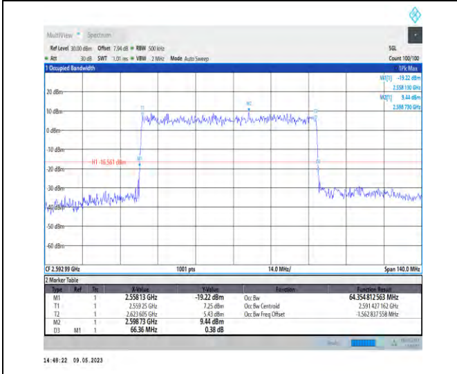
1-N41-PC3-30-70-M-5-DFT-256QAM-Outer_Full-180 @0-64.355-66.360-≤70-PASS
