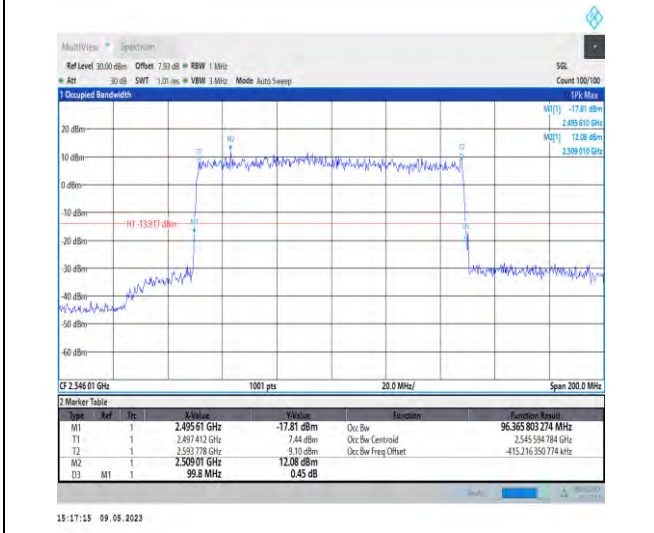
1-N41-PC3-30-100-L-5-DFT-256QAM-Outer_Full-27 @0-96.366-99.800-≤100-PASS
