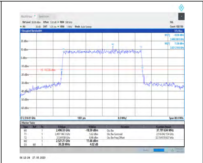
1-N41-PC3-30-40-L-9-CP-256QAM-Outer_Full-106 @0-37.792-39.280-<40-PASS
