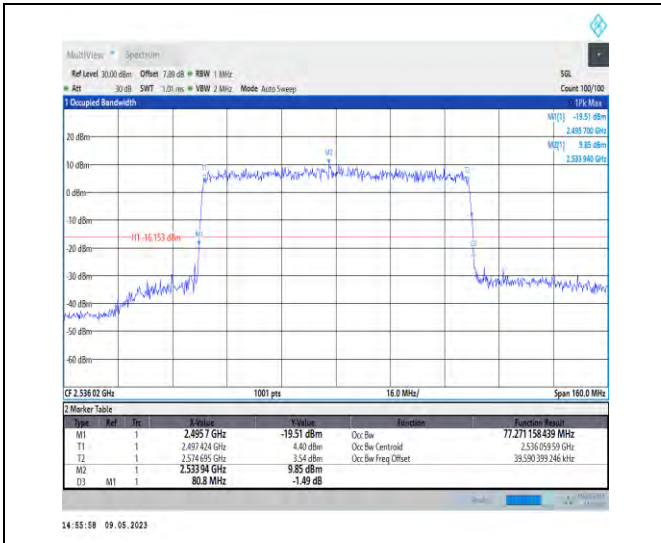
1-N41-PC3-30-80-L-9-CP-256QAM-Outer_Full-217@ 0-77.271-80.800-<80-PASS
