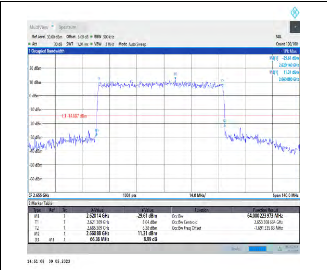
1-N41-PC3-30-70-H-3-DFT-16QAM-Outer_Full-180 @0-64-66.360-<=70-PASS
