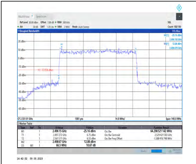
1-N41-PC3-30-70-L-4-DFT-64QAM-Outer_Full-180 @0-64.299-66.500-<70-PASS
