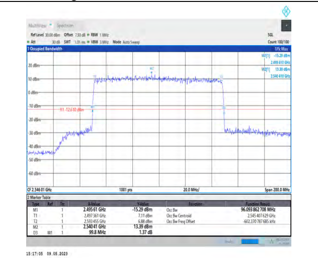
1-N41-PC3-30-100-L-4-DFT-64QAM-Outer_Full-270 @0-96.094-99.800-≤100-PASS
