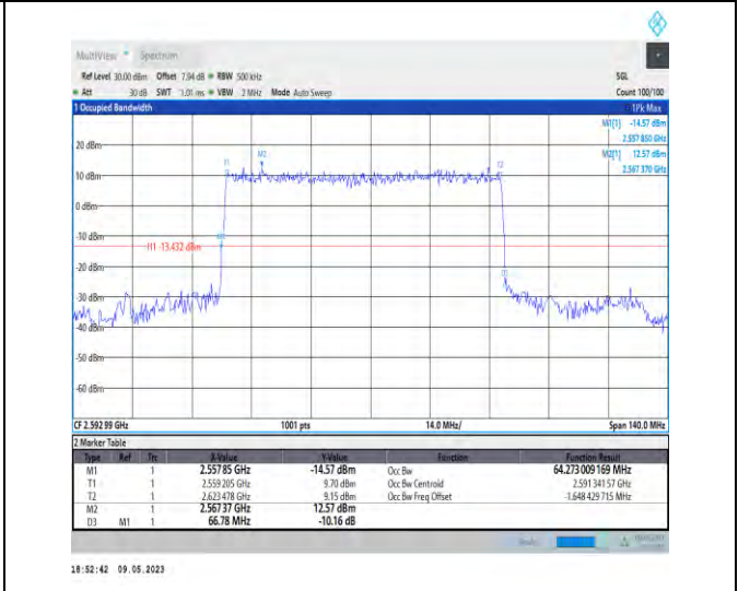
1-N41-PC3-30-70-M-2-DFT-PI2BPSK-Outer_Full-180 @0-64.273-66.780-<=70-PASS
