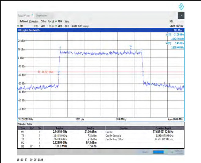
1-N41-PC3-30-100-M-9-CP-256QAM-Outer_Full-27 3@0-97.637-101.000-≤100-PASS
