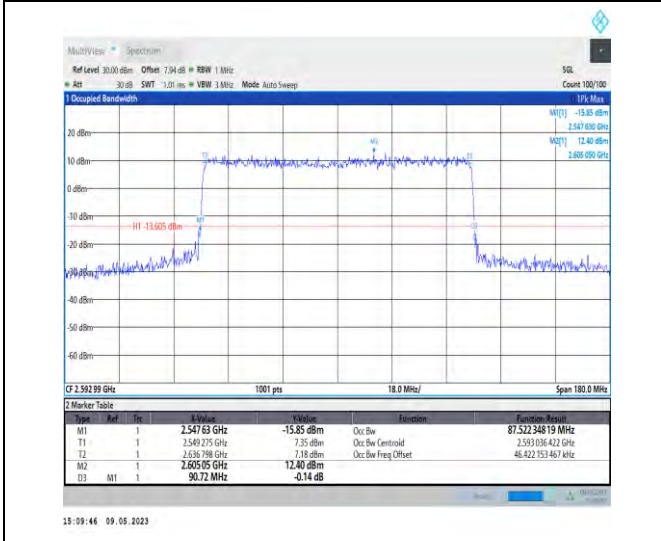
1-N41-PC3-30-90-M-7-CP-16QAM-Outer_Full-245 @0-87.522-90.720-<90-PASS
