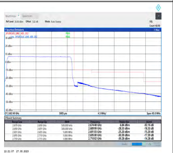
1-N41-PC3-30-20-H-6-CP-QPSK-Outer_Full-51@0-1--PASS-see graph
