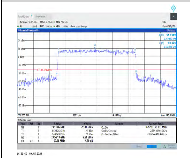
1-N41-PC3-30-70-H-8-CP-64QAM-Outer_Full-189@0 -67.205-69.860-<=70-PASS
