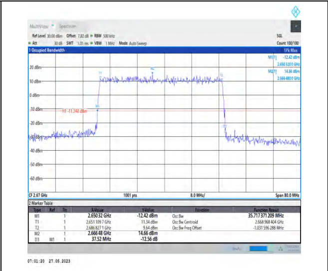
1-N41-PC3-30-40-H-3-DFT-16QAM-Outer_Full-100 @0-35.717-37.520-<40-PASS
