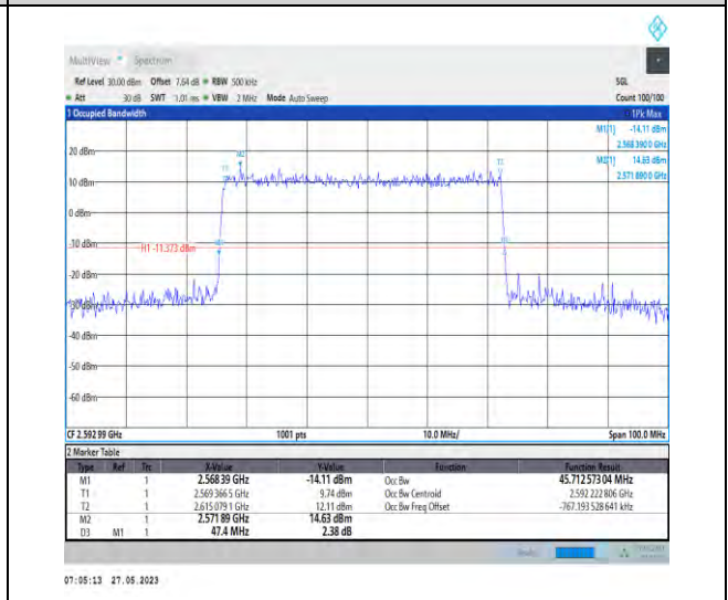
1-N41-PC3-30-50-M-3-DFT-16QAM-Outer_Full-128 @0-45.713-47.400-≤50-PASS
