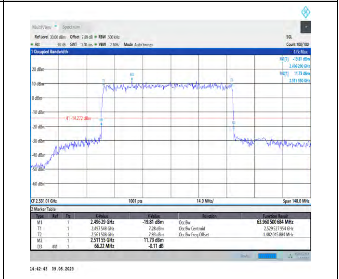
1-N41-PC3-30-70-L-3-DFT-16QAM-Outer_Full-180 @0-63.961-66.220-≤70-PASS
