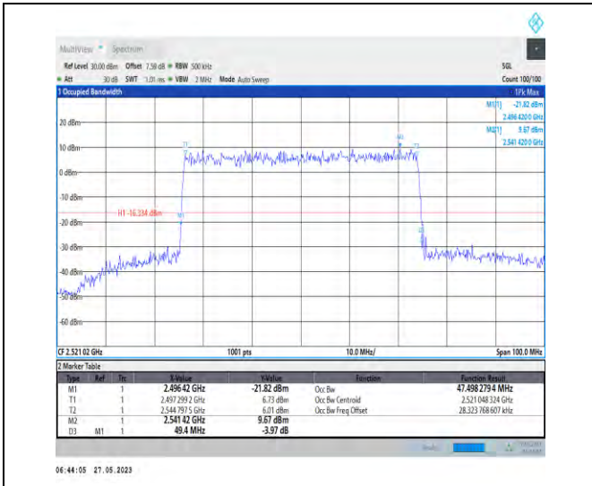
1-N41-PC3-30-50-L-9-CP-256QAM-Outer_Full-133@ 0-47.498-49.400-≤50-PASS
