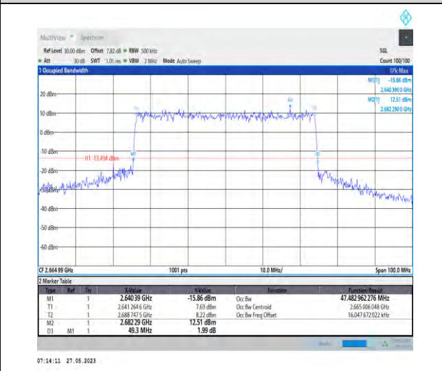
1-N41-PC3-30-50-H-8-CP-64QAM-Outer_Full-133@ 0-47.483-49.300-<=50-PASS
