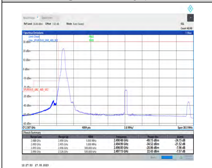
1-N41-PC3-30-30-L-4-CP-QPSK-Edge_1RB_Left-1@0-1--PASS-see graph
