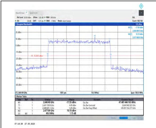
1-N41-PC3-30-50-H-9-CP-256QAM-Outer_Full-133 @0-47.481-49.000-≤50-PASS
