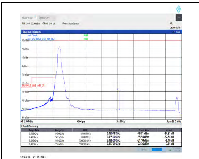
1-N41-PC3-30-30-L-1-DFT-PI2BPSK-Edge_1RB_Left-1@0-1--PASS-see graph
