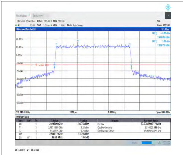
1-N41-PC3-30-40-L-8-CP-64QAM-Outer_Full-106 @0-37.778-39.680-<40-PASS
