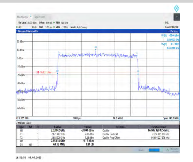
1-N41-PC3-30-70-H-9-CP-256QAM-Outer_Full-189@0 -66.847-69.160-<=70-PASS
