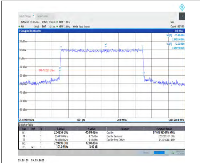
1-N41-PC3-30-100-M-6-CP-QPSK-Outer_Full-273@ 0-97.62-101.000-≤100-PASS
