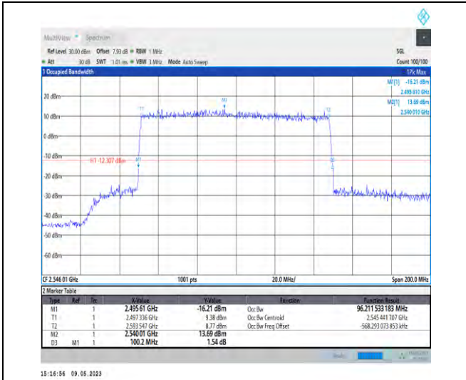
1-N41-PC3-30-100-L-3-DFT-16QAM-Outer_Full-270 @0-96.212-100.200-≤100-PASS
