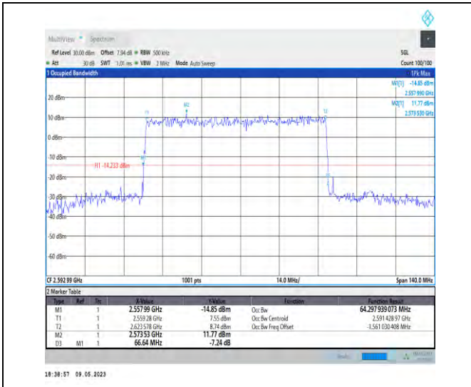
1-N41-PC3-30-70-M-3-DFT-16QAM-Outer_Full-180@ 0-64.298-66.640-≤70-PASS
