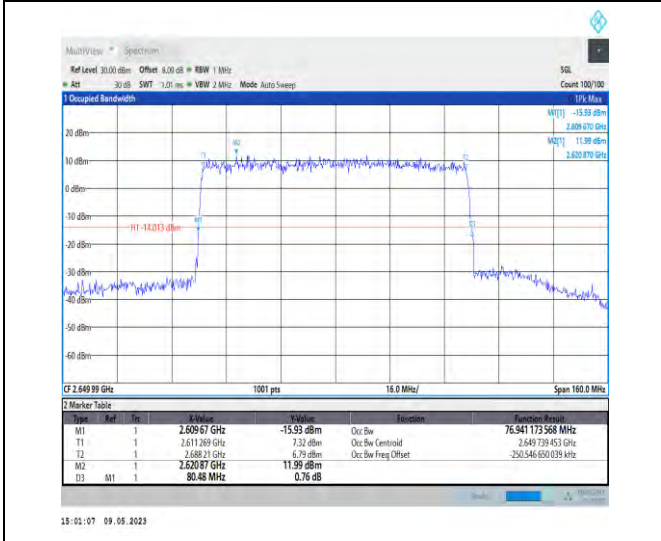
1-N41-PC3-30-80-H-5-DFT-256QAM-Outer_Full-216 @0-76.941-80.480-<80-PASS
