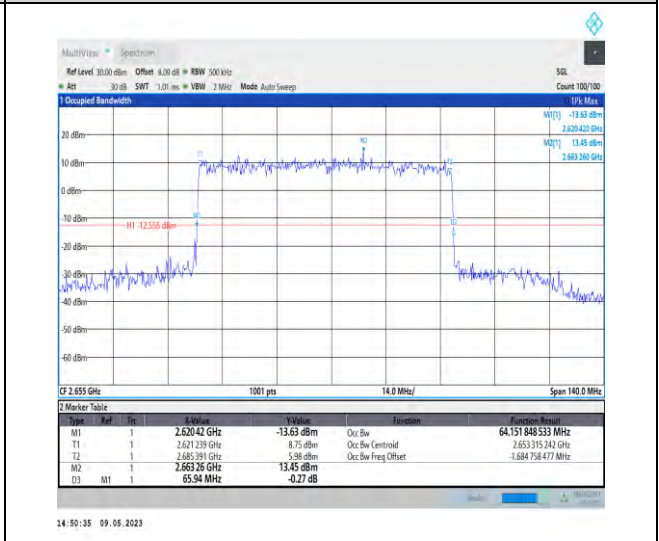
1-N41-PC3-30-70-H-1-DFT-QPSK-Outer_Full-180@ 0-64.152-65.940-≤70-PASS
