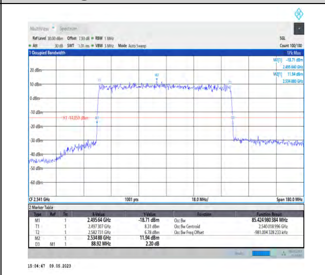
1-N41-PC3-30-90-L-5-DFT-256QAM-Outter_Full-240 @0-85.425-88.920-<=90-PASS
