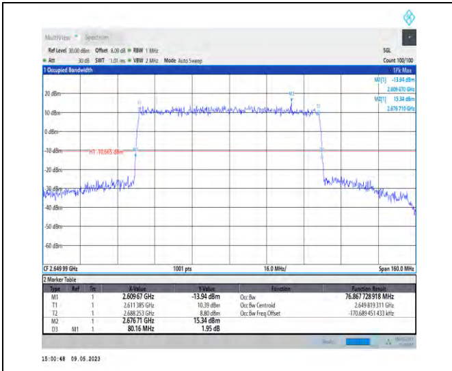
1-N41-PC3-30-80-H-3-DFT-16QAM-Outer_Full-216 @0-76.868-80.160-<80-PASS
