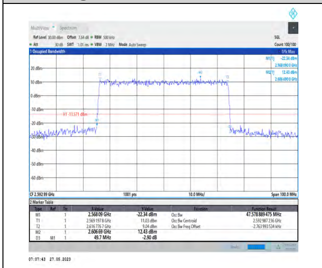
1-N41-PC3-30-50-M-6-CP-QPSK-Outer_Full-133@0 -47.579-49.700-<50-PASS
