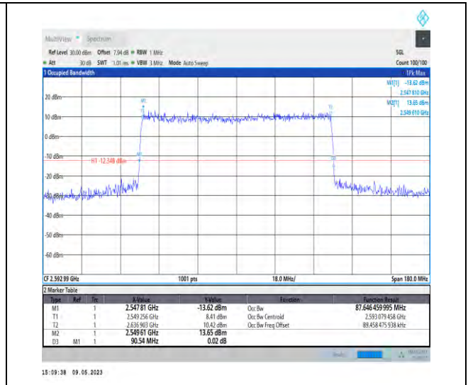
1-N41-PC3-30-90-M-6-CP-QPSK-Outer_Full-245 @0-87.646-90.540-<90-PASS
