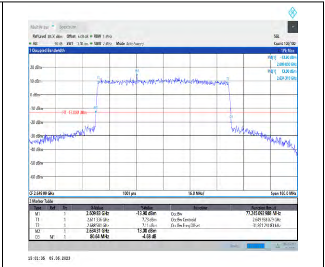
1-N41-PC3-30-80-H-8-CP-64QAM-Outer_Full-217@ 0-77.245-80.640-≤80-PASS
