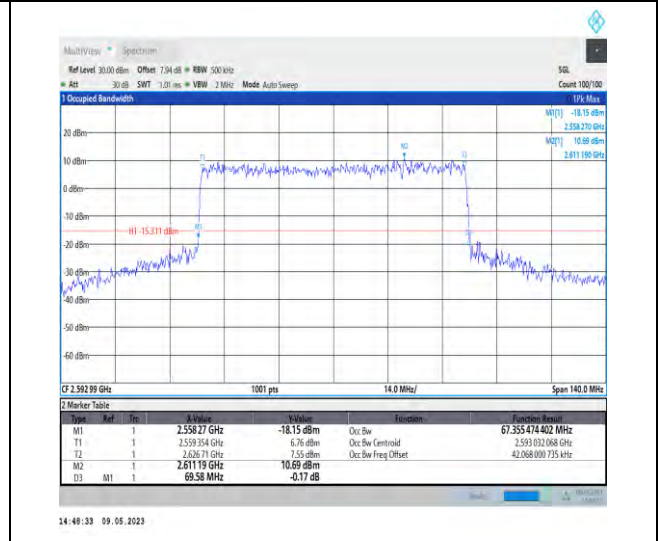
1-N41-PC3-30-70-M-6-CP-QPSK-Outer_Full-189@ 0-67.355-69.580-≤70-PASS
