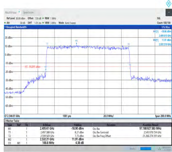
1-N41-PC3-30-100-L-8-CP-64QAM-Outer_Full-273 @0-97.181-100.800-≤100-PASS
