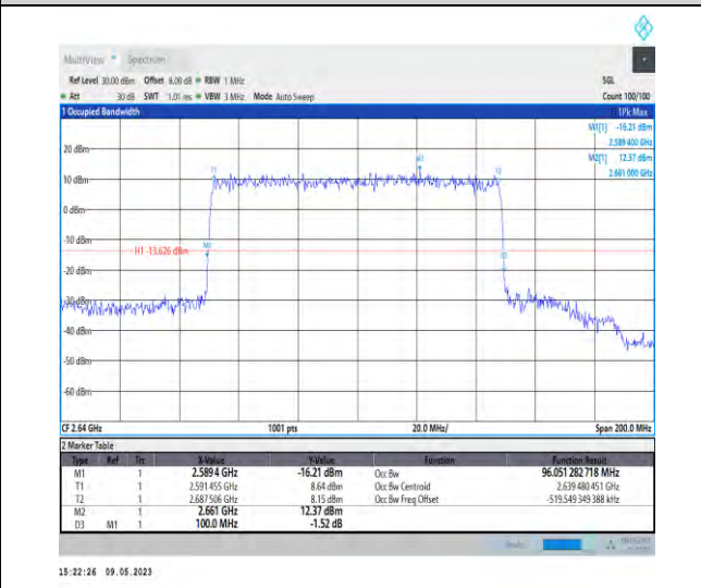
1-N41-PC3-30-100-H-4-DFT-64QAM-Outer_Full-270 @0-96.051-100.000-≤100-PASS
