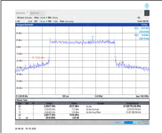
1-N41-PC3-30-70-M-7-CP-16QAM-Outer_Full-189@ 0-67.37-69.440-≤70-PASS
