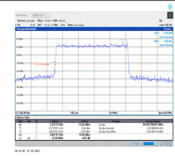
1-N41-PC3-30-40-M-4-DFT-64QAM-Outer_Full-100 @0-35.819-37.440-<40-PASS
