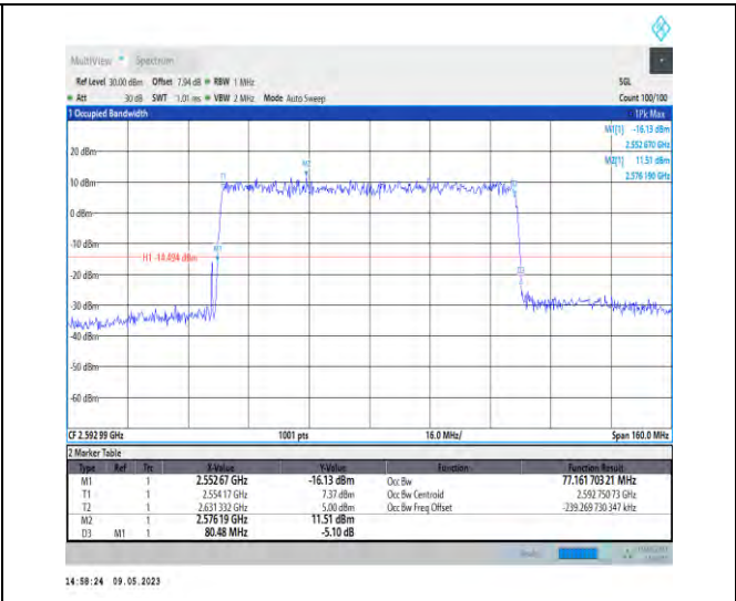
1-N41-PC3-30-80-M-5-DFT-256QAM-Outer_Full-216 @0-77.162-80.480-<80-PASS
