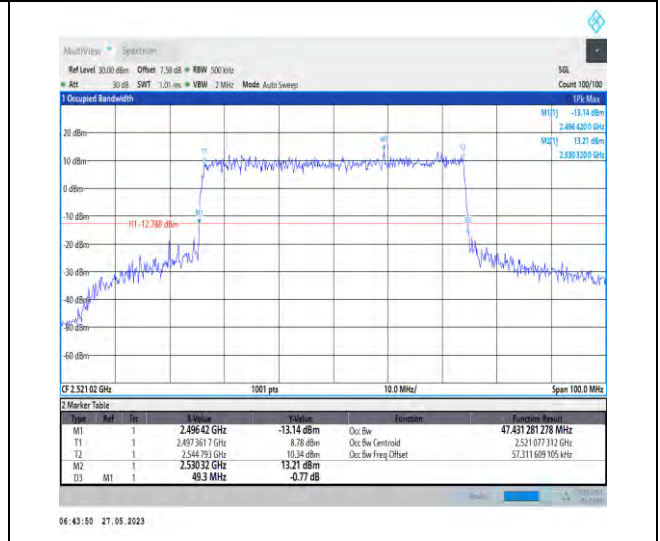
1-N41-PC3-30-50-L-8-CP-64QAM-Outer_Full-133@0 0-47.431-49.300-≤50-PASS
