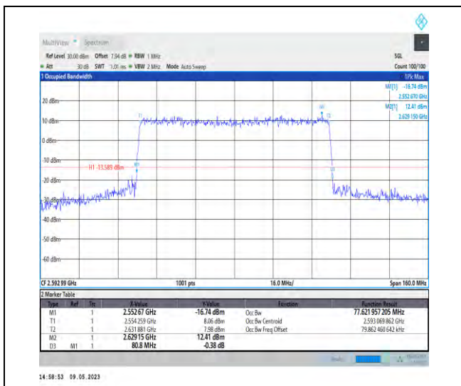
1-N41-PC3-30-80-M-8-CP-64QAM-Outer_Full-217 @0-77.622-80.800-<80-PASS
