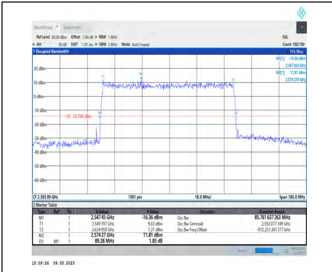
1-N41-PC3-30-90-M-5-DFT-256QAM-Outer_Full-240 @0-85.762-89.280-<90-PASS
