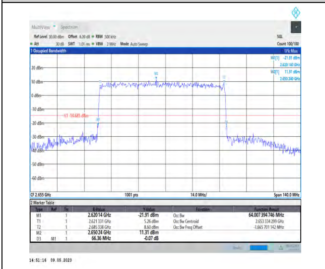
1-N41-PC3-30-70-H-4-DFT-64QAM-Outer_Full-180 @0-64.007-66.360-<=70-PASS
