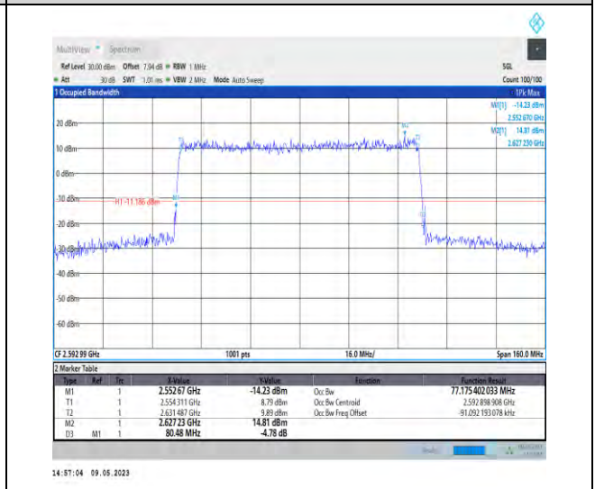
1-N41-PC3-30-80-M-3-DFT-16QAM-Outer_Full-216 @0-77.175-80.480-<80-PASS
