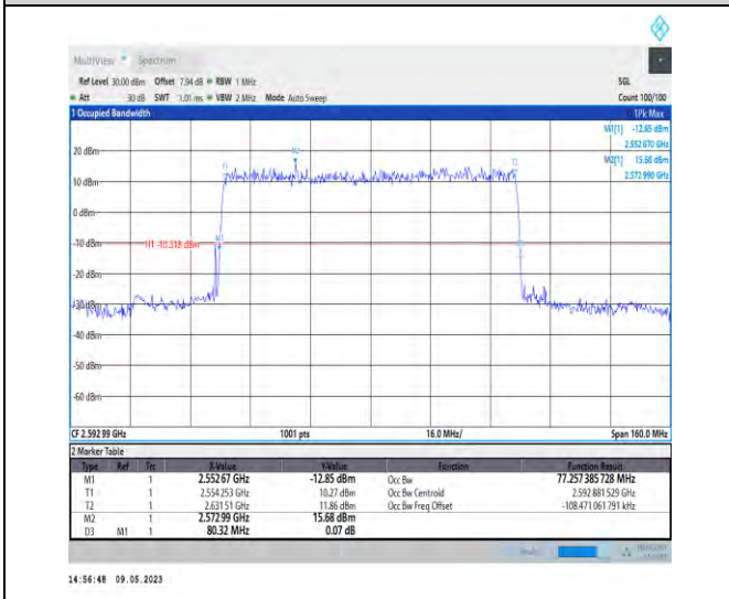
1-N41-PC3-30-80-M-2-DFT-PI2BPSK-Outer_Full-216 @0-77.257-80.320-<80-PASS
