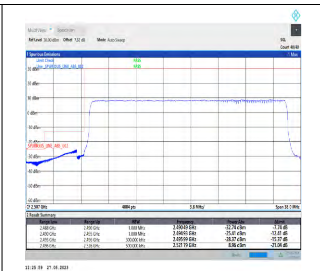
1-N41-PC3-30-30-L-3-DFT-PI2BPSK-Outer_Full-75@0-1--PASS-see graph
