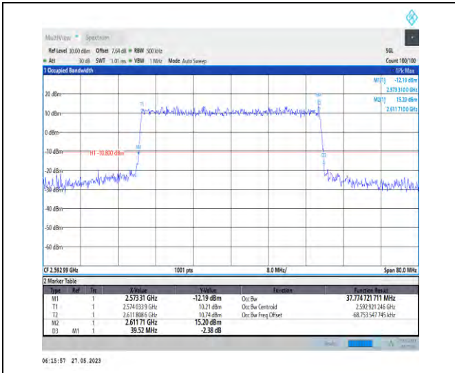
1-N41-PC3-30-40-M-7-CP-16QAM-Outer_Full-106@ @0-37.775-39.520-<40-PASS
