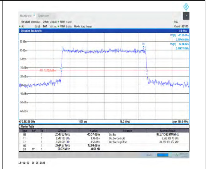
1-N41-PC3-30-90-M-8-CP-64QAM-Outer_Full-245 @0-87.572-90.720-<90-PASS
