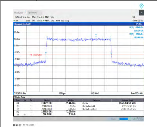
1-N41-PC3-30-100-M-7-CP-16QAM-Outer_Full-273 @0-97.445-100.800-≤100-PASS
