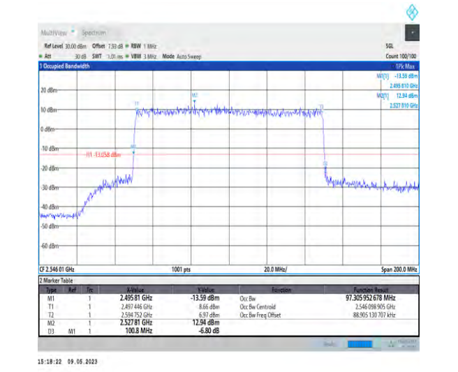
1-N41-PC3-30-100-L-6-CP-QPSK-Outer_Full-273 @0-97.306-100.800-≤100-PASS
