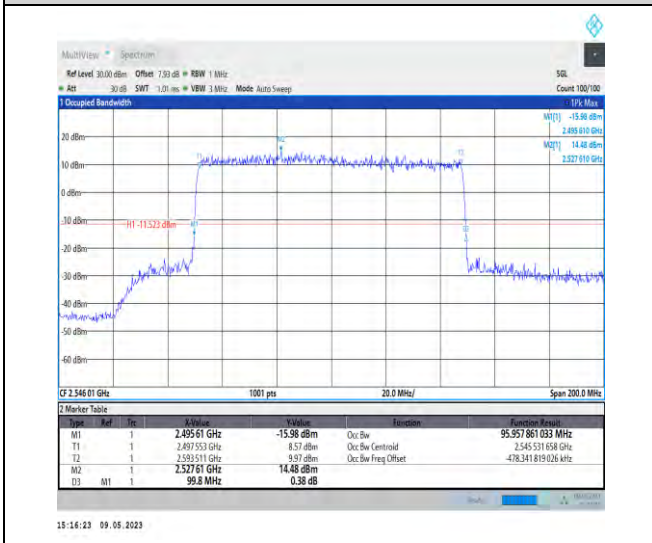
1-N41-PC3-30-100-L-1-DFT-QPSK-Outer_Full-270 @0-95.958-99.800-≤100-PASS
