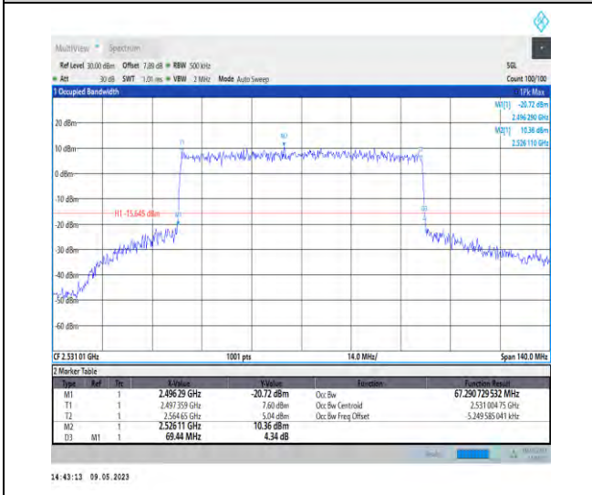
1-N41-PC3-30-70-L-6-CP-QPSK-Outer_Full-189@0 -67.291-69.440-<70-PASS
