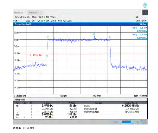
1-N41-PC3-30-70-M-1-DFT-QPSK-Outer_Full-180 @0-64.295-66.500-<=70-PASS
