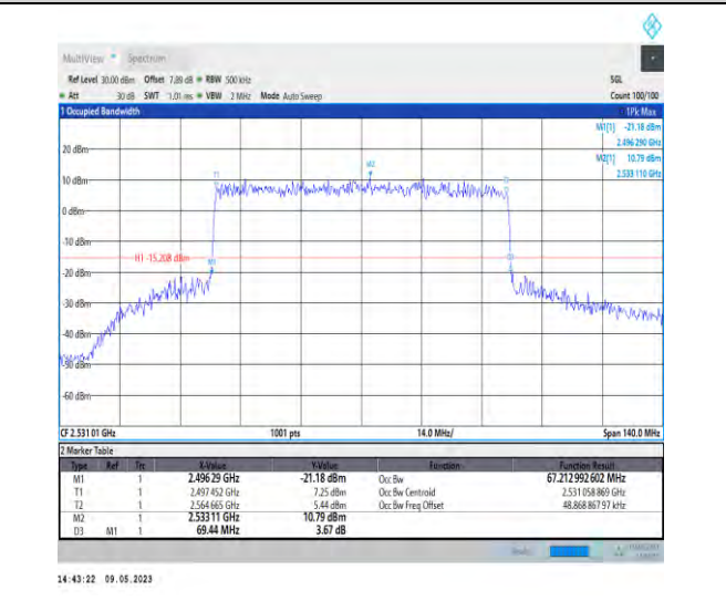
1-N41-PC3-30-70-L-7-CP-16QAM-Outer_Full-189@0 -67.213-69.440-<70-PASS
