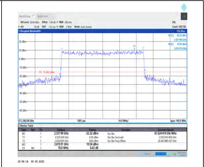
1-N41-PC3-30-70-M-8-CP-64QAM-Outer_Full-189 @0-67.624-70.000-≤70-PASS
