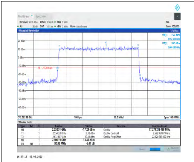
1-N41-PC3-30-80-M-4-DFT-64QAM-Outer_Full-216 @0-77.279-80.960-<80-PASS
