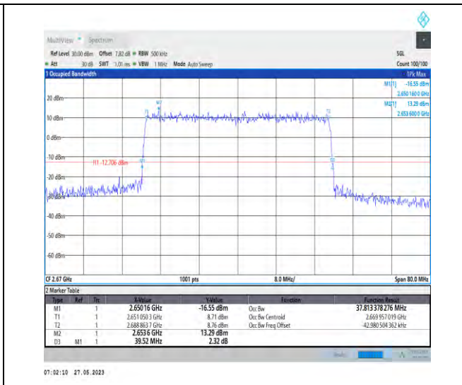
1-N41-PC3-30-40-H-7-CP-16QAM-Outer_Full-106@0 0-37.813-39.520-<40-PASS
