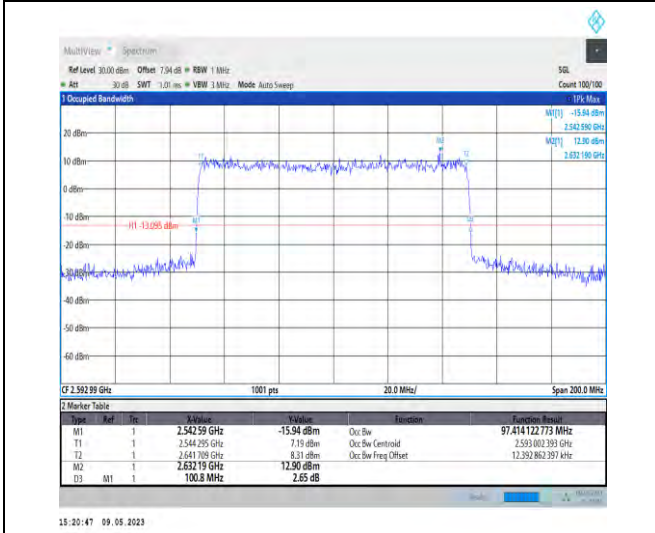
1-N41-PC3-30-100-M-8-CP-64QAM-Outer_Full-273 @0-97.414-100.800-≤100-PASS
