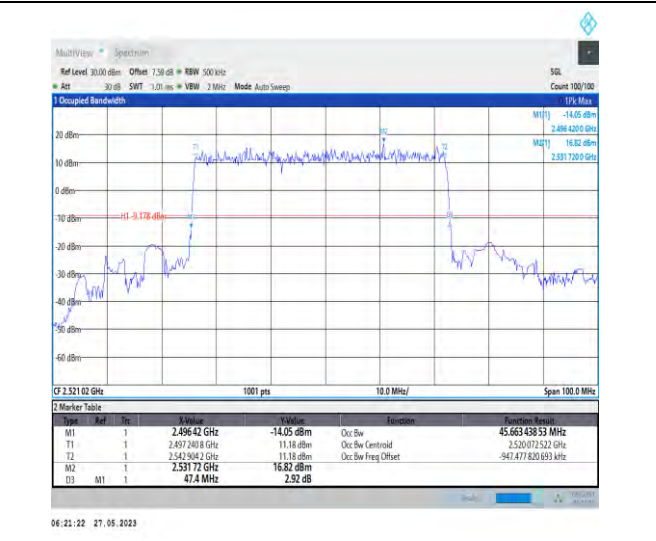
1-N41-PC3-30-50-L-2-DFT-PI2BPSK-Outter_Full-128@ 0-45.663-47.400-≤50-PASS
