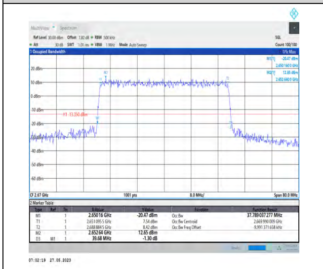
1-N41-PC3-30-40-H-8-CP-64QAM-Outer_Full-106@0 0-37.789-39.680-<40-PASS
