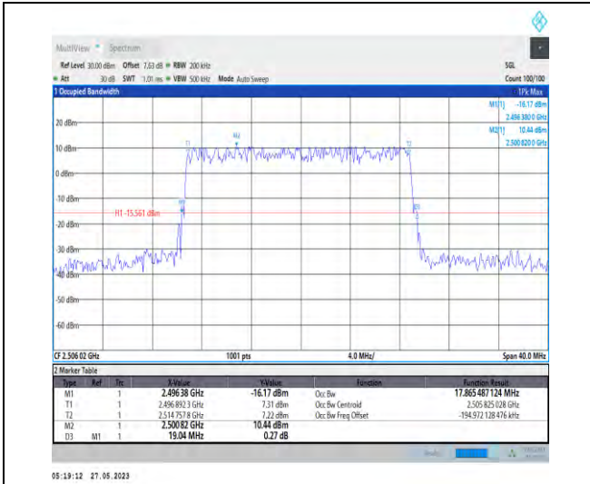
1-N41-PC3-30-20-L-5-DFT-256QAM-Outer_Full-50 @0-17.865-19.040-≤20-PASS
