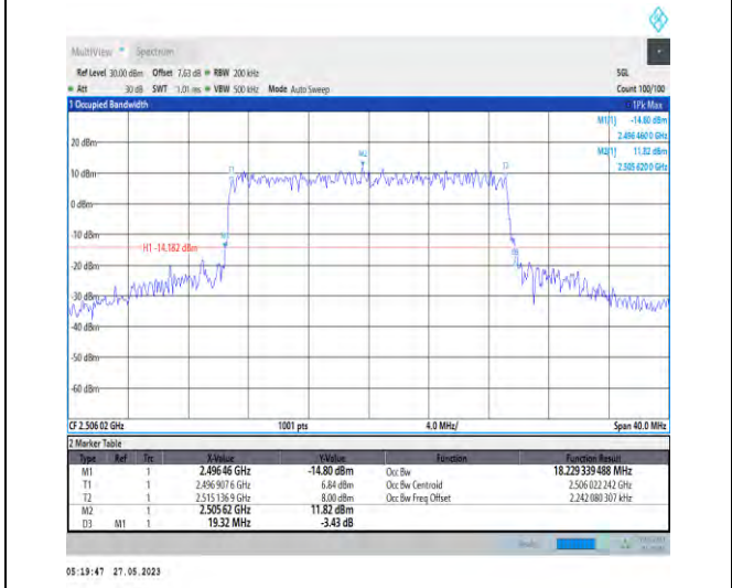
1-N41-PC3-30-20-L-8-CP-64QAM-Outer_Full-51@0- 18.229-19.320-≤20-PASS
