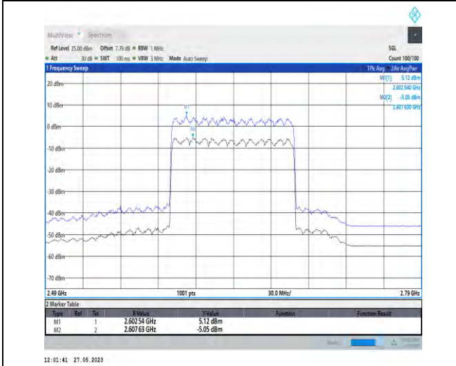
1-N41-PC3-30-100-H-1-DFT-256QAM-Outer_Full-270 @0-10.17-100%-0.00-10.17-PASS-≤13
