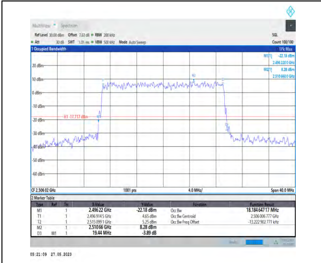
1-N41-PC3-30-20-L-9-CP-256QAM-Outer_Full-51@0 -18.185-19.440-≤20-PASS
