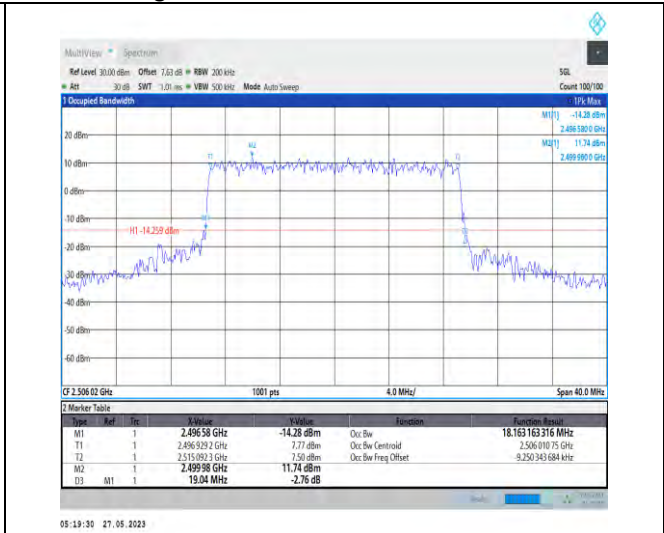
1-N41-PC3-30-20-L-6-CP-QPSK-Outer_Full-51@0-1 8.163-19.040-≤20-PASS
