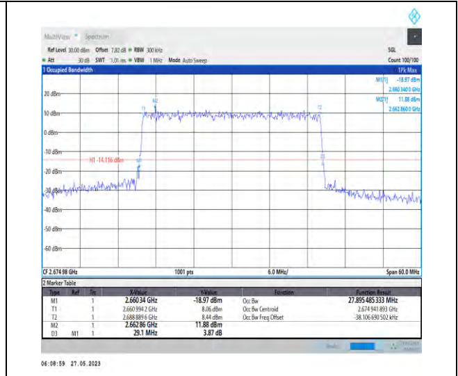
1-N41-PC3-30-30-H-6-CP-QPSK-Outer_Full-78@0-27.895-29.100-≤30-PASS
