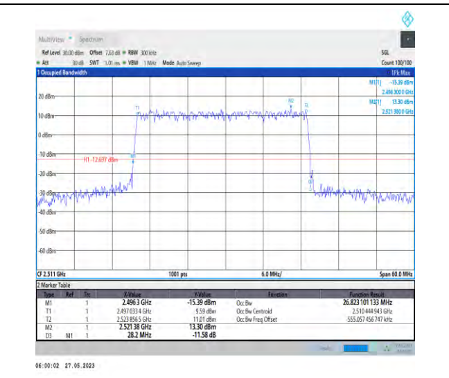
1-N41-PC3-30-30-L-4-DFT-64QAM-Outer_Full-75@0 0-26.823-28.200-≤30-PASS
