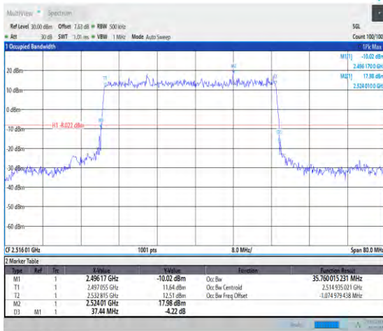
1-N41-PC3-30-40-L-2-DFT-PI2BPSK-Outer_Full-100 @0-35.76-37.440-<40-PASS
