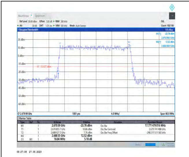
1-N41-PC3-30-20-H-3-DFT-16QAM-Outer_Full-50@ 0-17.771-18.840-<20-PASS
