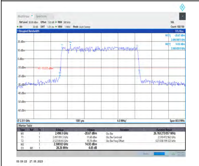
1-N41-PC3-30-30-L-1-DFT-QPSK-Outter_Full-75@0 -26.763-28.260-≤30-PASS
