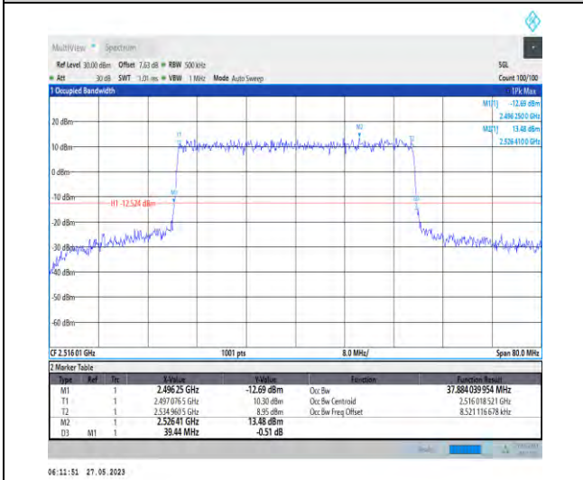
1-N41-PC3-30-40-L-6-CP-QPSK-Outer_Full-106@0 -37.884-39.440-<40-PASS
