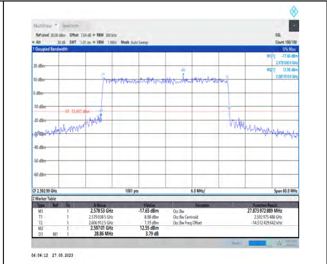
1-N41-PC3-30-30-M-7-CP-16QAM-Outer_Full-78@0-27.874-28.860-≤30-PASS
