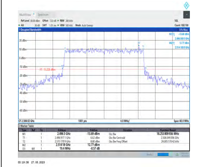
1-N41-PC3-30-20-L-7-CP-16QAM-Outer_Full-51@0- 18.254-19.400-≤20-PASS
