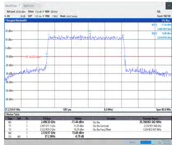
1-N41-PC3-30-40-L-3-DFT-16QAM-Outer_Full-100 @0-35.768-37.200-<40-PASS
