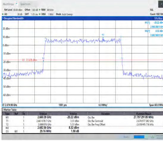
1-N41-PC3-30-30-H-9-CP-256QAM-Outer_Full-78@ 0-27.797-29.160-<30-PASS
