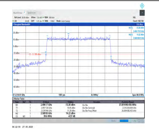
1-N41-PC3-30-40-L-7-CP-16QAM-Outer_Full-106@0 -37.82-39.600-<40-PASS
