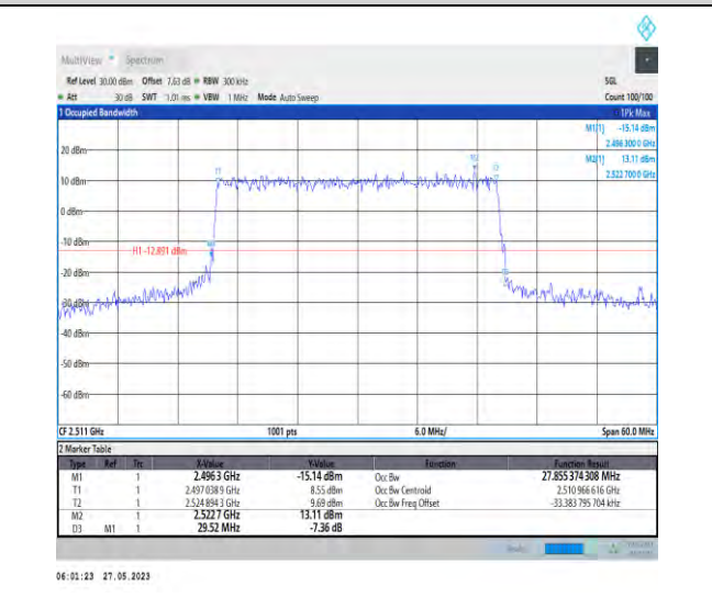
1-N41-PC3-30-30-L-6-CP-QPSK-Outer_Full-78@0- 27.855-29.520-≤30-PASS
