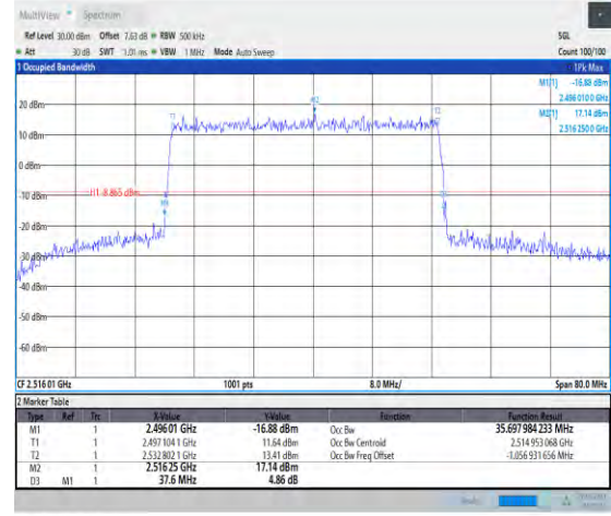
1-N41-PC3-30-40-L-1-DFT-QPSK-Outer_Full-100@ 0-35.698-37.600-<40-PASS
