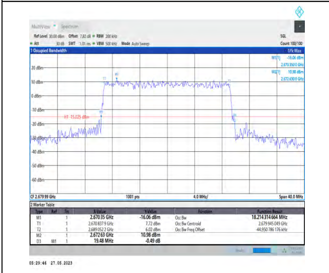
1-N41-PC3-30-20-H-6-CP-QPSK-Outer_Full-51@0- 18.214-19.480-<20-PASS
