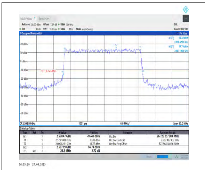
1-N41-PC3-30-30-M-2-DFT-PI2BPSK-Outter_Full-75 @0-26.723-28.200-<=30-PASS
