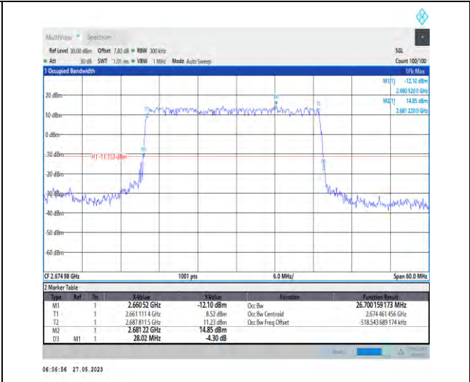
1-N41-PC3-30-30-H-2-DFT-PI2BPSK-Outer_Full-75@0-26.7-28.020-≤30-PASS
