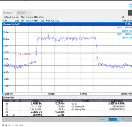
1-N38-PC3-30-30-M-2-DFT-PI2BPSK-Outer_Full-75 @0-26.666-28.080-≤30-PASS
