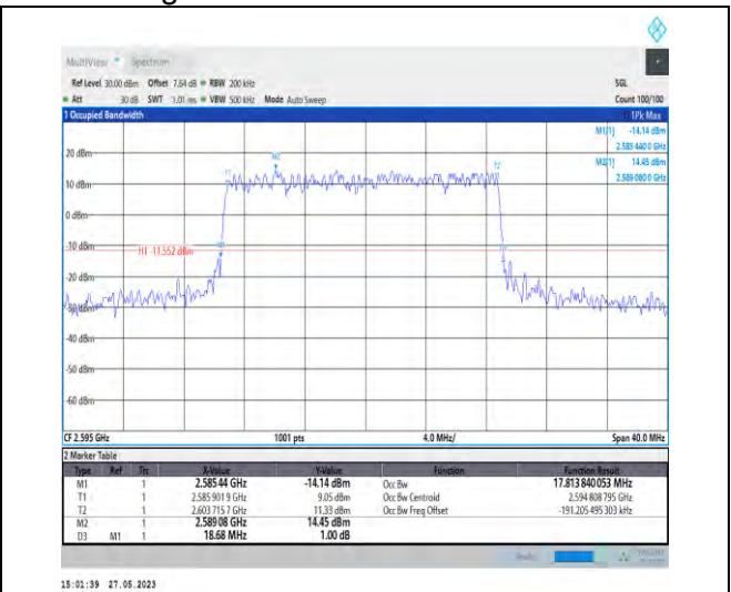
1-N38-PC3-30-20-M-1-DFT-QPSK-Outer_Full-50@ -17.814-18.680-<=20-PASS
