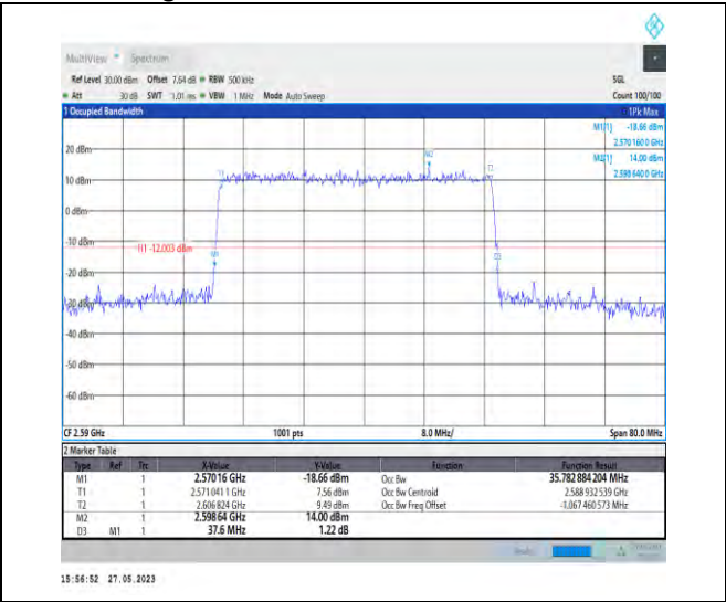
1-N38-PC3-30-40-L-4-DFT-64QAM-Outer_Full-100 @0-35.783-37.600-≤40-PASS
