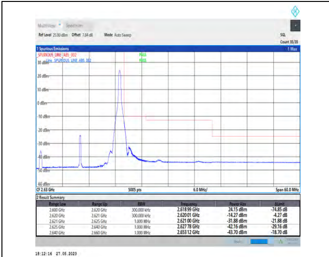
1-N38-PC3-30-20-H-2-DFT-PI2BPSK-Edge_1RB_Right -1@50-1--PASS-see graph
