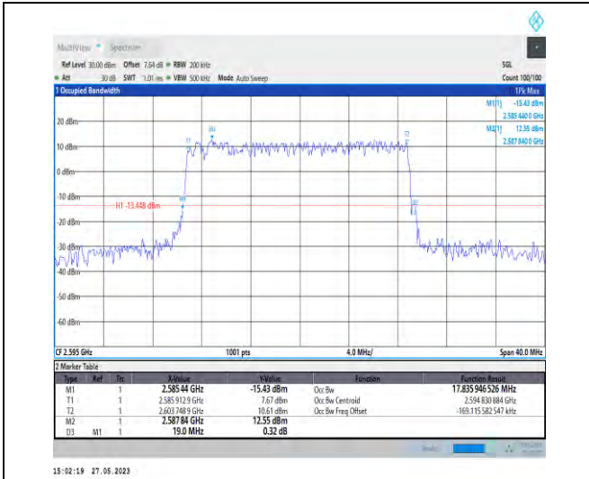
1-N38-PC3-30-20-M-4-DFT-64QAM-Outer_Full-50@ 0-17.836-19.000-≤20-PASS
