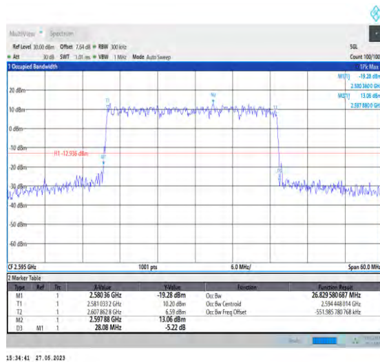
1-N38-PC3-30-30-M-4-DFT-64QAM-Outer_Full-75@ 0-26.83-28.080-≤30-PASS
