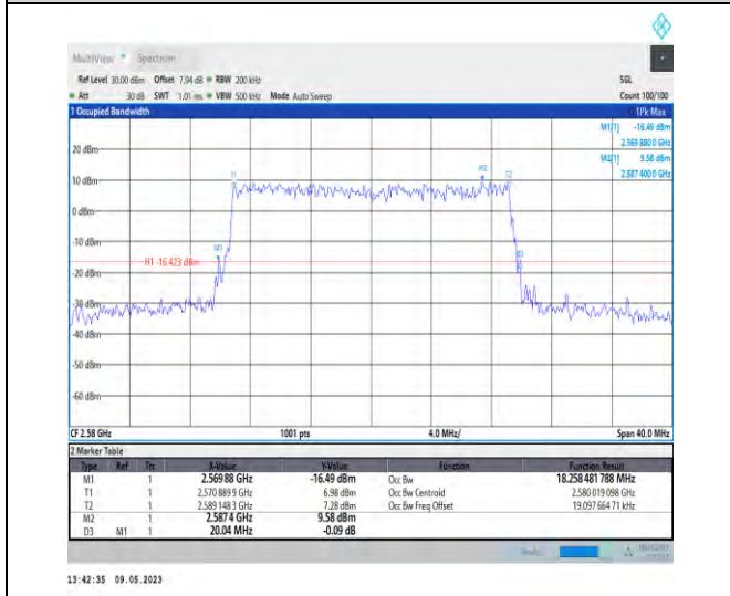
1-N38-PC3-30-20-L-7-CP-16QAM-Outer_Full-51@0- 18.258-20.040-≤20-PASS
