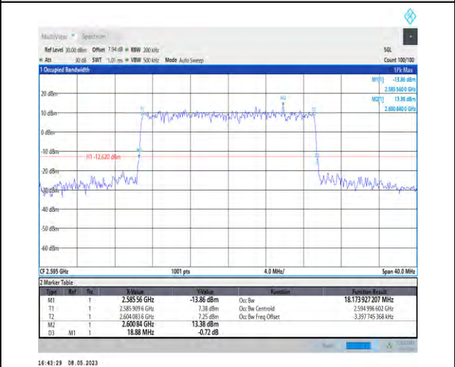
1-N38-PC3-30-20-M-7-CP-16QAM-Outer_Full-51@0- -18.174-18.880-≤20-PASS
