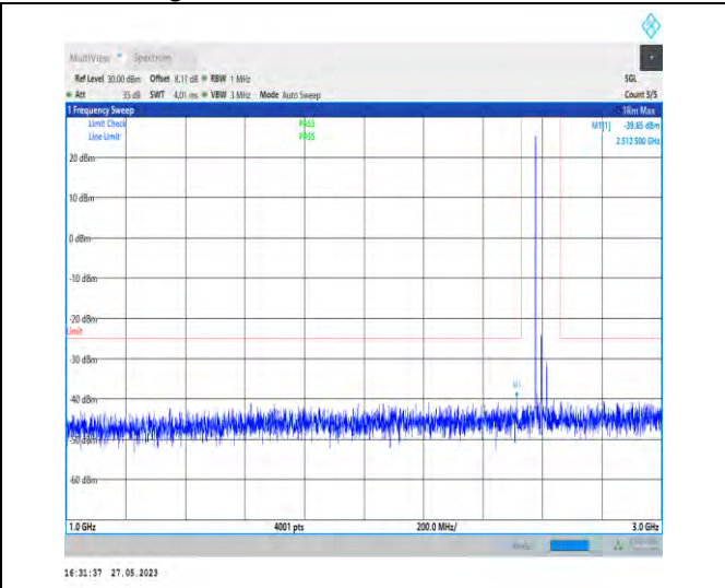
1-N38-PC3-30-40-M-1-N/A-DFT-PI2BPSK-Inner_1RB _Left-1@1-1000-3000-2512.50--39.85--25-PASS
