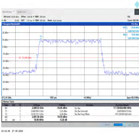
1-N38-PC3-30-20-H-5-DFT-256QAM-Outer_Full-50 @0-17.729-18.960-≤20-PASS
