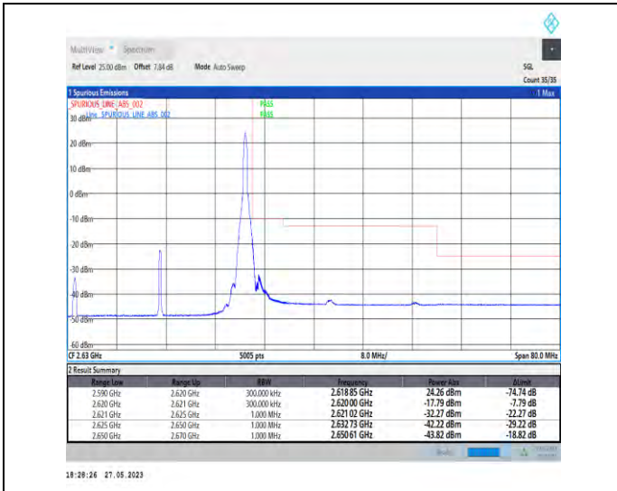
1-N38-PC3-30-30-H-2-DFT-PI2BPSK-Edge_1RB_Right -1@77-1--PASS-see graph
