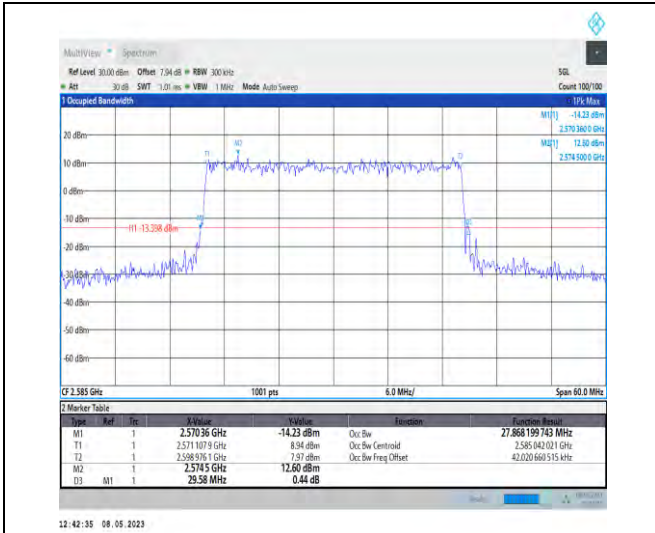
1-N38-PC3-30-30-L-6-CP-QPSK-Outer_Full-78@0-2 7.868-29.580-≤30-PASS
