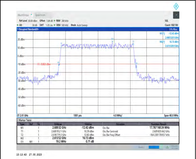
1-N38-PC3-30-20-H-2-DFT-PI2BPSK-Outer_Full-50@0 -17.767-19.200-≤20-PASS
