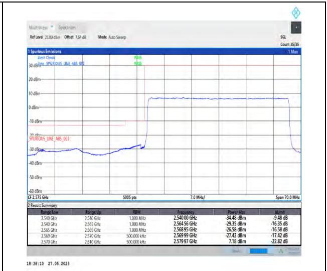
1-N38-PC3-30-40-L-3-DFT-PI2BPSK-Outer_Full-10 0@0-1--PASS-see graph
