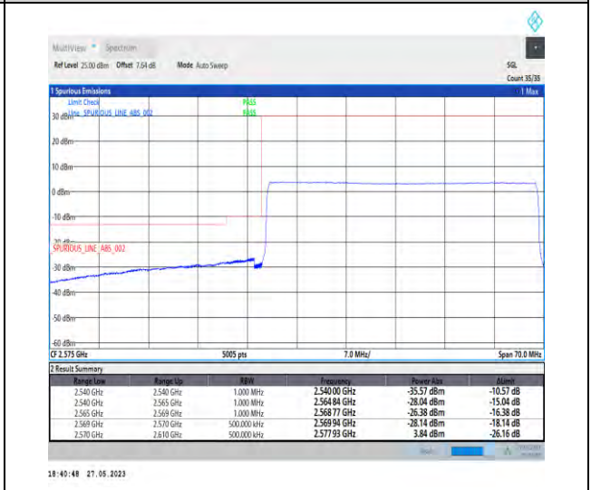
1-N38-PC3-30-40-L-6-CP-QPSK-Outer_Full-106@ 0-1--PASS-see graph
