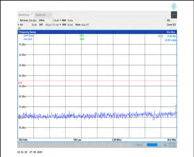
1-N38-PC3-30-40-M-1-N/A-DFT-PI2BPSK-Inner_1RB _Left-1@1-0.15-30-29.76--72.64--45-PASS
