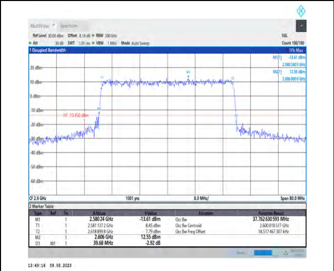
1-N38-PC3-30-40-H-8-CP-64QAM-Outer_Full-106@ 0-37.763-39.680-≤40-PASS
