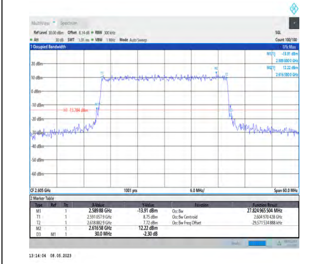
1-N38-PC3-30-30-H-6-CP-QPSK-Outer_Full-78@0-2 7.825-30.000-≤30-PASS
