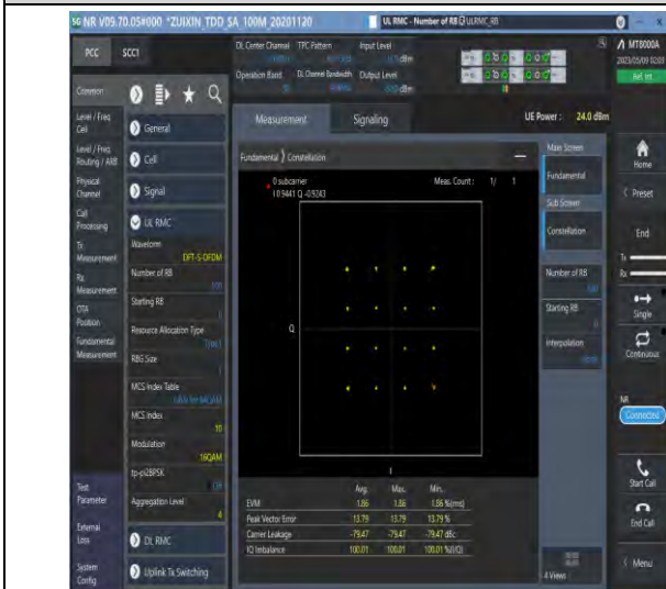
1-N38-PC3-30-40-M-3-DFT-16QAM-Outer_Full-100 @0-see graph-PASS
