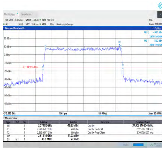
1-N38-PC3-30-40-M-9-CP-256QAM-Outer_Full-106@0 @0-37.904-40.000-≤40-PASS
