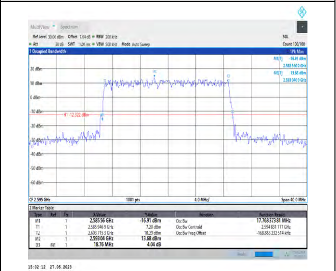
1-N38-PC3-30-20-M-3-DFT-16QAM-Outer_Full-50@ 0-17.768-18.760-<=20-PASS
