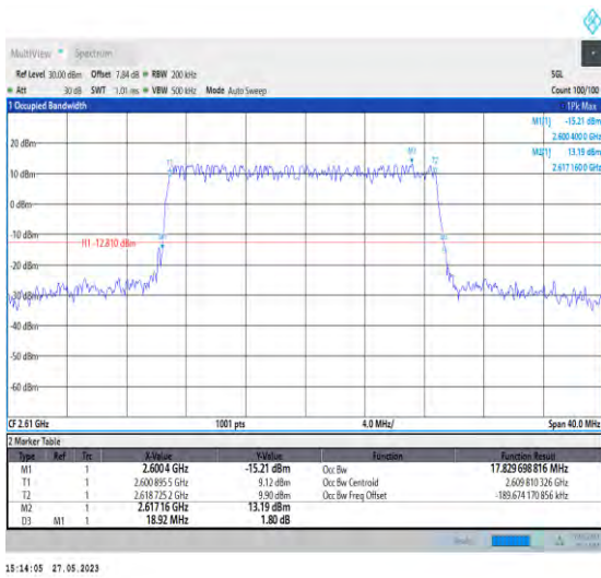
1-N38-PC3-30-20-H-3-DFT-16QAM-Outer_Full-50@ 0-17.83-18.920-≤20-PASS
