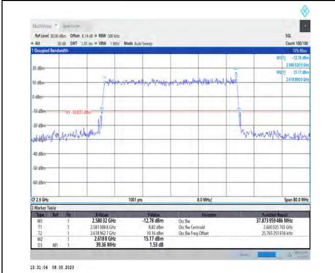
1-N38-PC3-30-40-H-7-CP-16QAM-Outer_Full-106@ 0-37.874-39.360-≤40-PASS
