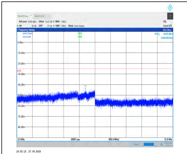
1-N38-PC3-30-40-H-1-N/A-DFT-PI2BPSK-Inner_1R B_Left-1@1-3000-12000-6955.05--44.32--25-PASS
