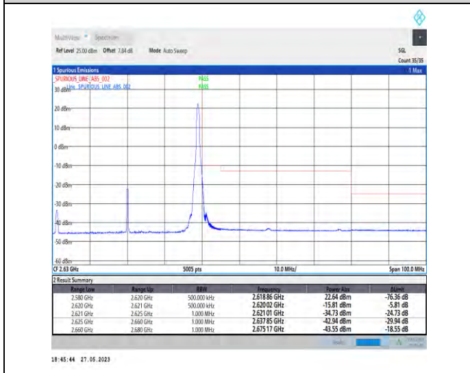
1-N38-PC3-30-40-H-5-CP-QPSK-Edge_1RB_Right-1@ 105-1--PASS-see graph
