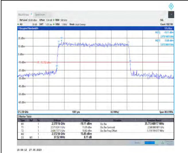
1-N38-PC3-30-40-L-1-DFT-QPSK-Outer_Full-100@0 -35.713-37.520-<math>\leq</math>40-PASS
