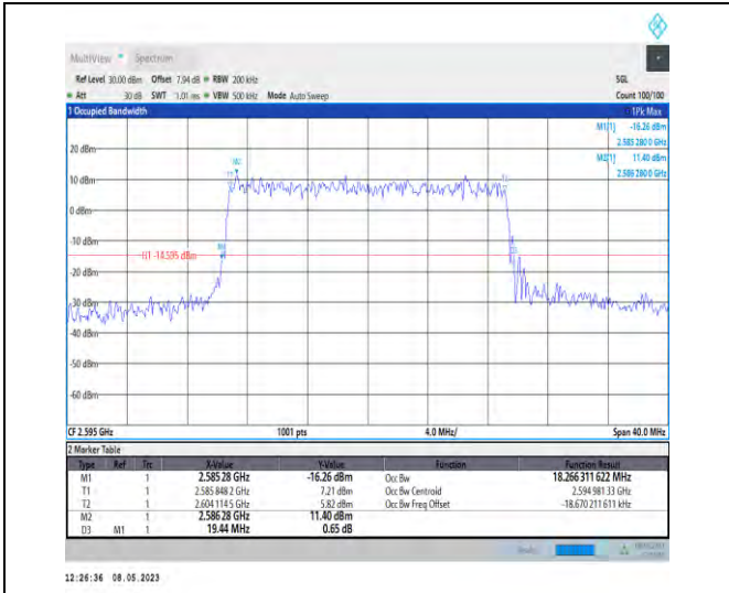
1-N38-PC3-30-20-M-8-CP-64QAM-Outer_Full-51@0 -18.266-19.440-≤20-PASS
