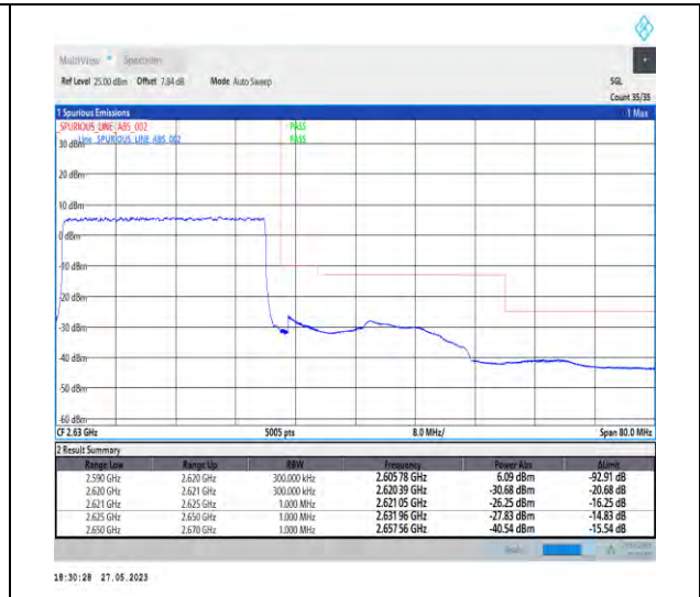
1-N38-PC3-30-30-H-3-DFT-PI2BPSK-Outer_Full-75@0-1--PASS-see graph
