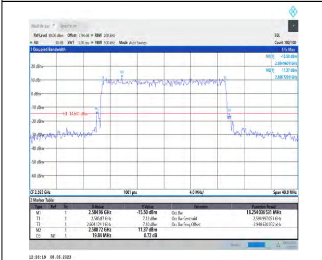
1-N38-PC3-30-20-M-6-CP-QPSK-Outer_Full-51@0- 18.254-19.840-≤20-PASS
