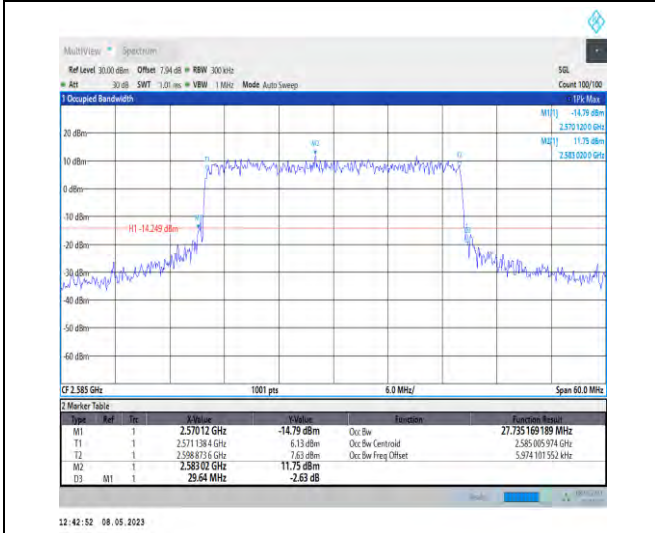
1-N38-PC3-30-30-L-8-CP-64QAM-Outer_Full-78@0- 27.735-29.640-≤30-PASS
