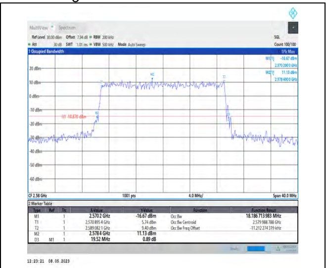
1-N38-PC3-30-20-L-6-CP-QPSK-Outer_Full-51@0-1 8.187-19.520-≤20-PASS
