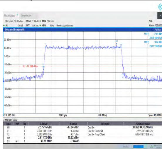
1-N38-PC3-30-40-M-7-CP-16QAM-Outer_Full-106@0 0-37.829-39.760-≤40-PASS
