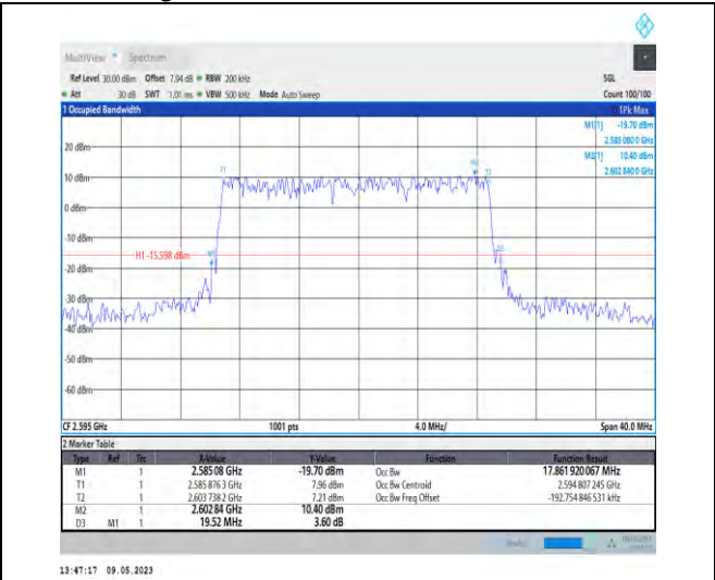
1-N38-PC3-30-20-M-5-DFT-256QAM-Outer_Full-50@ @0-17.862-19.520-≤20-PASS
