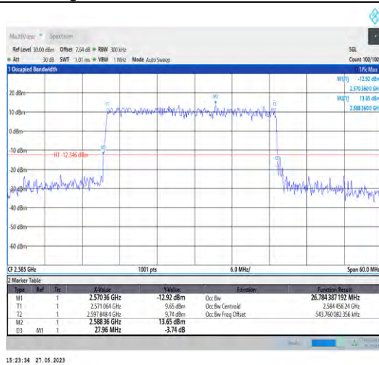
1-N38-PC3-30-30-L-3-DFT-16QAM-Outer_Full-75@ 0-26.784-27.960-≤30-PASS
