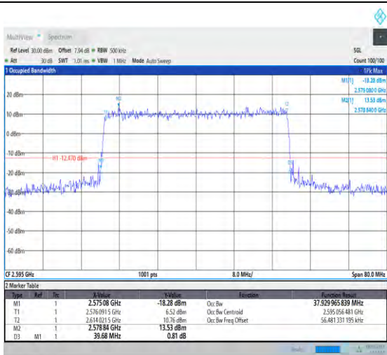
1-N38-PC3-30-40-M-6-CP-QPSK-Outer_Full-106@0 -37.93-39.680-≤40-PASS
