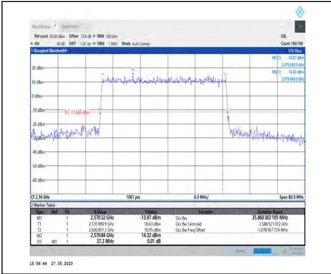
1-N38-PC3-30-40-L-3-DFT-16QAM-Outer_Full-100 @0-35.86-37.200-≤40-PASS
