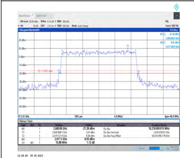
1-N38-PC3-30-20-H-9-CP-256QAM-Outer_Full-51@0 0-18.219-19.880-≤20-PASS
