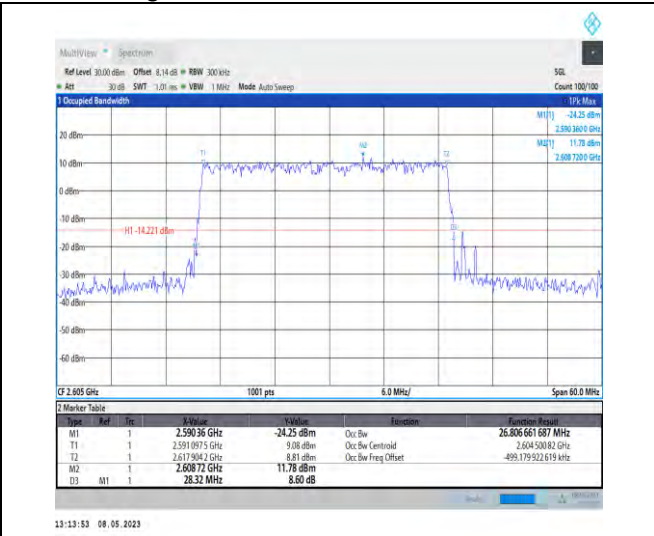
1-N38-PC3-30-30-H-5-DFT-256QAM-Outer_Full-75 @0-26.807-28.320-≤30-PASS
