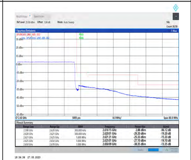
1-N38-PC3-30-30-H-6-CP-QPSK-Outer_Full-78@0-1--PASS-see graph
