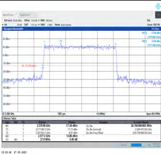
1-N38-PC3-30-30-L-4-DFT-64QAM-Outer_Full-75@ 0-26.766-27.900-≤30-PASS
