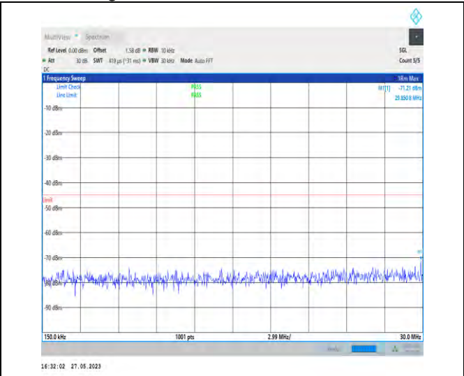
1-N38-PC3-30-40-H-1-N/A-DFT-PI2BPSK-Inner_1RB _Left-1@1-0.15-30-29.85--71.21--45-PASS
