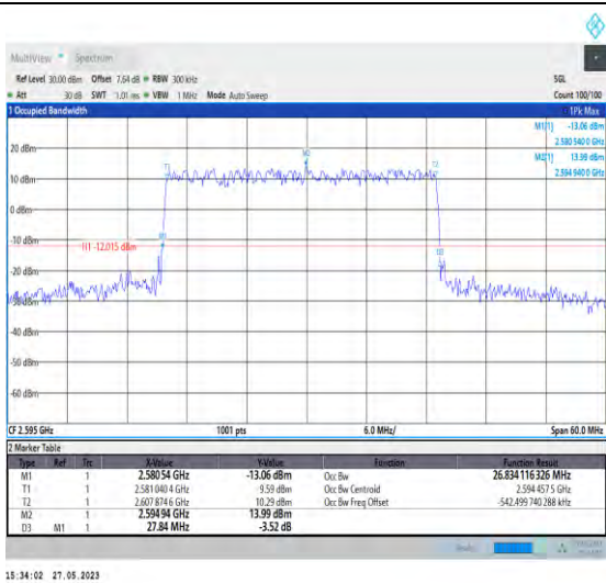
1-N38-PC3-30-30-M-1-DFT-QPSK-Outer_Full-75@0 -26.834-27.840-≤30-PASS
