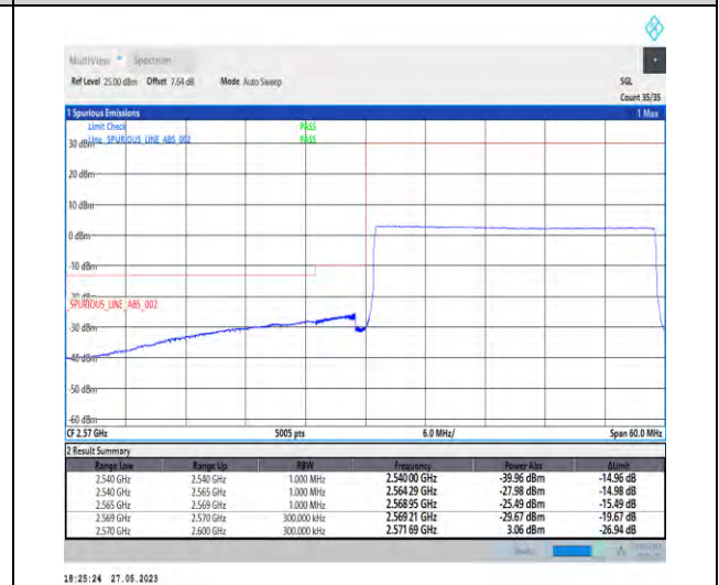
1-N38-PC3-30-30-L-6-CP-QPSK-Outer_Full-78@0-1--PASS-see graph
