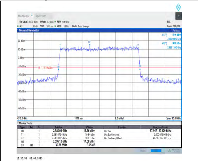
1-N38-PC3-30-40-H-6-CP-QPSK-Outer_Full-106@ -37.947-39.760-≤40-PASS
