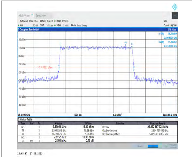
1-N38-PC3-30-30-H-4-DFT-64QAM-Outer_Full-75@ 0-26.822-28.080-≤30-PASS
