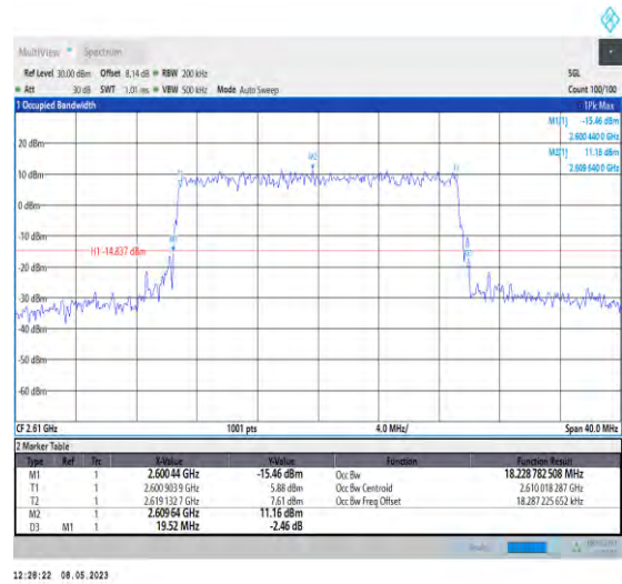
1-N38-PC3-30-20-H-6-CP-QPSK-Outer_Full-51@0- 18.229-19.520-≤20-PASS
