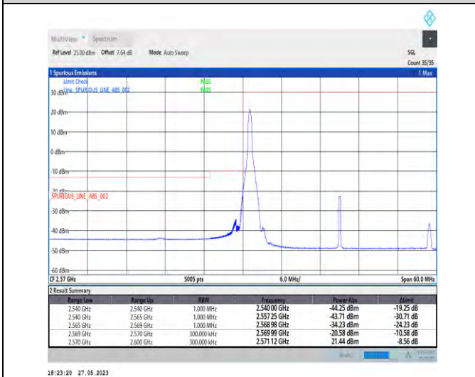
1-N38-PC3-30-30-L-4-CP-QPSK-Edge_1RB_Left-1@0-1--PASS-see graph
