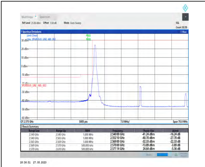
1-N38-PC3-30-40-L-1-DFT-PI2BPSK-Edge_1RB_Left -1@0-1--PASS-see graph
