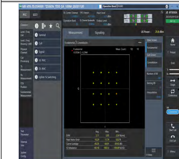
1-N38-PC3-30-40-M-7-CP-16QAM-Outer_Full-106@0-see graph-PASS
