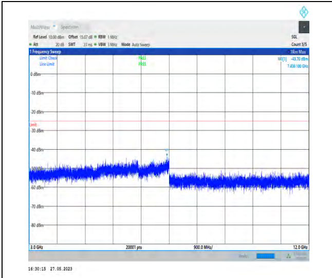
1-N38-PC3-30-40-L-1-N/A-DFT-PI2BPSK-Inner_1R B_Left-1@1-3000-12000-7436.10--43.70--25-PASS
