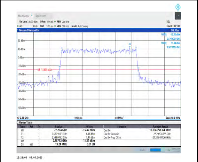
1-N38-PC3-30-20-L-8-CP-64QAM-Outer_Full-51@0- 18.135-19.240-≤20-PASS
