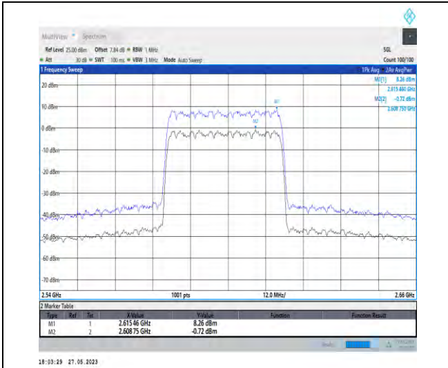
1-N38-PC3-30-40-H-1-DFT-256QAM-Outer_Full-100 @0-8.98-100%-0.00-8.98-PASS-≤13
