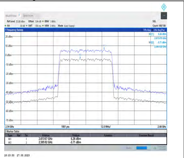
1-N38-PC3-30-40-H-2-CP-256QAM-Outer_Full-106 @0-9.97-100%-0.00-9.97-PASS-≤13
