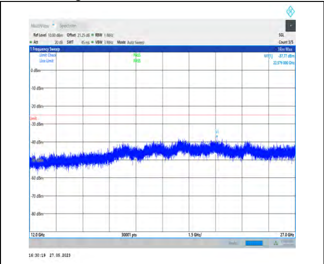
1-N38-PC3-30-40-L-1-N/A-DFT-PI2BPSK-Inner_1RB _Left-1@1-12000-27000-22579.00--37.77--25-PASS
