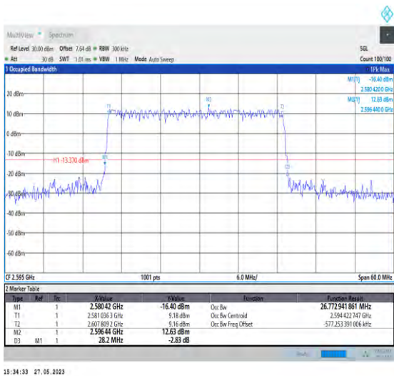
1-N38-PC3-30-30-M-3-DFT-16QAM-Outer_Full-75@ 0-26.773-28.200-≤30-PASS
