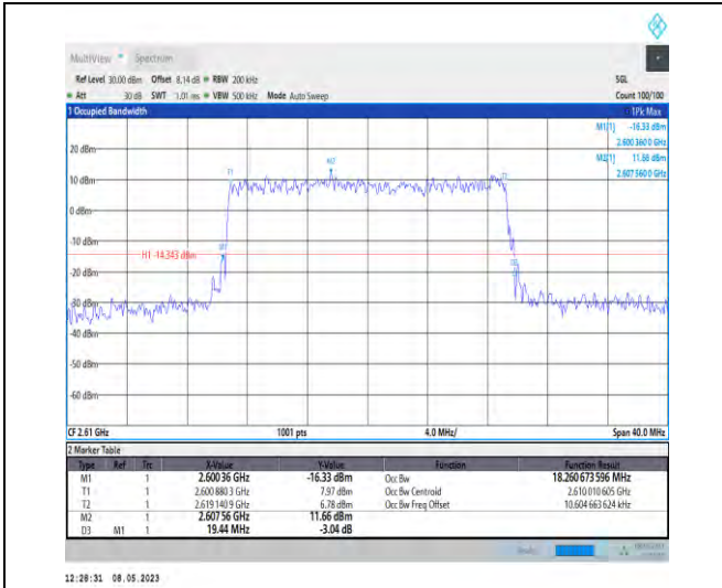
1-N38-PC3-30-20-H-7-CP-16QAM-Outer_Full-51@0 -18.261-19.440-≤20-PASS
