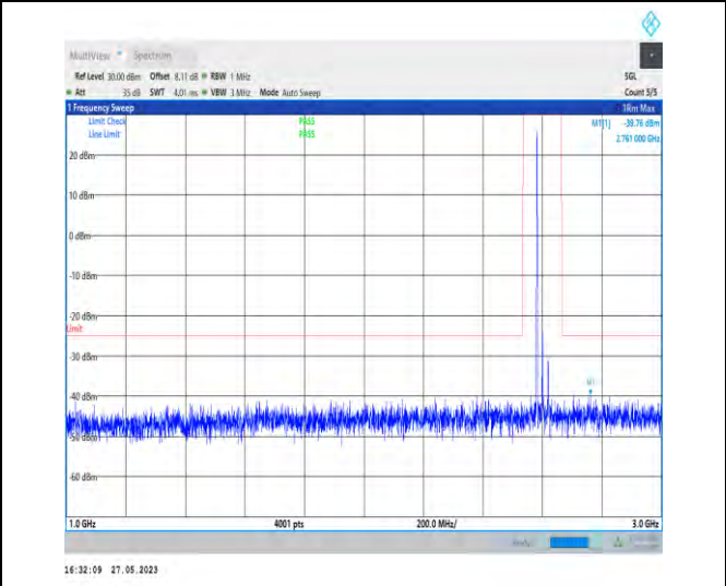
1-N38-PC3-30-40-H-1-N/A-DFT-PI2BPSK-Inner_1RB _Left-1@1-1000-3000-2761.00--39.76--25-PASS
