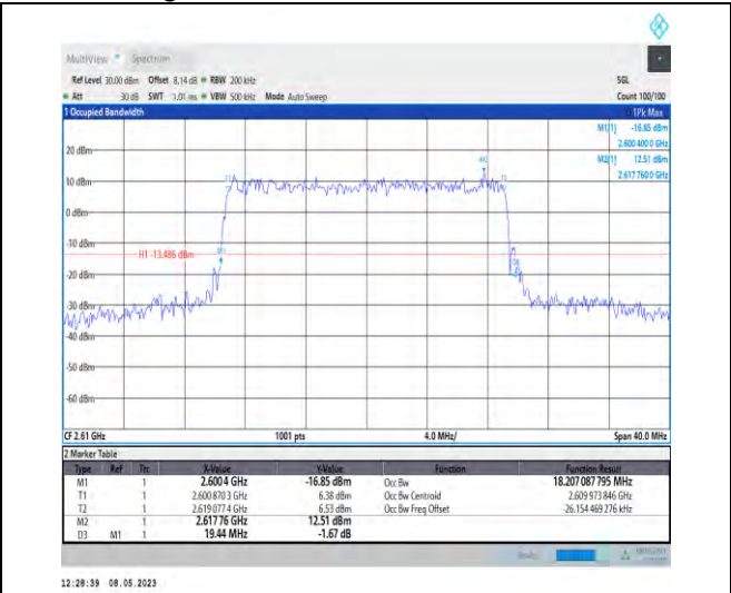
1-N38-PC3-30-20-H-8-CP-64QAM-Outer_Full-51@0 -18.207-19.440-≤20-PASS
