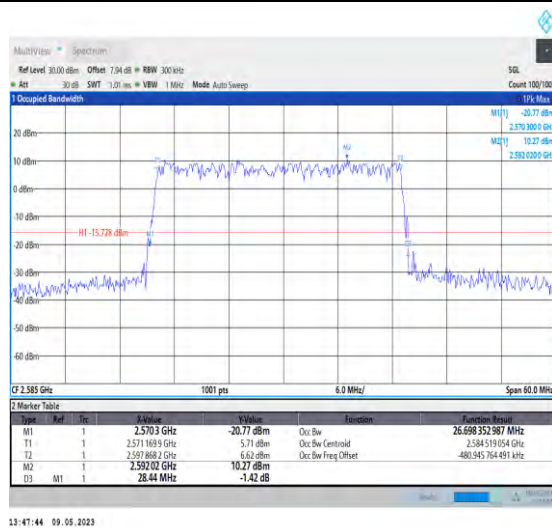
1-N38-PC3-30-30-L-5-DFT-256QAM-Outer_Full-75 @0-26.698-28.440-≤30-PASS
