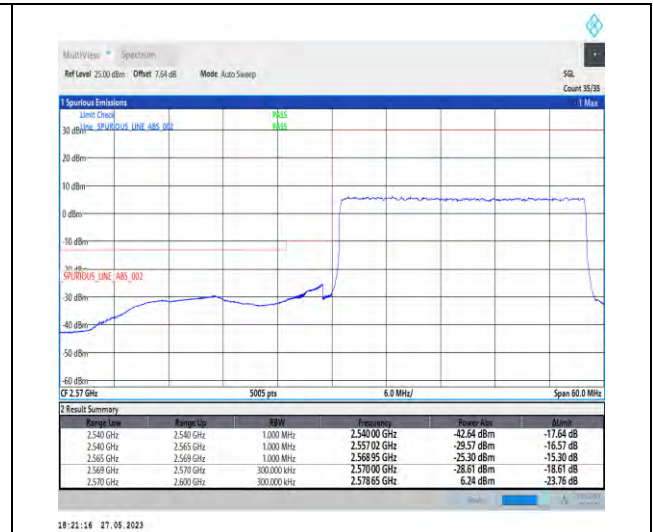
1-N38-PC3-30-30-L-3-DFT-PI2BPSK-Outer_Full-75@0-1--PASS-see graph
