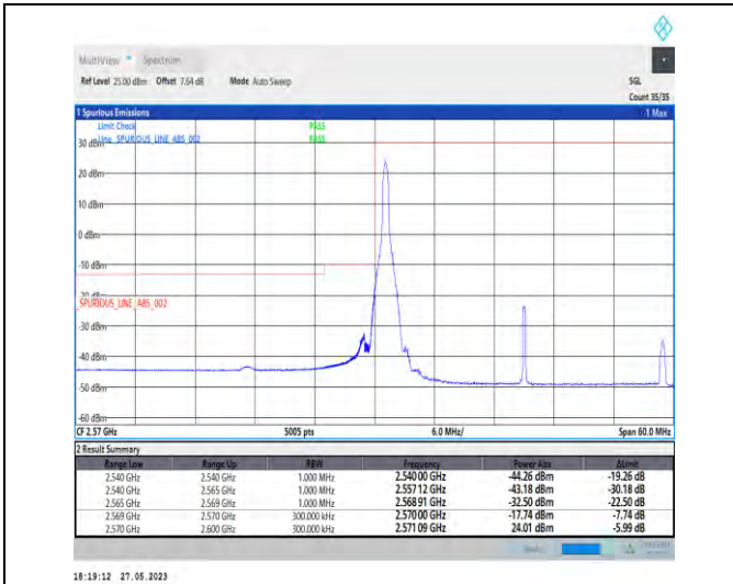
1-N38-PC3-30-30-L-1-DFT-PI2BPSK-Edge_1RB_Left-1@0-1--PASS-see graph
