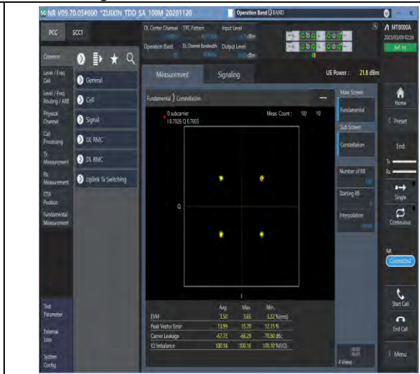
1-N38-PC3-30-40-M-6-CP-QPSK-Outer_Full-106@0-see graph-PASS
