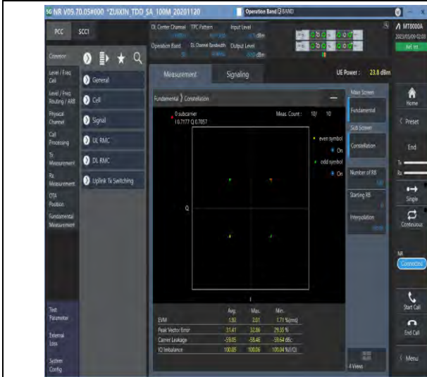
1-N38-PC3-30-40-M-1-DFT-PI2BPSK-Outer_Full-100 @0-see graph-PASS
