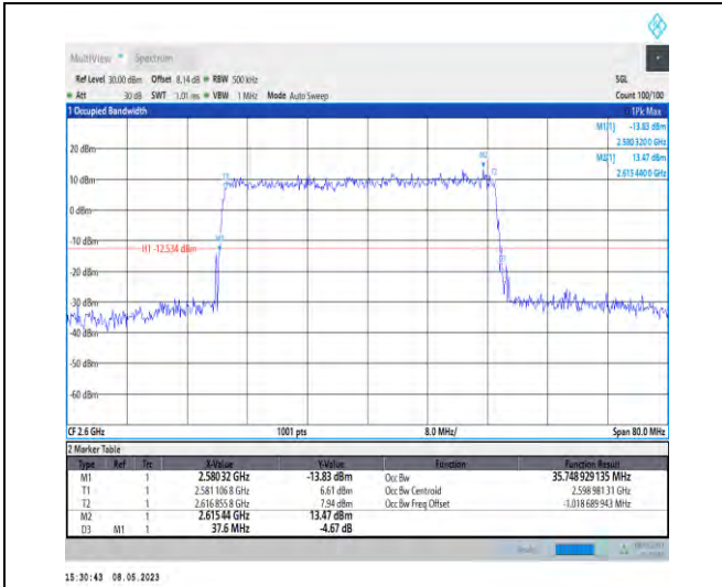
1-N38-PC3-30-40-H-5-DFT-256QAM-Outer_Full-100 @0-35.749-37.600-≤40-PASS
