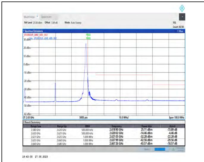
1-N38-PC3-30-40-H-2-DFT-PI2BPSK-Edge_1RB_Right -1@105-1--PASS-see graph
