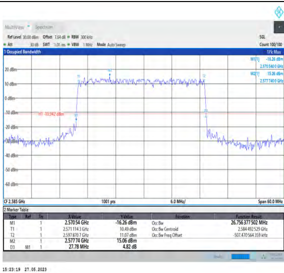
1-N38-PC3-30-30-L-2-DFT-PI2BPSK-Outer_Full-75 @0-26.756-27.780-≤30-PASS
