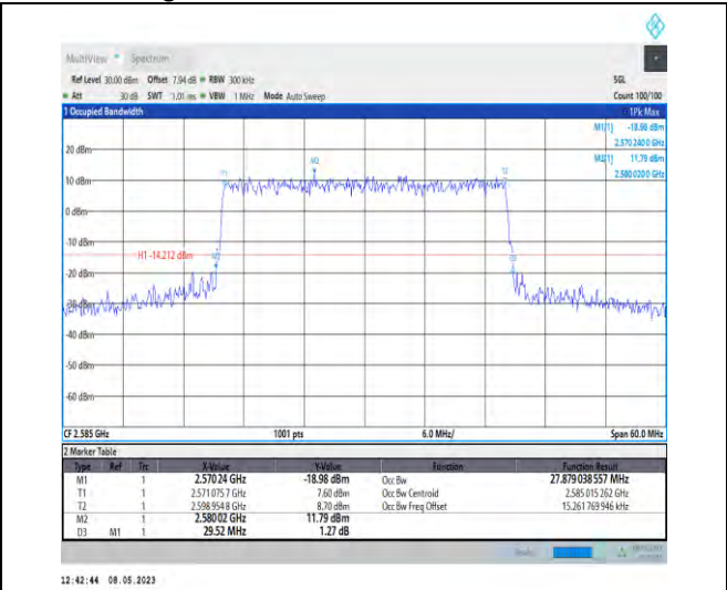
1-N38-PC3-30-30-L-7-CP-16QAM-Outer_Full-78@0- 27.879-29.520-≤30-PASS
