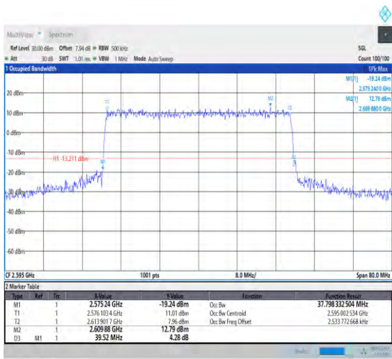
1-N38-PC3-30-40-M-8-CP-64QAM-Outer_Full-106@0 0-37.798-39.520-≤40-PASS
