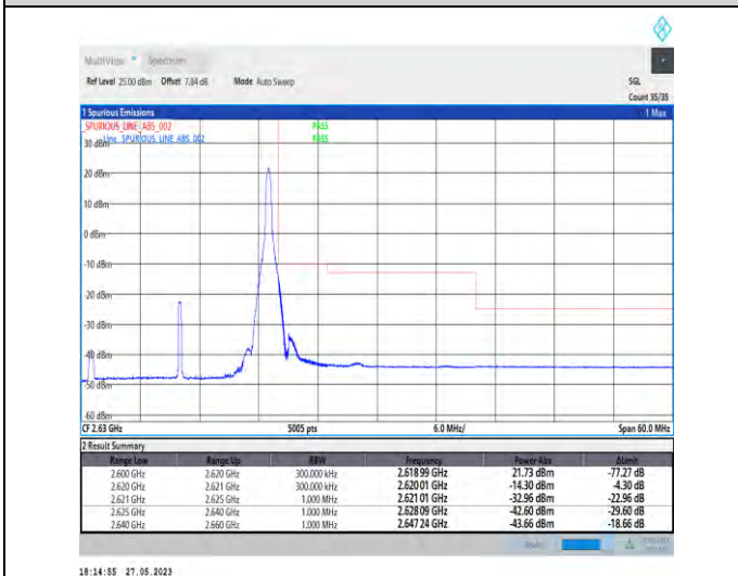
1-N38-PC3-30-20-H-5-CP-QPSK-Edge_1RB_Right-1@50-1--PASS-see graph
