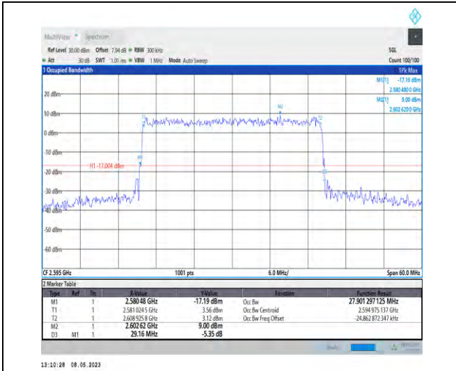
1-N38-PC3-30-30-M-9-CP-256QAM-Outer_Full-78@ 0-27.901-29.160-≤30-PASS
