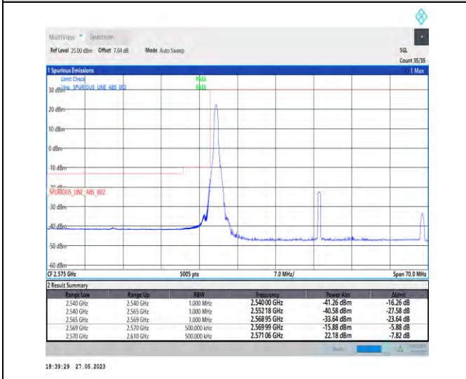
1-N38-PC3-30-40-L-4-CP-QPSK-Edge_1RB_Left-1@ 0-1--PASS-see graph
