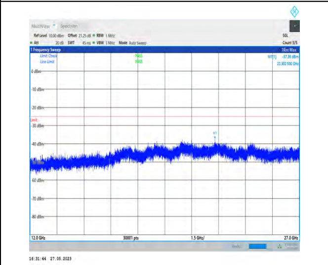
1-N38-PC3-30-40-M-1-N/A-DFT-PI2BPSK-Inner_1RB _Left-1@1-12000-27000-22302.50--37.39--25-PASS
