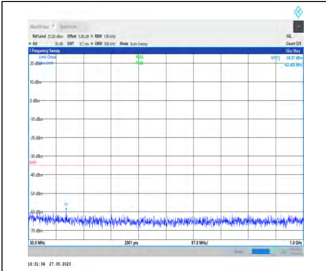
1-N38-PC3-30-40-M-1-N/A-DFT-PI2BPSK-Inner_1R B_Left-1@1-30-1000-162.41--59.37--35-PASS
