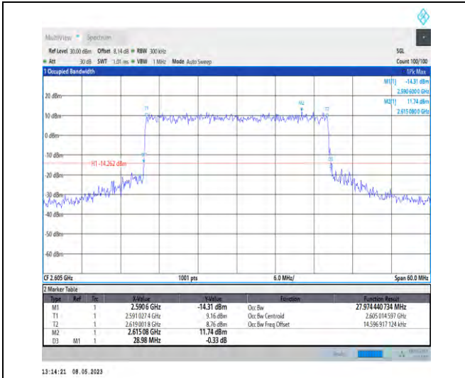
1-N38-PC3-30-30-H-8-CP-64QAM-Outer_Full-78@0 -27.974-28.980-<math>\leq</math>30-PASS
