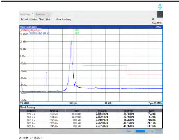
1-N38-PC3-30-30-H-5-CP-QPSK-Edge_1RB_Right-1@77-1--PASS-see graph
