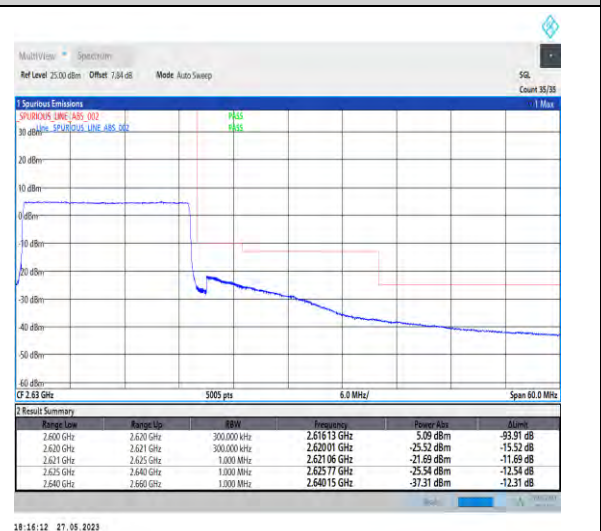
1-N38-PC3-30-20-H-6-CP-QPSK-Outer_Full-51@0-1--PASS-see graph
