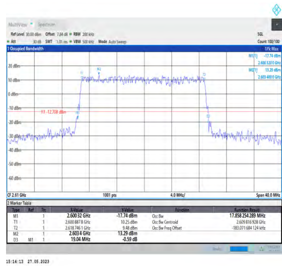
1-N38-PC3-30-20-H-4-DFT-64QAM-Outer_Full-50@ 0-17.858-19.040-≤20-PASS
