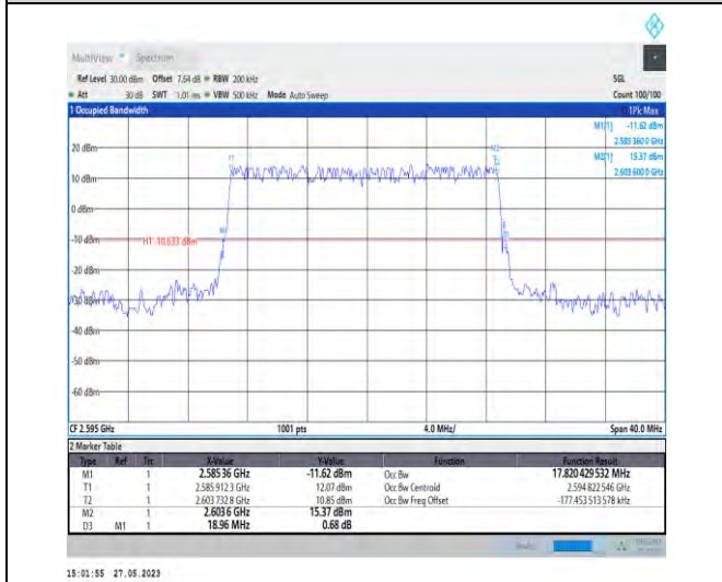
1-N38-PC3-30-20-M-2-DFT-PI2BPSK-Outer_Full-50 @0-17.82-18.960-<=20-PASS
