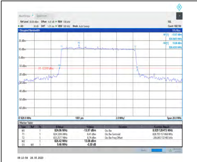
1-N26-824-849-PC3-15-10-L-3-DFT-16QAM-Outer_Full-50@0-8.929-9.460-≤10-PASS
