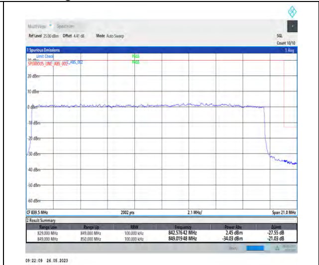
1-N26-824-849-PC3-15-20-H-3-DFT-PI2BPSK-Out_er_Full-100@0-1-seegraph-PASS-see graph
