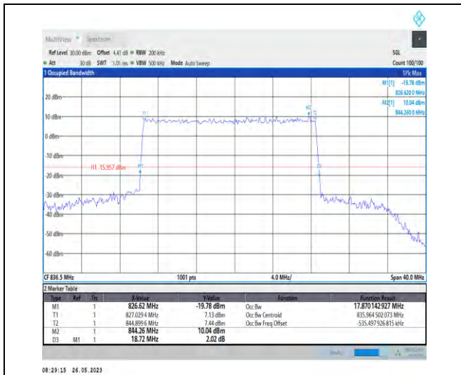
1-N26-824-849-PC3-15-20-M-5-DFT-256QAM-Outer_Full-100@0-17.87-18.720-≤20-PASS
