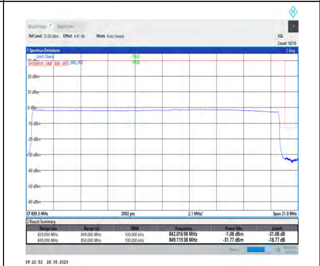
1-N26-824-849-PC3-15-20-H-6-CP-QPSK-Outer_Full-106@0-1-seegraph-PASS-see graph
