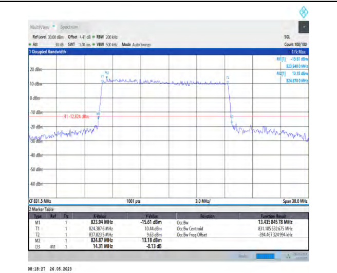
1-N26-824-849-PC3-15-15-L-4-DFT-64QAM-Outer_Full-75@0-13.436-14.310-≤15-PASS
