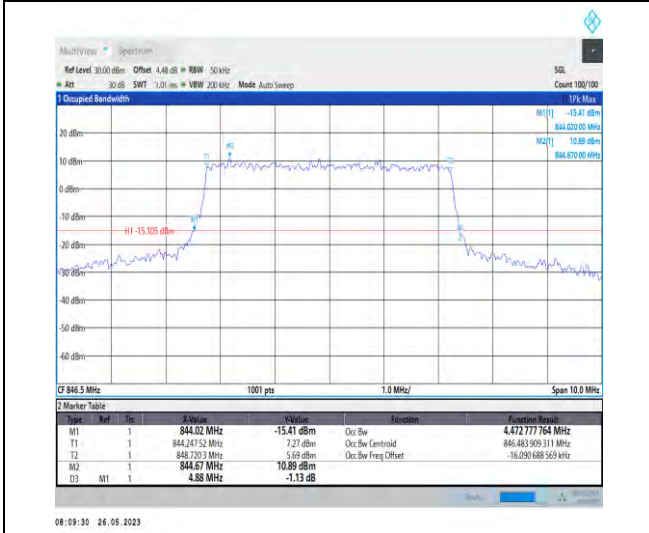
1-N26-824-849-PC3-15-5-H-6-CP-QPSK-Outer_Full-25@0-4.473-4.880-≤5-PASS
