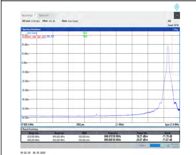
1-N26-824-849-PC3-15-20-H-5-CP-QPSK-Edge_1RB_Right-1@105-1-seegraph-PASS-see graph
