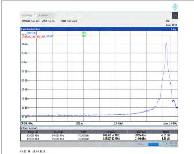
1-N26-824-849-PC3-15-20-H-2-DFT-PI2BPSK-Edge_1RB_Right-1@105-1-seegraph-PASS-see graph
