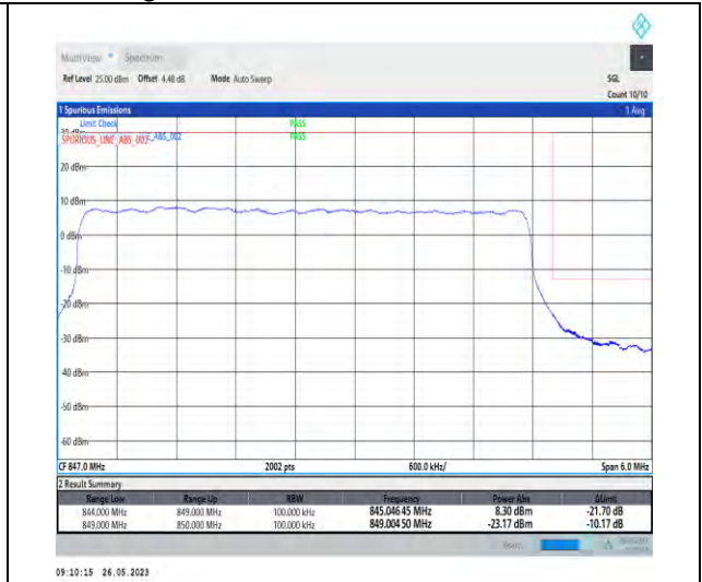
1-N26-824-849-PC3-15-5-H-3-DFT-PI2BPSK-Outer_Full-25@0-1-seegraph-PASS-see graph
