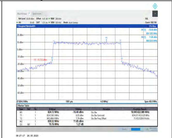
1-N26-824-849-PC3-15-20-L-7-CP-16QAM-Outer_Full-106@0-18.946-19.760-≤20-PASS
