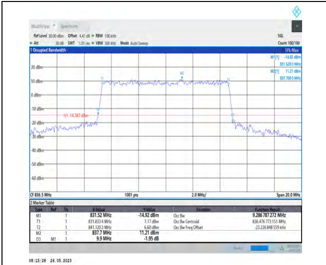
1-N26-824-849-PC3-15-10-M-7-CP-16QAM-Outer_F ull-52@0-9.287-9.900-≤10-PASS
