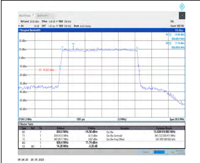
1-N26-824-849-PC3-15-15-H-5-DFT-256QAM-Outer_Full-75@0-13.438-14.280-≤15-PASS
