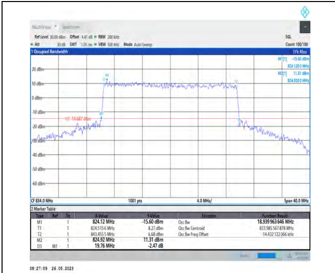
1-N26-824-849-PC3-15-20-L-6-CP-QPSK-Outer_Full -106@0-18.94-19.760-≤20-PASS
