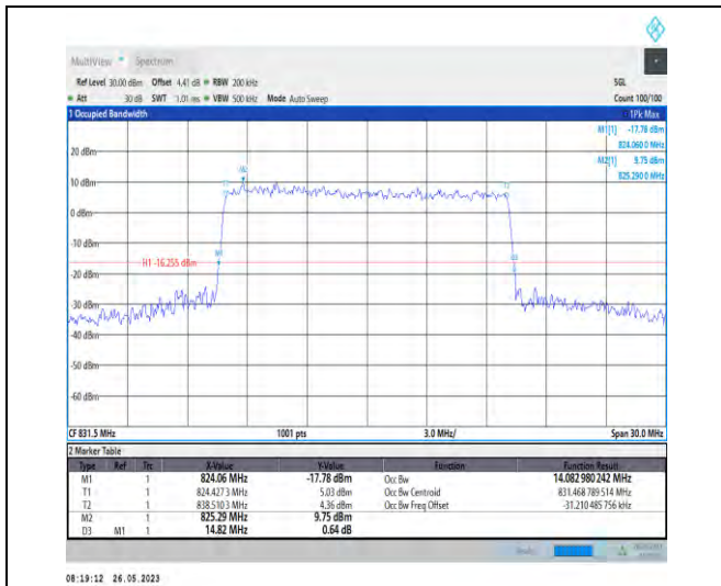
1-N26-824-849-PC3-15-15-L-9-CP-256QAM-Outer_Full-79@0-14.083-14.820-≤15-PASS
