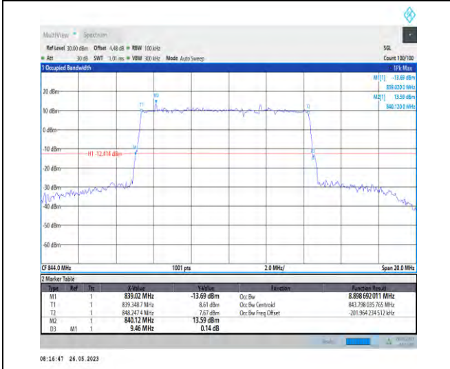
1-N26-824-849-PC3-15-10-H-4-DFT-64QAM-Outer_Full-50@0-8.899-9.460-≤10-PASS
