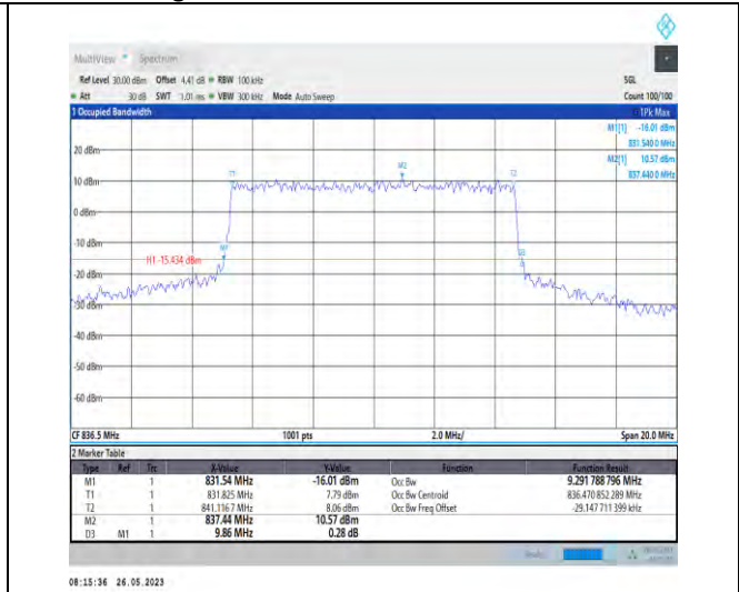
1-N26-824-849-PC3-15-10-M-8-CP-64QAM-Outer_F ull-52@0-9.292-9.860-≤10-PASS
