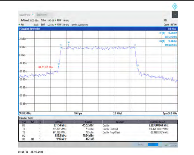
1-N26-824-849-PC3-15-10-M-6-CP-QPSK-Outer_Ful I-52@0-9.293-9.960-≤10-PASS
