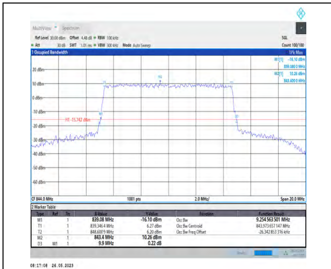
1-N26-824-849-PC3-15-10-H-6-CP-QPSK-Outer_Ful I-52@0-9.255-9.900-≤10-PASS
