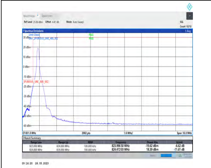
1-N26-824-849-PC3-15-15-L-4-CP-QPSK-Edge_1RB_Left-1@0-1-seegraph-PASS-see graph
