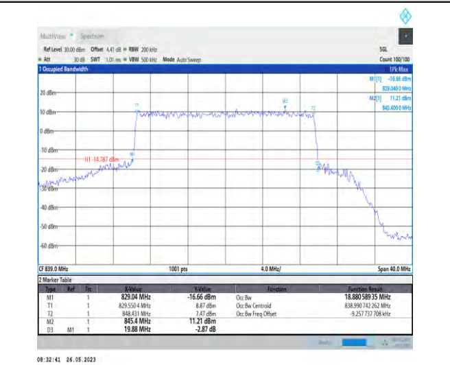
1-N26-824-849-PC3-15-20-H-7-CP-16QAM-Outer_Full-106@0-18.881-19.880-≤20-PASS
