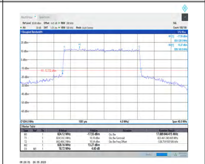
1-N26-824-849-PC3-15-20-L-1-DFT-QPSK-Outer_Full-100@0-17.89-18.720-≤20-PASS
