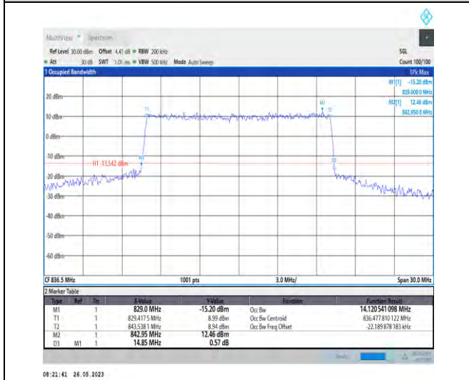
1-N26-824-849-PC3-15-15-M-6-CP-QPSK-Outer_Full-79@0-14.121-14.850-≤15-PASS
