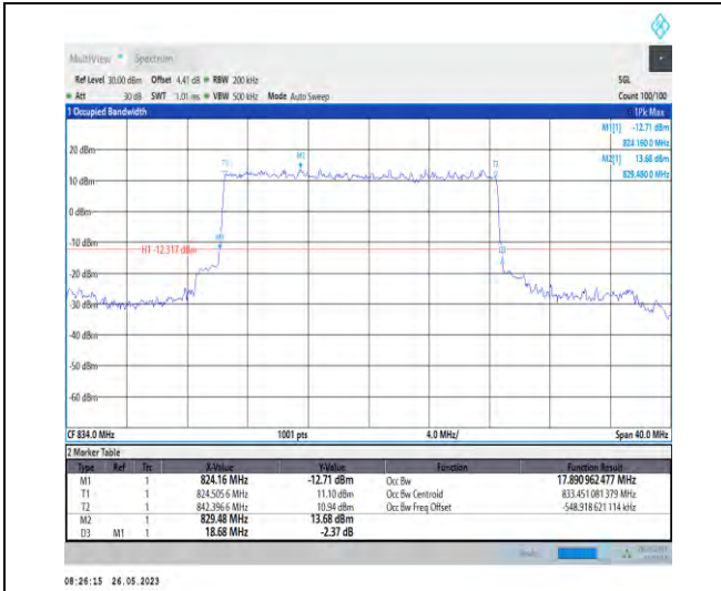
1-N26-824-849-PC3-15-20-L-2-DFT-PI2BPSK-Outer_Full-100@0-17.891-18.680-≤20-PASS
