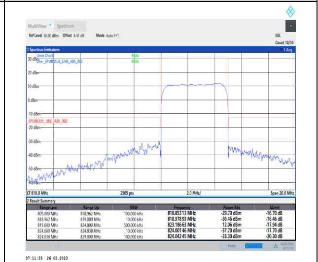
1-N26-814-824-PC3-15-5-H-6-CP-QPSK-Outer_Full-25@0-1--PASS-see graph
