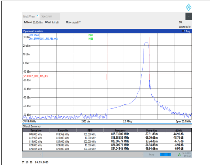
1-N26-814-824-PC3-15-5-H-2-DFT-PI2BPSK-Edge_1 RB_Right-1@24-1--PASS-see graph
