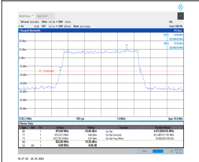
1-N26-814-824-PC3-15-5-H-5-DFT-256QAM-Outer_Full-25@0-4.473-4.840-≤5-PASS
