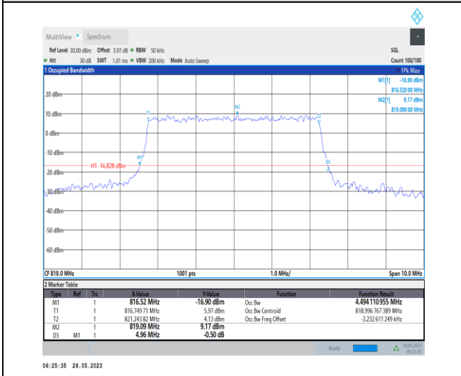
1-N26-814-824-PC3-15-5-M-6-CP-QPSK-Outer_Full-25@0-4.494-4.960-≤5-PASS
