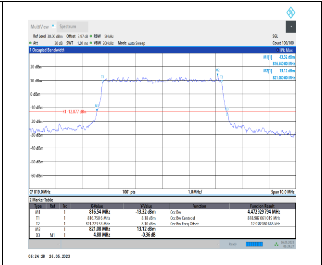
1-N26-814-824-PC3-15-5-M-1-DFT-QPSK-Outer_Fu II-25@0-4.473-4.880-<math>\leq</math>5-PASS
