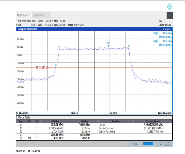
1-N26-814-824-PC3-15-5-H-6-CP-QPSK-Outer_Full-25@0-4.466-4.890-≤5-PASS
