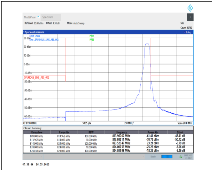
1-N26-814-824-PC3-15-10-H-2-DFT-PI2BPSK-Edge_1 RB_Right-1@51-1--PASS-see graph
