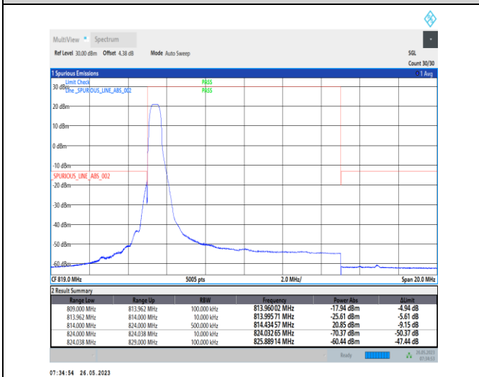
1-N26-814-824-PC3-15-10-L-4-CP-QPSK-Edge_1RB_Left-1@0-1--PASS-see graph
