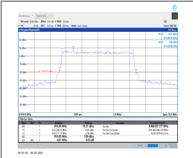
1-N26-814-824-PC3-15-5-L-9-CP-256QAM-Outer_Fu II-25@0-4.468-4.810-<math>\leq</math>5-PASS
