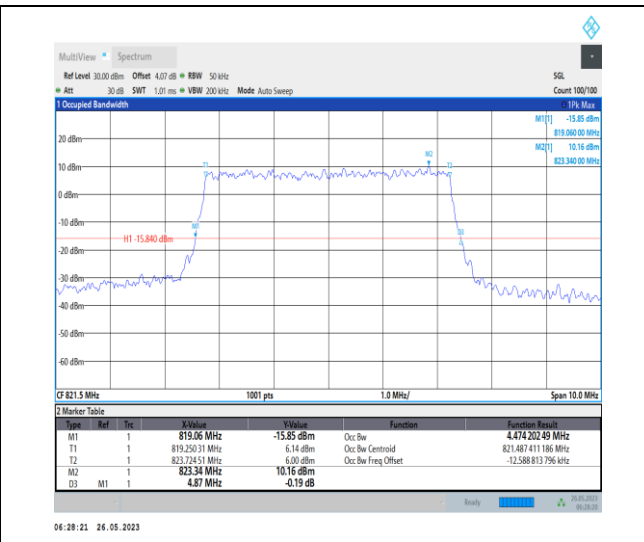
1-N26-814-824-PC3-15-5-H-8-CP-64QAM-Outer_Ful I-25@0-4.474-4.870≤5-PASS
