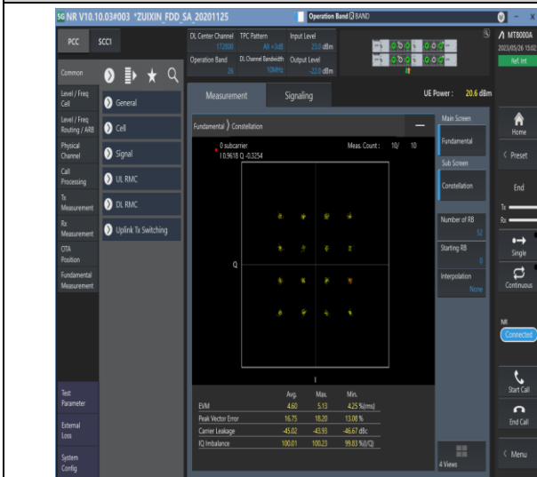
1-N26-814-824-PC3-15-10-M-7-CP-16QAM-Outer_F ull-52@0-see graph-PASS
