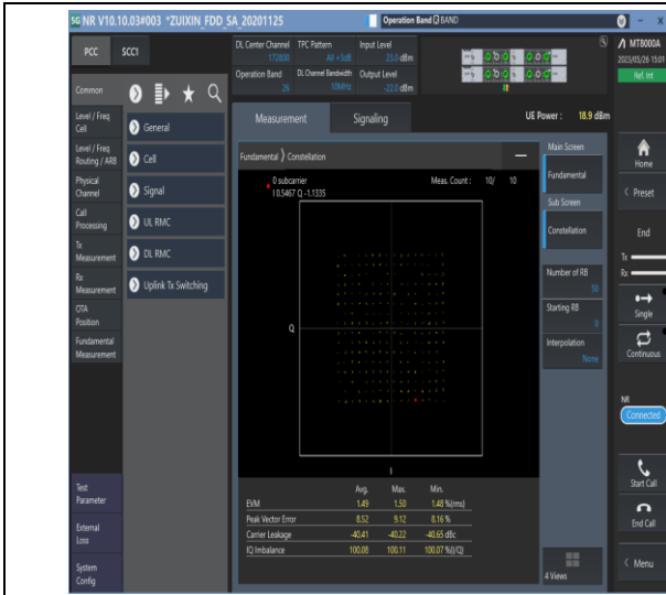
1-N26-814-824-PC3-15-10-M-5-DFT-256QAM-Outer_ Full-50@0-see graph-PASS
