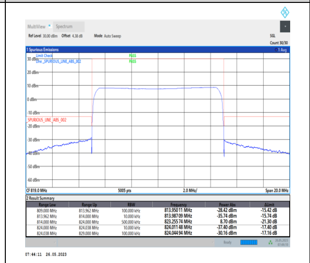
1-N26-814-824-PC3-15-10-H-6-CP-QPSK-Outer Full-52@0-1--PASS-see graph
