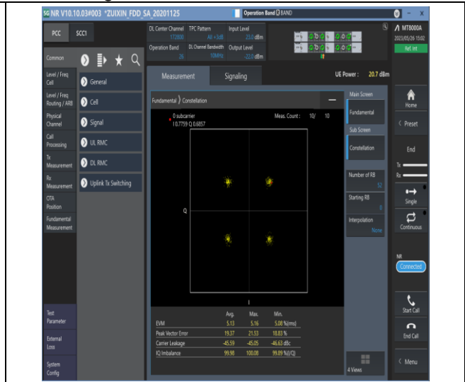
1-N26-814-824-PC3-15-10-M-6-CP-QPSK-Outer_F ull-52@0-see graph-PASS
