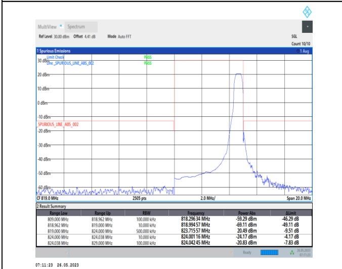
1-N26-814-824-PC3-15-5-H-5-CP-QPSK-Edge_1RB_Right-1@24-1--PASS-see graph
