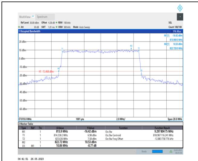
1-N26-814-824-PC3-15-10-M-6-CP-QPSK-Outer_Fu II-52@0-9.298-10.060-≤10-PASS
