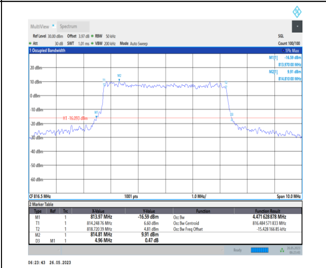
1-N26-814-824-PC3-15-5-L-8-CP-64QAM-Outer_Full-25@0-4.472-4.960-≤5-PASS
