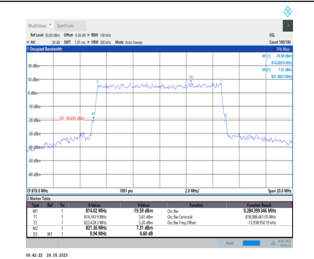
1-N26-814-824-PC3-15-10-M-9-CP-256QAM-Outer_ Full-52@0-9.284-9.940-≤10-PASS
