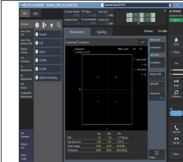
1-N26-814-824-PC3-15-10-M-1-DFT-PI2BPSK-Outer_Full-50@0-see graph-PASS
