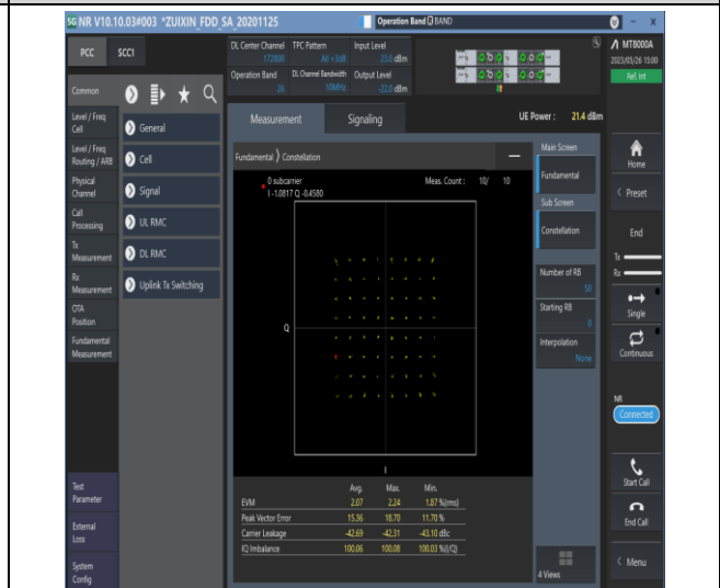
1-N26-814-824-PC3-15-10-M-4-DFT-64QAM-Outer_Full-50@0-see graph-PASS
