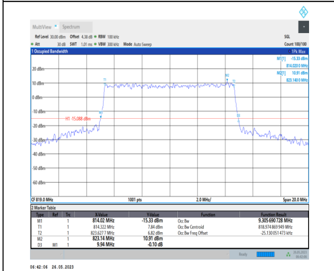
1-N26-814-824-PC3-15-10-M-8-CP-64QAM-Outer_F ull-52@0-9.306-9.940-≤10-PASS
