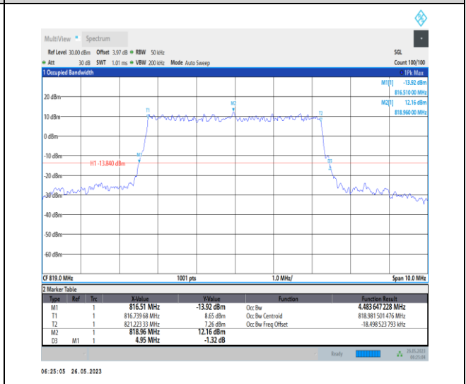
1-N26-814-824-PC3-15-5-M-3-DFT-16QAM-Outer_Full-25@0-4.484-4.950-<math>\leq</math>5-PASS
