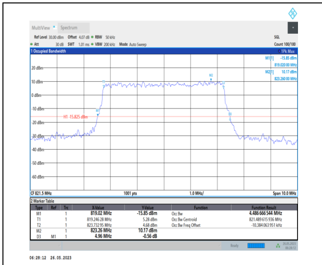
1-N26-814-824-PC3-15-5-H-7-CP-16QAM-Outer_Ful I-25@0-4.487-4.960≤5-PASS
