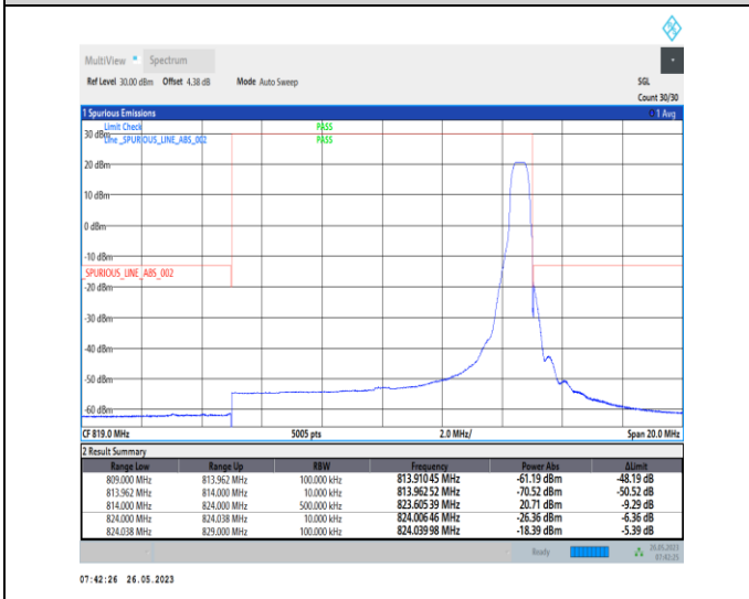
1-N26-814-824-PC3-15-10-H-5-CP-QPSK-Edge_1RB Right-1@51-1--PASS-see graph
