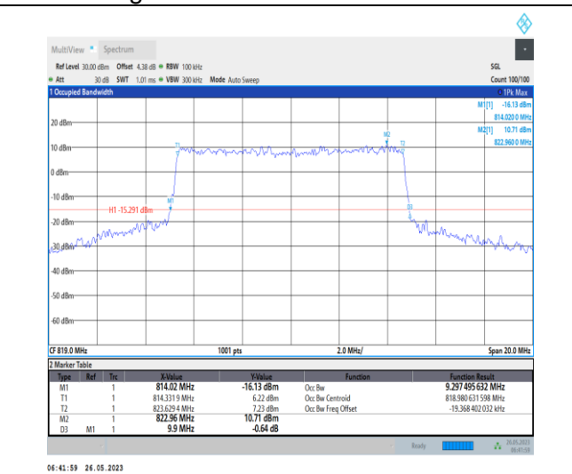
1-N26-814-824-PC3-15-10-M-7-CP-16QAM-Outer_F ull-52@0-9.297-9.900-≤10-PASS
