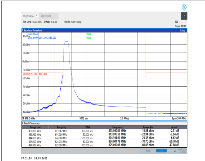
1-N26-814-824-PC3-15-10-L-1-DFT-PI2BPSK-Edge_1 RB_Left-1@0-1--PASS-see graph
