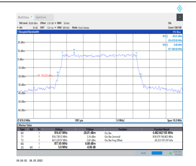
1-N26-814-824-PC3-15-5-M-9-CP-256QAM-Outer_F uII-25@0-4.482-5.000-≤5-PASS
