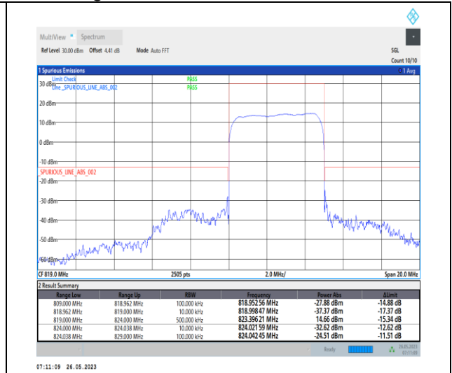
1-N26-814-824-PC3-15-5-H-3-DFT-PI2BPSK-Outer_Full-25@0-1--PASS-see graph
