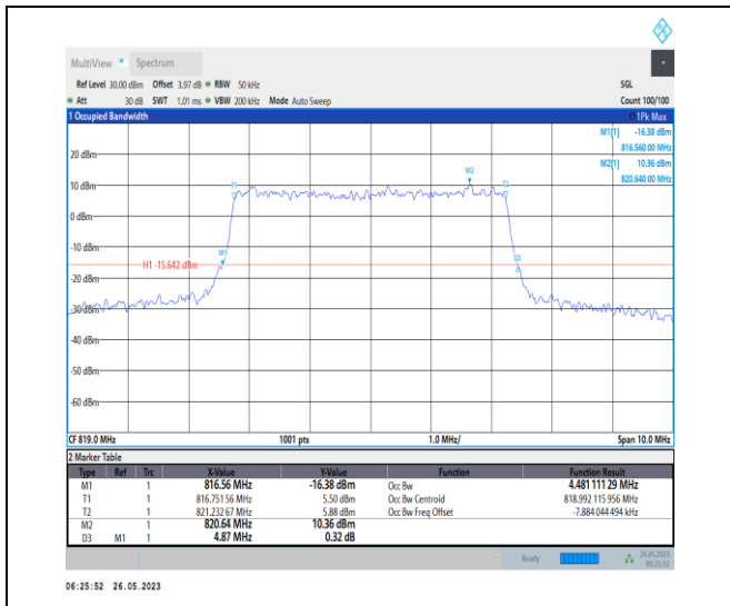
1-N26-814-824-PC3-15-5-M-8-CP-64QAM-Outer_Fu II-25@0-4.481-4.870-≤5-PASS
