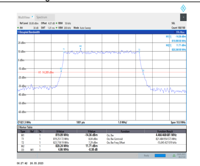
1-N26-814-824-PC3-15-5-H-4-DFT-64QAM-Outer_Full-25@0-4.466-4.860-≤5-PASS
