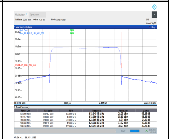
1-N26-814-824-PC3-15-10-L-6-CP-QPSK-Outer_F ull-52@0-1--PASS-see graph
