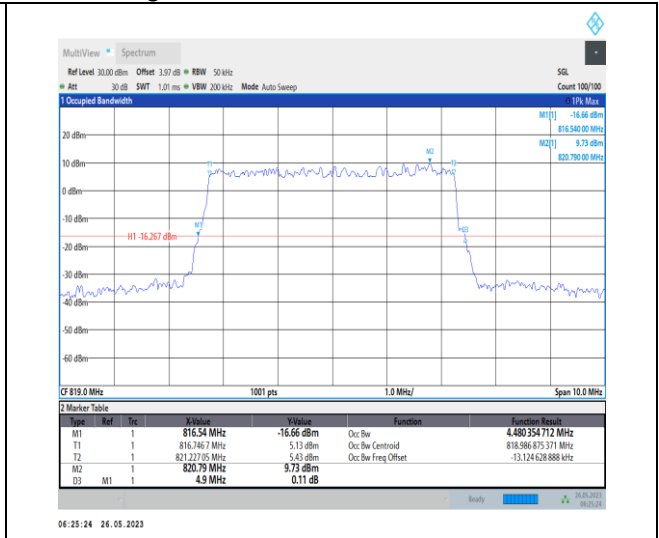
1-N26-814-824-PC3-15-5-M-5-DFT-256QAM-Outer_Full-25@0-4.48-4.900-≤5-PASS
