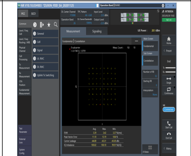
1-N26-814-824-PC3-15-10-M-8-CP-64QAM-Outer_ Full-52@0-see graph-PASS
