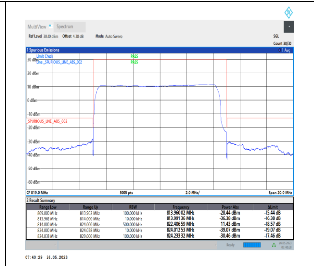
1-N26-814-824-PC3-15-10-H-3-DFT-PI2BPSK-Out er_Full-50@0-1--PASS-see graph
