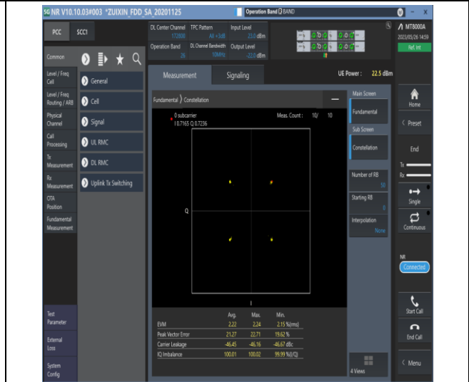
1-N26-814-824-PC3-15-10-M-2-DFT-QPSK-Outer_Full-50@0-see graph-PASS
