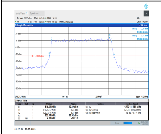
1-N26-814-824-PC3-15-5-H-1-DFT-QPSK-Outer_Ful I-25@0-4.47-4.830-≤5-PASS
