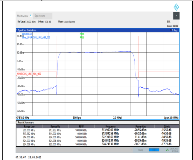
1-N26-814-824-PC3-15-10-L-3-DFT-PI2BPSK-Out er_Full-50@0-1--PASS-see graph
