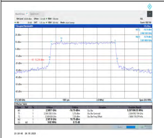
1-N7-PC3-15-10-L-8-CP-64QAM-Outer_Full-52@0-9. 9.268-9.820-≤10-PASS
