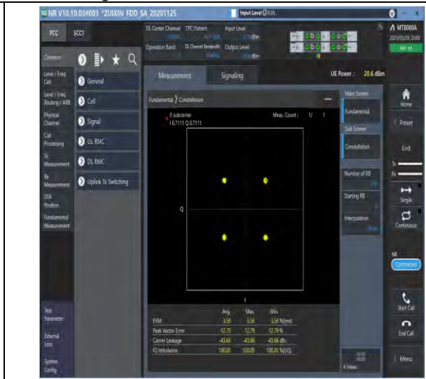
1-N7-PC3-15-40-M-6-CP-QPSK-Outer_Full-216@0-see graph-PASS
