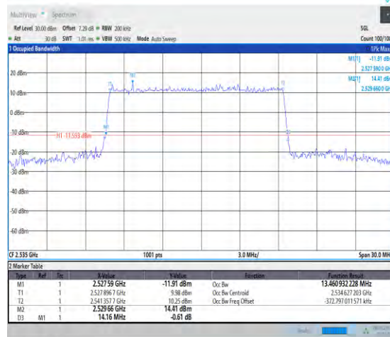
1-N7-PC3-15-15-M-3-DFT-16QAM-Outer_Full-75@0 -13.461-14.160≤15-PASS
