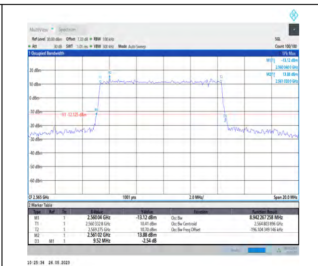
1-N7-PC3-15-10-H-1-DFT-QPSK-Outer_Full-50@0-8.942-9.520-≤10-PASS
