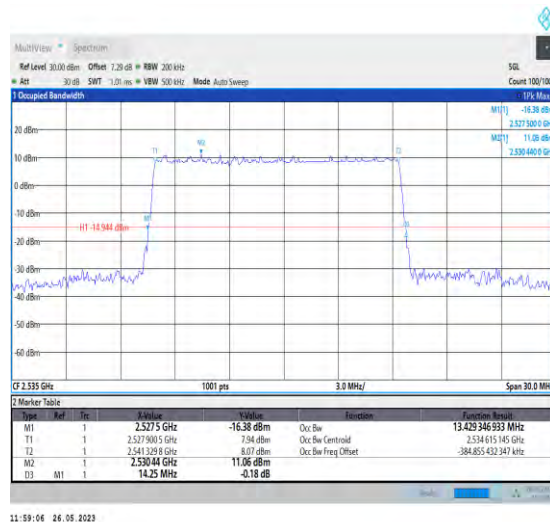
1-N7-PC3-15-15-M-5-DFT-256QAM-Outer_Full-75@0 0-13.429-14.250≤15-PASS
