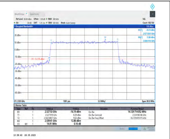
1-N7-PC3-15-15-M-7-CP-16QAM-Outer_Full-79@0-1 14.13-14.910-≤15-PASS
