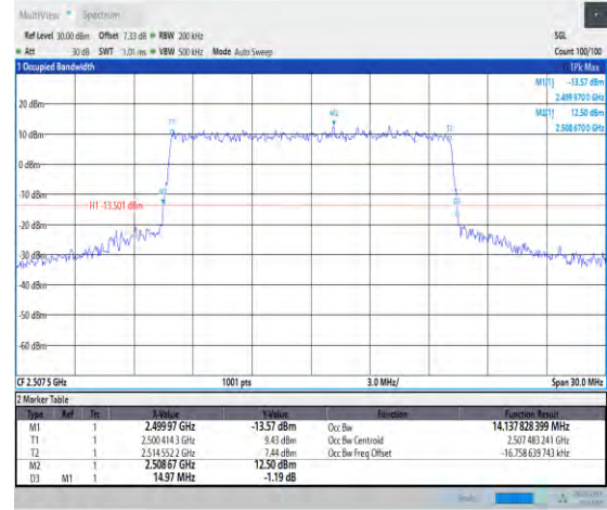
1-N7-PC3-15-15-L-8-CP-64QAM-Outer_Full-79@0-1 4.138-14.970-≤15-PASS
