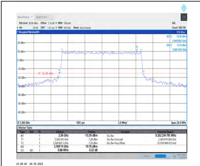
1-N7-PC3-15-10-H-8-CP-64QAM-Outer_Full-52@0-9.262-9.880-≤10-PASS
