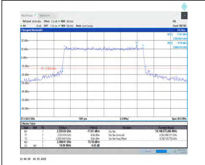
1-N7-PC3-15-15-H-7-CP-16QAM-Outer_Full-79@0-1 4.148-14.940-≤15-PASS
