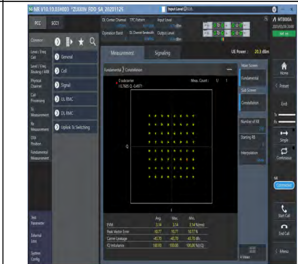
1-N7-PC3-15-40-M-8-CP-64QAM-Outer_Full-216@0-see graph-PASS
