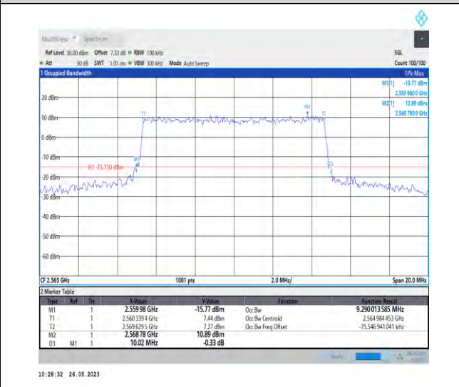
1-N7-PC3-15-10-H-7-CP-16QAM-Outer_Full-52@0- 9.29-10.020-≤10-PASS
