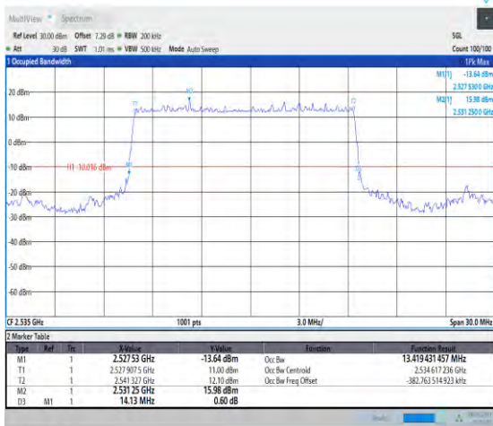
1-N7-PC3-15-15-M-2-DFT-PI2BPSK-Outer_Full-75@0 0-13.419-14.130≤15-PASS
