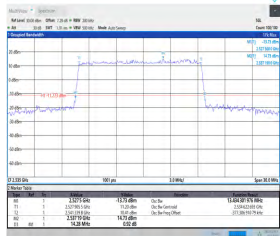
1-N7-PC3-15-15-M-1-DFT-QPSK-Outer_Full-75@0-1 13.434-14.280-≤15-PASS
