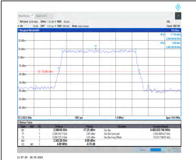
1-N7-PC3-15-5-L-5-DFT-256QAM-Outer_Full-25@0-4.483-4.890-≤5-PASS
