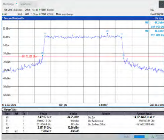
1-N7-PC3-15-15-L-7-CP-16QAM-Outer_Full-79@0-1 4.125-15.000-≤15-PASS
