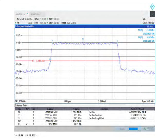
1-N7-PC3-15-10-L-6-CP-QPSK-Outer_Full-52@0-9. 278-9.920-≤10-PASS
