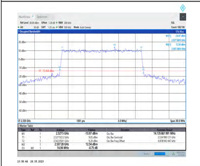
1-N7-PC3-15-15-M-8-CP-64QAM-Outer_Full-79@0-1 14.136-14.940-≤15-PASS
