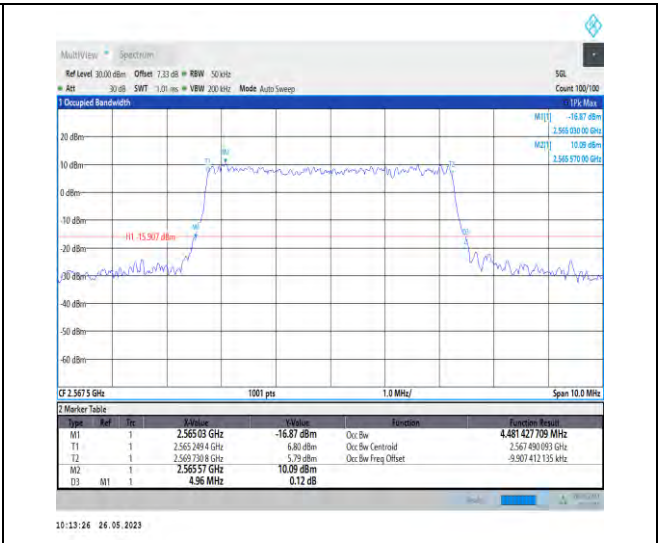
1-N7-PC3-15-5-H-8-CP-64QAM-Outer_Full-25@0-4. 481-4.960-≤5-PASS
