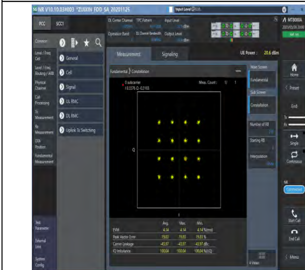
1-N7-PC3-15-40-M-7-CP-16QAM-Outer_Full-216@0-see graph-PASS
