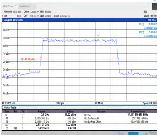
1-N7-PC3-15-15-L-9-CP-256QAM-Outer_Full-79@0-1 14.111-14.970-≤15-PASS
