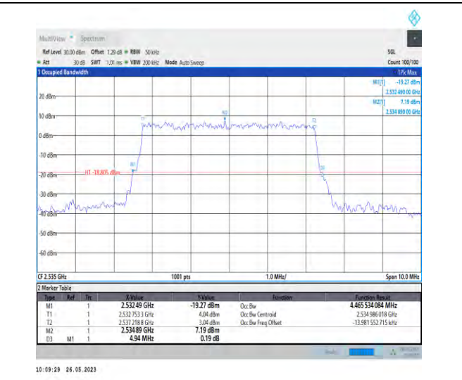
1-N7-PC3-15-5-M-9-CP-256QAM-Outer_Full-25@0-4 .466-4.940-≤5-PASS
