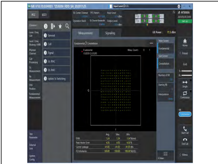
1-N7-PC3-15-40-M-9-CP-256QAM-Outer_Full-216@0-see graph-PASS
