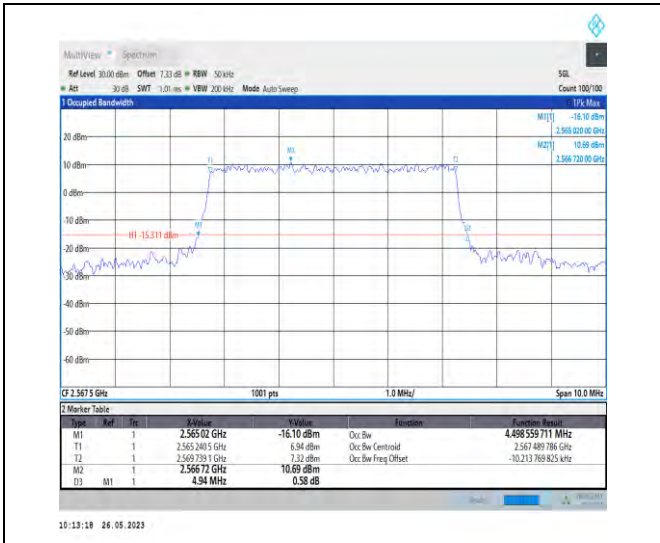
1-N7-PC3-15-5-H-7-CP-16QAM-Outer_Full-25@0-4. 499-4.940-≤5-PASS
