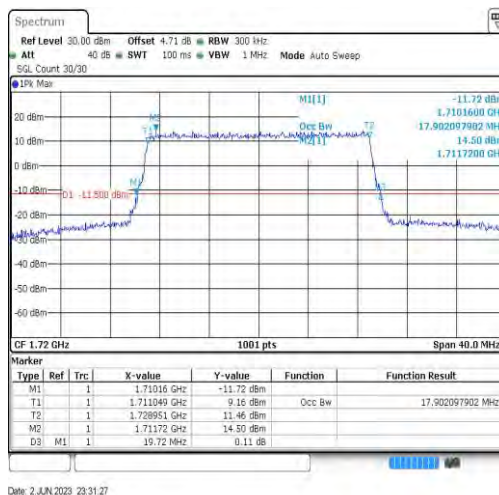
Band66-20MHz-64QAM-132072-100RB#0-17.902
