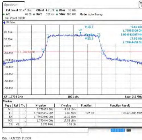
Band66-1.4MHz-QPSK-132665-6RB#0-1.085
