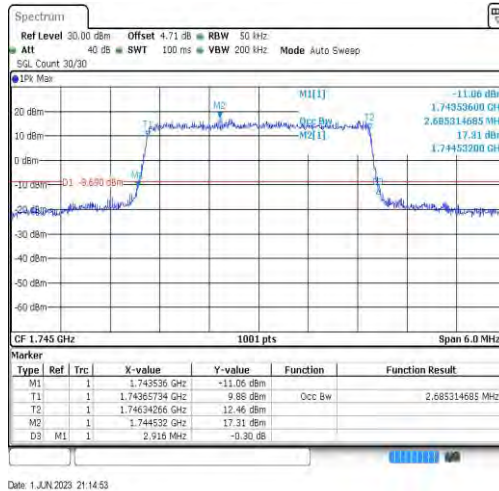
Band66-3MHz-QPSK-132322-15RB#0-2.685
