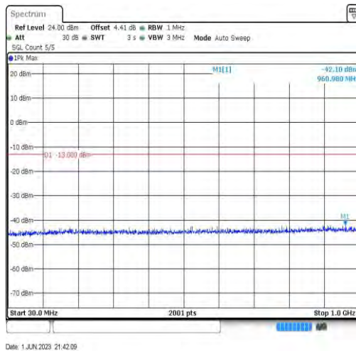
Band66-20MHz-QPSK-132322-1RB#0-Range3:30~1000MHz
