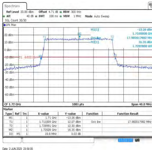
Band66-20MHz-QPSK-132072-100RB#0-17.982
