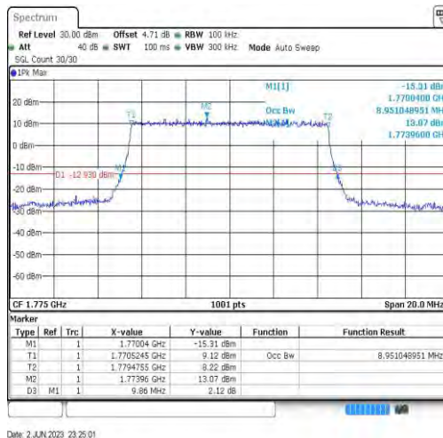
Band66-10MHz-64QAM-132622-50RB#0-8.951
