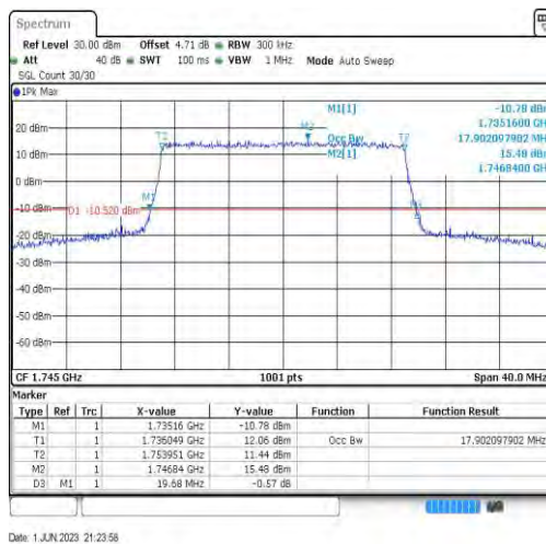
Band66-20MHz-16QAM-132322-100RB#0-17.902
