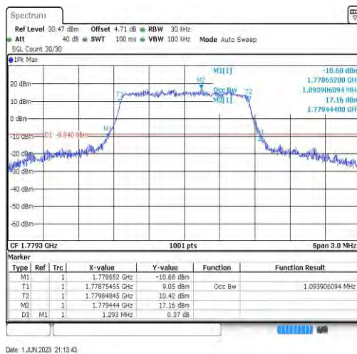
Band66-1.4MHz-16QAM-132665-6RB#0-1.094
