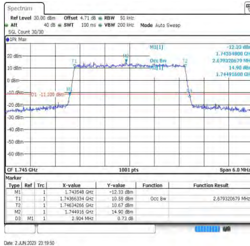
Band66-3MHz-64QAM-132322-15RB#0-2.679
