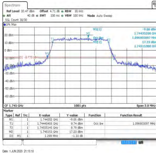
Band66-1.4MHz-16QAM-132322-6RB#0-1.097
