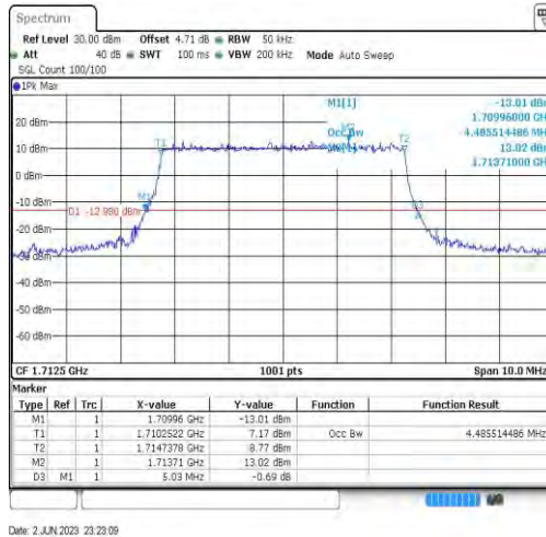
Band66-5MHz-64QAM-131997-25RB#0-4.486
