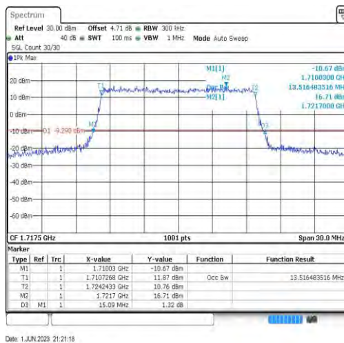
Band66-15MHz-16QAM-132047-75RB#0-13.516
