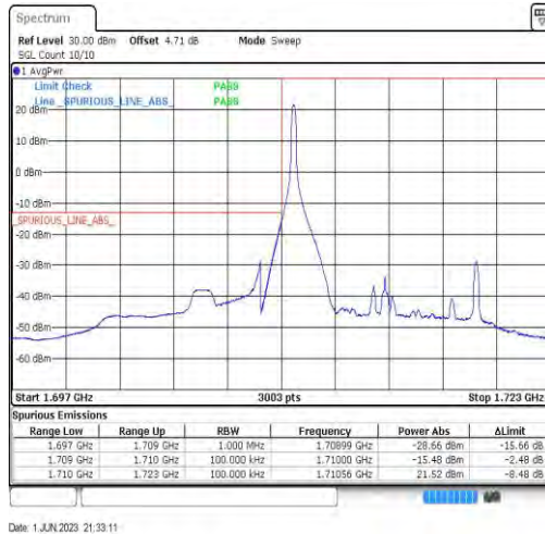
Band66-10MHz-QPSK-132022-1RB#0
