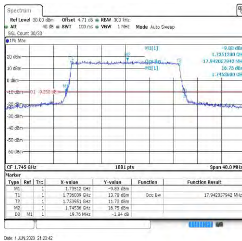
Band66-20MHz-QPSK-132322-100RB#0-17.942
