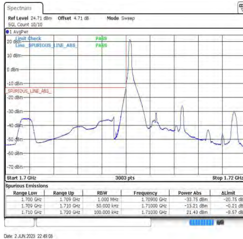
Band66-5MHz-QPSK-131997-1RB#0
