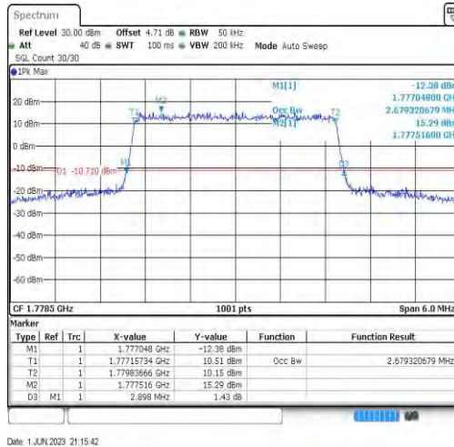
Band66-3MHz-16QAM-132657-15RB#0-2.679
