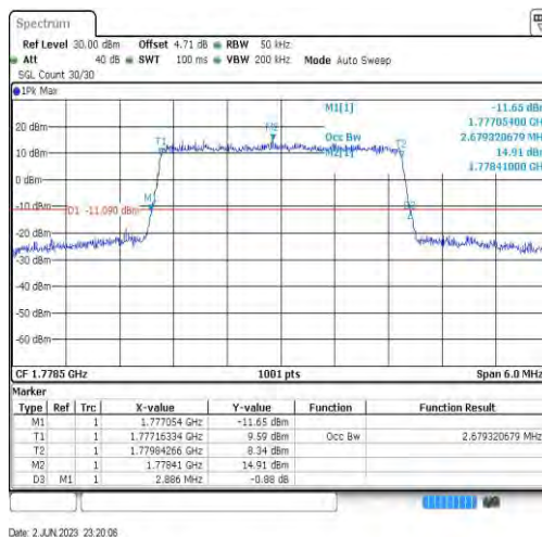
Band66-3MHz-64QAM-132657-15RB#0-2.679
