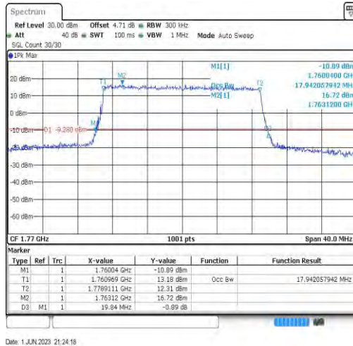
Band66-20MHz-QPSK-132572-100RB#0-17.942
