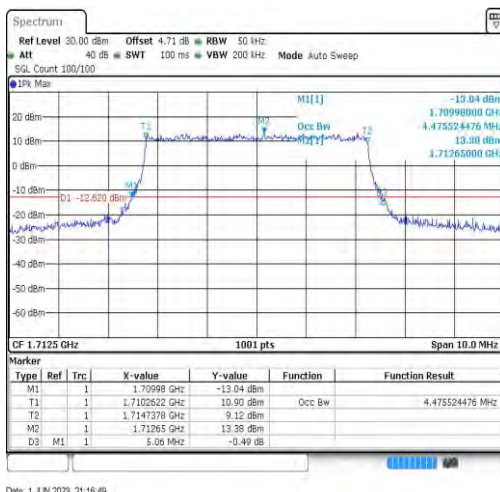
Band66-5MHz-16QAM-131997-25RB#0-4.476
