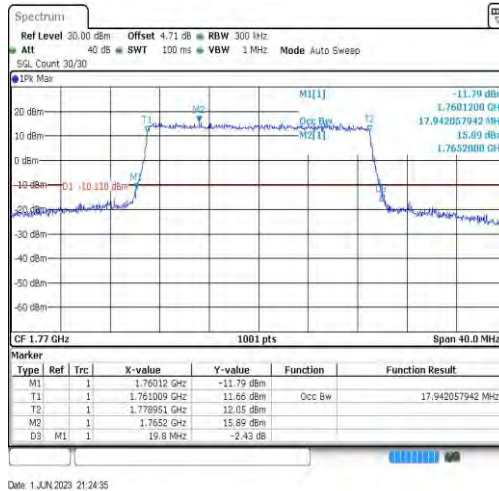
Band66-20MHz-16QAM-132572-100RB#0-17.942
