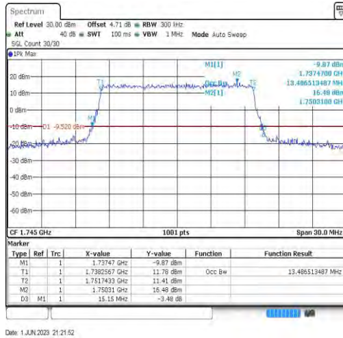
Band66-15MHz-16QAM-132322-75RB#0-13.487
