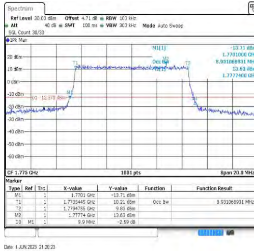
Band66-10MHz-16QAM-132622-50RB#0-8.931
