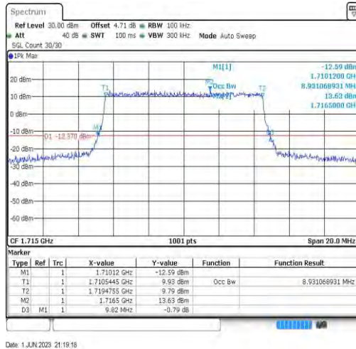
Band66-10MHz-16QAM-132022-50RB#0-8.931
