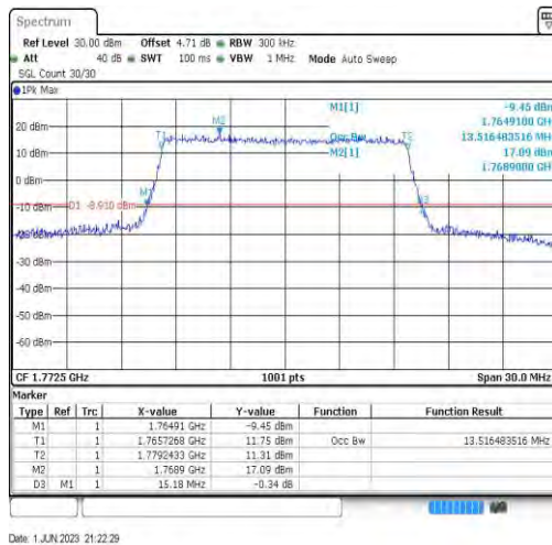
Band66-15MHz-16QAM-132597-75RB#0-13.516
