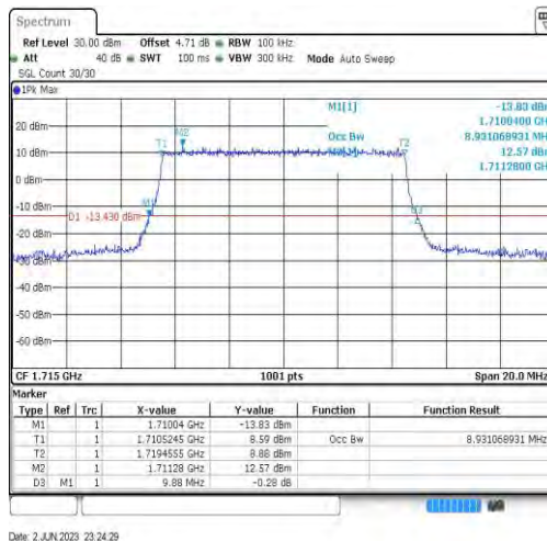
Band66-10MHz-64QAM-132022-50RB#0-8.931
