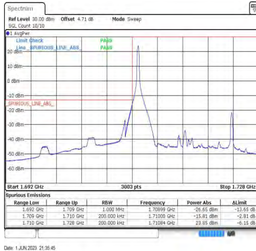
Band66-15MHz-QPSK-132047-1RB#0
