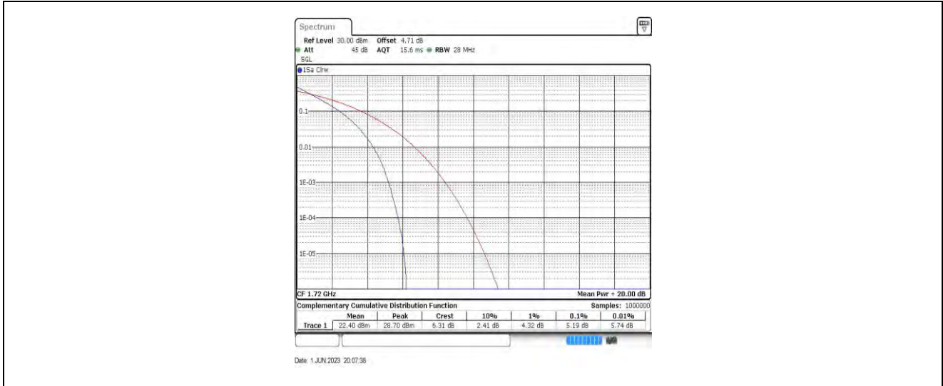
Band66-20MHz-QPSK-132072-100RB#0
