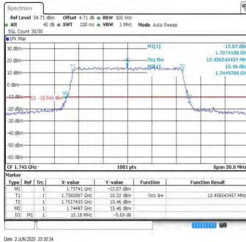
Band66-15MHz-64QAM-132322-75RB#0-13.457
