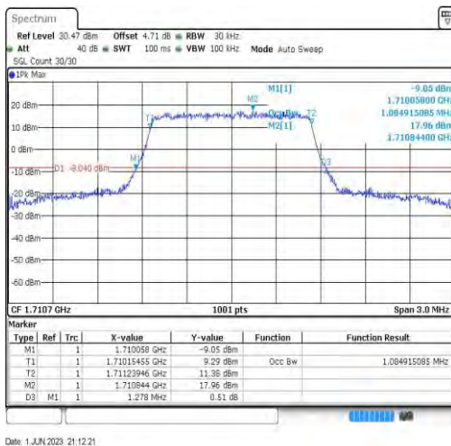
Band66-1.4MHz-QPSK-131979-6RB#0-1.085
