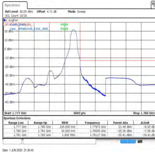
Band66-1.4MHz-QPSK-132665-1RB#5
