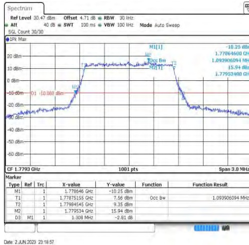
Band66-1.4MHz-64QAM-132665-6RB#0-1.094
