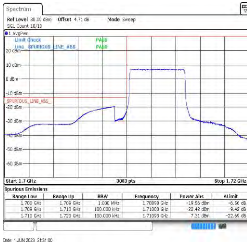
Band66-5MHz-QPSK-131997-25RB#0
