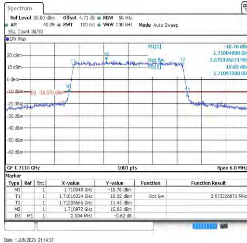
Band66-3MHz-16QAM-131987-15RB#0-2.673
