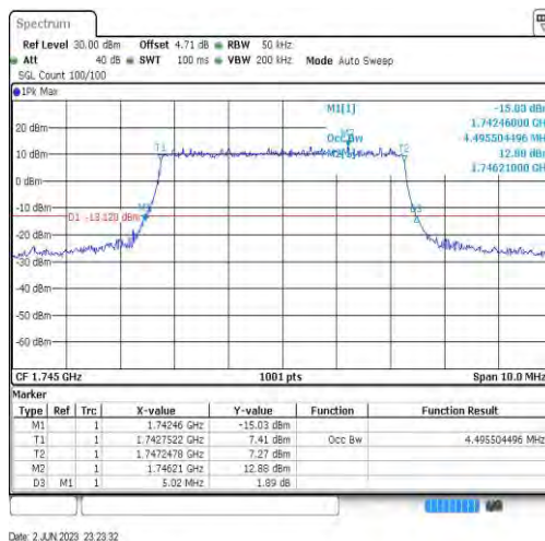
Band66-5MHz-64QAM-132322-25RB#0-4.496
