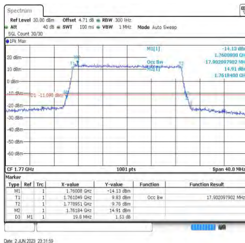
Band66-20MHz-64QAM-132572-100RB#0-17.902
