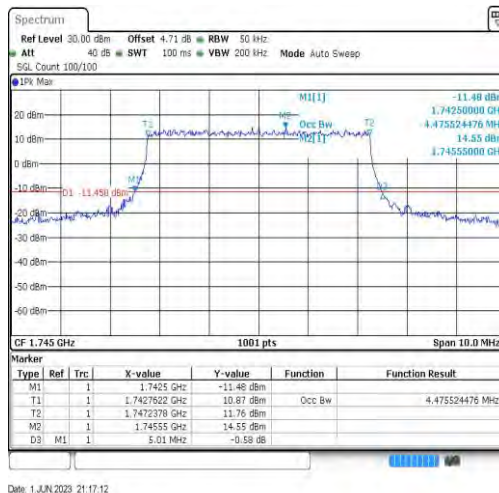
Band66-5MHz-QPSK-132322-25RB#0-4.476
