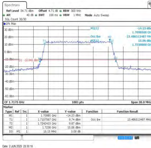
Band66-15MHz-64QAM-132047-75RB#0-13.487
