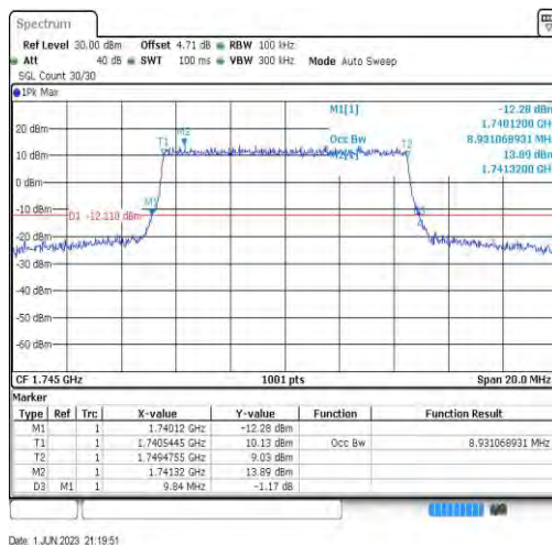
Band66-10MHz-16QAM-132322-50RB#0-8.931
