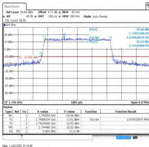
Band66-3MHz-16QAM-132322-15RB#0-2.679
