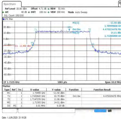
Band66-5MHz-QPSK-131997-25RB#0-4.476
