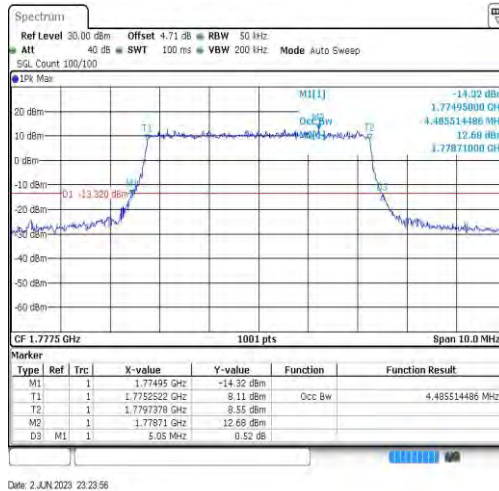
Band66-5MHz-64QAM-132647-25RB#0-4.486
