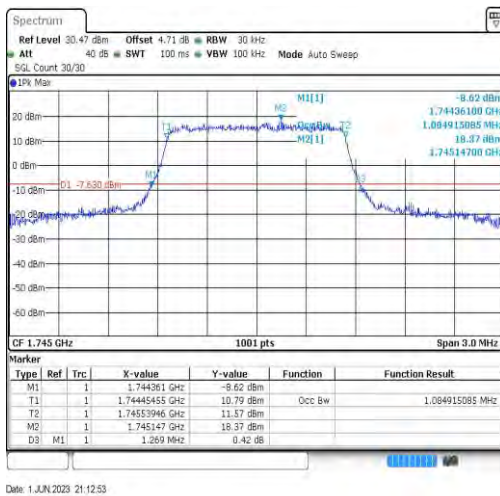
Band66-1.4MHz-QPSK-132322-6RB#0-1.085
