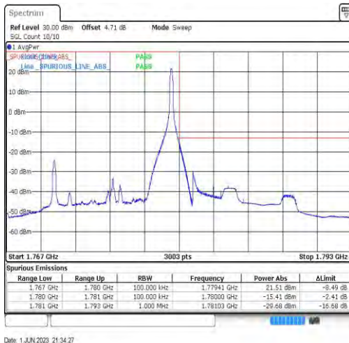
Band66-10MHz-QPSK-132622-1RB#49
