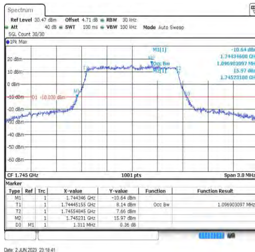
Band66-1.4MHz-64QAM-132322-6RB#0-1.097
