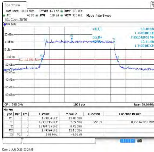
Band66-10MHz-64QAM-132322-50RB#0-8.951
