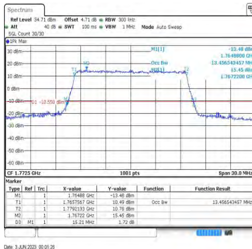
Band66-15MHz-64QAM-132597-75RB#0-13.457
