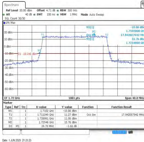
Band66-20MHz-16QAM-132072-100RB#0-17.942
