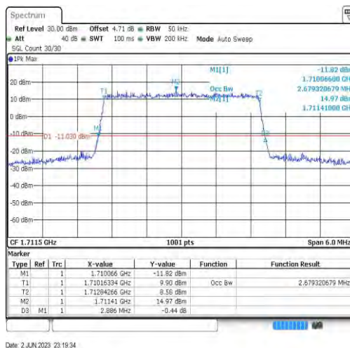
Band66-3MHz-64QAM-131987-15RB#0-2.679
