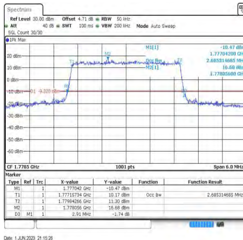
Band66-3MHz-QPSK-132657-15RB#0-2.685
