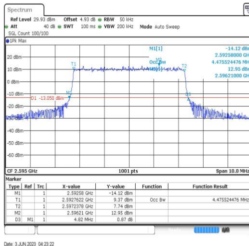
Band41-5MHz-64QAM-40640-25RB#0-4.476
