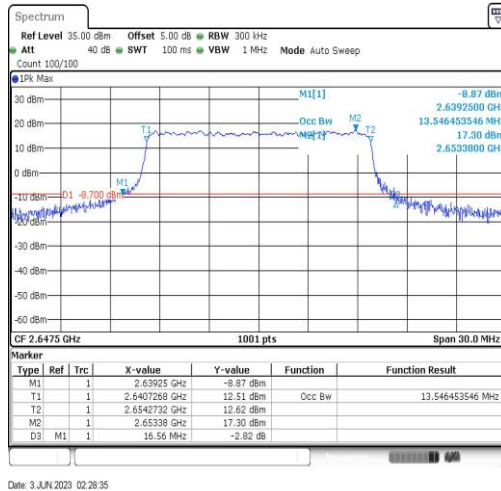
Band41-15MHz-QPSK-41165-75RB#0-13.546
