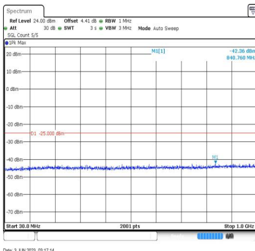
Band41-20MHz-QPSK-40640-1RB#0-Range3:30~1000MHz
