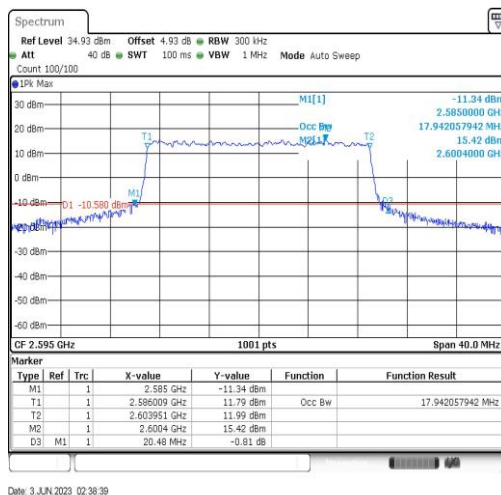
Band41-20MHz-16QAM-40640-100RB#0-17.942
