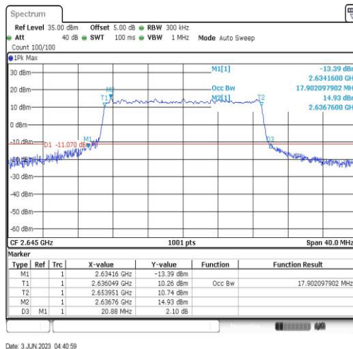
Band41-20MHz-64QAM-41140-100RB#0-17.902
