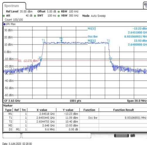
Band41-10MHz-QPSK-41190-50RB#0-8.931
