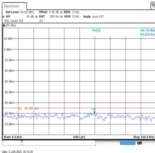
Band41-20MHz-QPSK-40140-1RB#0-Range1:0.009~0.15MHz
