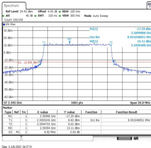
Band41-10MHz-64QAM-40640-50RB#0-8.951
