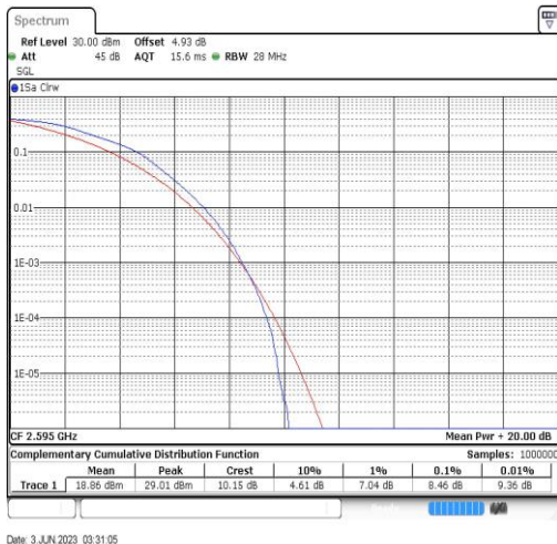
Band41-20MHz-16QAM-40640-100RB#0
