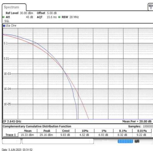
Band41-20MHz-16QAM-41140-100RB#0
