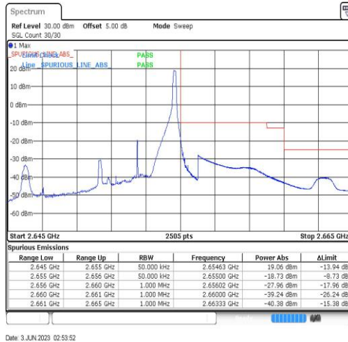
Band41-5MHz-QPSK-41215-1RB#24
