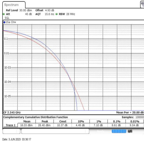
Band41-20MHz-64QAM-40140-100RB#0
