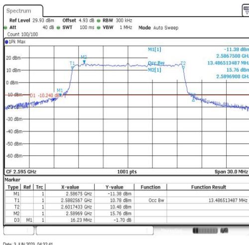
Band41-15MHz-64QAM-40640-75RB#0-13.487
