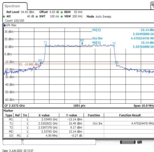
Band41-5MHz-16QAM-40065-25RB#0-4.476
