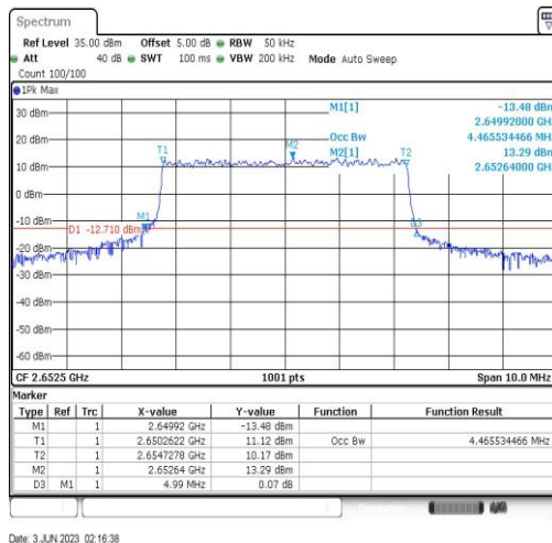
Band41-5MHz-16QAM-41215-25RB#0-4.466
