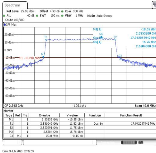
Band41-20MHz-16QAM-40140-100RB#0-17.942
