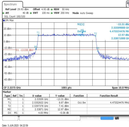
Band41-5MHz-64QAM-40065-25RB#0-4.476
