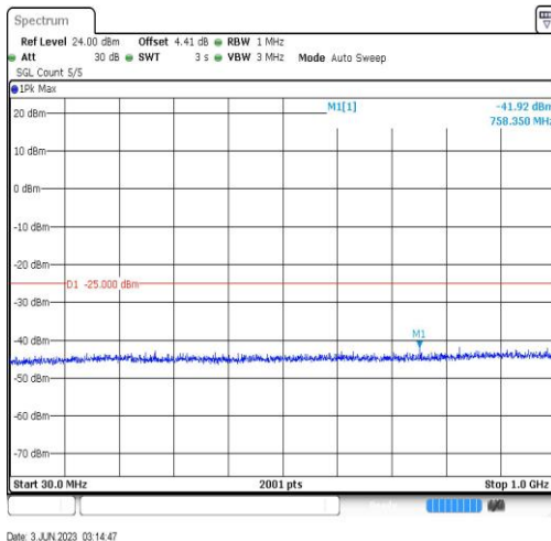
Band41-20MHz-QPSK-40140-1RB#0-Range3:30~1000MHz
