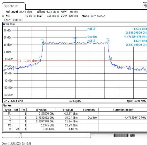
Band41-5MHz-QPSK-40065-25RB#0-4.476
