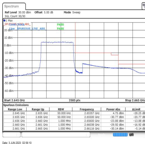
Band41-5MHz-QPSK-41215-25RB#0
