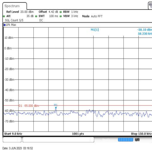
Band41-20MHz-QPSK-40640-1RB#0-Range1:0.009~0.15MHz
