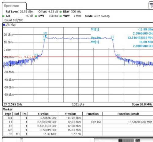
Band41-15MHz-16QAM-40640-75RB#0-13.516
