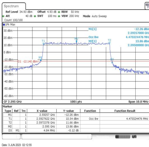
Band41-5MHz-QPSK-40640-25RB#0-4.476
