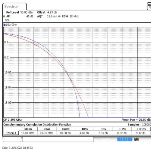
Band41-20MHz-64QAM-40640-100RB#0
