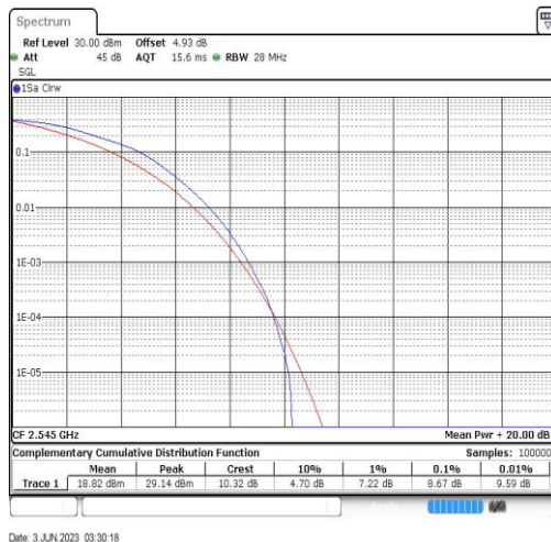
Band41-20MHz-16QAM-40140-100RB#0
