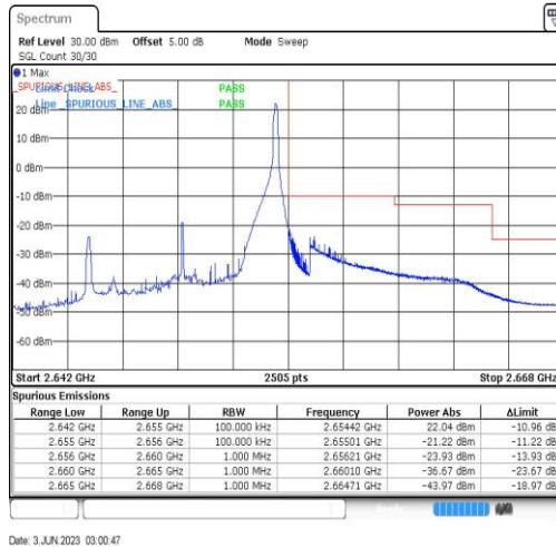
Band41-10MHz-QPSK-41190-1RB#49
