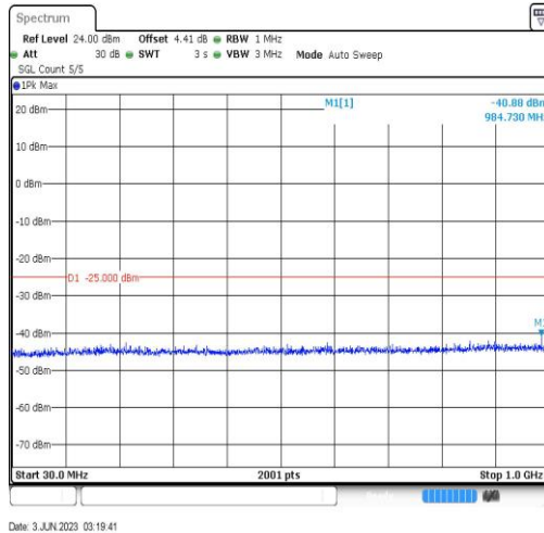
Band41-20MHz-QPSK-41140-1RB#0-Range3:30~1000MHz
