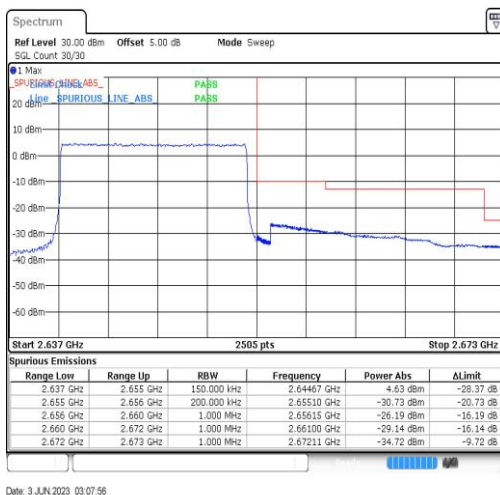
Band41-15MHz-QPSK-41165-75RB#0
