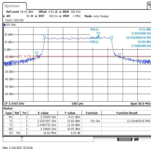
Band41-15MHz-16QAM-40115-75RB#0-13.516
