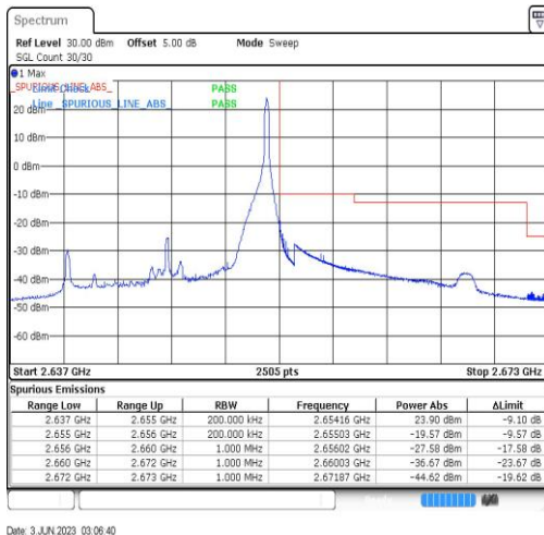
Band41-15MHz-QPSK-41165-1RB#74
