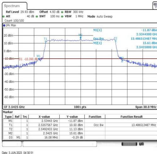
Band41-15MHz-64QAM-40115-75RB#0-13.487
