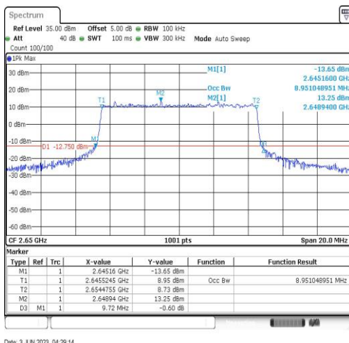
Band41-10MHz-64QAM-41190-50RB#0-8.951
