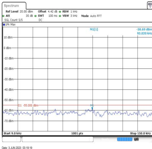
Band41-20MHz-QPSK-41140-1RB#0-Range1:0.009~0.15MHz
