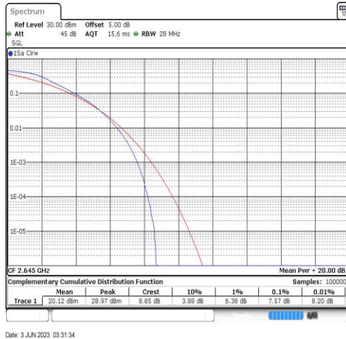
Band41-20MHz-QPSK-41140-100RB#0
