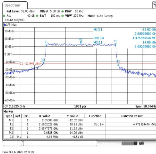
Band41-5MHz-QPSK-41215-25RB#0-4.476
