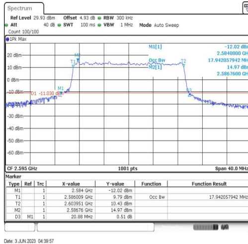
Band41-20MHz-64QAM-40640-100RB#0-17.942
