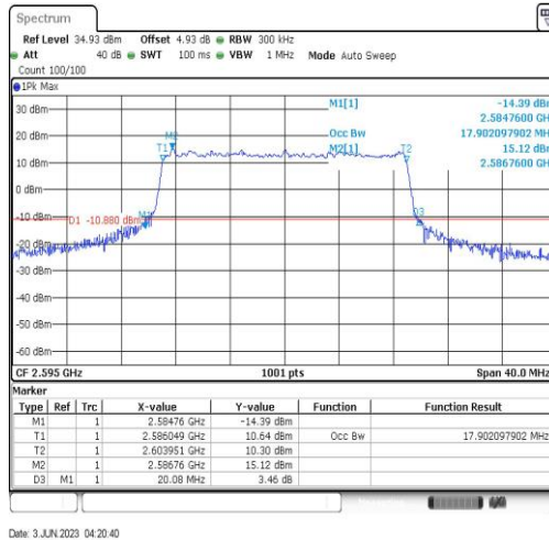
Band38-20MHz-64QAM-38000-100RB#0-17.902
