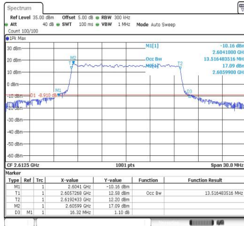
Band38-15MHz-16QAM-38175-75RB#0-13.516
