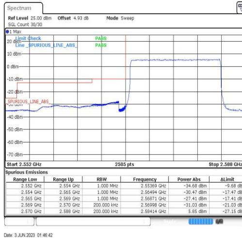
Band38-15MHz-QPSK-37825-75RB#0
