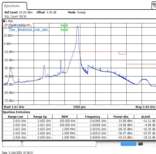
Band38-5MHz-QPSK-38225-1RB#24
