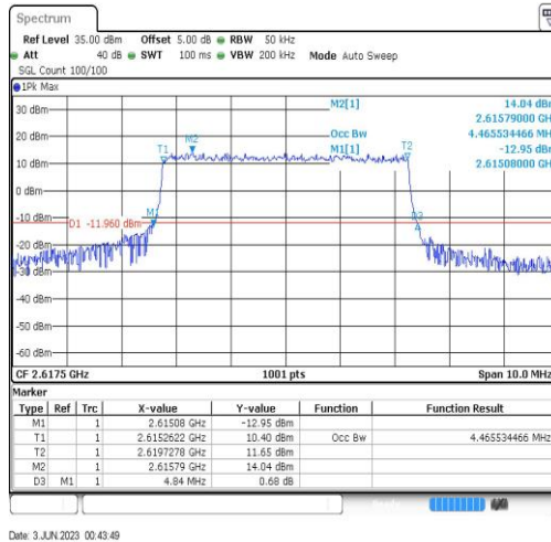
Band38-5MHz-QPSK-38225-25RB#0-4.466
