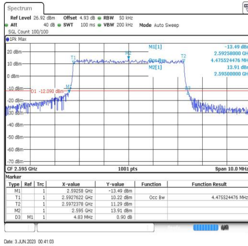
Band38-5MHz-QPSK-3800-25RB#0-4.476
