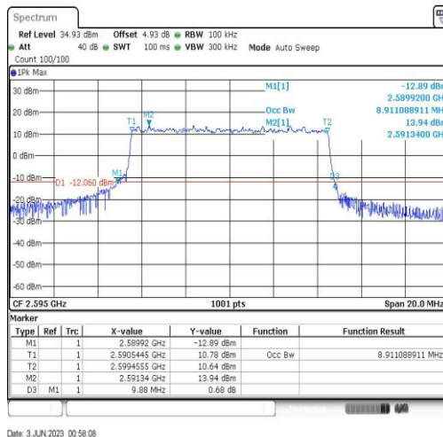
Band38-10MHz-16QAM-38000-50RB#0-8.911
