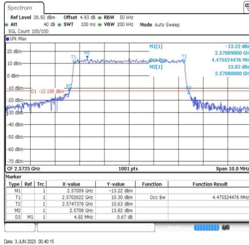
Band38-5MHz-QPSK-3775-25RB#0-4.476
