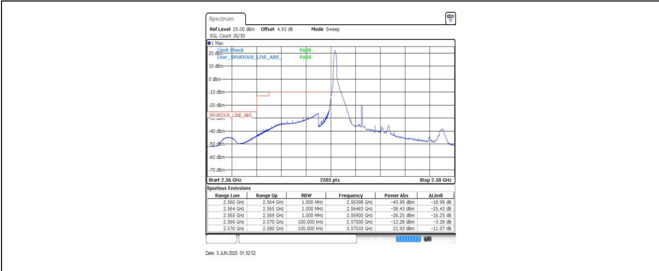
Band38-5MHz-QPSK-37775-1RB#0
