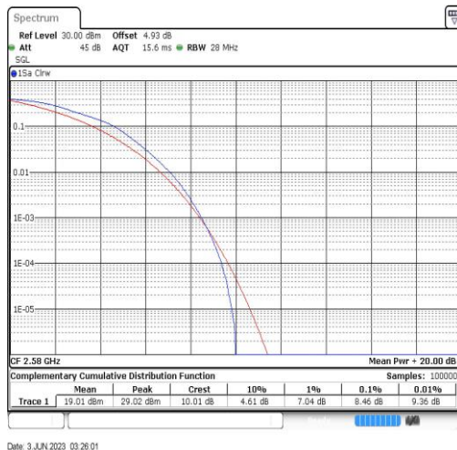
Band38-20MHz-16QAM-37850-100RB#0
