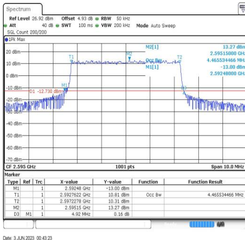
Band38-5MHz-16QAM-38000-25RB#0-4.466
