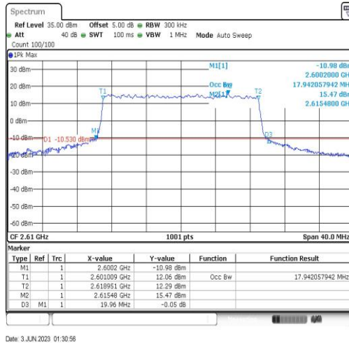
Band38-20MHz-16QAM-38150-100RB#0-17.942
