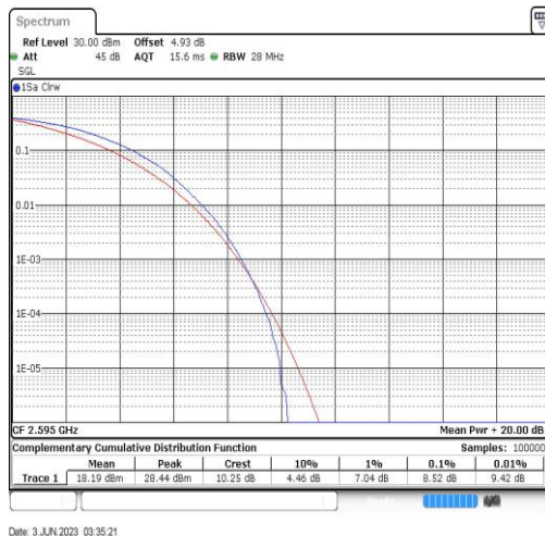
Band38-20MHz-64QAM-38000-100RB#0
