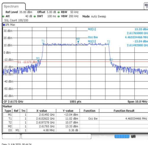
Band38-5MHz-16QAM-38225-25RB#0-4.466
