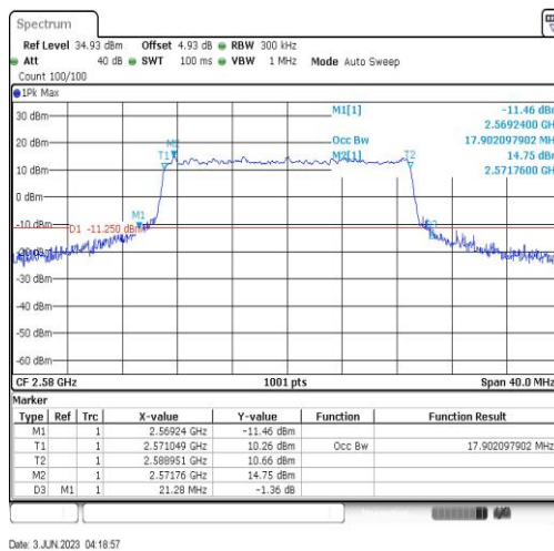
Band38-20MHz-64QAM-37850-100RB#0-17.902
