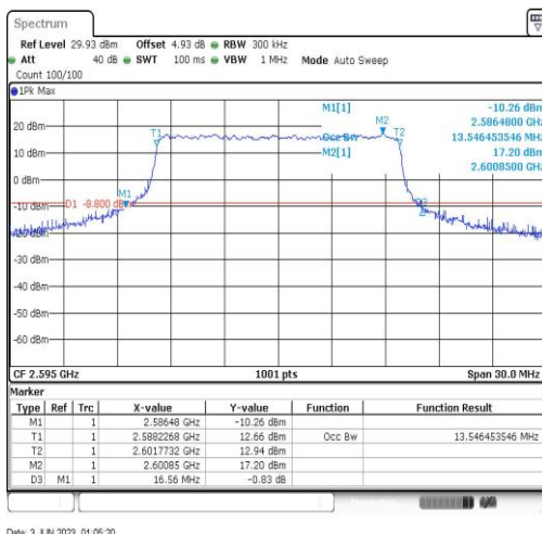
Band38-15MHz-QPSK-38000-75RB#0-13.546
