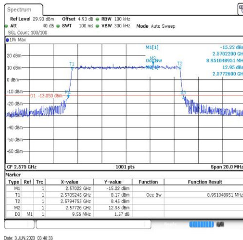
Band38-10MHz-64QAM-37800-50RB#0-8.951
