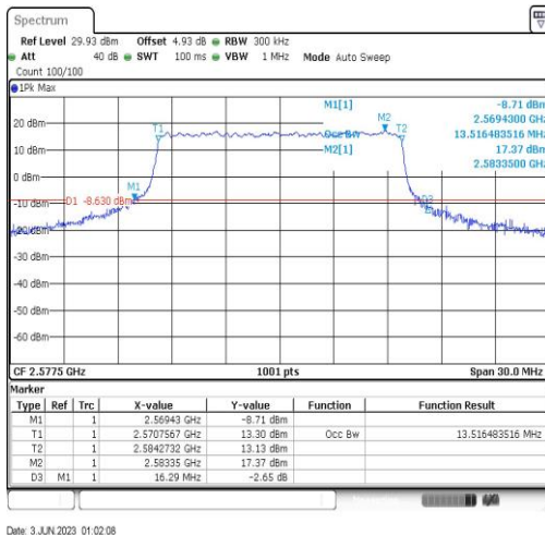
Band38-15MHz-QPSK-37825-75RB#0-13.516
