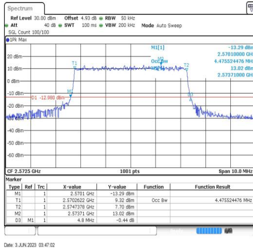
Band38-5MHz-64QAM-37775-25RB#0-4.476
