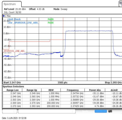
Band38-20MHz-QPSK-37850-100RB#0
