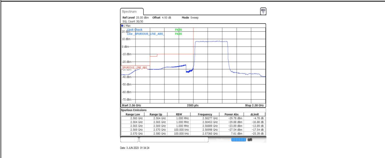
Band38-5MHz-QPSK-37775-25RB#0
