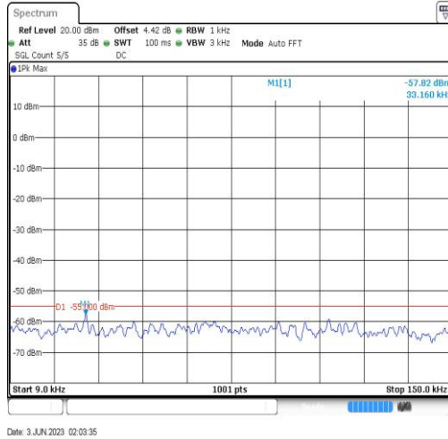
Band38-20MHz-QPSK-38150-1RB#0-Range1:0.009~0.15MHz
