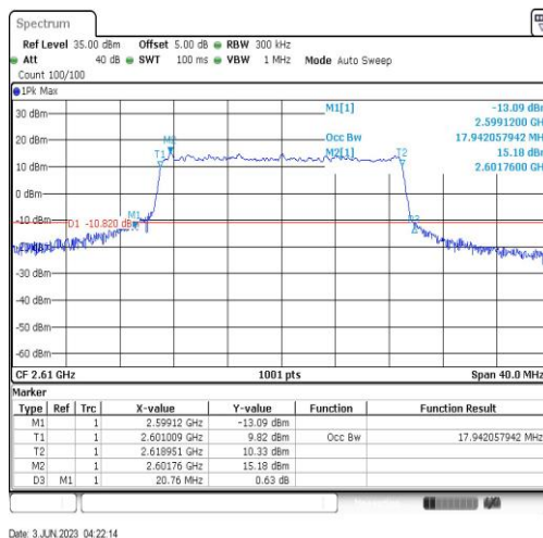
Band38-20MHz-64QAM-38150-100RB#0-17.942
