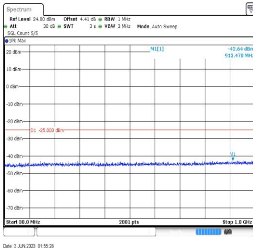
Band38-20MHz-QPSK-37850-1RB#0-Range3:30~1000MHz
