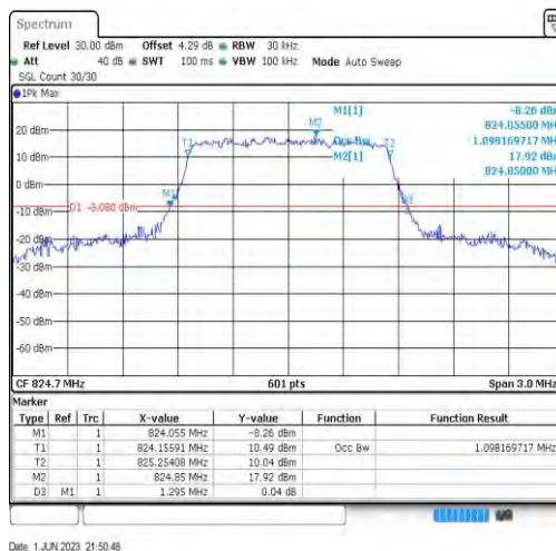
Band26-1.4MHz-16QAM-26797-6RB#0-1.098
