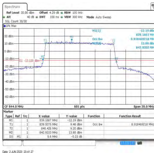
Band26-10MHz-64QAM-26990-50RB#0-8.918
