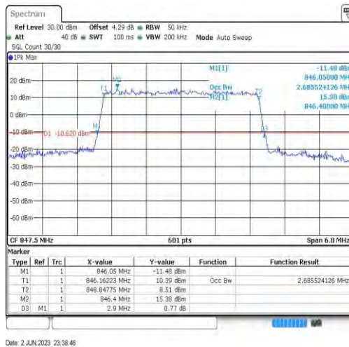
Band26-3MHz-64QAM-27025-15RB#0-2.686
