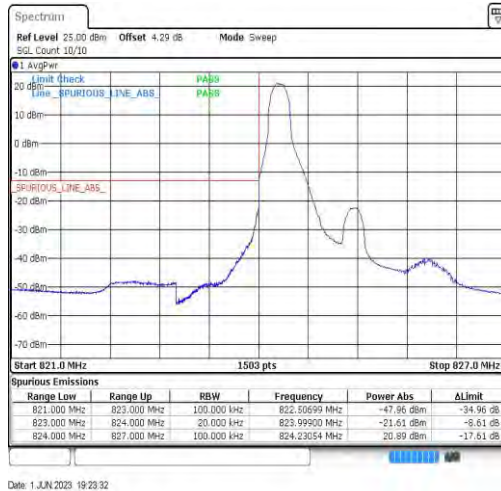
Band26-1.4MHz-16QAM-26797-1RB#0
