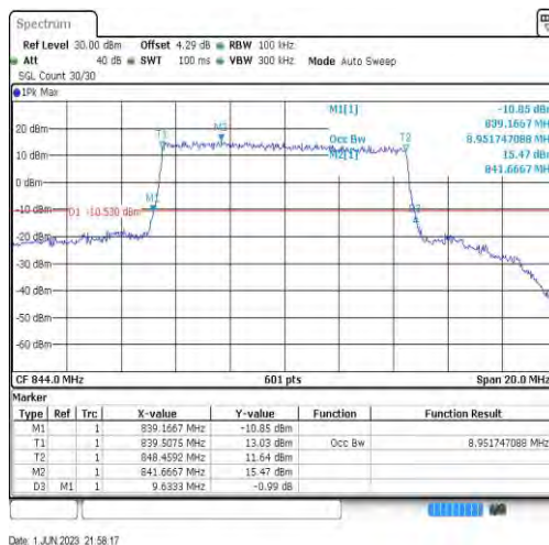
Band26-10MHz-QPSK-26990-50RB#0-8.952
