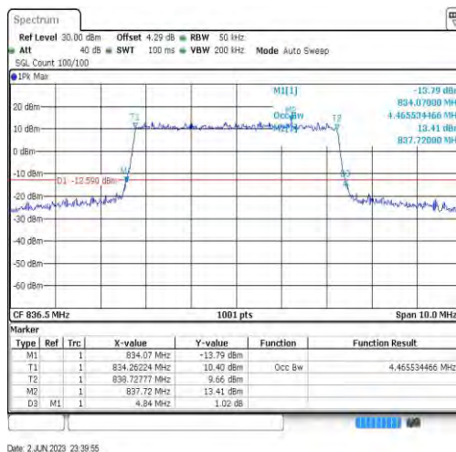
Band26-5MHz-64QAM-26915-25RB#0-4.466
