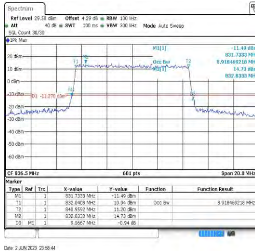
Band26-10MHz-16QAM-26915-50RB#0-8.918
