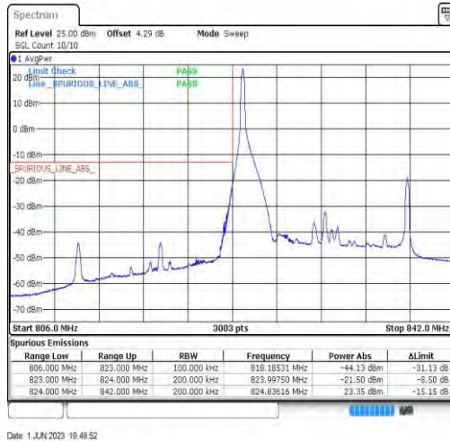
Band26-15MHz-16QAM-26865-1RB#0
