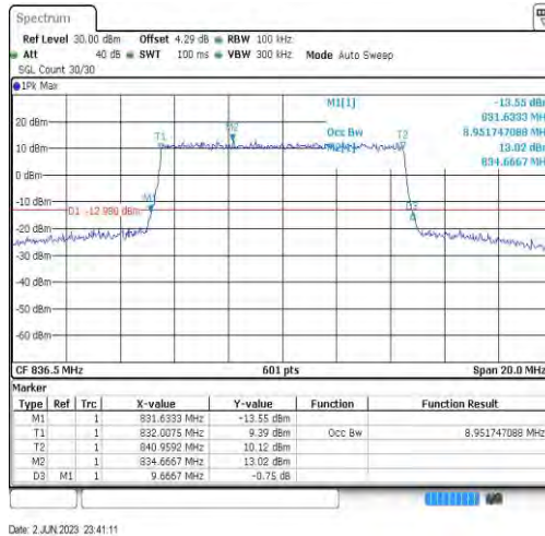
Band26-10MHz-64QAM-26915-50RB#0-8.952
