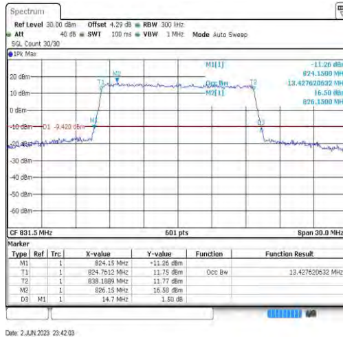
Band26-15MHz-64QAM-26865-75RB#0-13.428
