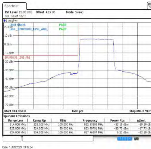
Band26-5MHz-16QAM-26815-25RB#0
