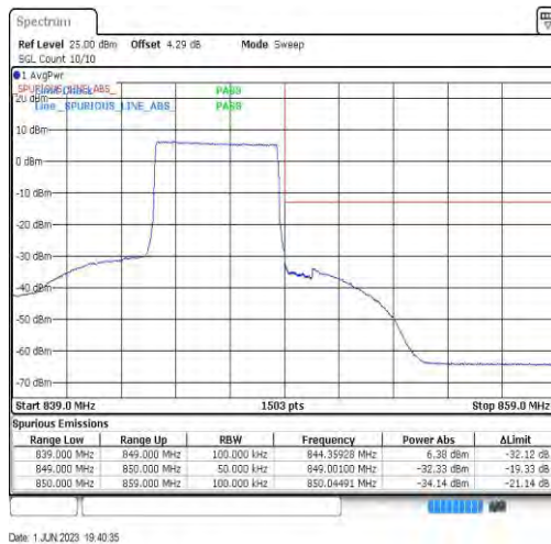
Band26-5MHz-16QAM-27015-25RB#0
