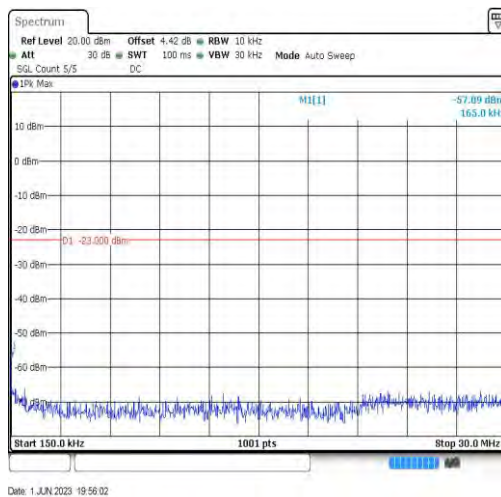
Band26-15MHz-QPSK-26915-1RB#0-Range2:0.15~30MHz
