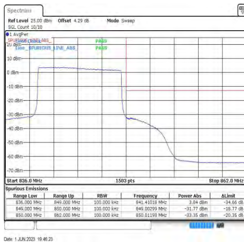
Band26-10MHz-16QAM-26990-50RB#0
