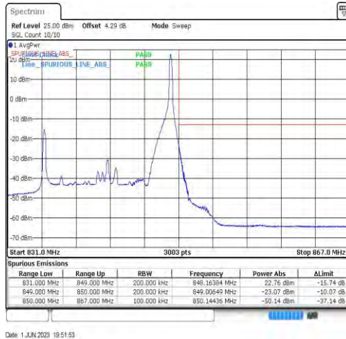
Band26-15MHz-16QAM-26965-1RB#74
