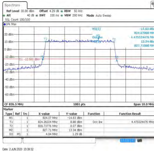
Band26-5MHz-64QAM-26815-25RB#0-4.476
