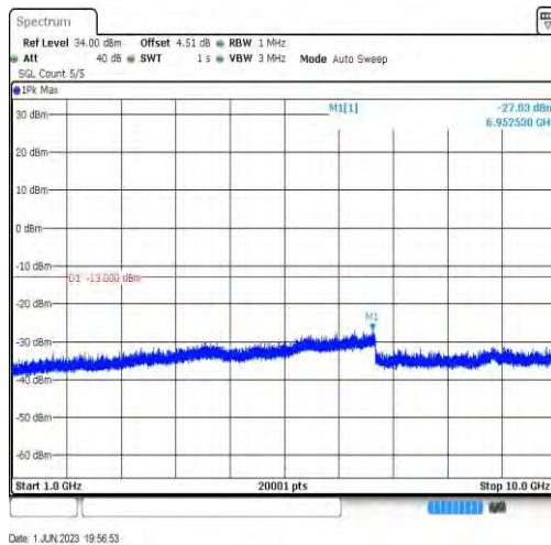
Band26-15MHz-QPSK-26965-1RB#0-Range4:1000~10000MHz
