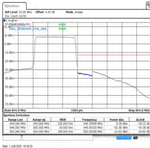
Band26-3MHz-16QAM-27025-15RB#0
