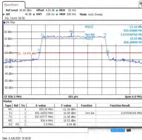
Band26-3MHz-64QAM-26915-15RB#0-2.676
