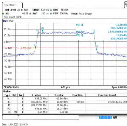
Band26-3MHz-16QAM-26915-15RB#0-2.676
