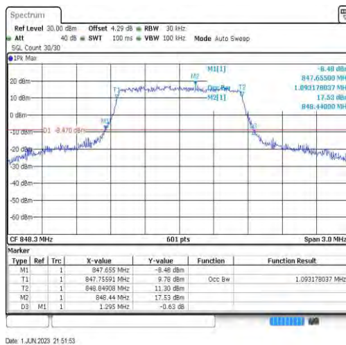
Band26-1.4MHz-16QAM-27033-6RB#0-1.093
