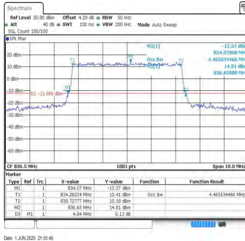
Band26-5MHz-16QAM-26915-25RB#0-4.466
