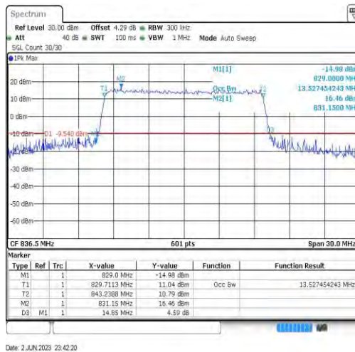
Band26-15MHz-64QAM-26915-75RB#0-13.527
