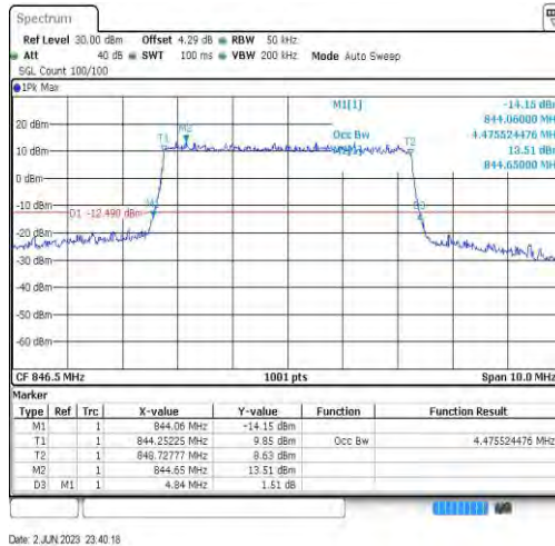
Band26-5MHz-64QAM-27015-25RB#0-4.476
