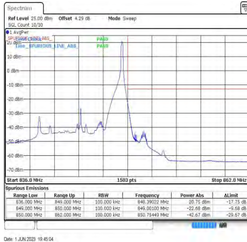
Band26-10MHz-16QAM-26990-1RB#49
