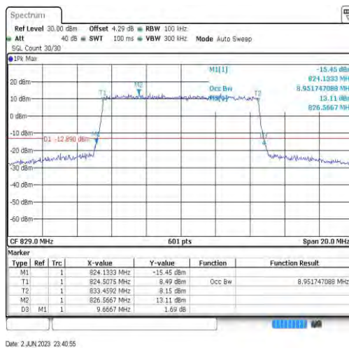
Band26-10MHz-64QAM-26840-50RB#0-8.952
