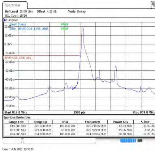
Band26-5MHz-16QAM-26815-1RB#0
