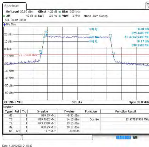
Band26-15MHz-QPSK-26915-75RB#0-13.478
