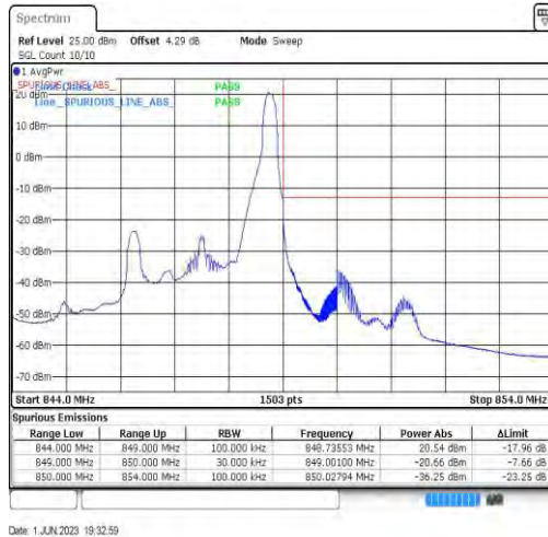
Band26-3MHz-16QAM-27025-1RB#14
