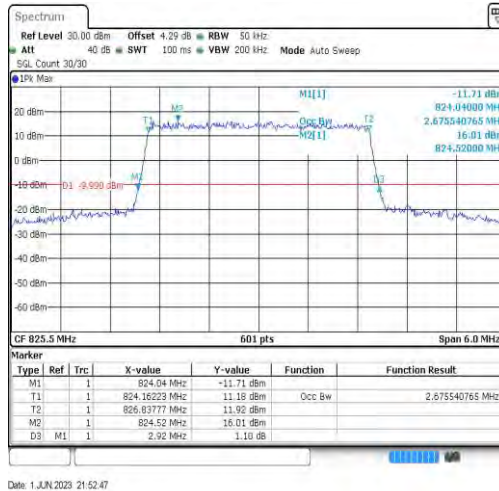
Band26-3MHz-16QAM-26805-15RB#0-2.676
