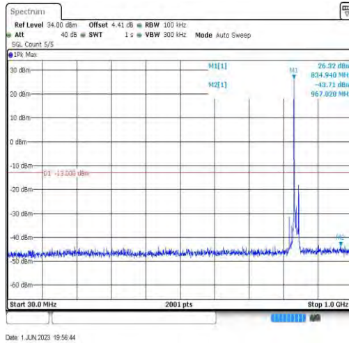
Band26-15MHz-QPSK-26965-1RB#0-Range3:30~1000MHz
