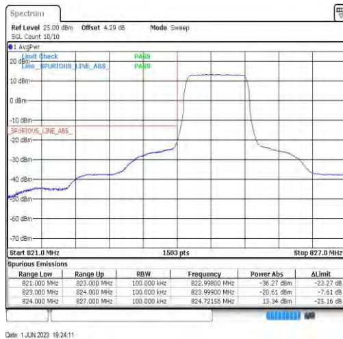
Band26-1.4MHz-QPSK-26797-6RB#0
