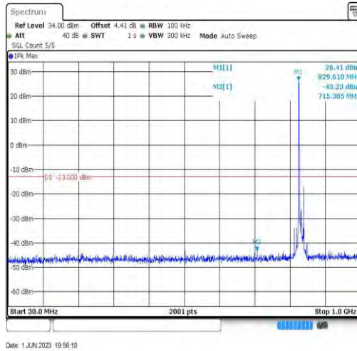
Band26-15MHz-QPSK-26915-1RB#0-Range3:30~1000MHz
