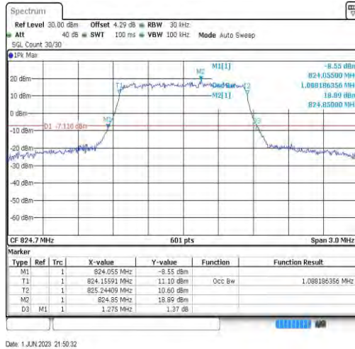
Band26-1.4MHz-QPSK-26797-6RB#0-1.088
