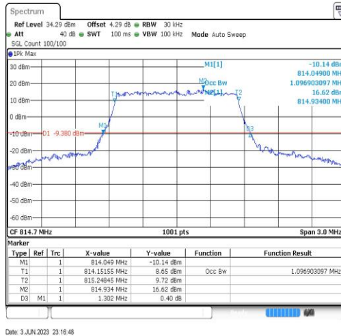
Band26-1.4MHz-64QAM-26697-6RB#0-1.097
