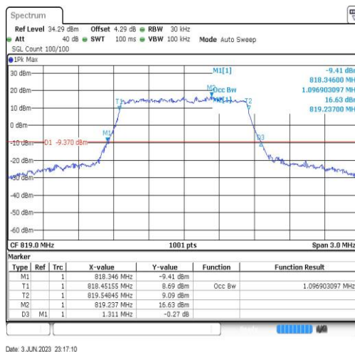
Band26-1.4MHz-64QAM-26740-6RB#0-1.097
