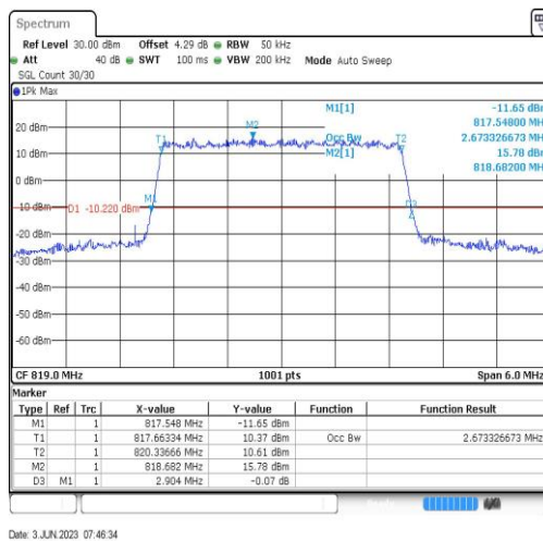
Band26-3MHz-16QAM-26740-15RB#0-2.673
