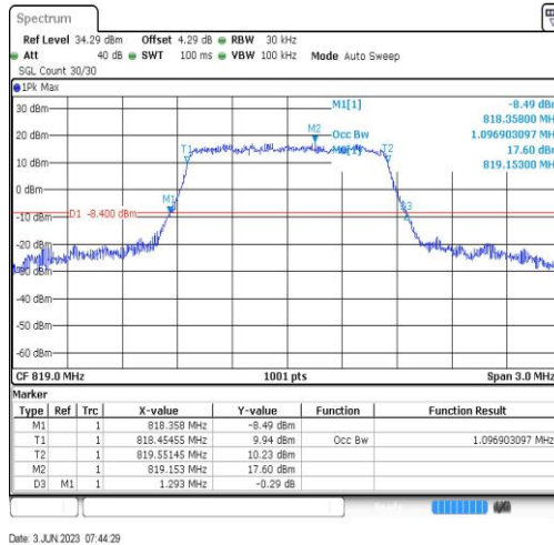
Band26-1.4MHz-16QAM-26740-6RB#0-1.097
