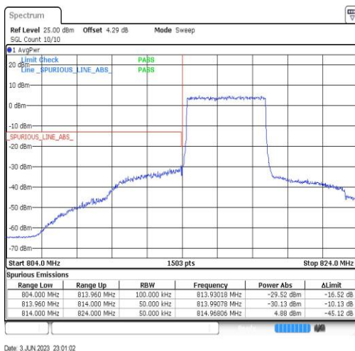
Band26-5MHz-QPSK-26715-25RB#0
