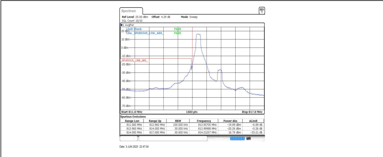
Band26-1.4MHz-QPSK-26697-1RB#0
