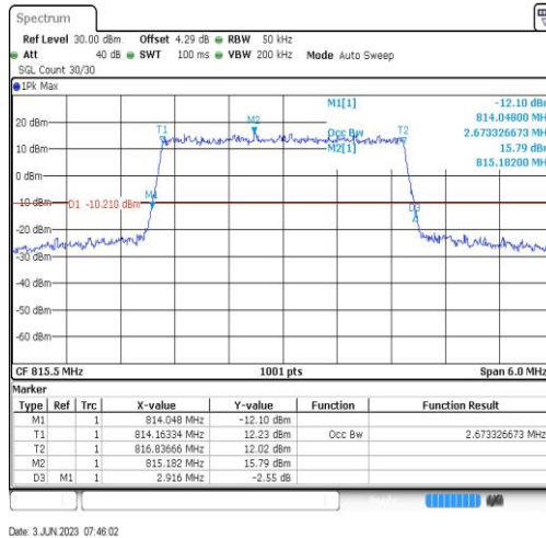
Band26-3MHz-16QAM-26705-15RB#0-2.673
