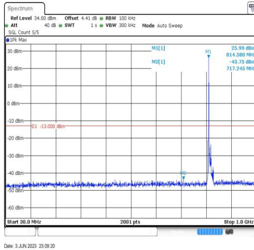
Band26-10MHz-QPSK-26740-1RB#0-Range3:30~1000MHz
