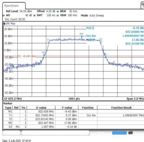
Band26-1.4MHz-16QAM-26783-6RB#0-1.097
