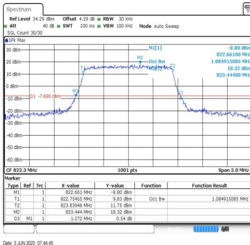
Band26-1.4MHz-QPSK-26783-6RB#0-1.085
