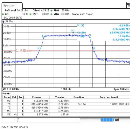
Band26-1.4MHz-QPSK-26740-6RB#0-1.088
