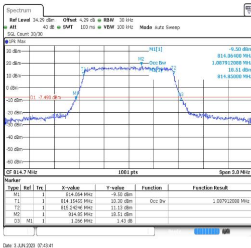
Band26-1.4MHz-QPSK-26697-6RB#0-1.088
