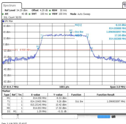
Band26-1.4MHz-16QAM-26697-6RB#0-1.097
