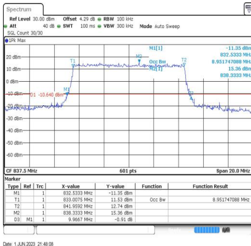
Band19-10MHz-QPSK-24075-50RB#0-8.952
