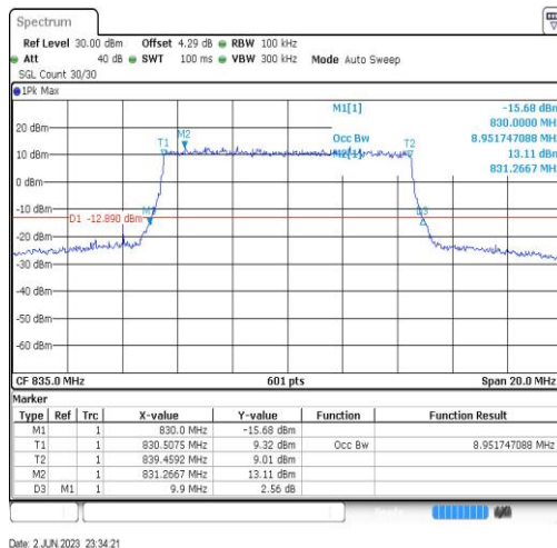
Band19-10MHz-64QAM-24050-50RB#0-8.952
