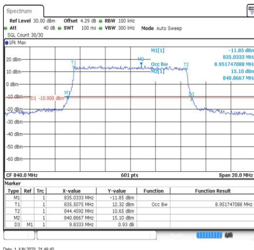
Band19-10MHz-QPSK-24100-50RB#0-8.952
