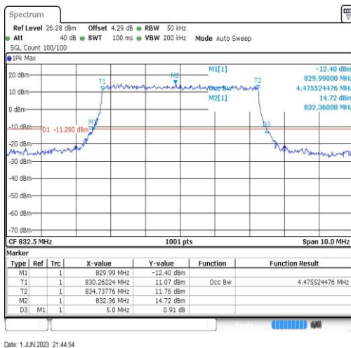
Band19-5MHz-QPSK-24025-25RB#0-4.476
