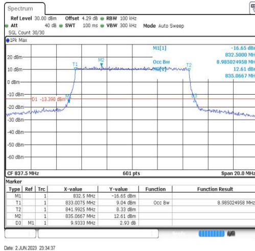
Band19-10MHz-64QAM-24075-50RB#0-8.985
