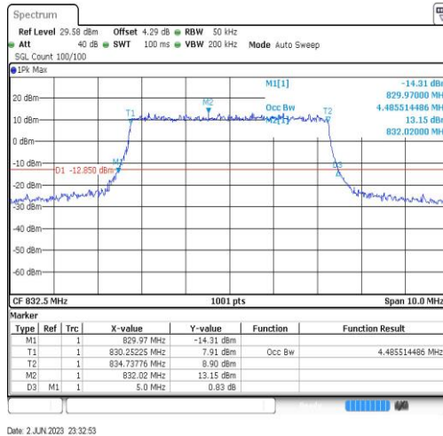
Band19-5MHz-64QAM-24025-25RB#0-4.486
