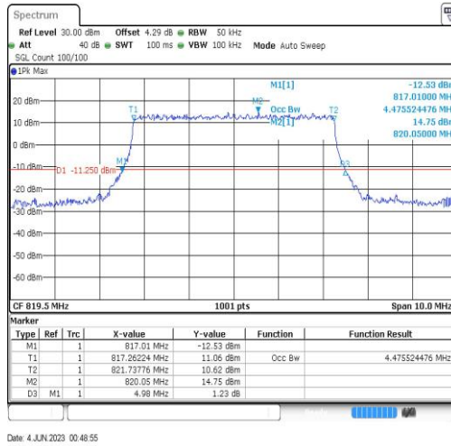
18(815-824)-5MHz-QPSK-23895-25RB#0
