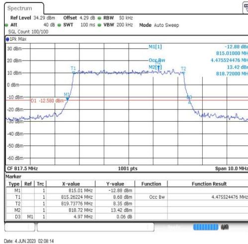
18(815-824)-5MHz-64QAM-23875-25RB#0-4.476
