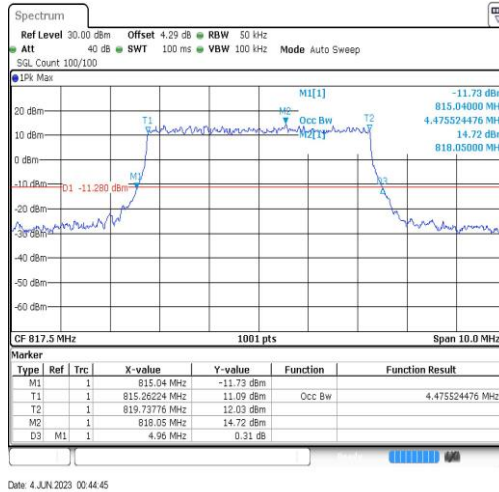
18(815-824)-5MHz-QPSK-23875-25RB#0
