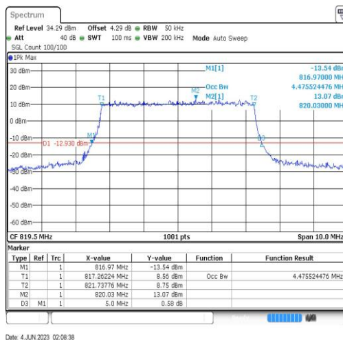
18(815-824)-5MHz-64QAM-23895-25RB#0-4.476
