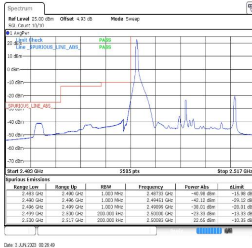
Band7-15MHz-QPSK-20825-1RB#0
