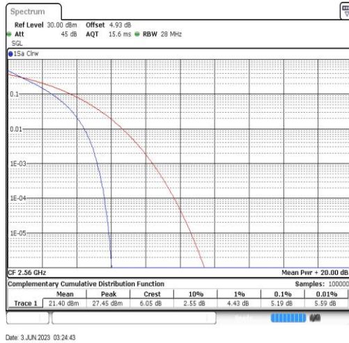
Band7-20MHz-QPSK-21350-100RB#0
