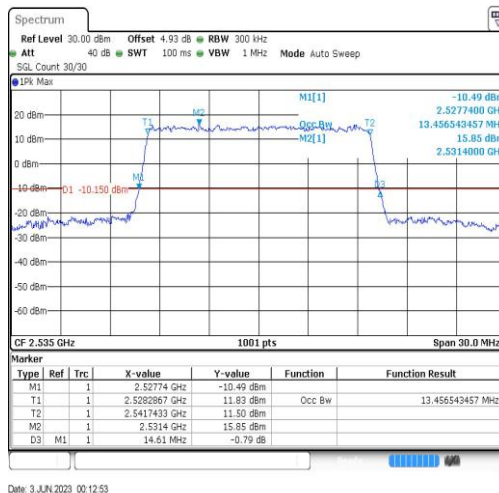
Band7-15MHz-QPSK-21100-75RB#0-13.457
