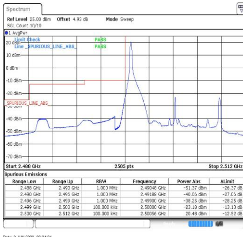
Band7-10MHz-QPSK-20800-1RB#0
