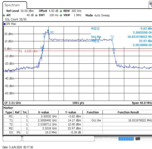
Band7-20MHz-16QAM-20850-100RB#0-18.022
