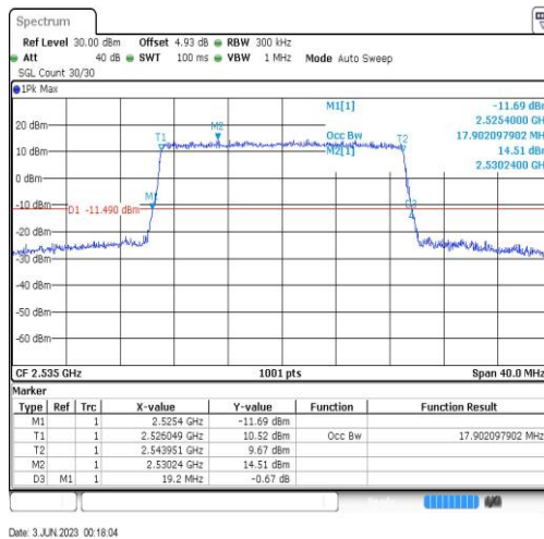
Band7-20MHz-16QAM-21100-100RB#0-17.902
