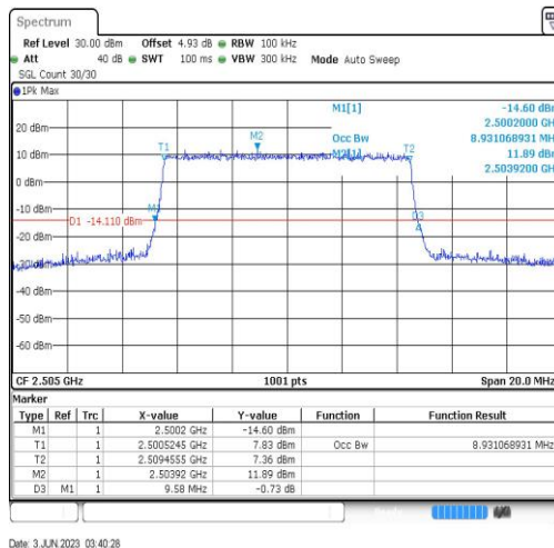
Band7-10MHz-64QAM-20800-50RB#0-8.931
