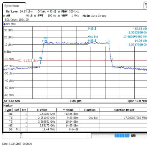
Band7-20MHz-64QAM-21350-100RB#0-17.902
