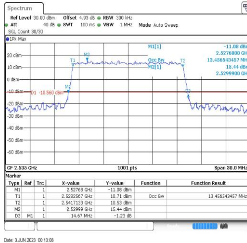
Band7-15MHz-16QAM-21100-75RB#0-13.457
