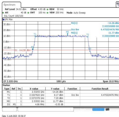
Band7-5MHz-64QAM-21100-25RB#0-4.476
