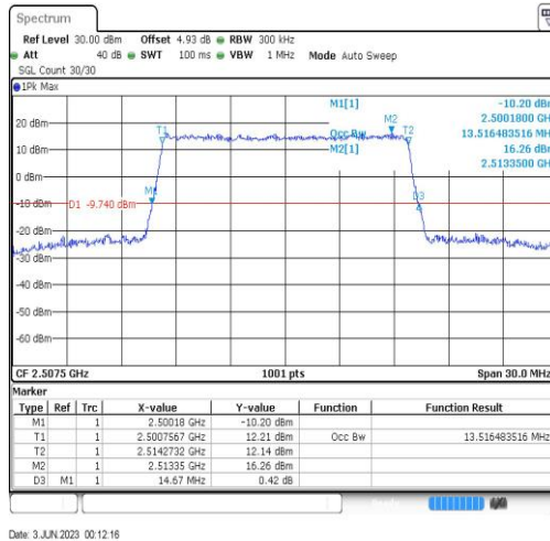
Band7-15MHz-QPSK-20825-75RB#0-13.516
