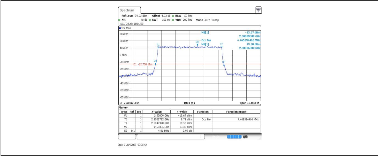
Band7-5MHz-QPSK-20775-25RB#0-4.466
