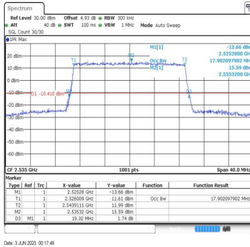
Band7-20MHz-QPSK-21100-100RB#0-17.902
