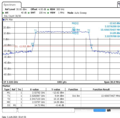
Band7-15MHz-64QAM-21100-75RB#0-13.427
