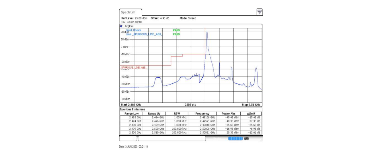
Band7-5MHz-QPSK-20775-1RB#0
