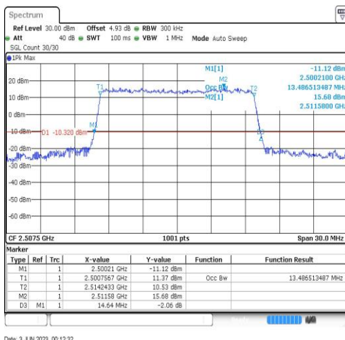
Band7-15MHz-16QAM-20825-75RB#0-13.487
