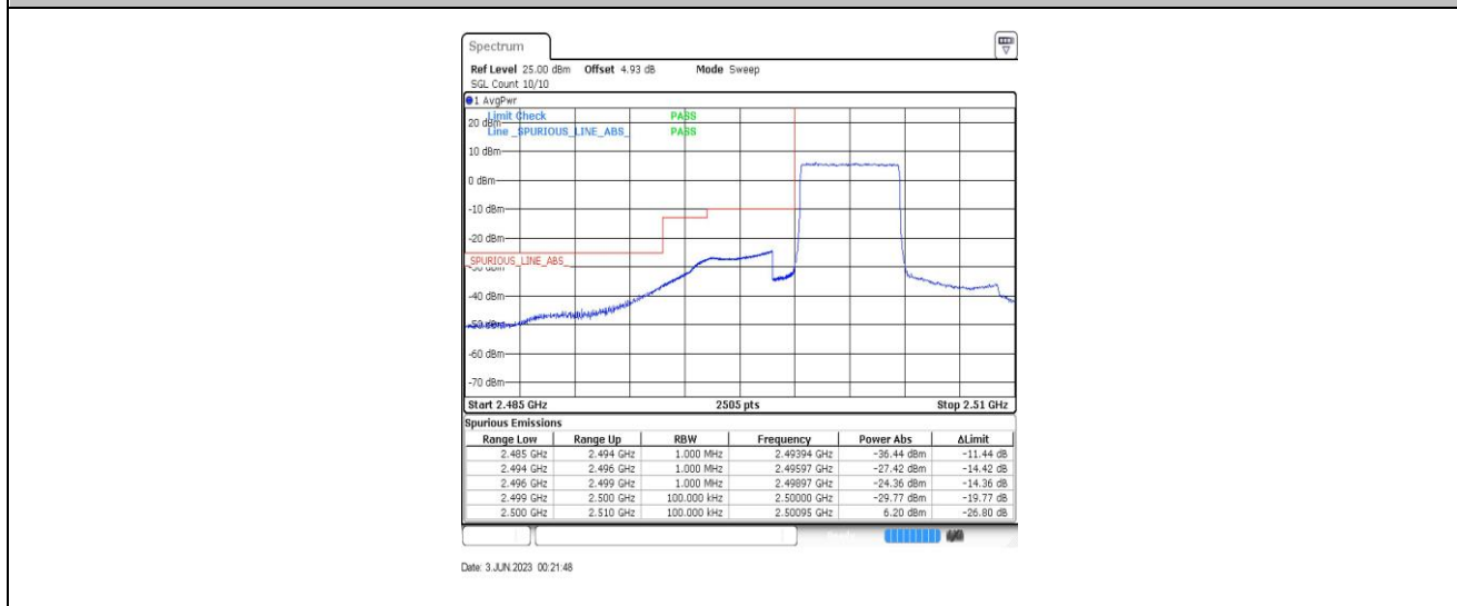
Band7-5MHz-QPSK-20775-25RB#0
