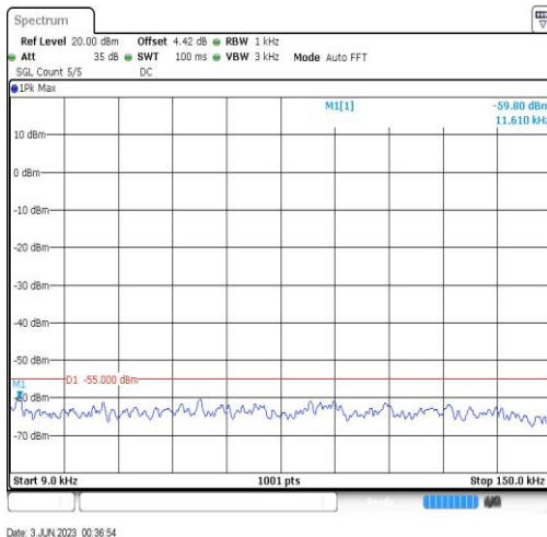
Band7-20MHz-QPSK-21350-1RB#0-Range1:0.009~0.15MHz
