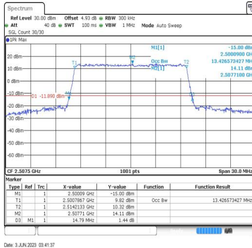
Band7-15MHz-64QAM-20825-75RB#0-13.427
