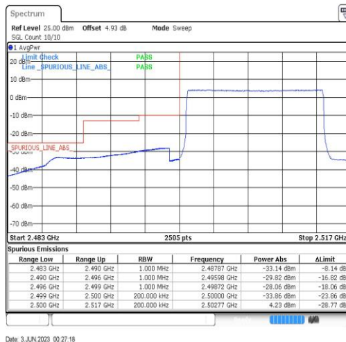
Band7-15MHz-QPSK-20825-75RB#0
