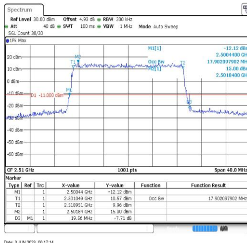
Band7-20MHz-QPSK-20850-100RB#0-17.902
