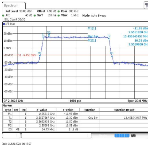
Band7-15MHz-QPSK-21375-75RB#0-13.457
