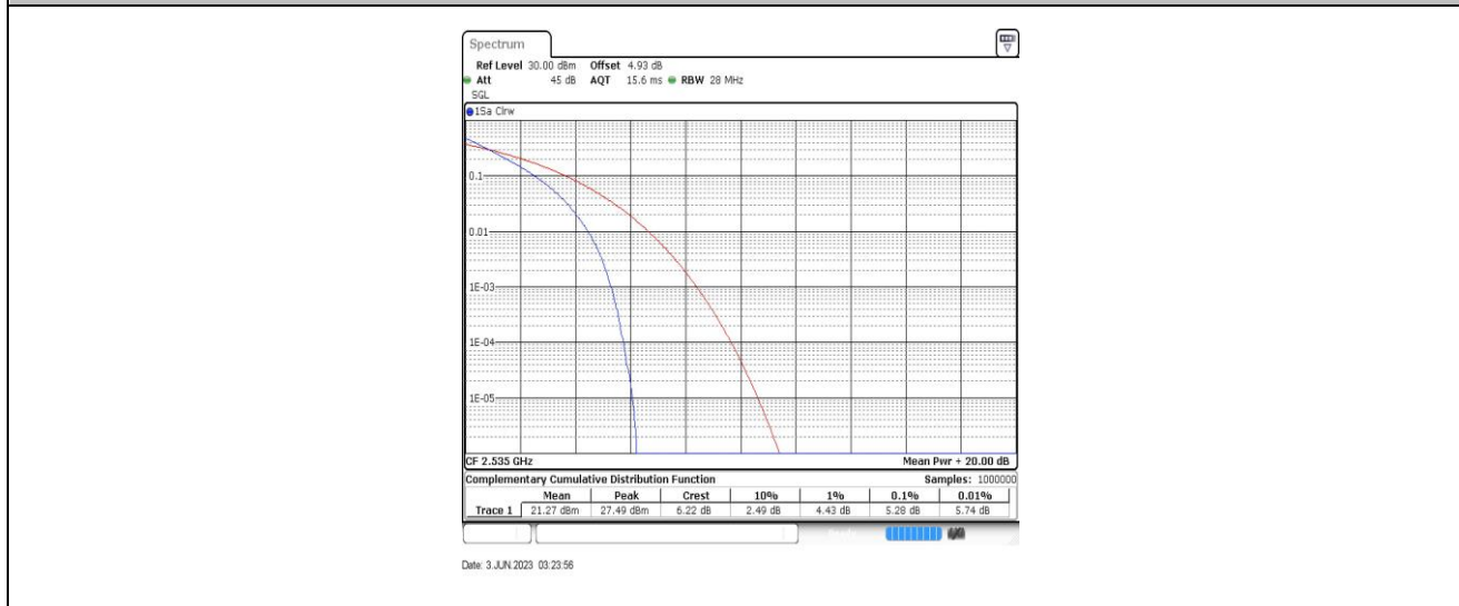
Band7-20MHz-QPSK-21100-100RB#0
