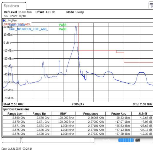
Band7-5MHz-QPSK-21425-1RB#24
