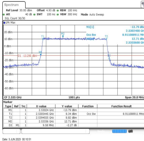
Band7-10MHz-16QAM-21100-50RB#0-8.911
