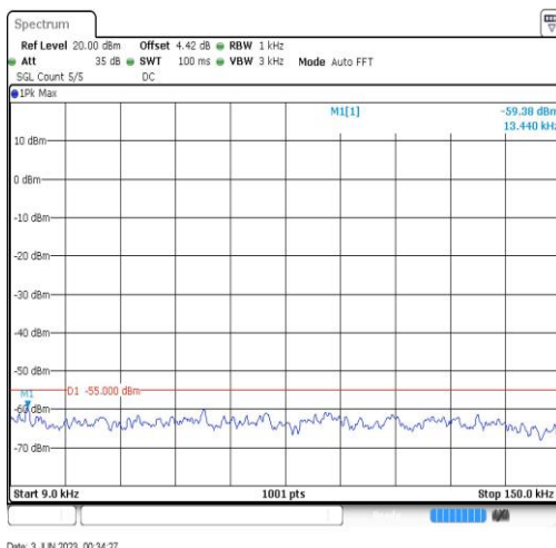
Band7-20MHz-QPSK-21100-1RB#0-Range1:0.009~0.15MHz
