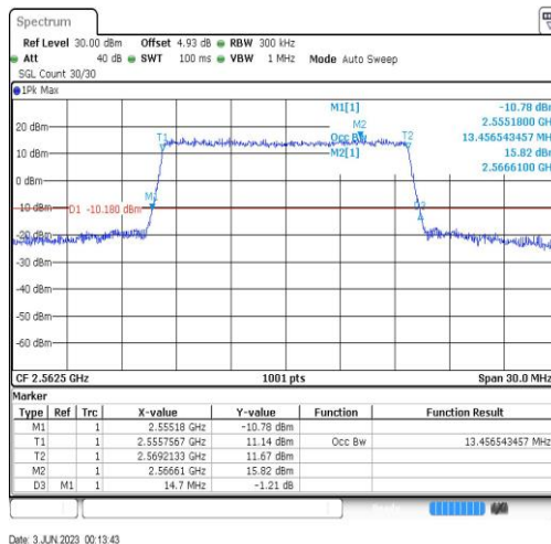
Band7-15MHz-16QAM-21375-75RB#0-13.457
