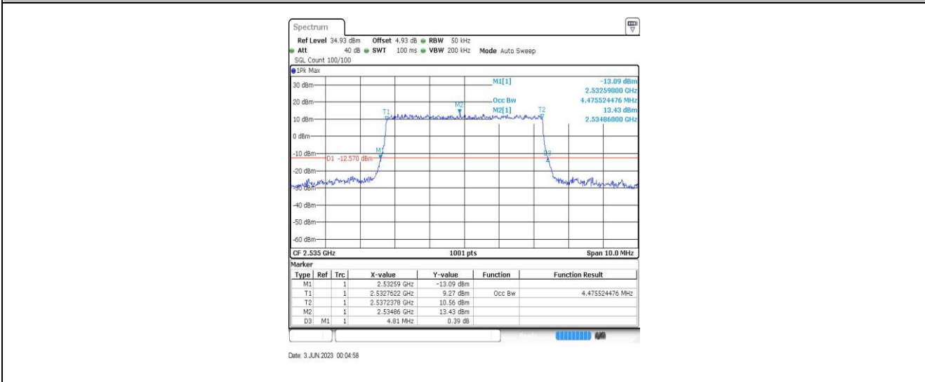
Band7-5MHz-QPSK-21100-25RB#0-4.476
