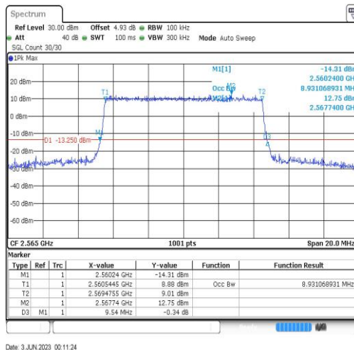
Band7-10MHz-16QAM-21400-50RB#0-8.931
