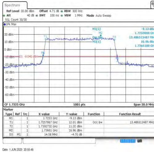
Band4-15MHz-16QAM-20175-75RB#0-13.487
