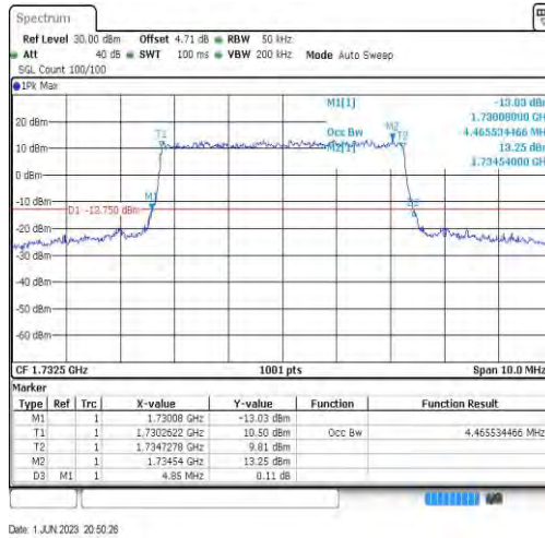
Band4-5MHz-16QAM-20175-25RB#0-4.466
