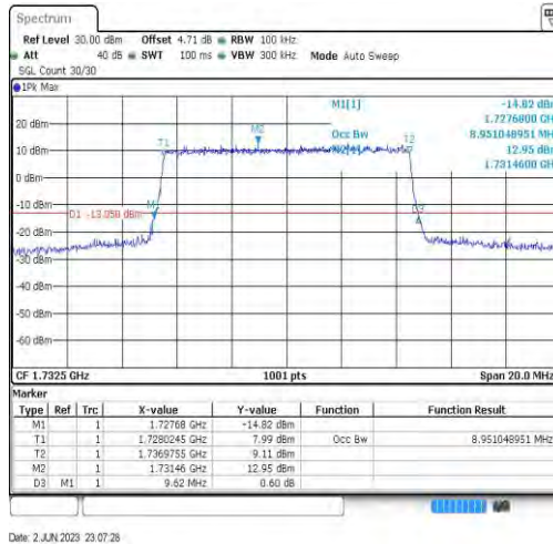
Band4-10MHz-64QAM-20175-50RB#0-8.951
