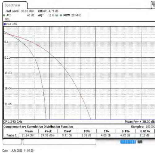
Band4-20MHz-QPSK-20300-100RB#0
