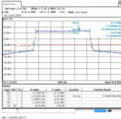
Band4-20MHz-16QAM-20050-100RB#0-17.942
