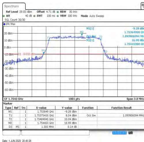
Band4-1.4MHz-16QAM-20393-6RB#0-1.094
