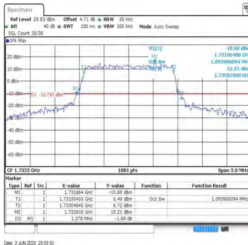
Band4-1.4MHz-64QAM-20175-6RB#0-1.094
