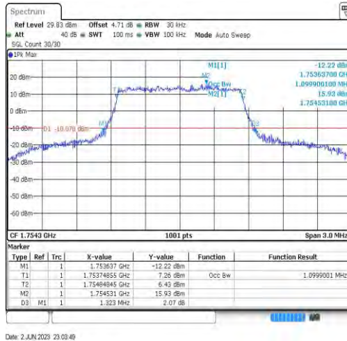
Band4-1.4MHz-64QAM-20393-6RB#0-1.1
