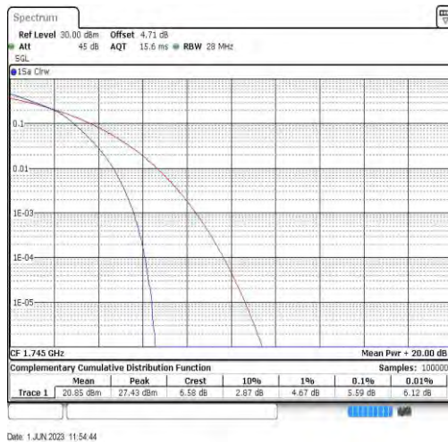
Band4-20MHz-16QAM-20300-100RB#0
