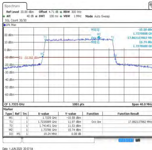
Band4-20MHz-16QAM-20175-100RB#0-17.862
