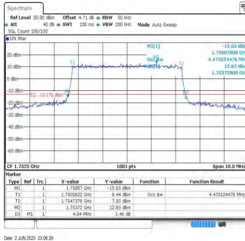
Band4-5MHz-64QAM-20375-25RB#0-4.476
