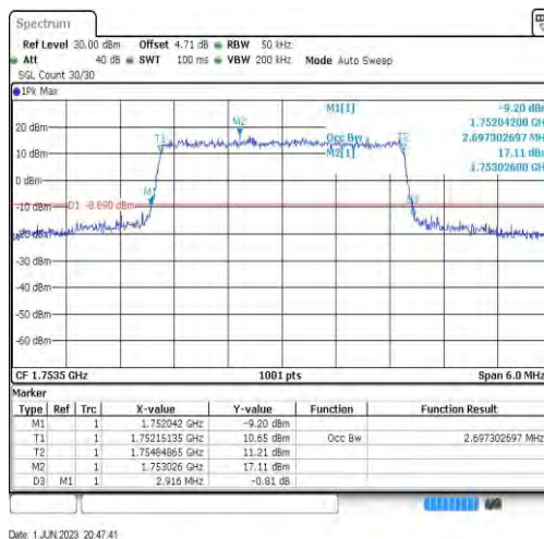
Band4-3MHz-QPSK-20385-15RB#0-2.697
