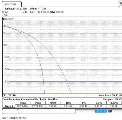
Band4-20MHz-64QAM-20050-100RB#0
