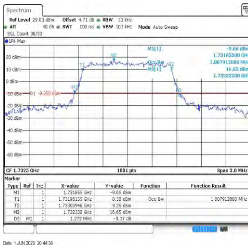
Band4-1.4MHz-QPSK-20175-6RB#0-1.088
