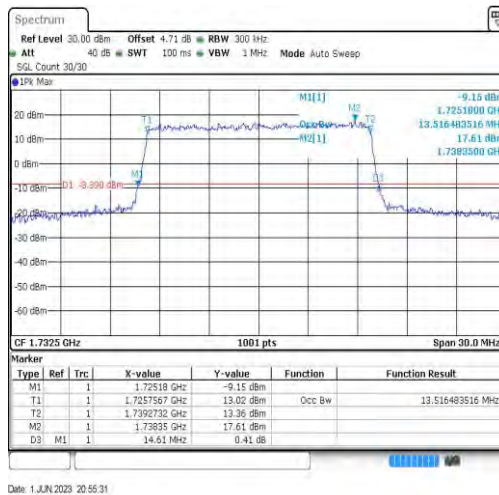
Band4-15MHz-QPSK-20175-75RB#0-13.516
