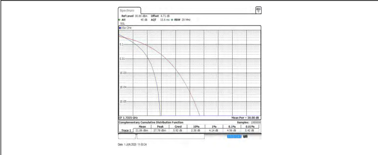
Band4-20MHz-QPSK-20175-100RB#0
