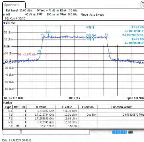
Band4-3MHz-16QAM-19965-15RB#0-2.679
