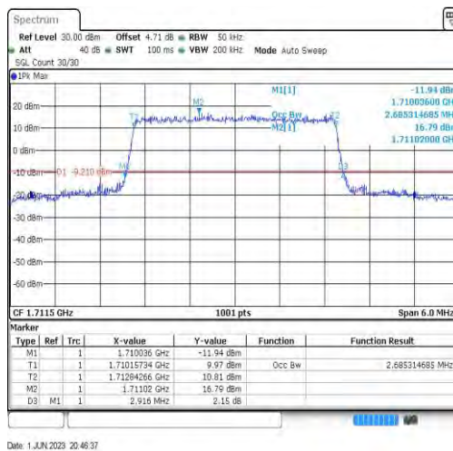
Band4-3MHz-QPSK-19965-15RB#0-2.685
