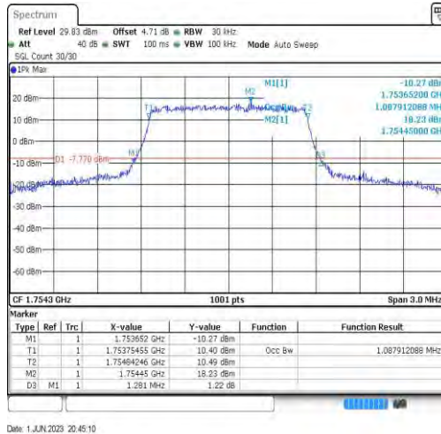
Band4-1.4MHz-QPSK-20393-6RB#0-1.088
