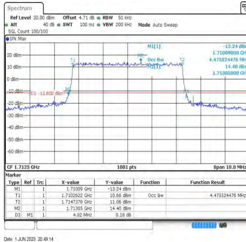
Band4-5MHz-QPSK-19975-25RB#0-4.476
