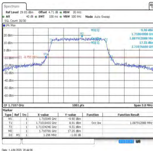
Band4-1.4MHz-QPSK-19957-6RB#0-1.088
