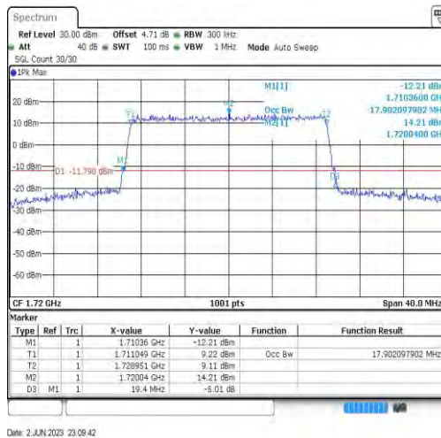
Band4-20MHz-64QAM-20050-100RB#0-17.902
