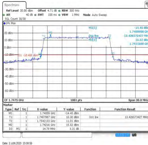
Band4-15MHz-64QAM-20325-75RB#0-13.427
