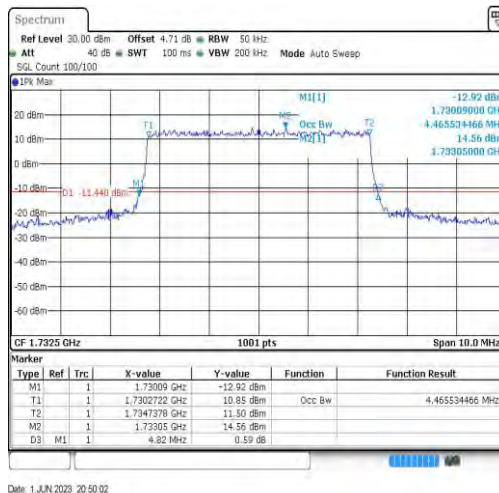
Band4-5MHz-QPSK-20175-25RB#0-4.466
