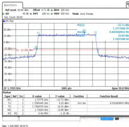
Band4-10MHz-16QAM-20175-50RB#0-8.931
