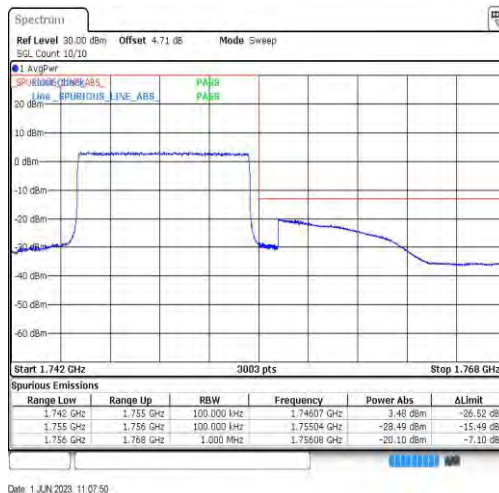
Band4-10MHz-QPSK-20350-50RB#0
