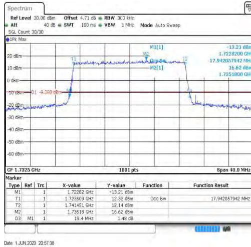
Band4-20MHz-QPSK-20175-100RB#0-17.942
