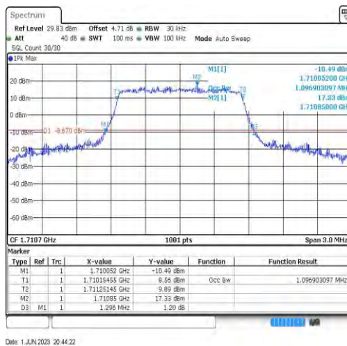
Band4-1.4MHz-16QAM-19957-6RB#0-1.097
