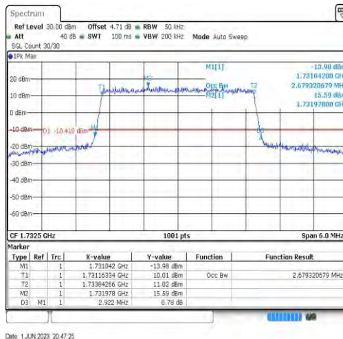
Band4-3MHz-16QAM-20175-15RB#0-2.679
