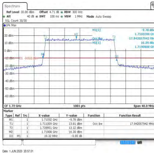
Band4-20MHz-QPSK-20050-100RB#0-17.942
