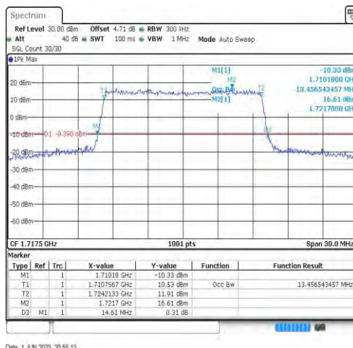
Band4-15MHz-16QAM-20025-75RB#0-13.457
