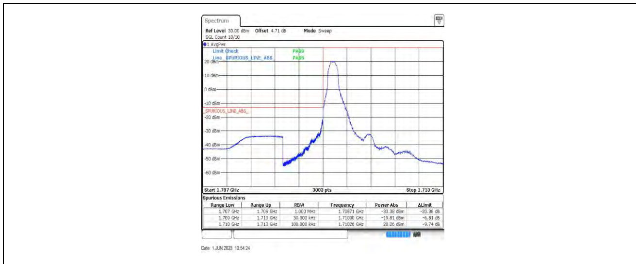
Band4-1.4MHz-QPSK-19957-1RB#0
