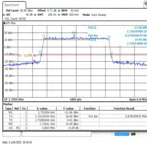
Band4-3MHz-64QAM-20175-15RB#0-2.679
