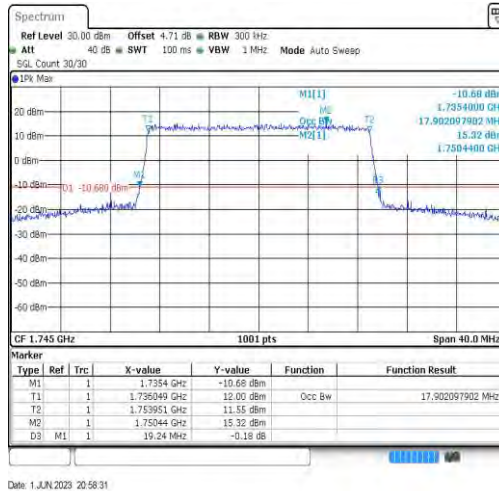
Band4-20MHz-16QAM-20300-100RB#0-17.902
