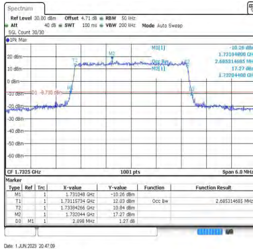
Band4-3MHz-QPSK-20175-15RB#0-2.685
