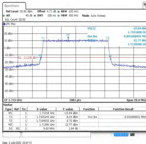
Band4-10MHz-64QAM-20000-50RB#0-8.931
