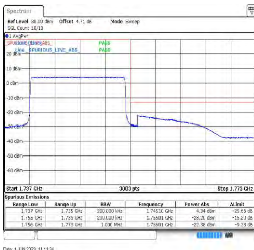
Band4-15MHz-QPSK-20325-75RB#0
