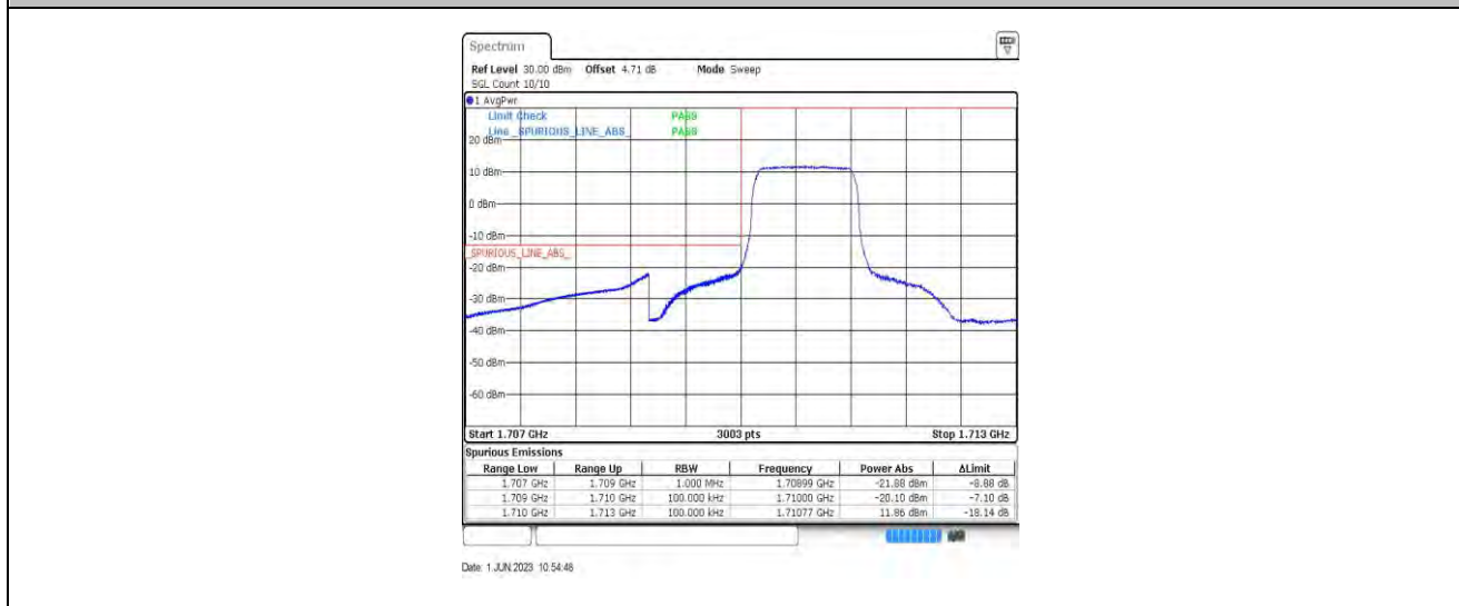
Band4-1.4MHz-QPSK-19957-6RB#0
