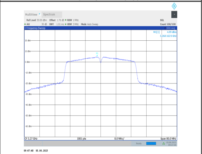
11n40SISO-Ant22-5270
