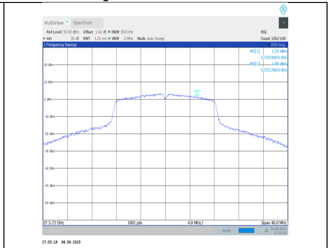
11a-Ant22-5720 UNII-3
