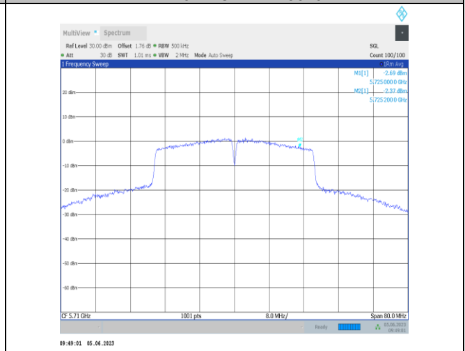
11n40SISO-Ant22-5710 UNII-3
