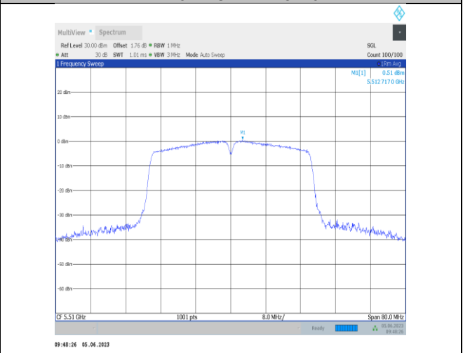
11n40SISO-Ant22-5510
