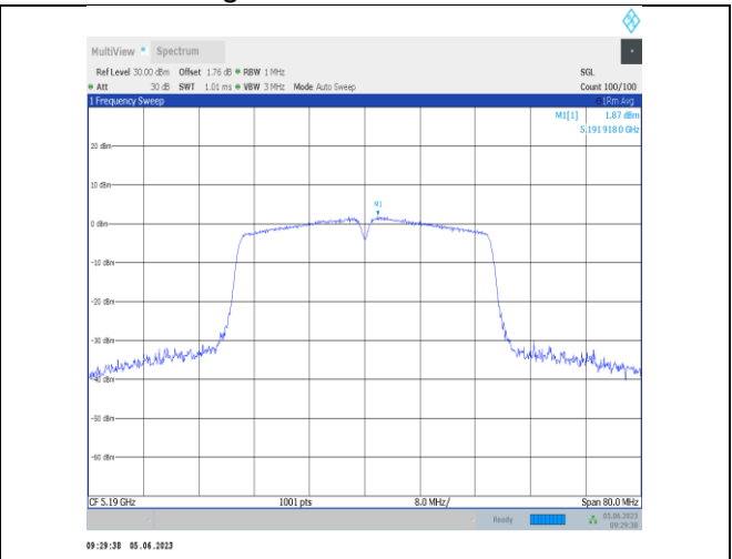
11n40SISO-Ant22-5190
