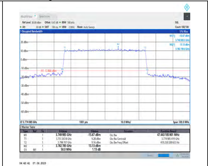
1-N78-3700-3800-PC3-30-50-H-6-CP-QPSK-Outer Full-133@0-Ant1-47.443-50.000-≤50-PASS
