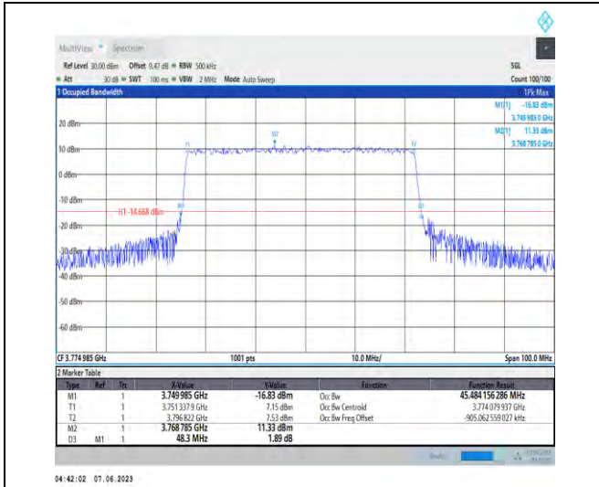
1-N78-3700-3800-PC3-30-50-H-5-DFT-256QAM-Out er_Full-128@0-Ant1-45.484-48.300-≤50-PASS
