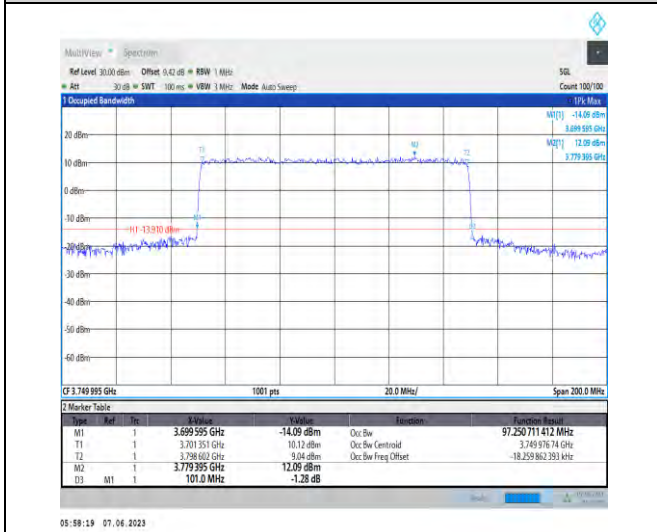
1-N78-3700-3800-PC3-30-100-H-6-CP-QPSK-Outer _Full-273@0-Ant1-97.251-101.000-≤100-PASS
