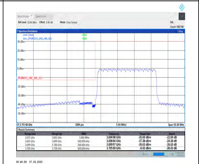
1-N78-3700-3800-PC3-30-20-L-6-CP-QPSK-Outer_Full-51@0-Ant1-1--PASS-see graph
