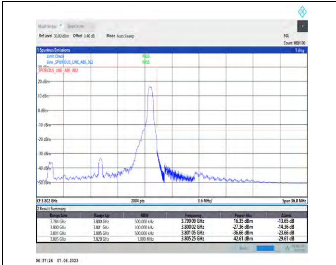
1-N78-3700-3800-PC3-30-15-H-2-DFT-PI2BPSK-Edge_1RB_Right-1@37-Ant1-1--PASS-see graph
