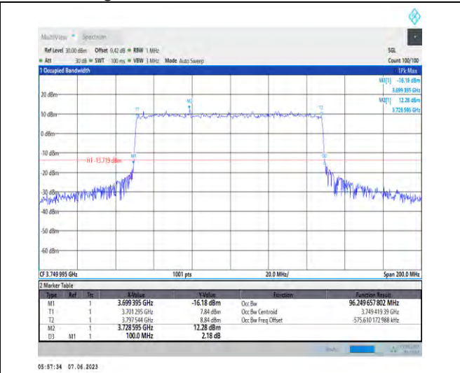
1-N78-3700-3800-PC3-30-100-H-5-DFT-256QAM-O uter_Full-270@0-Ant1-96.25-100.000-≤100-PASS
