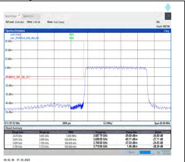
1-N78-3700-3800-PC3-30-25-L-3-DFT-PI2BPSK-Outer_Full-64@0-Ant1-1--PASS-see graph
