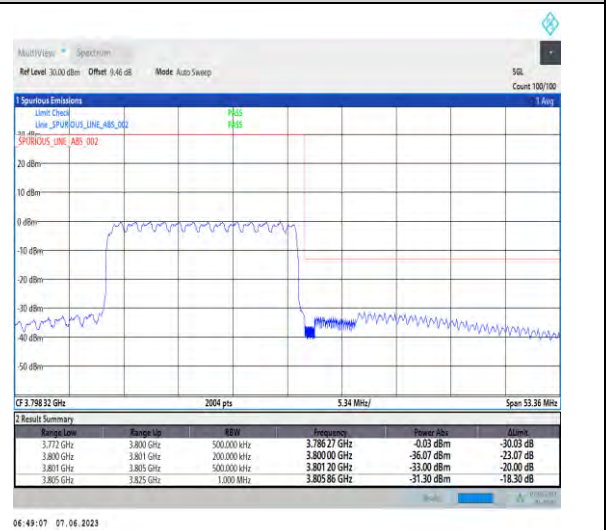
1-N78-3700-3800-PC3-30-20-H-6-CP-QPSK-Outer_Full-51@0-Ant1-1--PASS-see graph
