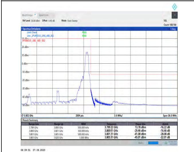
1-N78-3700-3800-PC3-30-15-H-5-CP-QPSK-Edge_1RB_Right-1@37-Ant1-1--PASS-see graph
