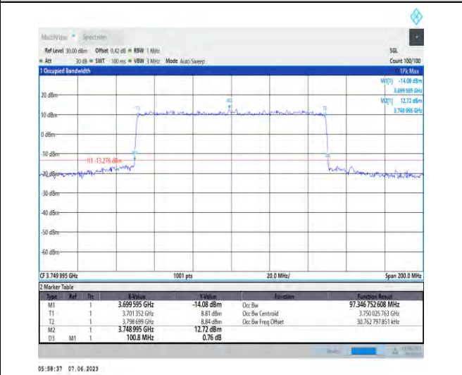
1-N78-3700-3800-PC3-30-100-H-7-CP-16QAM-Outer _Full-273@0-Ant1-97.347-100.800-≤100-PASS
