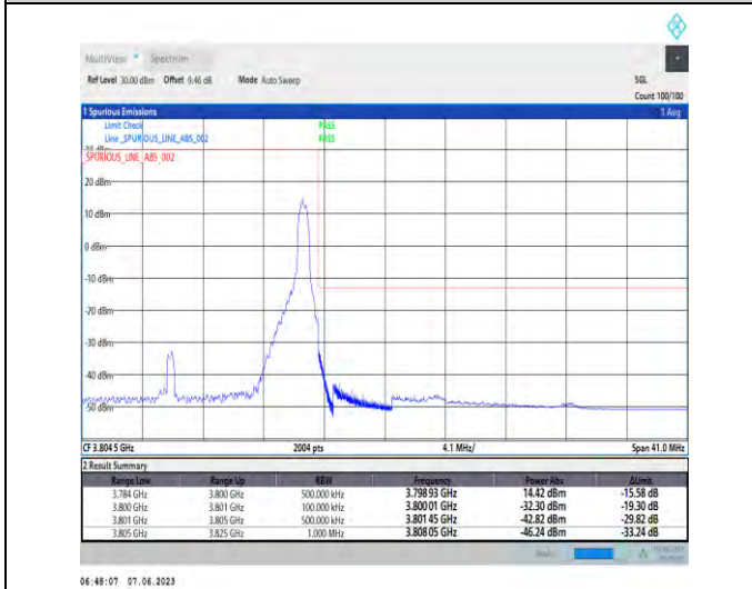
1-N78-3700-3800-PC3-30-20-H-5-CP-QPSK-Edge_1RB_Right-1@50-Ant1-1--PASS-see graph
