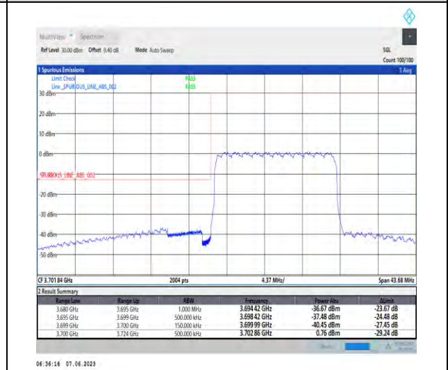
1-N78-3700-3800-PC3-30-15-L-6-CP-QPSK-Outer_Full-38@0-Ant1-1--PASS-see graph
