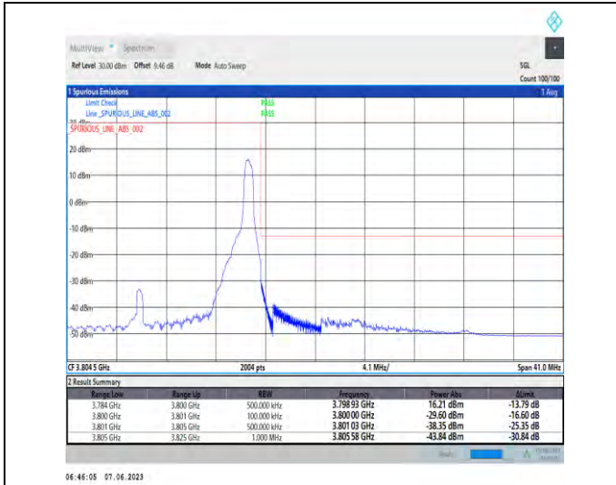
1-N78-3700-3800-PC3-30-20-H-2-DFT-PI2BPSK-Edge_1RB_Right-1@50-Ant1-1--PASS-see graph
