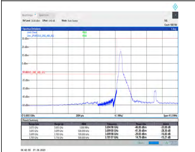
1-N78-3700-3800-PC3-30-20-L-4-CP-QPSK-Edge_1RB_Left-1@0-Ant1-1--PASS-see graph
