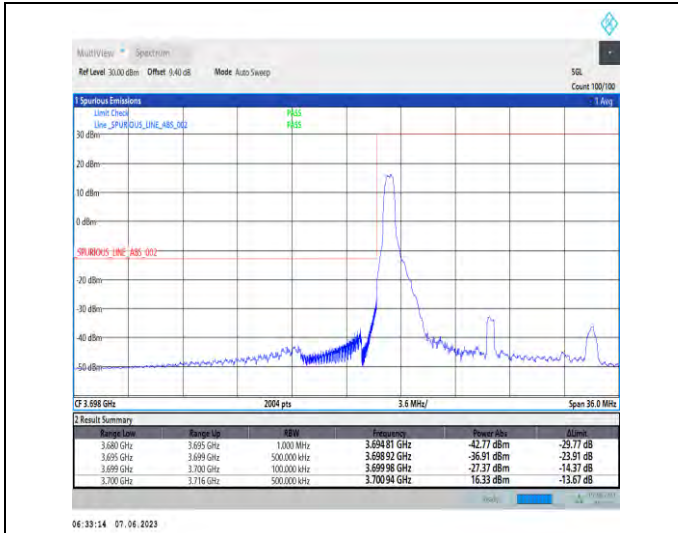
1-N78-3700-3800-PC3-30-15-L-1-DFT-PI2BPSK-Edge_1RB_Left-1@0-Ant1-1--PASS-see graph
