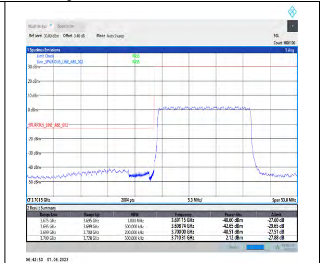
1-N78-3700-3800-PC3-30-20-L-3-DFT-PI2BPSK-Outer_Full-50@0-Ant1-1--PASS-see graph
