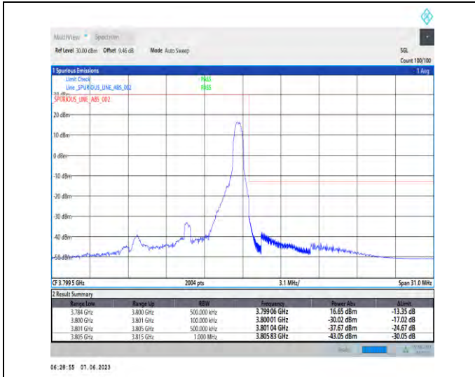
1-N78-3700-3800-PC3-30-10-H-2-DFT-PI2BPSK-Edge_1RB_Right-1@23-Ant1-1--PASS-see graph
