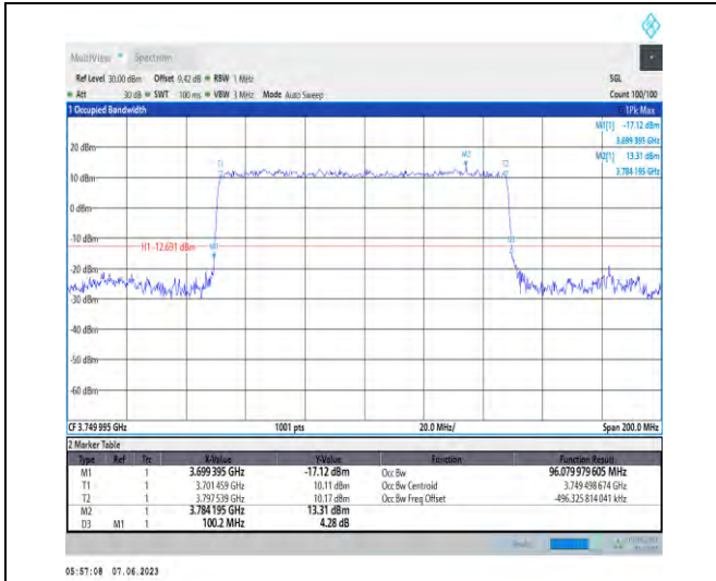
1-N78-3700-3800-PC3-30-100-H-4-DFT-64QAM-Out er_Full-270@0-Ant1-96.08-100.200-≤100-PASS
