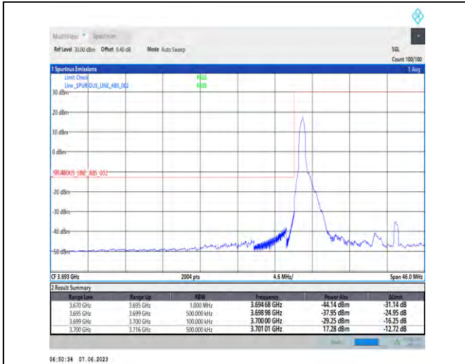
1-N78-3700-3800-PC3-30-25-L-1-DFT-PI2BPSK-Edge_1RB_Left-1@0-Ant1-1--PASS-see graph
