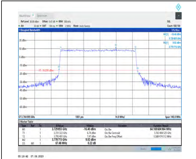
1-N78-3700-3800-PC3-30-70-H-5-DFT-256QAM-Out er_Full-180@0-Ant1-64.17-67.480-≤70-PASS
