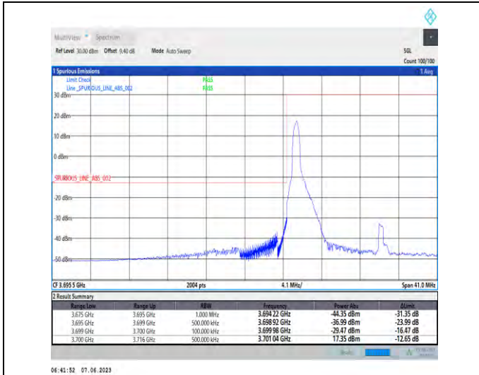
1-N78-3700-3800-PC3-30-20-L-1-DFT-PI2BPSK-Edge_1RB_Left-1@0-Ant1-1--PASS-see graph
