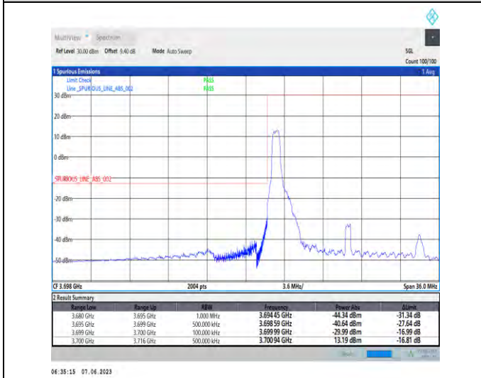
1-N78-3700-3800-PC3-30-15-L-4-CP-QPSK-Edge_1RB_Left-1@0-Ant1-1--PASS-see graph
