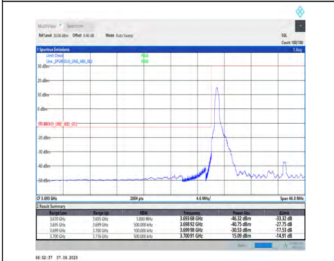
1-N78-3700-3800-PC3-30-25-L-4-CP-QPSK-Edge_1RB_Left-1@0-Ant1-1--PASS-see graph
