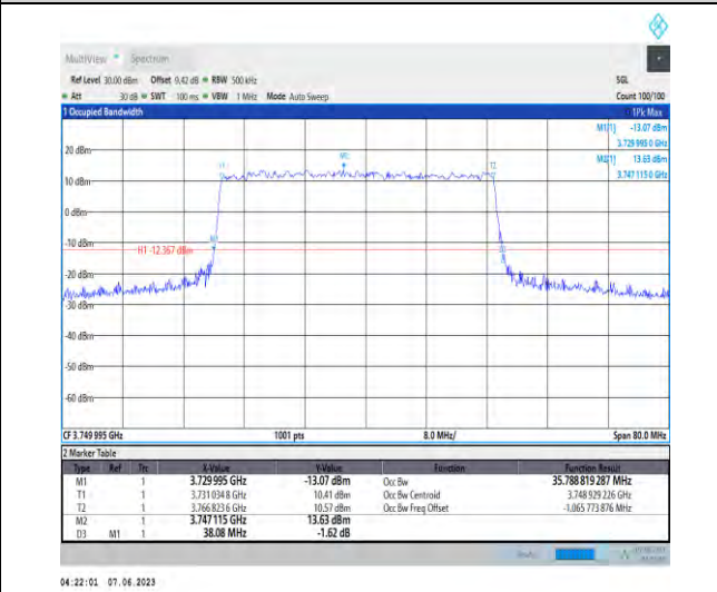
1-N78-3700-3800-PC3-30-40-M-4-DFT-64QAM-Outer_Full-100@0-Ant1-35.789-38.080-≤40-PASS
