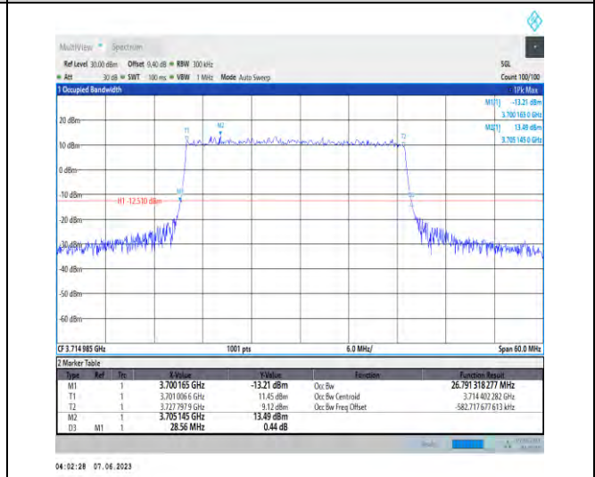
1-N78-3700-3800-PC3-30-30-L-4-DFT-64QAM-Outer_Full-75@0-Ant1-26.791-28.560-≤30-PASS
