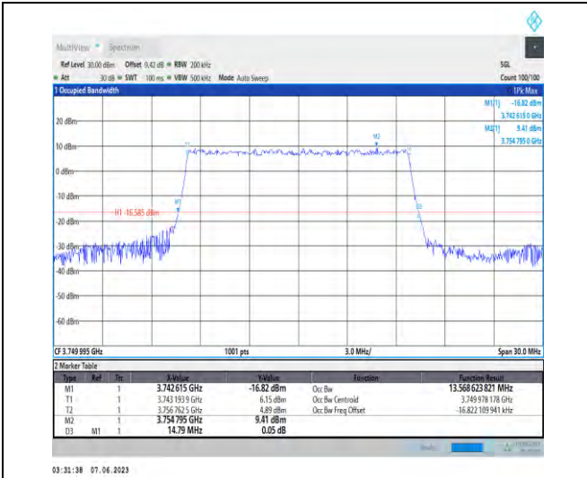
1-N78-3700-3800-PC3-30-15-M-9-CP-256QAM-Out er_Full-38@0-Ant1-13.569-14.790-≤15-PASS
