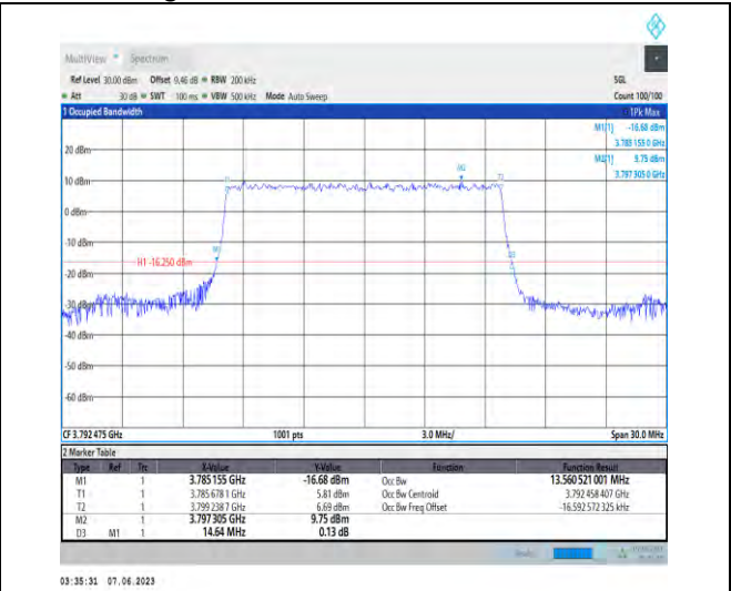
1-N78-3700-3800-PC3-30-15-H-9-CP-256QAM-Outer_Full-38@0-Ant1-13.561-14.640-≤15-PASS
