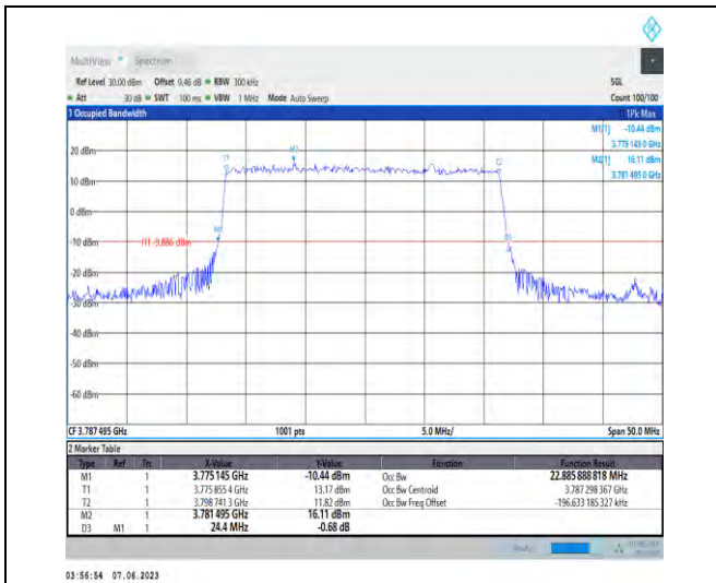
1-N78-3700-3800-PC3-30-25-H-2-DFT-PI2BPSK-Outer_Full-64@0-Ant1-22.886-24.400-≤25-PASS
