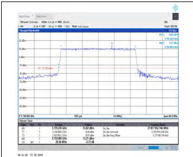
1-N78-3700-3800-PC3-30-30-M-8-CP-64QAM-Outer_Full-78@0-Ant1-27.818-29.580-≤30-PASS
