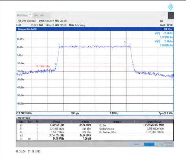
1-N78-3700-3800-PC3-30-15-M-8-CP-64QAM-Outer Full-38@0-Ant1-13.576-14.790-≤15-PASS
