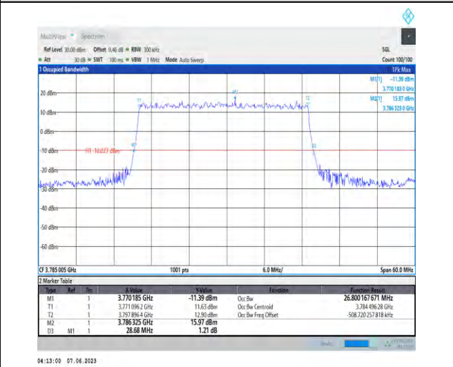
1-N78-3700-3800-PC3-30-30-H-2-DFT-PI2BPSK-Outer_Full-75@0-Ant1-26.8-28.680-≤30-PASS
