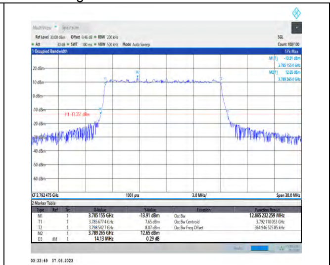
1-N78-3700-3800-PC3-30-15-H-5-DFT-256QAM-Outer_Full-36@0-Ant1-12.865-14.130-≤15-PASS
