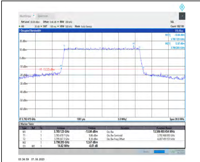
1-N78-3700-3800-PC3-30-15-H-8-CP-64QAM-Outer_Full-38@0-Ant1-13.596-14.820-≤15-PASS
