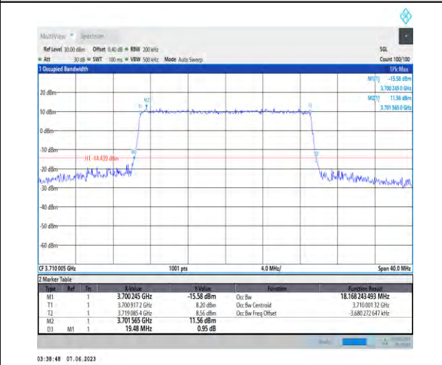
1-N78-3700-3800-PC3-30-20-L-6-CP-QPSK-Outer_Full-51@0-Ant1-18.168-19.480-≤20-PASS
