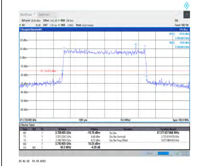
1-N78-3700-3800-PC3-30-50-L-9-CP-256QAM-Outer_Full-133@0-Ant1-47.571-49.3-≤50-PASS
