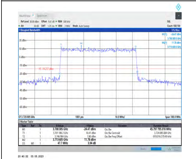
1-N78-3700-3800-PC3-30-50-L-5-DFT-256QAM-Outer_Full-128@0-Ant1-45.798-47.700-≤50-PASS
