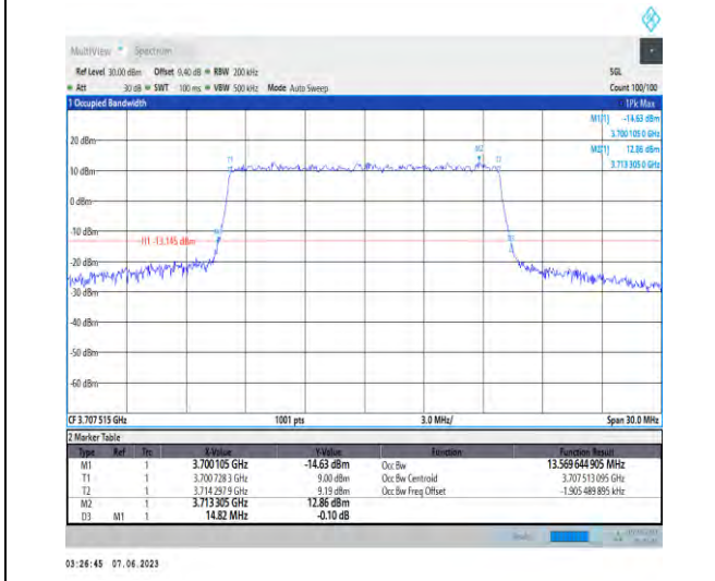
1-N78-3700-3800-PC3-30-15-L-8-CP-64QAM-Outer_Full-38@0-Ant1-13.57-14.820-≤15-PASS
