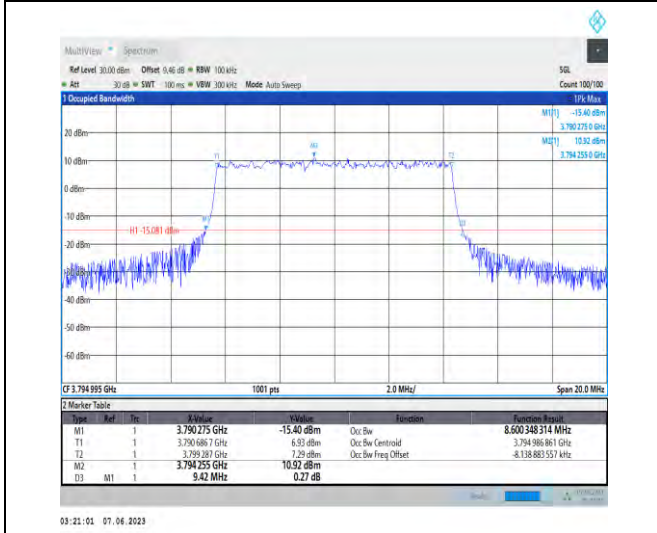
1-N78-3700-3800-PC3-30-10-H-5-DFT-256QAM-Outer_Full-24@0-Ant1-8.6-9.420-≤10-PASS
