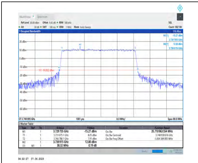
1-N78-3700-3800-PC3-30-40-M-5-DFT-256QAM-Out er_Full-100@0-Ant1-35.711-38.320-≤40-PASS
