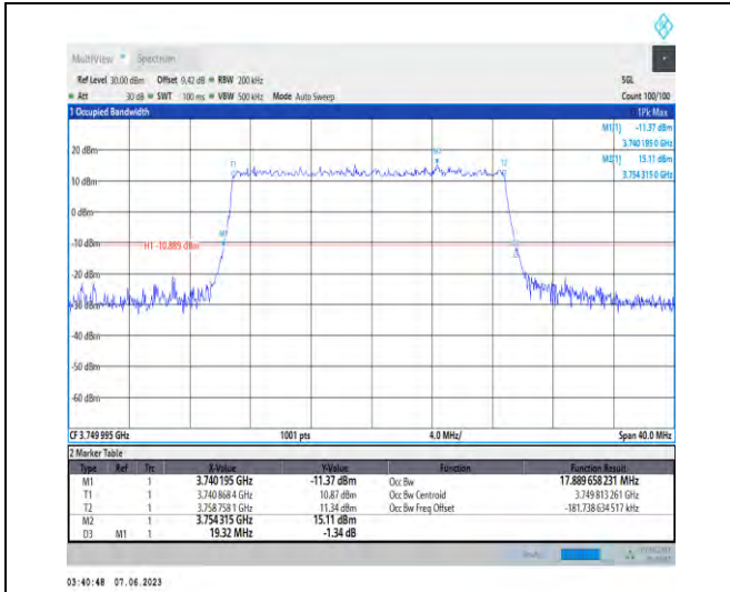
1-N78-3700-3800-PC3-30-20-M-2-DFT-PI2BPSK-Outer_Full-50@0-Ant1-17.89-19.320-≤20-PASS
