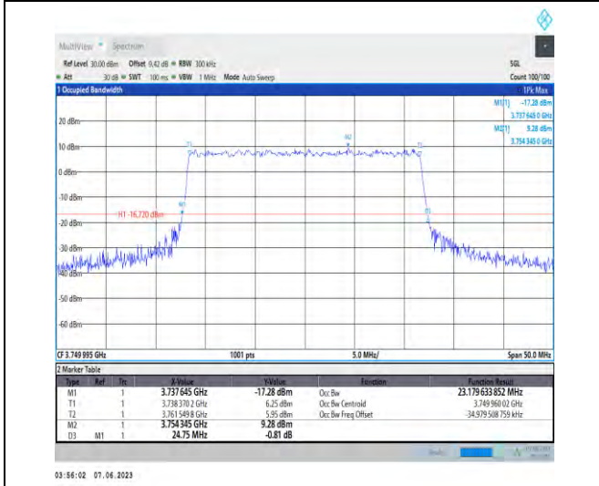
1-N78-3700-3800-PC3-30-25-M-9-CP-256QAM-Outer_Full-65@0-Ant1-23.18-24.750-≤25-PASS
