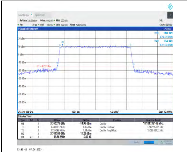
1-N78-3700-3800-PC3-30-20-M-6-CP-QPSK-Outer_Full-51@0-Ant1-18.184-19.560-≤20-PASS
