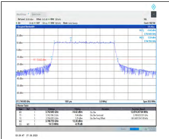
1-N78-3700-3800-PC3-30-15-M-5-DFT-256QAM-Out er_Full-36@0-Ant1-12.874-14.130-≤15-PASS
