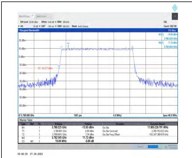
1-N78-3700-3800-PC3-30-20-H-5-DFT-256QAM-Out _Full-50@0-Ant1-17.803-19.040-≤20-PASS
