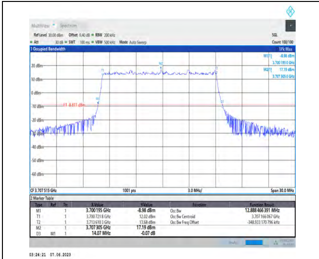
1-N78-3700-3800-PC3-30-15-L-2-DFT-PI2BPSK-Out er_Full-36@0-Ant1-12.888-14.070-≤15-PASS
