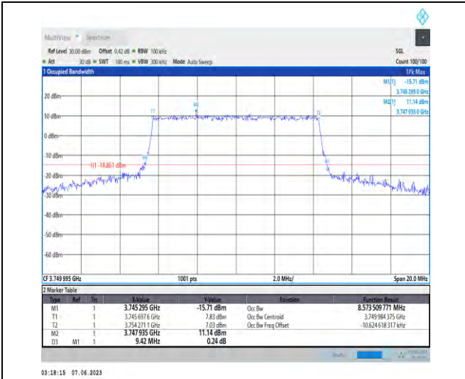
1-N78-3700-3800-PC3-30-10-M-8-CP-64QAM-Outer_Full-24@0-Ant1-8.574-9.420-≤10-PASS
