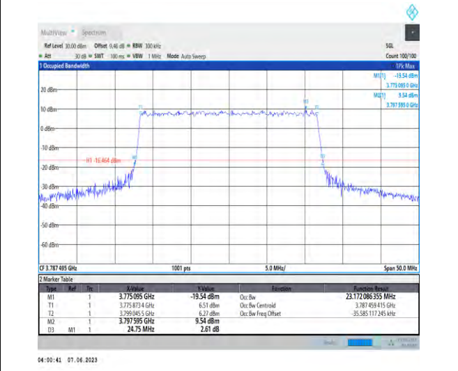
1-N78-3700-3800-PC3-30-25-H-9-CP-256QAM-Outer_Full-65@0-Ant1-23.172-24.750-<=25-PASS
