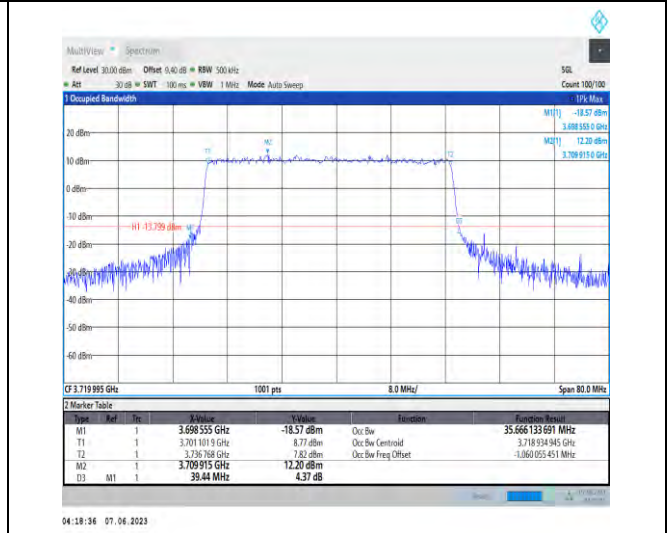
1-N78-3700-3800-PC3-30-40-L-5-DFT-256QAM-Outer_Full-100@0-Ant1-35.666-39.440-≤40-PASS
