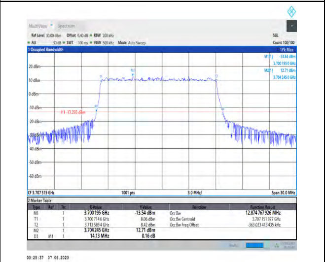
1-N78-3700-3800-PC3-30-15-L-5-DFT-256QAM-Outer_Full-36@0-Ant1-12.875-14.130-≤15-PASS
