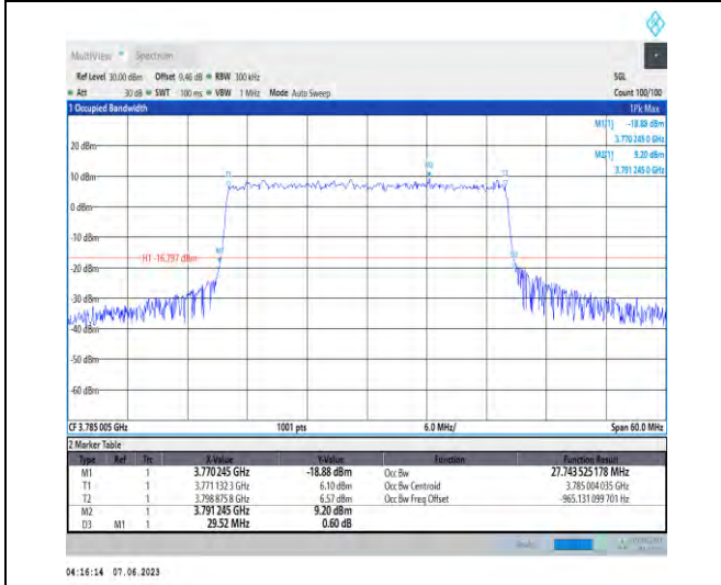
1-N78-3700-3800-PC3-30-30-H-9-CP-256QAM-Outer_Full-78@0-Ant1-27.744-29.520-≤30-PASS
