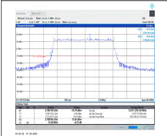
1-N78-3700-3800-PC3-30-15-L-4-DFT-64QAM-Outer_Full-36@0-Ant1-12.911-14.280-≤15-PASS
