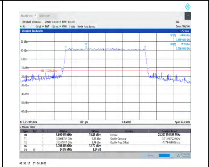
1-N78-3700-3800-PC3-30-25-L-7-CP-16QAM-Outer_Full-65@0-Ant1-23.228-24.950-≤25-PASS
