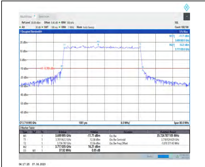
1-N78-3700-3800-PC3-30-40-L-2-DFT-PI2BPSK-Out er_Full-100@0-Ant1-35.725-37.920-≤40-PASS
