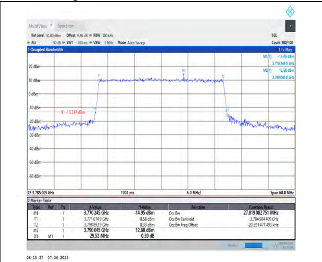
1-N78-3700-3800-PC3-30-30-H-8-CP-64QAM-Outer_Full-78@0-Ant1-27.819-29.520-≤30-PASS
