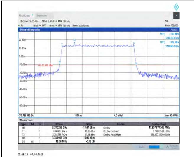
1-N78-3700-3800-PC3-30-20-H-1-DFT-QPSK-Outer_Full-50@0-Ant1-17.858-19.080-≤20-PASS
