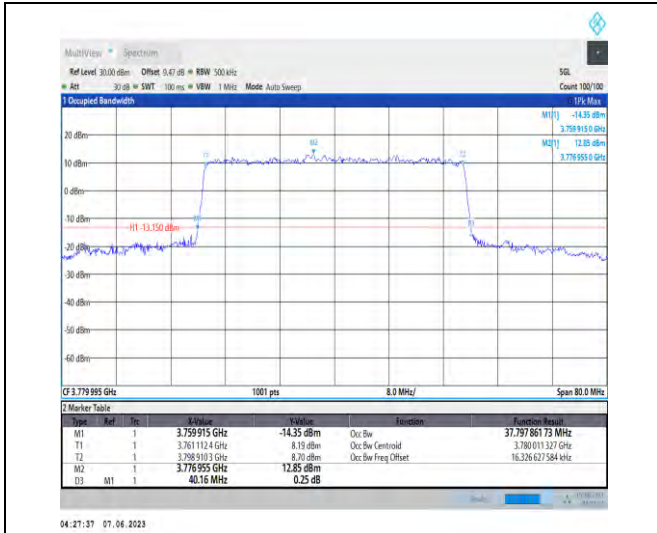
1-N78-3700-3800-PC3-30-40-H-8-CP-64QAM-Outer_Full-106@0-Ant1-37.798-40.160-≤40-PASS
