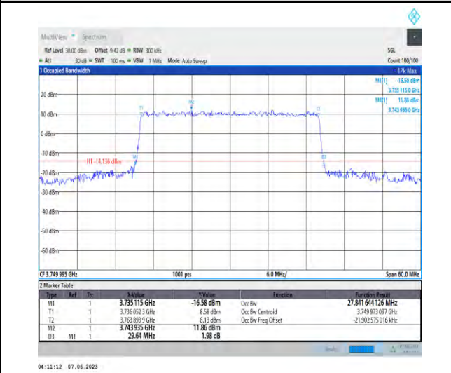
1-N78-3700-3800-PC3-30-30-M-7-CP-16QAM-Outer_Full-78@0-Ant1-27.842-29.640-≤30-PASS
