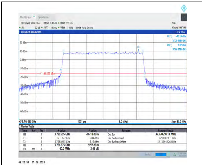
1-N78-3700-3800-PC3-30-40-M-9-CP-256QAM-Out er_Full-106@0-Ant1-37.77-40.000-≤40-PASS
