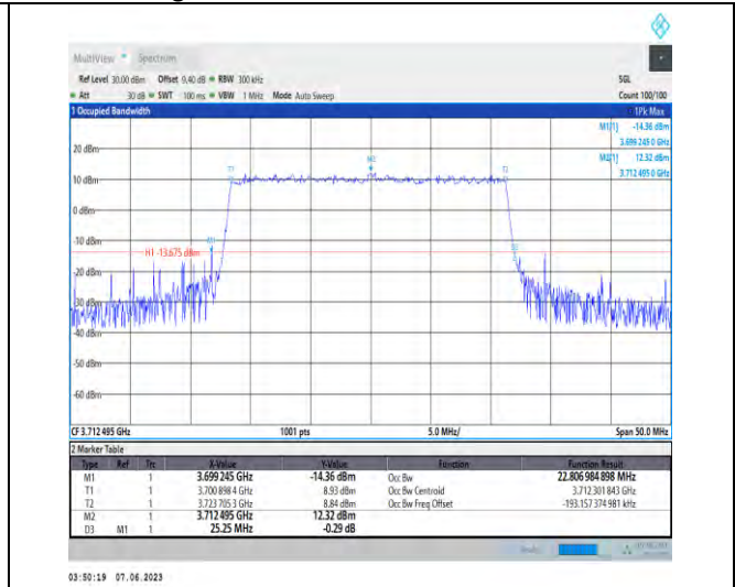
1-N78-3700-3800-PC3-30-25-L-5-DFT-256QAM-Outer_Full-64@0-Ant1-22.807-25.250-≤25-PASS
