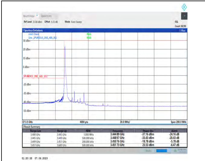
1-N78-3450-3550-PC3-30-25-L-1-DFT-PI2BPSK-Edge_1RB_Left-1@0-Ant1-1--PASS-see graph
