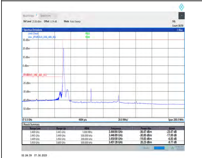
1-N78-3450-3550-PC3-30-70-L-4-CP-QPSK-Edge_1RB_Left-1@0-Ant1-1--PASS-see graph
