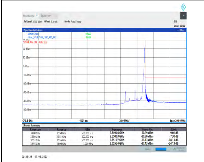
1-N78-3450-3550-PC3-30-25-H-5-CP-QPSK-Edge_1RB_Right-1@64-Ant1-1--PASS-see graph
