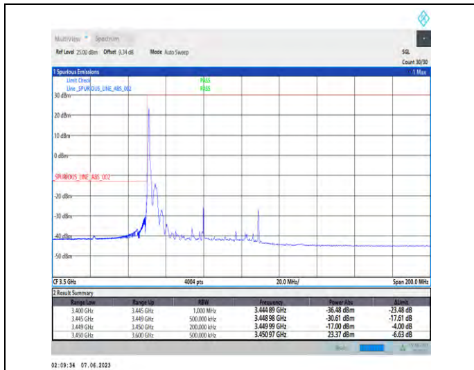
1-N78-3450-3550-PC3-30-60-L-1-DFT-PI2BPSK-Edge_1RB_Left-1@0-Ant1-1--PASS-see graph
