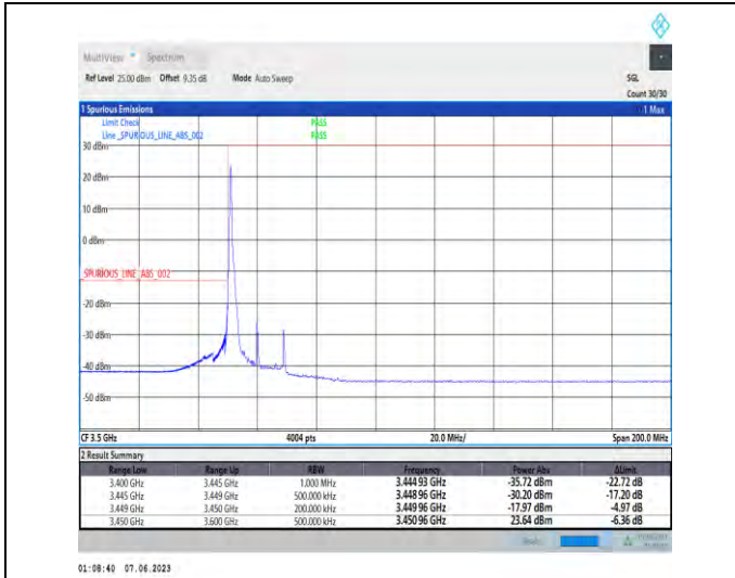
1-N78-3450-3550-PC3-30-20-L-1-DFT-PI2BPSK-Edge_1RB_Left-1@0-Ant1-1--PASS-see graph
