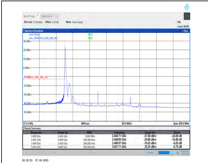
1-N78-3450-3550-PC3-30-80-L-1-DFT-PI2BPSK-Edge_1RB_Left-1@0-Ant1-1--PASS-see graph
