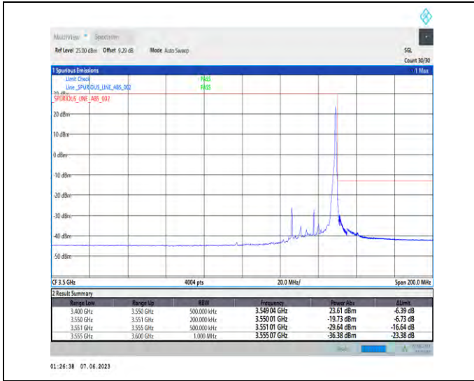
1-N78-3450-3550-PC3-30-25-H-2-DFT-PI2BPSK-Edge_1RB_Right-1@64-Ant1-1--PASS-see graph
