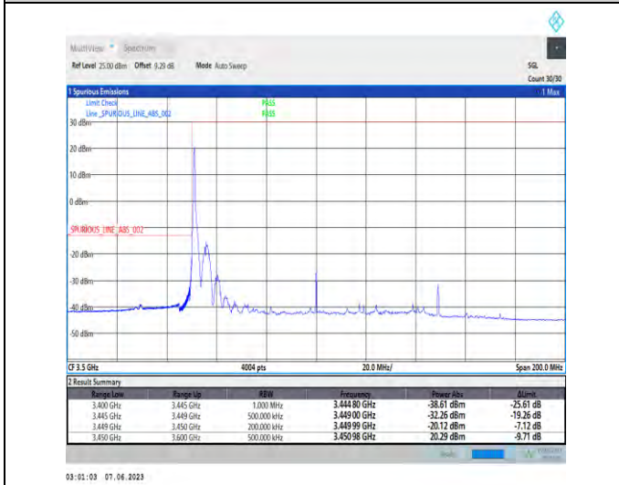
1-N78-3450-3550-PC3-30-100-L-4-CP-QPSK-Edge_1RB_Left-1@0-Ant1-1--PASS-see graph
