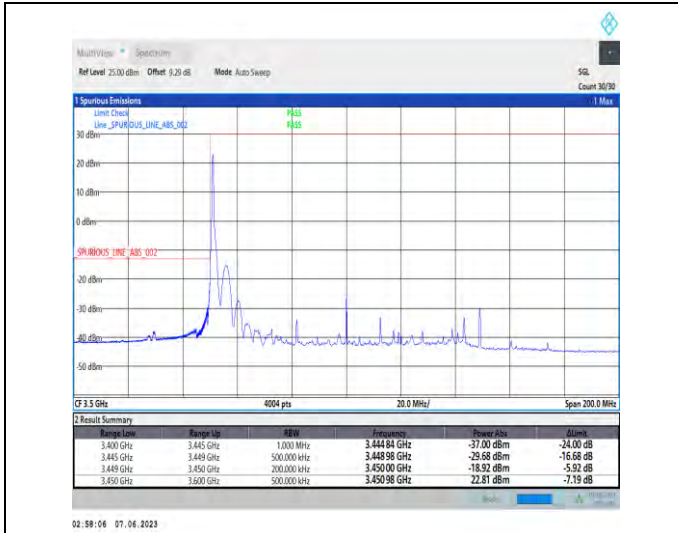
1-N78-3450-3550-PC3-30-100-L-1-DFT-PI2BPSK-Edge_e_1RB_Left-1@0-Ant1-1--PASS-see graph
