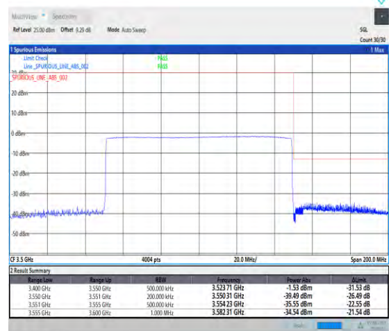
1-N78-3450-3550-PC3-30-100-H-6-CP-QPSK-Outer_Full-273@0-Ant1-1--PASS-see graph
