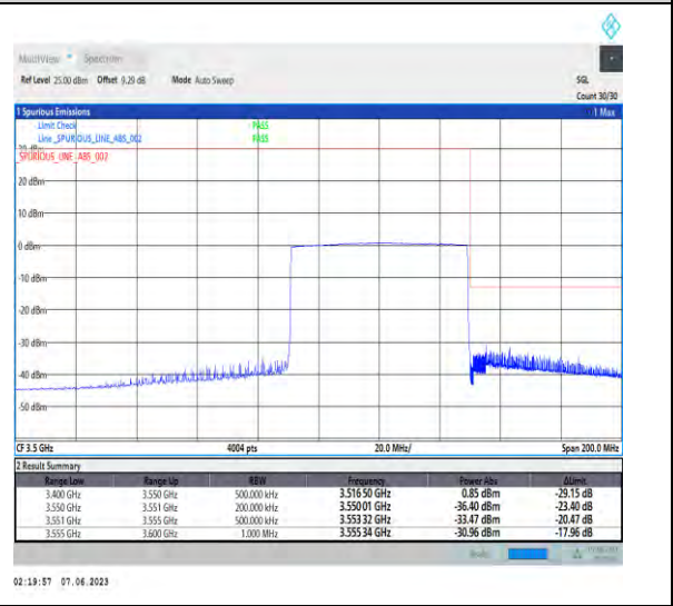
1-N78-3450-3550-PC3-30-60-H-6-CP-QPSK-Outer_Full-162@0-Ant1-1--PASS-see graph
