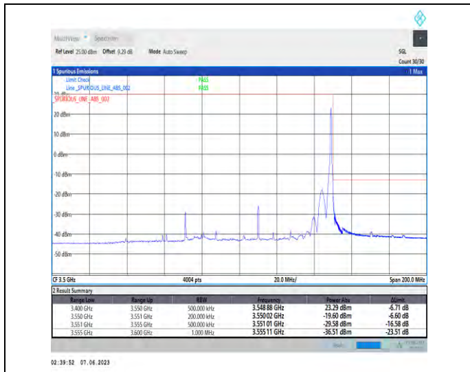
1-N78-3450-3550-PC3-30-80-H-2-DFT-PI2BPSK-Edge_1RB_Right-1@216-Ant1-1--PASS-see graph
