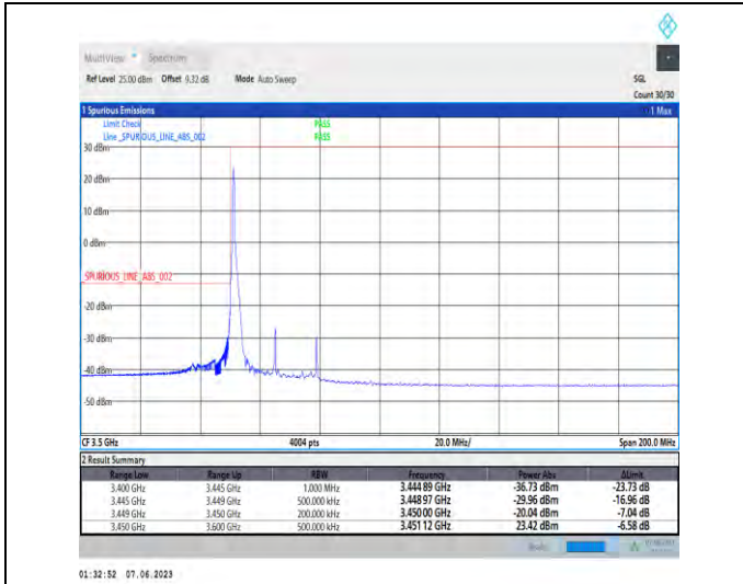
1-N78-3450-3550-PC3-30-30-L-1-DFT-PI2BPSK-Edge_1RB_Left-1@0-Ant1-1--PASS-see graph
