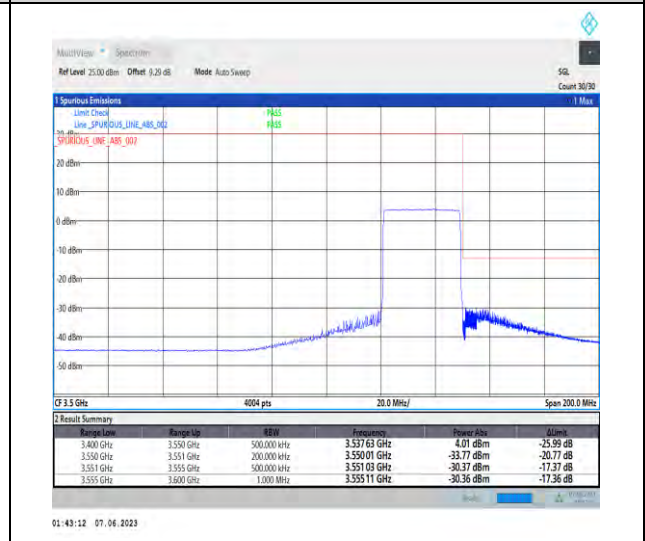
1-N78-3450-3550-PC3-30-30-H-6-CP-QPSK-Outer_Full-78@0-Ant1-1--PASS-see graph
