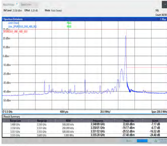
1-N78-3450-3550-PC3-30-100-H-2-DFT-PI2BPSK-Edge_1RB_Right-1@272-Ant1-1--PASS-see graph
