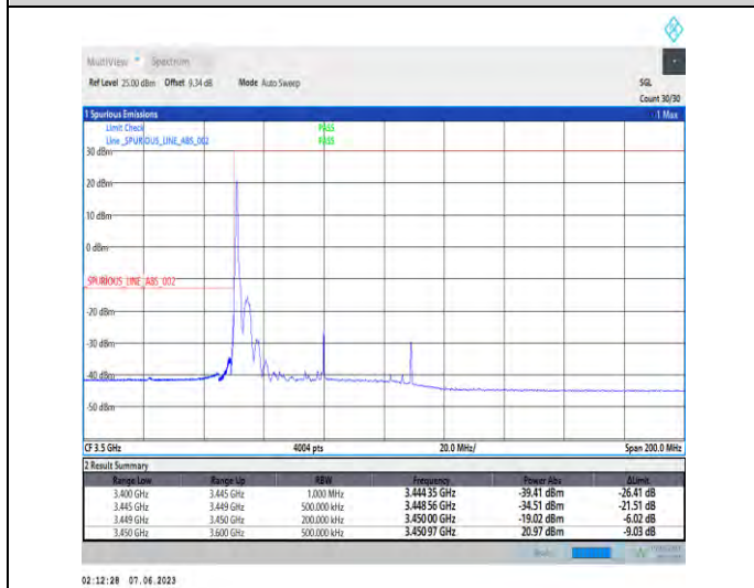
1-N78-3450-3550-PC3-30-60-L-4-CP-QPSK-Edge_1RB_Left-1@0-Ant1-1--PASS-see graph
