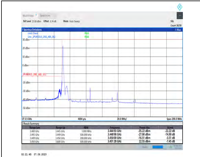
1-N78-3450-3550-PC3-30-70-L-1-DFT-PI2BPSK-Edge_1RB_Left-1@0-Ant1-1--PASS-see graph
