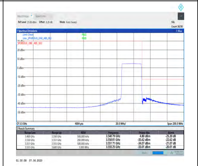
1-N78-3450-3550-PC3-30-25-H-6-CP-QPSK-Outer_Full-65@0-Ant1-1--PASS-see graph
