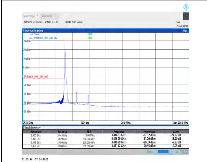
1-N78-3450-3550-PC3-30-30-L-4-CP-QPSK-Edge_1RB_Left-1@0-Ant1-1--PASS-see graph
