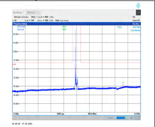
1-N78-3450-3550-PC3-30-100-M-1-N/A-DFT-PI2BPS K-Inner_1RB_Left-1@1-1000-6000-Ant1-5321.50--39 .27--13-PASS
