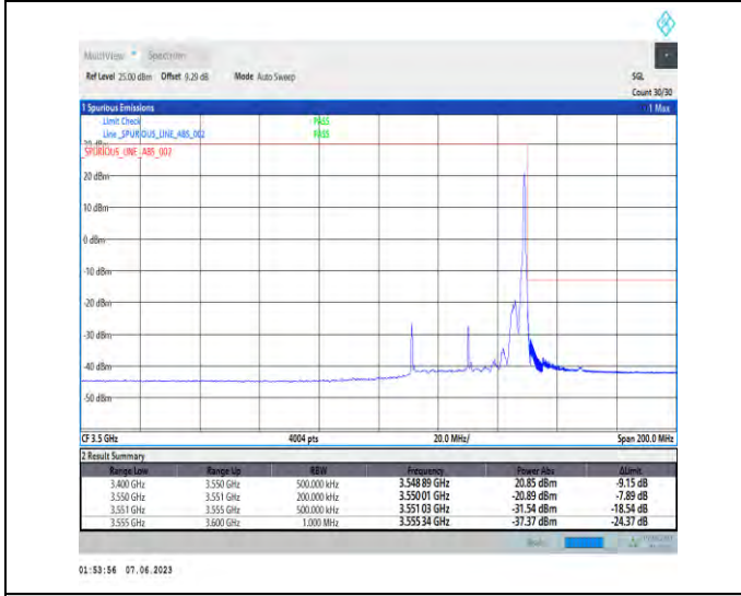
1-N78-3450-3550-PC3-30-40-H-5-CP-QPSK-Edge_1RB_Right-1@105-Ant1-1--PASS-see graph
