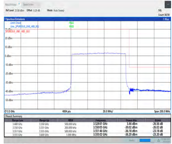
1-N78-3450-3550-PC3-30-70-H-3-DFT-PI2BPSK-Outer_Full-180@0-Ant1-1--PASS-see graph
