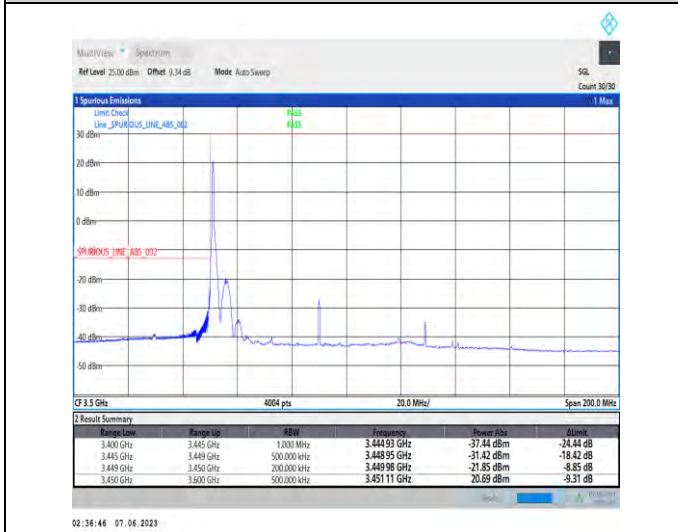
1-N78-3450-3550-PC3-30-80-L-4-CP-QPSK-Edge_1RB_Left-1@0-Ant1-1--PASS-see graph
