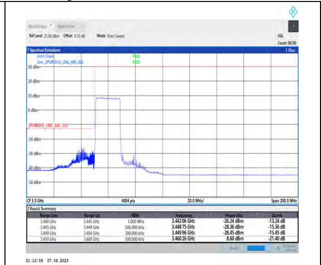
1-N78-3450-3550-PC3-30-20-L-3-DFT-PI2BPSK-Outer_Full-50@0-Ant1-1--PASS-see graph
