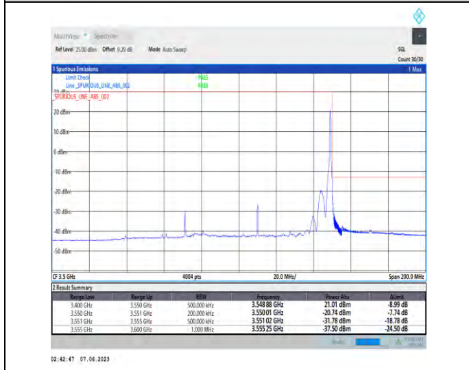
1-N78-3450-3550-PC3-30-80-H-5-CP-QPSK-Edge_1RB_Right-1@216-Ant1-1--PASS-see graph
