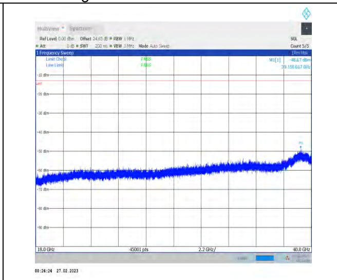
1-N78-3450-3550-PC3-30-100-L-1-N/A-DFT-PI2BPS K-Inner_1RB_Left-1@1-18000-40000-Ant1-18000.00 --61.91--13-PASS
