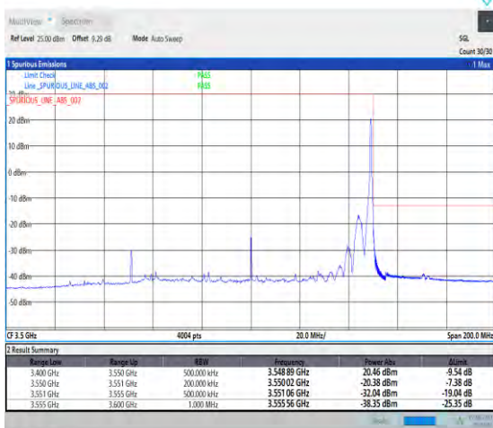
1-N78-3450-3550-PC3-30-100-H-5-CP-QPSK-Edge_1RB_Right-1@272-Ant1-1--PASS-see graph
