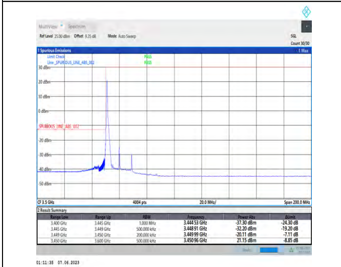
1-N78-3450-3550-PC3-30-20-L-4-CP-QPSK-Edge_1RB_Left-1@0-Ant1-1--PASS-see graph
