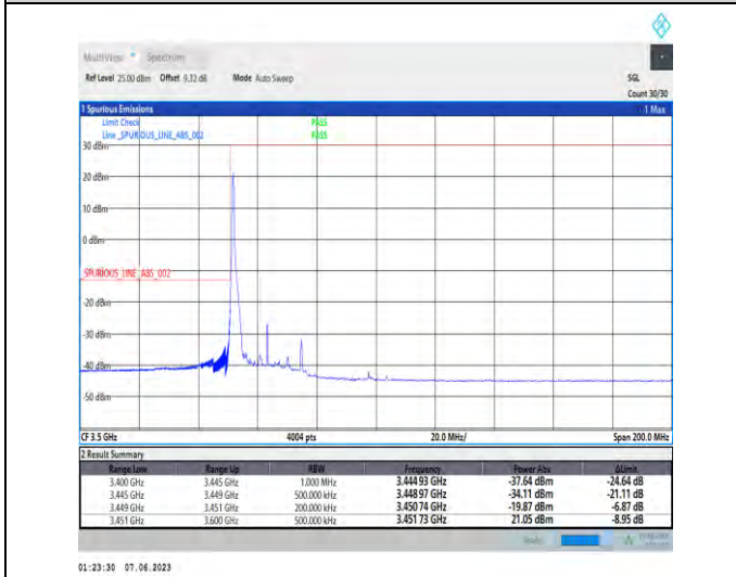
1-N78-3450-3550-PC3-30-25-L-4-CP-QPSK-Edge_1RB_Left-1@0-Ant1-1--PASS-see graph
