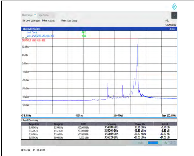
1-N78-3450-3550-PC3-30-40-H-2-DFT-PI2BPSK-Edge_1RB_Right-1@105-Ant1-1--PASS-see graph
