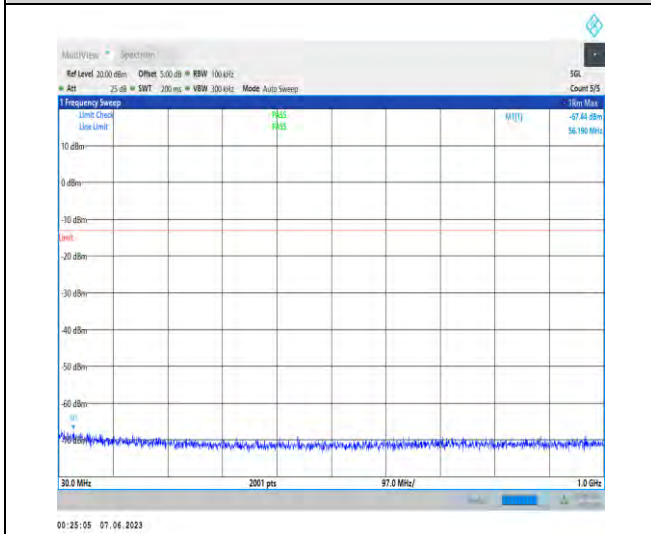
1-N78-3450-3550-PC3-30-100-H-1-N/A-DFT-PI2BP SK-Inner_1RB_Left-1@1-30-1000-Ant1-56.19--67.4 4--13-PASS
