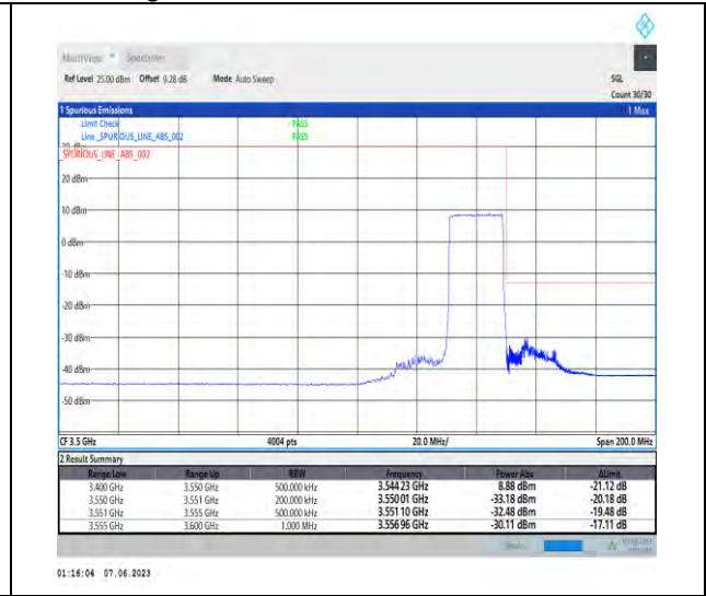
1-N78-3450-3550-PC3-30-20-H-3-DFT-PI2BPSK-Outer_Full-50@0-Ant1-1--PASS-see graph
