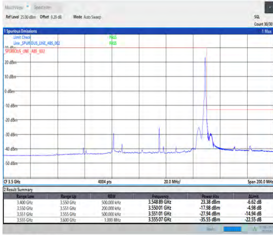
1-N78-3450-3550-PC3-30-70-H-2-DFT-PI2BPSK-Edge_1RB_Right-1@188-Ant1-1--PASS-see graph
