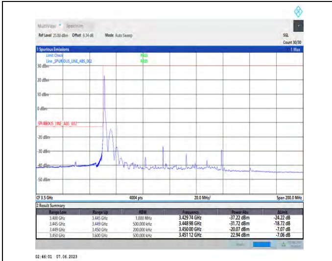
1-N78-3450-3550-PC3-30-90-L-1-DFT-PI2BPSK-Edge_1RB_Left-1@0-Ant1-1--PASS-see graph
