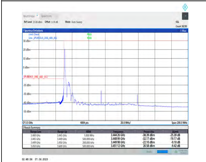
1-N78-3450-3550-PC3-30-90-L-4-CP-QPSK-Edge_1RB_Left-1@0-Ant1-1--PASS-see graph
