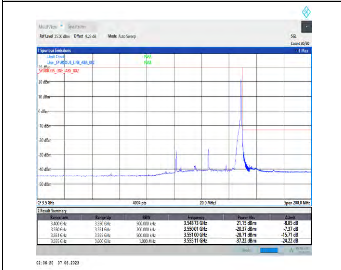
1-N78-3450-3550-PC3-30-50-H-5-CP-QPSK-Edge_1RB_Right-1@132-Ant1-1--PASS-see graph
