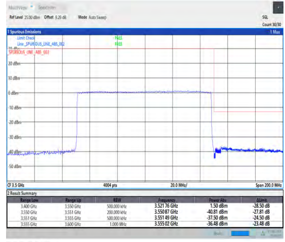
1-N78-3450-3550-PC3-30-100-H-3-DFT-PI2BPSK-Outer_Full-270@0-Ant1-1--PASS-see graph
