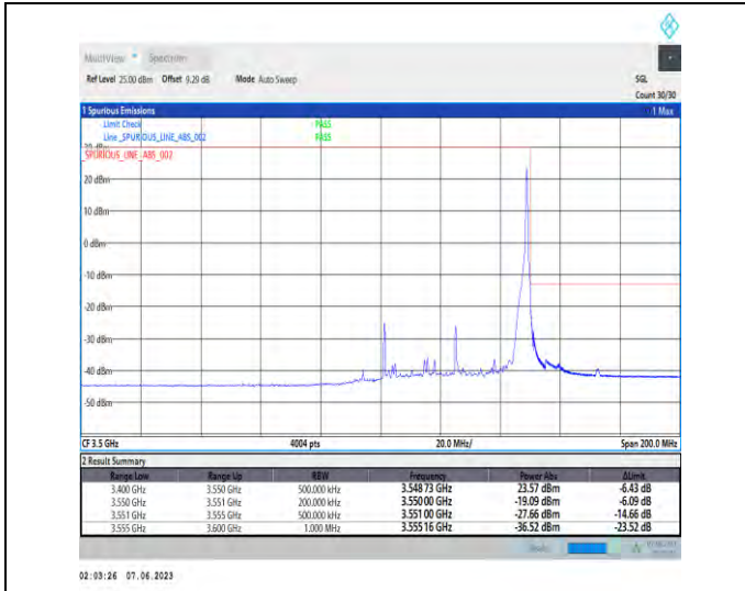
1-N78-3450-3550-PC3-30-50-H-2-DFT-PI2BPSK-Edge_1RB_Right-1@132-Ant1-1--PASS-see graph
