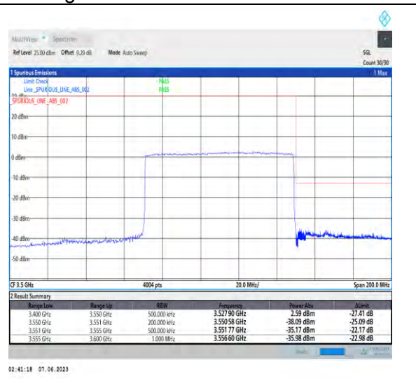
1-N78-3450-3550-PC3-30-80-H-3-DFT-PI2BPSK-Outer_Full-216@0-Ant1-1--PASS-see graph
