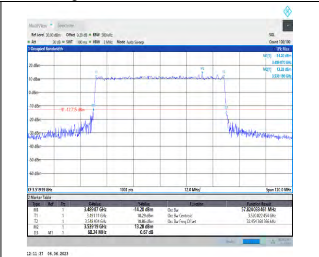
1-N78-3450-3550-PC3-30-60-H-3-DFT-16QAM-Outer_Full-162@0-Ant1-57.824-60.240-≤60-PASS
