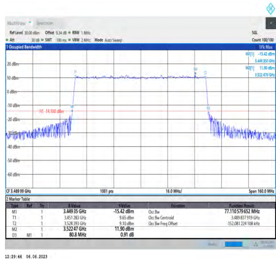
1-N78-3450-3550-PC3-30-80-L-5-DFT-256QAM-Out er_Full-216@0-Ant1-77.111-80.800-≤80-PASS
