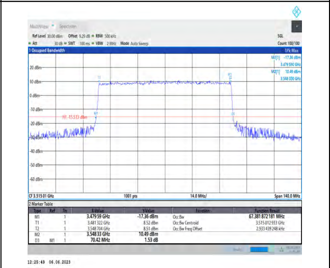
1-N78-3450-3550-PC3-30-70-H-6-CP-QPSK-Outer_Full-189@0-Ant1-67.382-70.420-≤70-PASS
