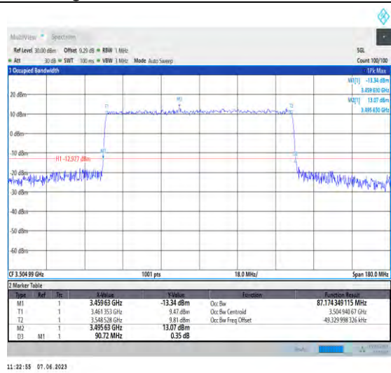
1-N78-3450-3550-PC3-30-90-H-6-CP-QPSK-Outer_ Full-245@0-Ant1-87.174-90.720-≤90-PASS
