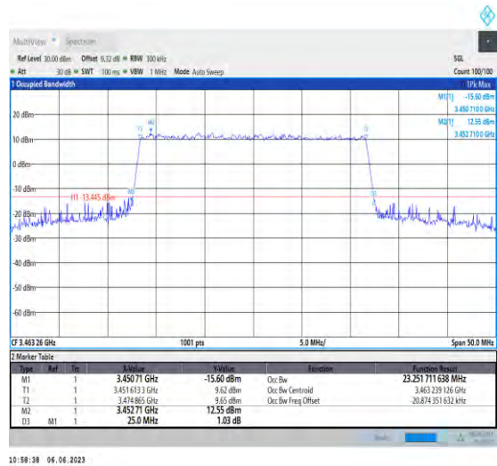
1-N78-3450-3550-PC3-30-25-L-7-CP-16QAM-Outer_Full-65@0-Ant1-23.252-25.000-≤25-PASS
