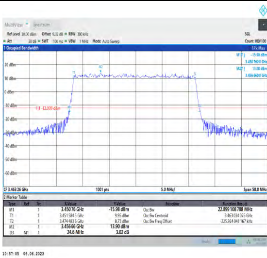
1-N78-3450-3550-PC3-30-25-L-4-DFT-64QAM-Outer_Full-64@0-Ant1-22.899-24.600-≤25-PASS
