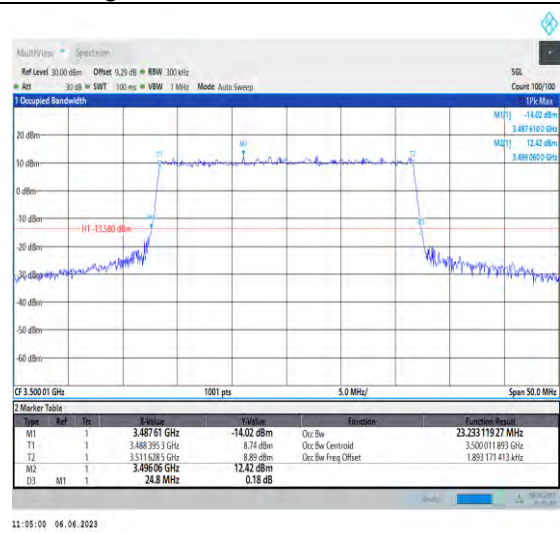
1-N78-3450-3550-PC3-30-25-M-8-CP-64QAM-Outer _Full-65@0-Ant1-23.233-24.800-≤25-PASS
