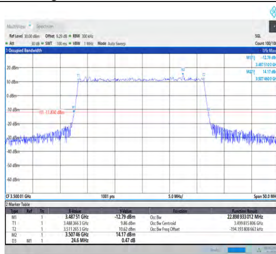
1-N78-3450-3550-PC3-30-25-M-4-DFT-64QAM-Outer_Full-64@0-Ant1-22.899-24.600-≤25-PASS
