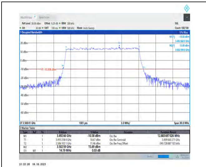
1-N78-3450-3550-PC3-30-15-M-1-DFT-QPSK-Outer_Full-36@0-Ant1-12.884-14.190-≤15-PASS
