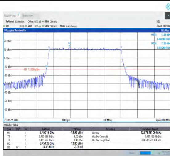
1-N78-3450-3550-PC3-30-15-L-3-DFT-16QAM-Out er_Full-36@0-Ant1-12.849-14.160-≤15-PASS
