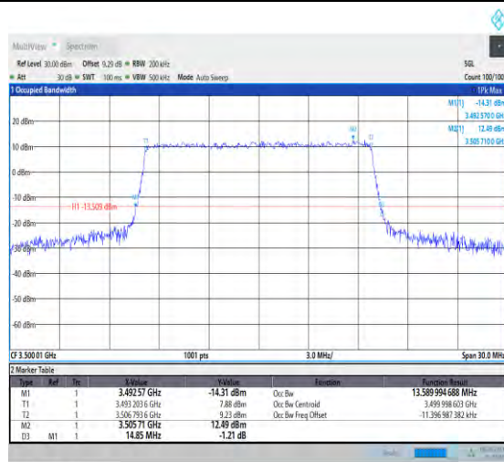
1-N78-3450-3550-PC3-30-15-M-6-CP-QPSK-Outer Full-38@0-Ant1-13.574-14.760-≤15-PASS
