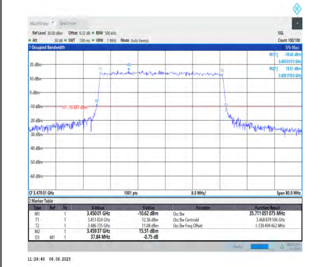
1-N78-3450-3550-PC3-30-40-L-1-DFT-QPSK-Outer_Full-100@0-Ant1-35.711-37.840-≤40-PASS
