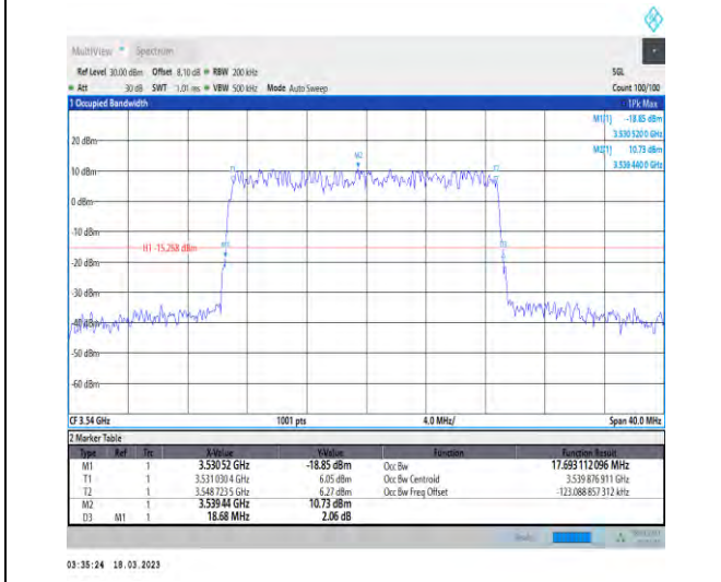
1-N78-3450-3550-30-20-H-3-DFT-16QAM-Outer_Full-50@0-Ant1-17.693-18.680-≤20-PASS
