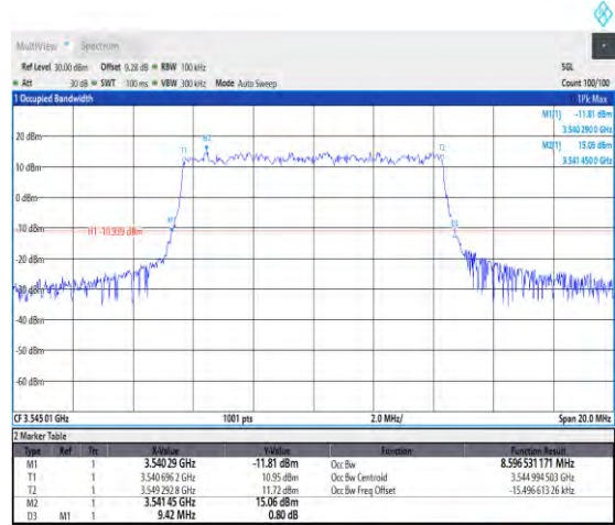
1-N78-3450-3550-PC3-30-10-M-9-CP-256QAM-Outer_Full-24@0-Ant1-8.565-9.460-≤10-PASS
