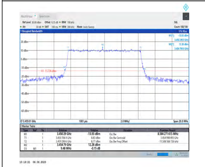
1-N78-3450-3550-PC3-30-10-L-7-CP-16QAM-Outer Full-24@0-Ant1-8.584-9.480-≤10-PASS
