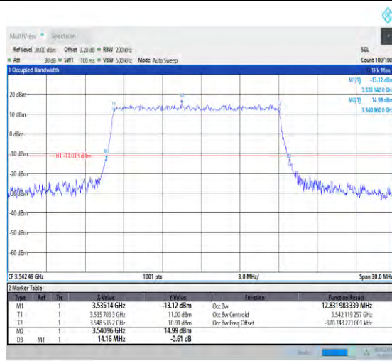
1-N78-3450-3550-PC3-30-15-H-1-DFT-QPSK-Outer_Full-36@0-Ant1-12.869-14.130-≤15-PASS
