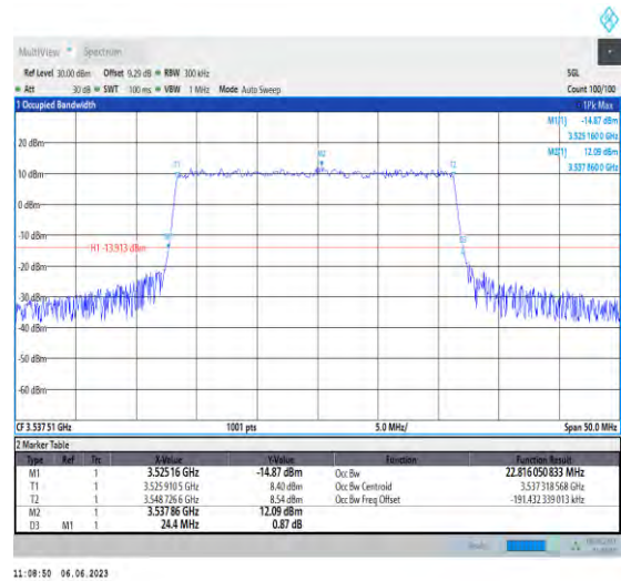
1-N78-3450-3550-PC3-30-25-H-5-DFT-256QAM-Outer_Full-64@0-Ant1-22.816-24.400-≤25-PASS
