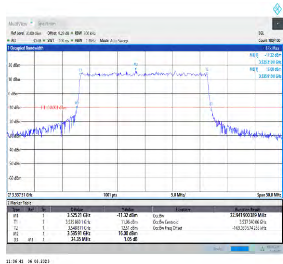
1-N78-3450-3550-PC3-30-25-H-1-DFT-QPSK-Outer _Full-64@0-Ant1-22.942-24.350-≤25-PASS
