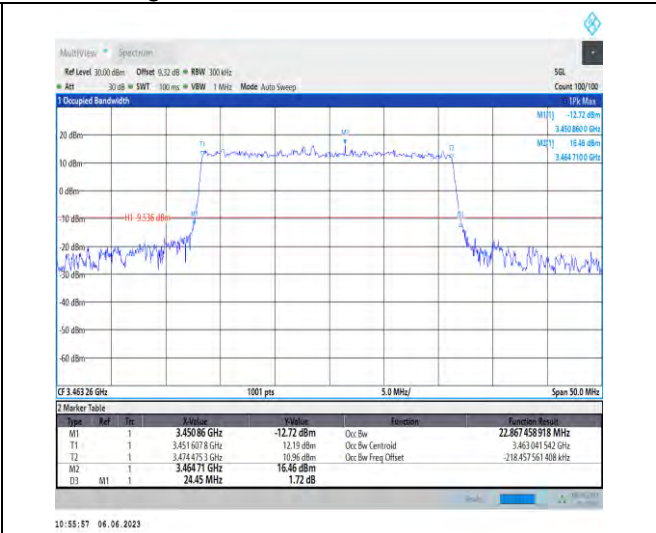
1-N78-3450-3550-PC3-30-25-L-1-DFT-QPSK-Outer_Full-64@0-Ant1-22.867-24.450-≤25-PASS
