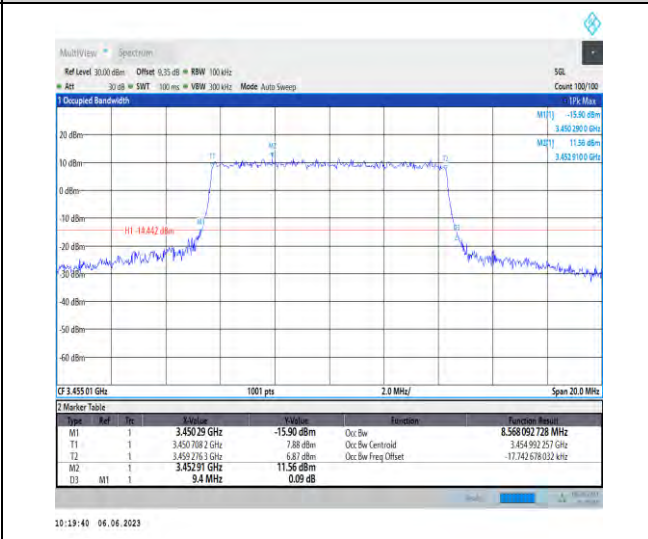
1-N78-3450-3550-PC3-30-10-L-8-CP-64QAM-Outer Full-24@0-Ant1-8.568-9.400-≤10-PASS
