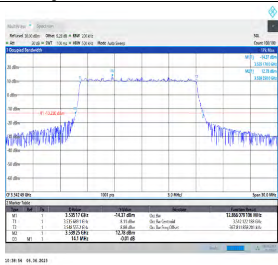
1-N78-3450-3550-PC3-30-15-H-5-DFT-256QAM-Outer_Full-36@0-Ant1-12.866-14.100-≤15-PASS
