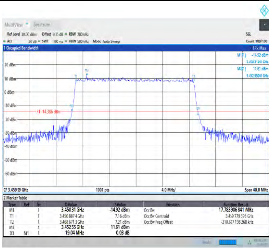
1-N78-3450-3550-PC3-30-20-L-3-DFT-16QAM-Outer_Full-50@0-Ant1-17.848-19.200-≤20-PASS
