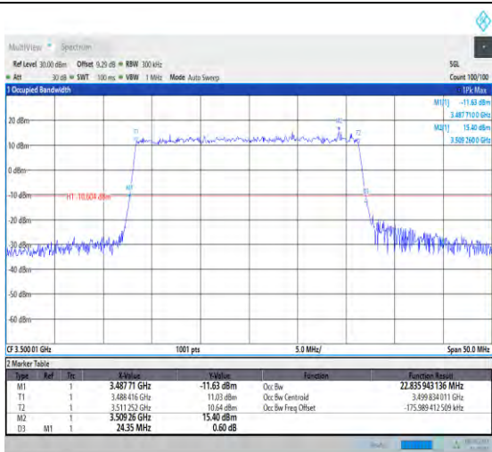
1-N78-3450-3550-PC3-30-25-M-3-DFT-16QAM-Outer_Full-64@0-Ant1-22.836-24.350-≤25-PASS
