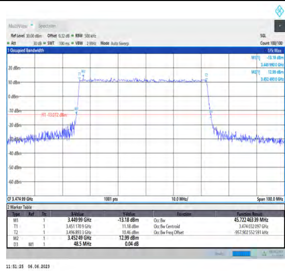
1-N78-3450-3550-PC3-30-50-L-4-DFT-64QAM-Outer_Full-128@0-Ant1-45.722-48.500-≤50-PASS
