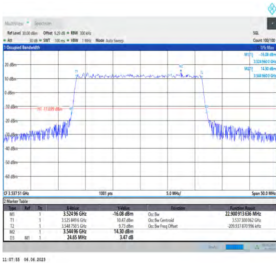
1-N78-3450-3550-PC3-30-25-H-4-DFT-64QAM-Outer_Full-64@0-Ant1-22.901-24.650-≤25-PASS
