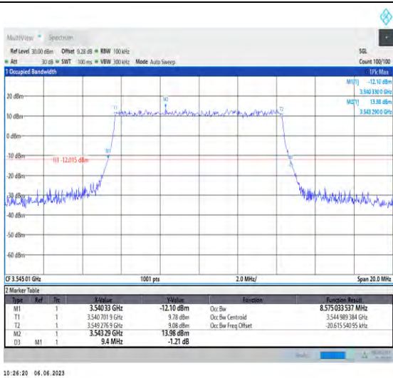
1-N78-3450-3550-PC3-30-10-H-3-DFT-16QAM-Outer_Full-24@0-Ant1-8.575-9.400-≤10-PASS
