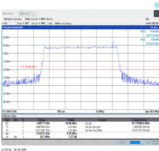
1-N78-3450-3550-PC3-30-25-M-9-CP-256QAM-Outer _Full-65@0-Ant1-23.18-24.700-≤25-PASS
