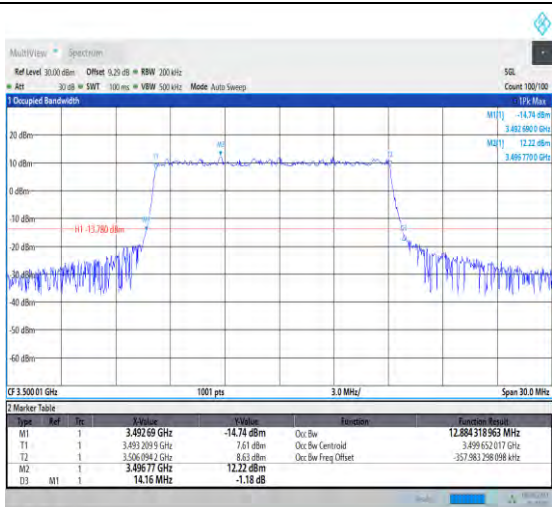
1-N78-3450-3550-PC3-30-15-M-5-DFT-256QAM-Out er_Full-36@0-Ant1-12.884-14.160-≤15-PASS
