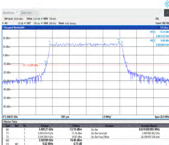
1-N78-3450-3550-PC3-30-10-L-9-CP-256QAM-Outer_Full-24@0-Ant1-8.566-9.300-≤10-PASS
