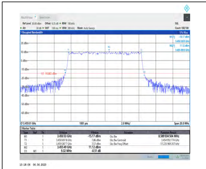
1-N78-3450-3550-PC3-30-10-L-5-DFT-256QAM-Out er_Full-24@0-Ant1-8.59-9.320-≤10-PASS
