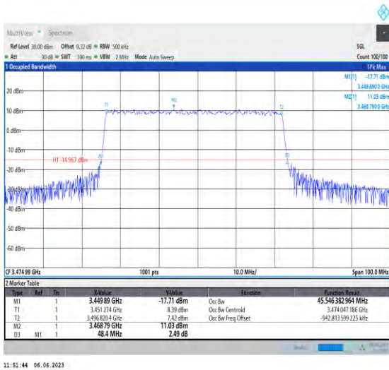
1-N78-3450-3550-PC3-30-50-L-5-DFT-256QAM-Outer_Full-128@0-Ant1-45.546-48.400-≤50-PASS
