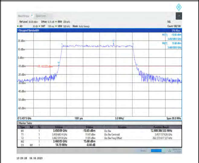
1-N78-3450-3550-PC3-30-15-L-1-DFT-QPSK-Outer_Full-36@0-Ant1-12.908-14.190-≤15-PASS
