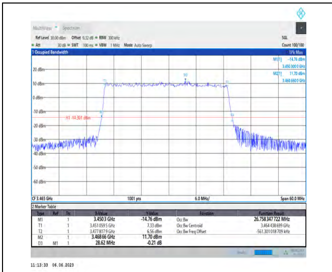
1-N78-3450-3550-PC3-30-30-L-5-DFT-256QAM-Out_er_Full-75@0-Ant1-26.758-28.620-≤30-PASS
