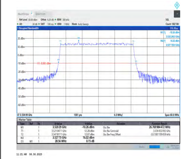
1-N78-3450-3550-PC3-30-30-H-2-DFT-PI2BPSK-Outer_Full-75@0-Ant1-26.77-28.560-≤30-PASS
