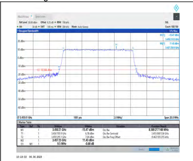
1-N78-3450-3550-PC3-30-10-L-6-CP-QPSK-Outer Full-24@0-Ant1-8.589-9.500-≤10-PASS
