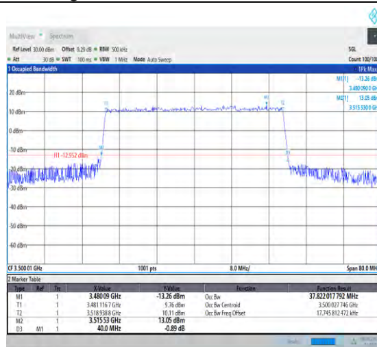
1-N78-3450-3550-PC3-30-40-M-6-CP-QPSK-Outer_Full-106@0-Ant1-37.822-40.000-<40-PASS
