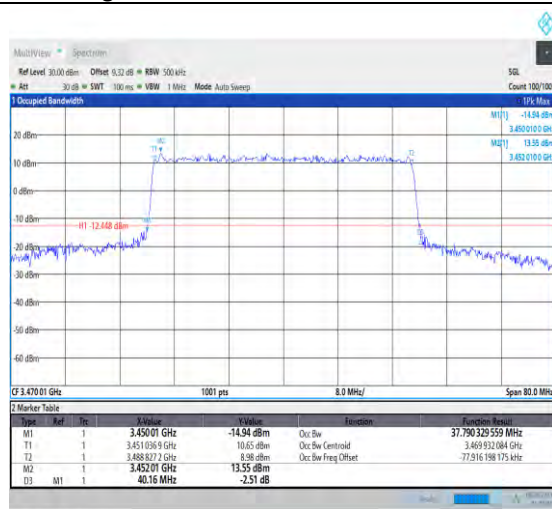
1-N78-3450-3550-PC3-30-40-L-7-CP-16QAM-Outer_Full-106@0-Ant1-37.79-40.160-≤40-PASS
