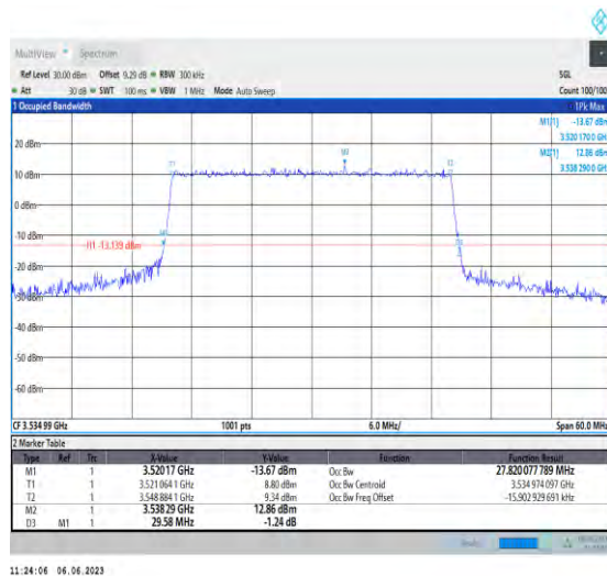
1-N78-3450-3550-PC3-30-30-H-6-CP-QPSK-Outer_Full-78@0-Ant1-27.82-29.580-≤30-PASS
