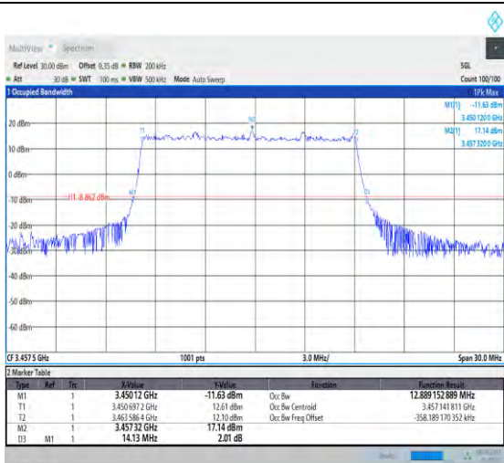
1-N78-3450-3550-PC3-30-15-L-2-DFT-PI2BPSK-Out er_Full-36@0-Ant1-12.889-14.130-≤15-PASS
