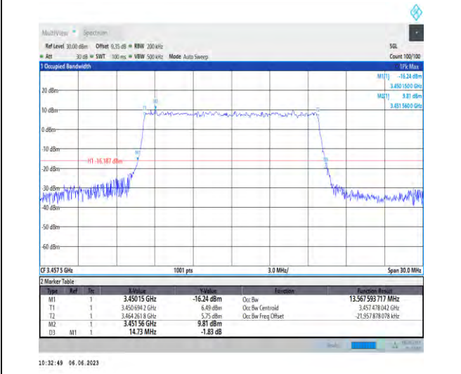
1-N78-3450-3550-PC3-30-15-L-9-CP-256QAM-Outer_Full-38@0-Ant1-13.568-14.730-≤15-PASS
