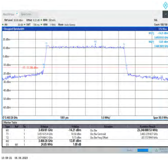
1-N78-3450-3550-PC3-30-25-L-6-CP-QPSK-Outer_Full-65@0-Ant1-23.249-24.850-≤25-PASS
