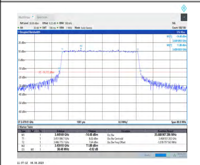
1-N78-3450-3550-PC3-30-40-L-5-DFT-256QAM-Outer_Full-100@0-Ant1-35.689-38.480-≤40-PASS
