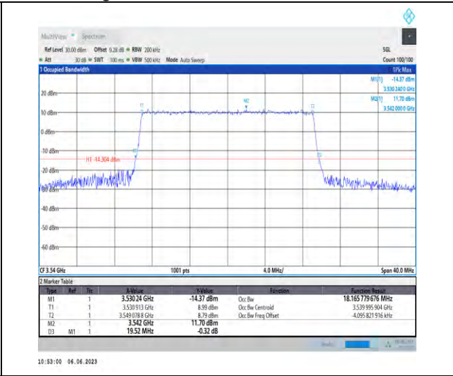
1-N78-3450-3550-PC3-30-20-H-6-CP-QPSK-Outer _Full-51@0-Ant1-18.166-19.520-≤20-PASS
