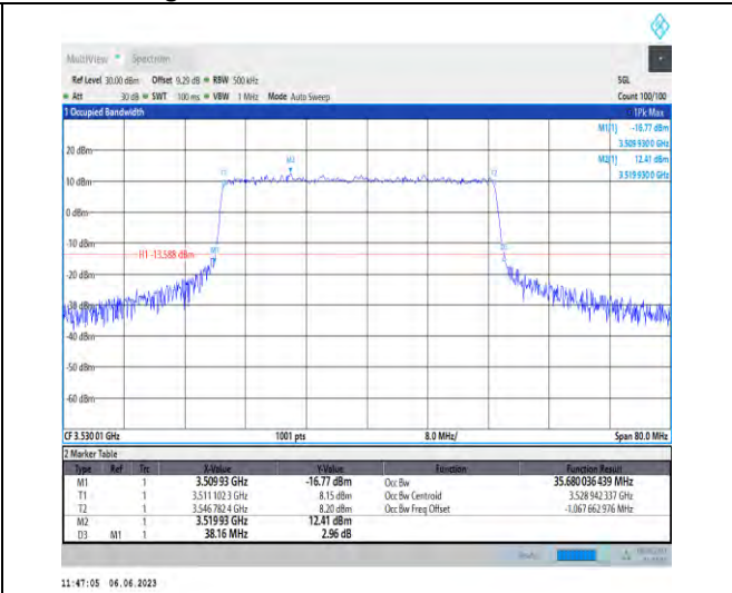
1-N78-3450-3550-PC3-30-40-H-5-DFT-256QAM-Outer_Full-100@0-Ant1-35.68-38.160-≤40-PASS
