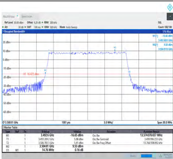
1-N78-3450-3550-PC3-30-15-M-9-CP-256QAM-Outer_Full-38@0-Ant1-13.574-14.760-≤15-PASS
