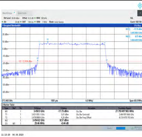
1-N78-3450-3550-PC3-30-30-L-9-CP-256QAM-Outer_Full-78@0-Ant1-27.793-29.460-≤30-PASS
