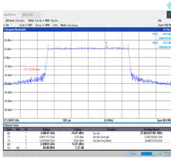
1-N78-3450-3550-PC3-30-40-M-8-CP-64QAM-Outer_Full-106@0-Ant1-37.843-40.080-<40-PASS
