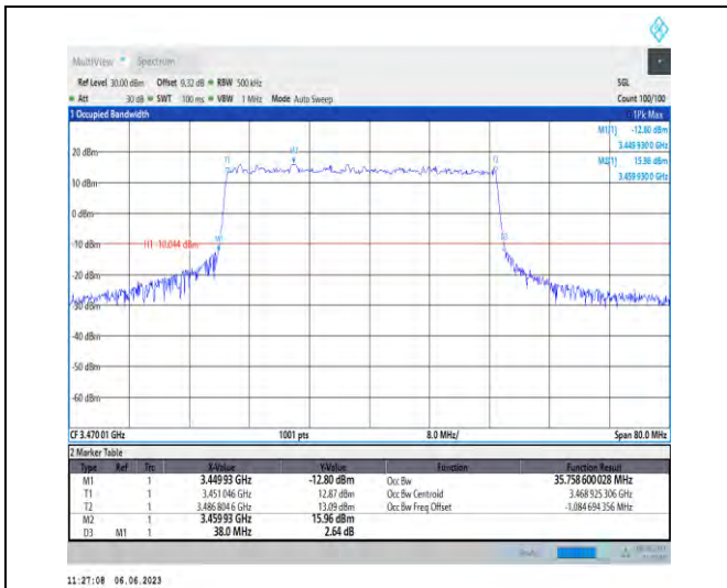
1-N78-3450-3550-PC3-30-40-L-2-DFT-PI2BPSK-Out_er_Full-100@0-Ant1-35.759-38.000-≤40-PASS
