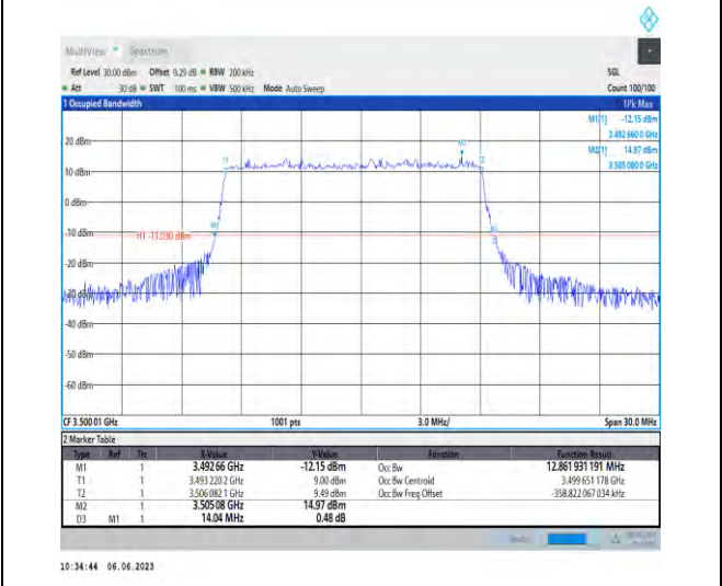
1-N78-3450-3550-PC3-30-15-M-4-DFT-64QAM-Outer_Full-36@0-Ant1-12.862-14.040-≤15-PASS
