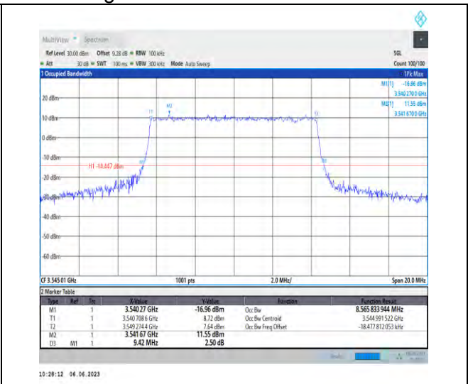
1-N78-3450-3550-PC3-30-10-H-8-CP-64QAM-Outer_Full-24@0-Ant1-8.566-9.420-≤10-PASS
