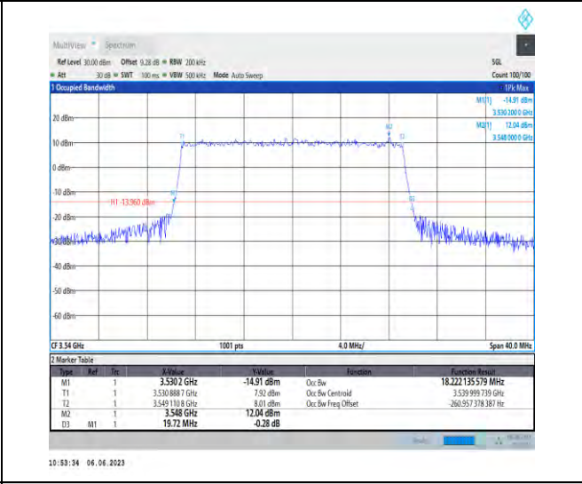
1-N78-3450-3550-PC3-30-20-H-8-CP-64QAM-Outer _Full-51@0-Ant1-18.222-19.720-≤20-PASS
