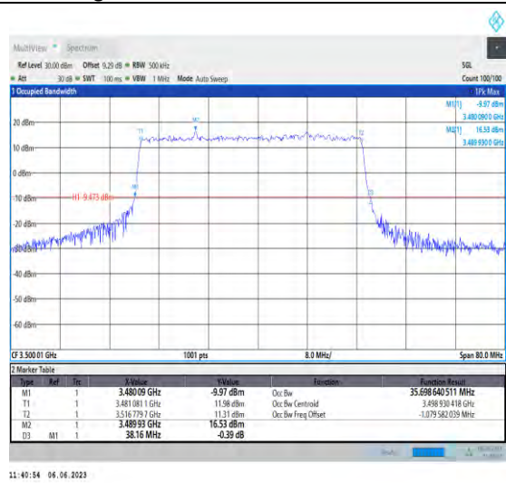
1-N78-3450-3550-PC3-30-40-M-2-DFT-PI2BPSK-Outer_Full-100@0-Ant1-35.699-38.160-≤40-PASS
