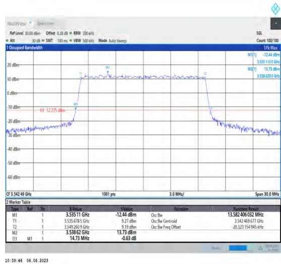
1-N78-3450-3550-PC3-30-15-H-7-CP-16QAM-Outer_Full-38@0-Ant1-13.582-14.730-≤15-PASS
