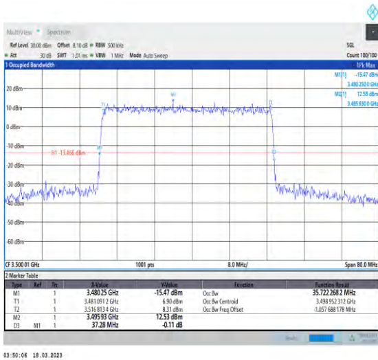
1-N78-3450-3550-PC3-30-40-M-3-DFT-16QAM-Outer_Full-100@0-Ant1-35.722-37.28-≤40-PASS
