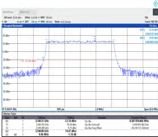
1-N78-3450-3550-PC3-30-10-M-8-CP-64QAM-Outer_Full-24@0-Ant1-8.569-9.400-≤10-PASS
