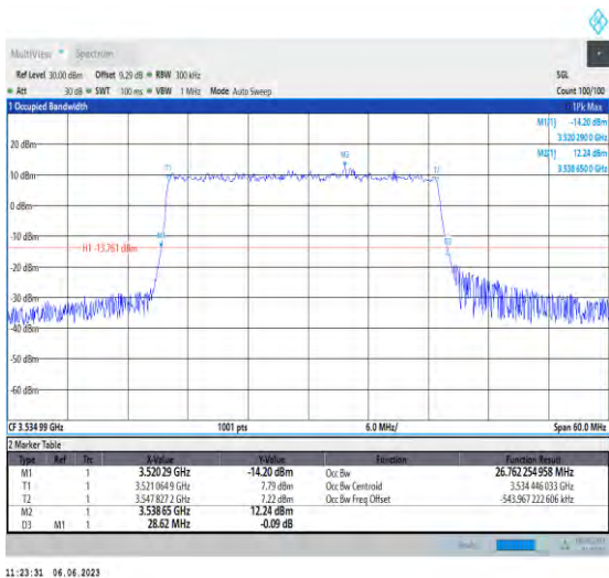
1-N78-3450-3550-PC3-30-30-H-5-DFT-256QAM-Outer_Full-75@0-Ant1-26.762-28.620-≤30-PASS
