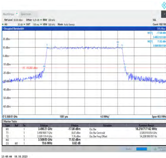
1-N78-3450-3550-PC3-30-20-M-8-CP-64QAM-Outer_Full-51@0-Ant1-18.219-19.600-≤20-PASS
