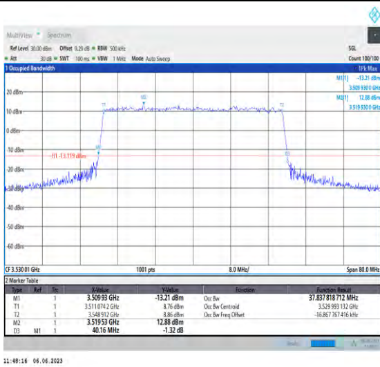
1-N78-3450-3550-PC3-30-40-H-8-CP-64QAM-Outer_Full-106@0-Ant1-37.838-40.160-≤40-PASS
