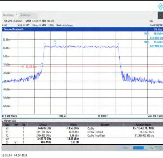
1-N78-3450-3550-PC3-30-50-L-3-DFT-16QAM-Outer_Full-128@0-Ant1-45.716-48.600-≤50-PASS
