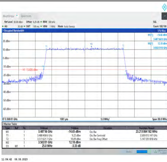
1-N78-3450-3550-PC3-30-25-M-7-CP-16QAM-Outer _Full-65@0-Ant1-23.213-25.000-≤25-PASS
