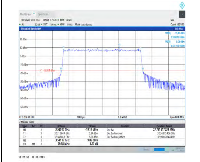
1-N78-3450-3550-PC3-30-30-H-9-CP-256QAM-Outer_Full-78@0-Ant1-27.782-29.580-≤30-PASS
