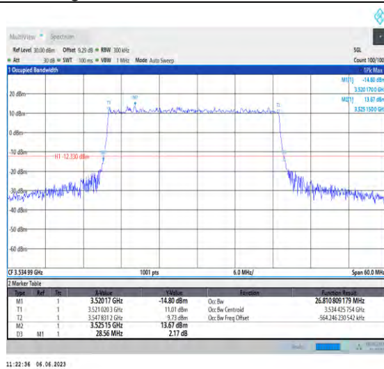
1-N78-3450-3550-PC3-30-30-H-4-DFT-64QAM-Outer_Full-75@0-Ant1-26.811-28.560-≤30-PASS
