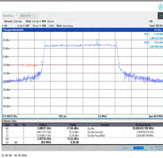
1-N78-3450-3550-PC3-30-40-M-1-DFT-QPSK-Outer_Full-100@0-Ant1-35.69-38.000-≤40-PASS
