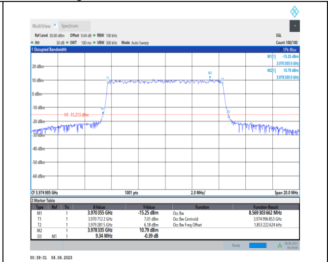
1-N77-3700-3980-PC3-30-10-H-8-CP-64QAM-Outer_Full-24@0-Ant1-8.569-9.340-≤10-PASS
