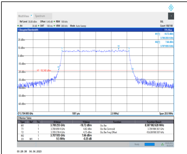
1-N77-3700-3980-PC3-30-10-L-9-CP-256QAM-Outer_Full-24@0-Ant1-8.588-9.500-≤10-PASS
