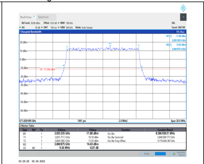
1-N77-3700-3980-PC3-30-10-M-1-DFT-QPSK-Outer_Full-24@0-Ant1-8.587-9.360-≤10-PASS
