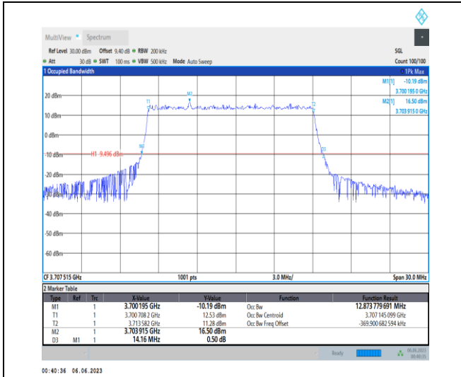
1-N77-3700-3980-PC3-30-15-L-2-DFT-PI2BPSK-Out er_Full-36@0-Ant1-12.874-14.160-≤15-PASS
