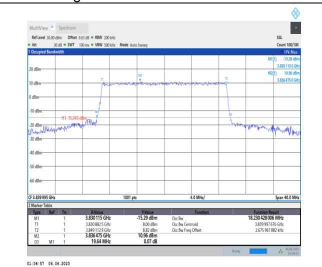
1-N77-3700-3980-PC3-30-20-M-8-CP-64QAM-Outer_Full-51@0-Ant1-18.23-19.640-≤20-PASS
