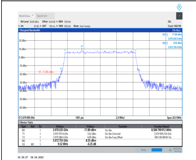
1-N77-3700-3980-PC3-30-10-H-9-CP-256QAM-Outer_Full-24@0-Ant1-8.585-9.520-≤10-PASS
