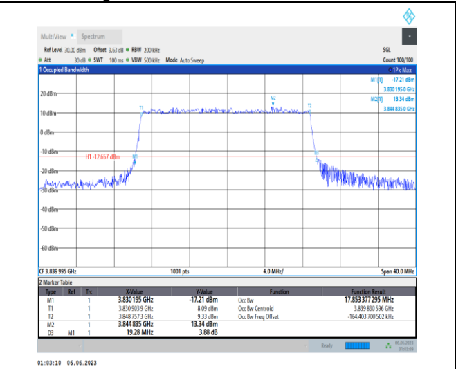
1-N77-3700-3980-PC3-30-20-M-4-DFT-64QAM-Outer_Full-50@0-Ant1-17.853-19.280-≤20-PASS
