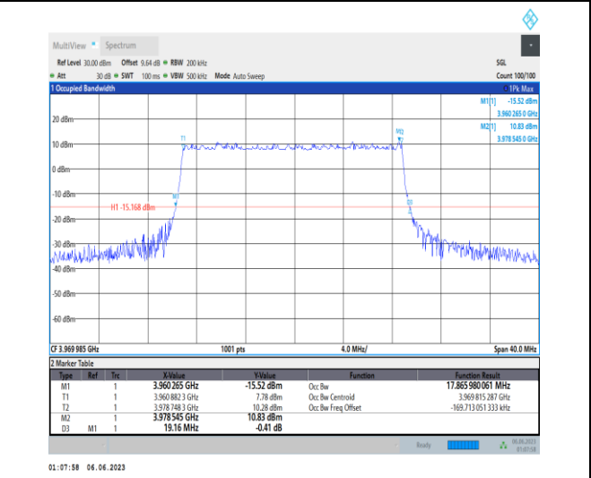
1-N77-3700-3980-PC3-30-20-H-5-DFT-256QAM-Outer_Full-50@0-Ant1-17.866-19.160-≤20-PASS
