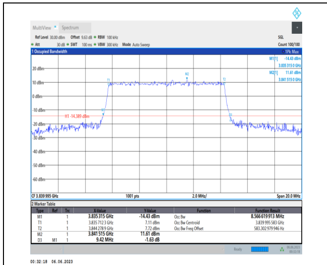
1-N77-3700-3980-PC3-30-10-M-8-CP-64QAM-Outer_Full-24@0-Ant1-8.567-9.420-≤10-PASS
