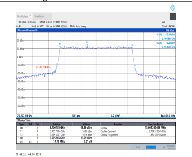
1-N77-3700-3980-PC3-30-15-L-7-CP-16QAM-Outer_Full-38@0-Ant1-13.604-14.730-≤15-PASS
