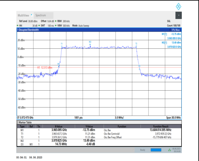
1-N77-3700-3980-PC3-30-15-H-7-CP-16QAM-Outer_Full-38@0-Ant1-13.604-14.730-≤15-PASS
