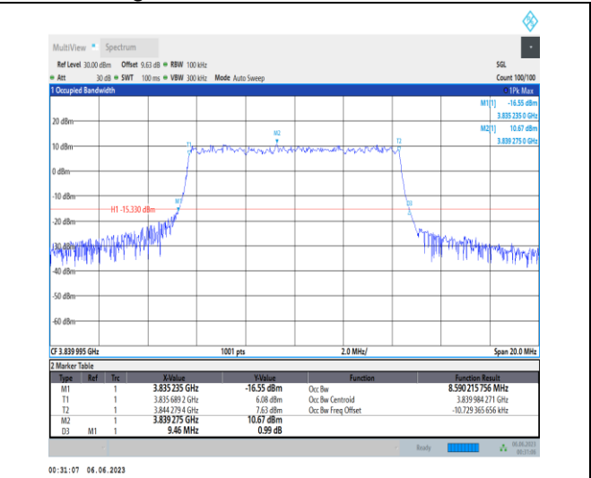
1-N77-3700-3980-PC3-30-10-M-5-DFT-256QAM-Out er_Full-24@0-Ant1-8.59-9.460-≤10-PASS
