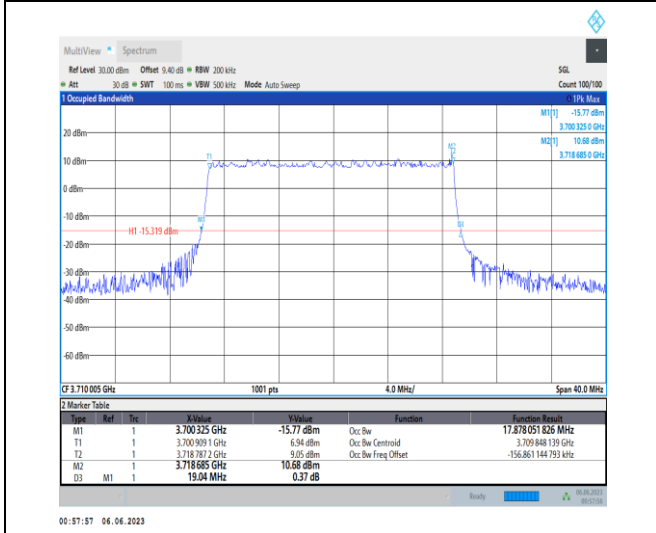
1-N77-3700-3980-PC3-30-20-L-5-DFT-256QAM-Outer_Full-50@0-Ant1-17.878-19.040-≤20-PASS
