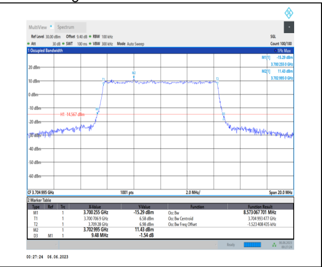
1-N77-3700-3980-PC3-30-10-L-6-CP-QPSK-Outer_Full-24@0-Ant1-8.573-9.480-≤10-PASS
