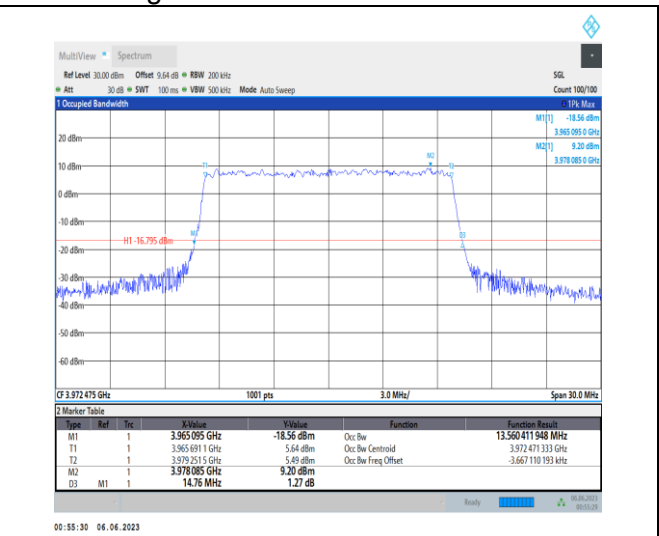
1-N77-3700-3980-PC3-30-15-H-9-CP-256QAM-Outer_Full-38@0-Ant1-13.56-14.760-≤15-PASS
