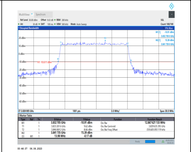
1-N77-3700-3980-PC3-30-15-M-4-DFT-64QAM-Outer_Full-36@0-Ant1-12.868-13.980-≤15-PASS
