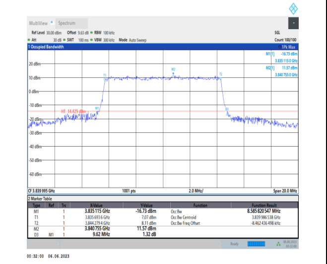
1-N77-3700-3980-PC3-30-10-M-7-CP-16QAM-Outer _Full-24@0-Ant1-8.586-9.620-≤10-PASS
