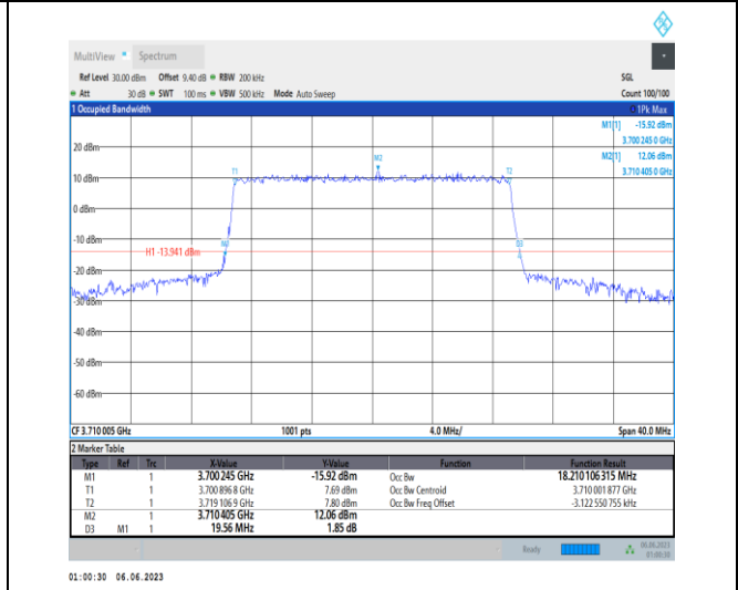
1-N77-3700-3980-PC3-30-20-L-7-CP-16QAM-Outer_Full-51@0-Ant1-18.21-19.560-≤20-PASS
