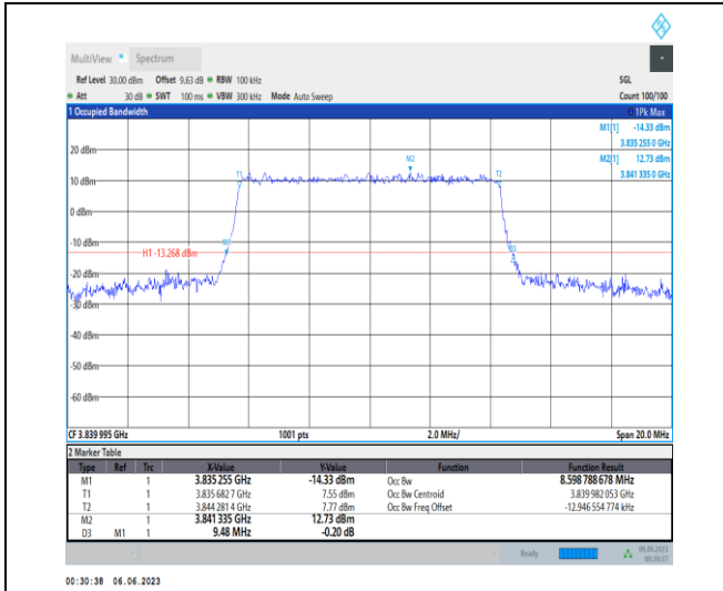
1-N77-3700-3980-PC3-30-10-M-4-DFT-64QAM-Out er_Full-24@0-Ant1-8.599-9.480-≤10-PASS
