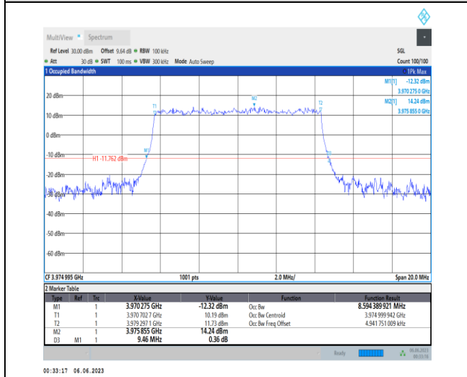
1-N77-3700-3980-PC3-30-10-H-1-DFT-QPSK-Outer_Full-24@0-Ant1-8.594-9.460-≤10-PASS
