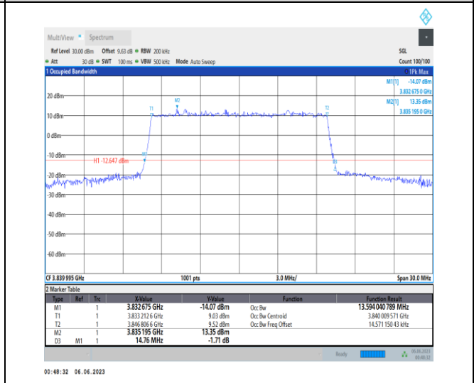
1-N77-3700-3980-PC3-30-15-M-8-CP-64QAM-Outer_Full-38@0-Ant1-13.594-14.760-≤15-PASS
