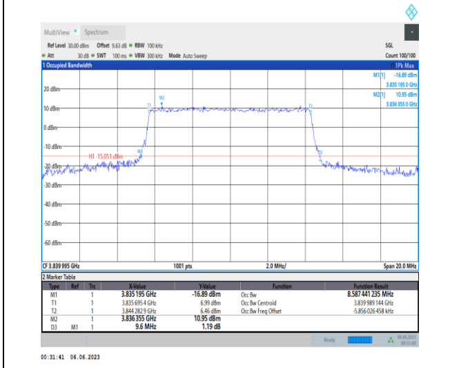
1-N77-3700-3980-PC3-30-10-M-6-CP-QPSK-Outer Full-24@0-Ant1-8.587-9.600-≤10-PASS
