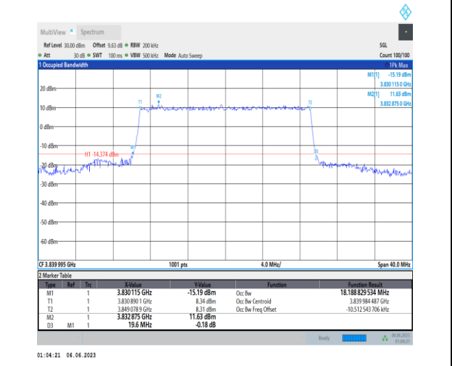
1-N77-3700-3980-PC3-30-20-M-6-CP-QPSK-Outer_Full-51@0-Ant1-18.189-19.600-≤20-PASS
