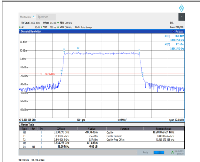
1-N77-3700-3980-PC3-30-20-M-9-CP-256QAM-Outer_Full-51@0-Ant1-18.202-19.560-≤20-PASS
