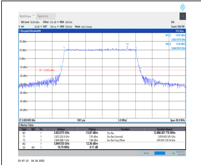
1-N77-3700-3980-PC3-30-15-M-5-DFT-256QAM-Outer_Full-36@0-Ant1-12.886-14.190-≤15-PASS
