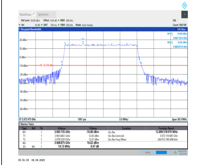
1-N77-3700-3980-PC3-30-15-H-2-DFT-PI2BPSK-Outer_Full-36@0-Ant1-12.9-14.130-≤15-PASS
