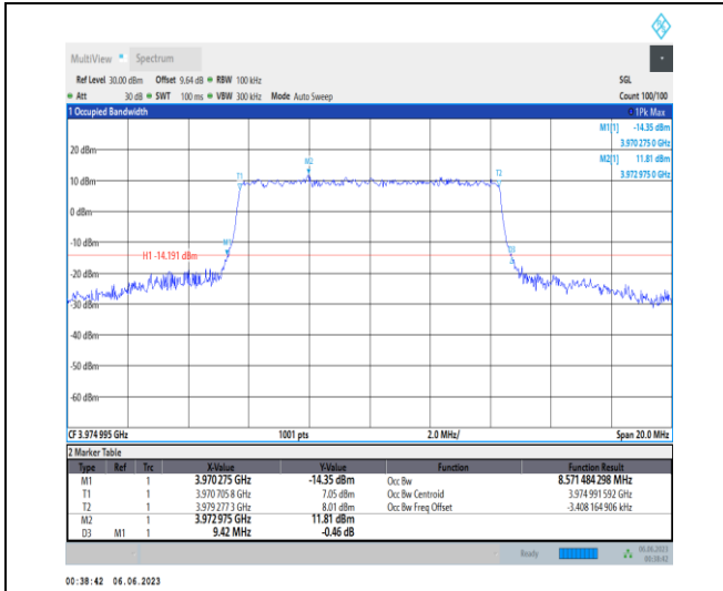
1-N77-3700-3980-PC3-30-10-H-7-CP-16QAM-Outer_Full-24@0-Ant1-8.571-9.420-≤10-PASS
