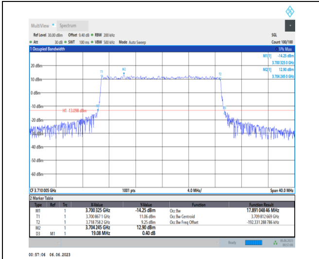
1-N77-3700-3980-PC3-30-20-L-3-DFT-16QAM-Outer_Full-50@0-Ant1-17.891-19.080-≤20-PASS
