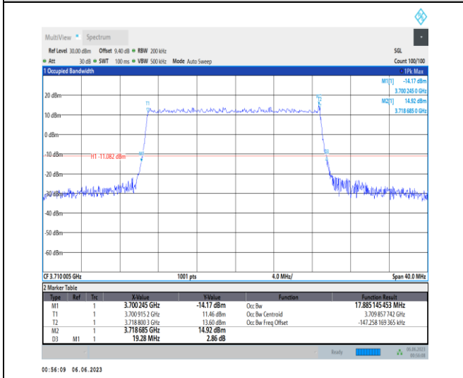
1-N77-3700-3980-PC3-30-20-L-1-DFT-QPSK-Outer_Full-50@0-Ant1-17.885-19.280-≤20-PASS
