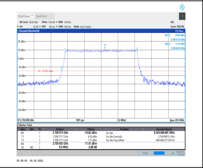
1-N77-3700-3980-PC3-30-10-L-8-CP-64QAM-Outer_Full-24@0-Ant1-8.566-9.400-≤10-PASS
