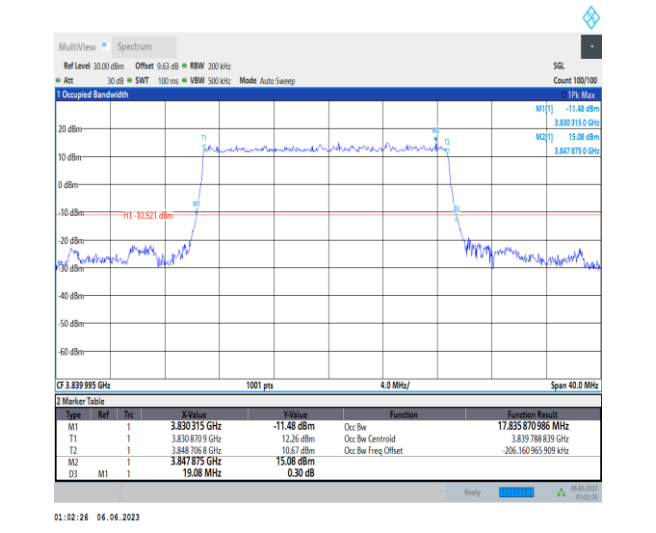
1-N77-3700-3980-PC3-30-20-M-2-DFT-PI2BPSK-Outer_Full-50@0-Ant1-17.836-19.080-≤20-PASS
