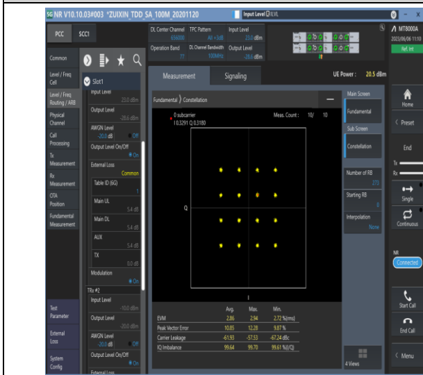
1-N77-3700-3980-PC3-30-100-M-7-CP-16QAM-Outer_Full-273@0-Ant1-see graph-PASS
