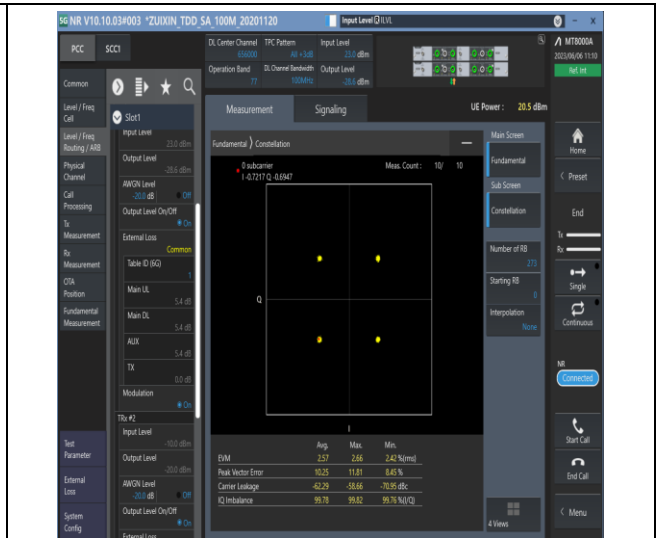
1-N77-3700-3980-PC3-30-100-M-6-CP-QPSK-Outer_Full-273@0-Ant1-see graph-PASS
