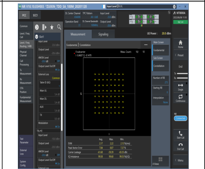
1-N77-3700-3980-PC3-30-100-M-8-CP-64QAM-Outer_Full-273@0-Ant1-see graph-PASS
