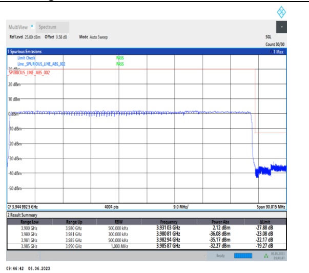
1-N77-3700-3980-PC3-30-80-H-3-DFT-PI2BPSK-Outer_Full-216@0-Ant1-1--PASS-see graph
