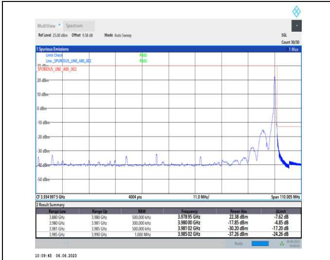
1-N77-3700-3980-PC3-30-100-H-2-DFT-PI2BPSK-Edge_1_RB_Right-1@272-Ant1-1--PASS-see graph
