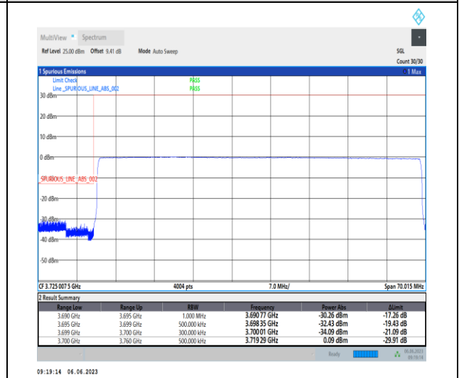
1-N77-3700-3980-PC3-30-60-L-6-CP-QPSK-Outer_Full-162@0-Ant1-1--PASS-see graph
