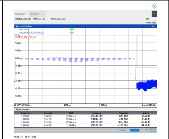
1-N77-3700-3980-PC3-30-60-H-6-CP-QPSK-Outer_Full-162@0-Ant1-1--PASS-see graph
