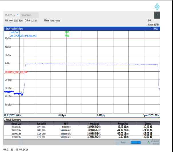
1-N77-3700-3980-PC3-30-70-L-6-CP-QPSK-Outer_Full-189@0-Ant1-1--PASS-see graph
