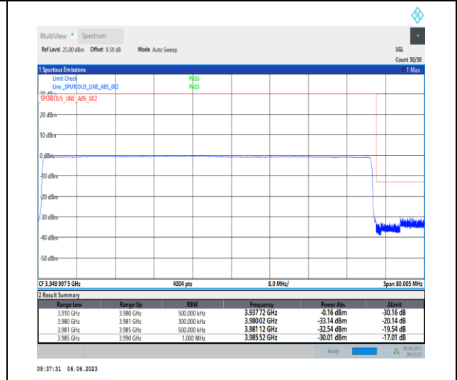
1-N77-3700-3980-PC3-30-70-H-6-CP-QPSK-Outer_Full-189@0-Ant1-1--PASS-see graph
