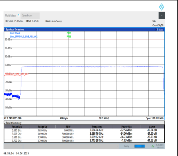
1-N77-3700-3980-PC3-30-90-L-6-CP-QPSK-Outer_Full-245@0-Ant1-1--PASS-see graph
