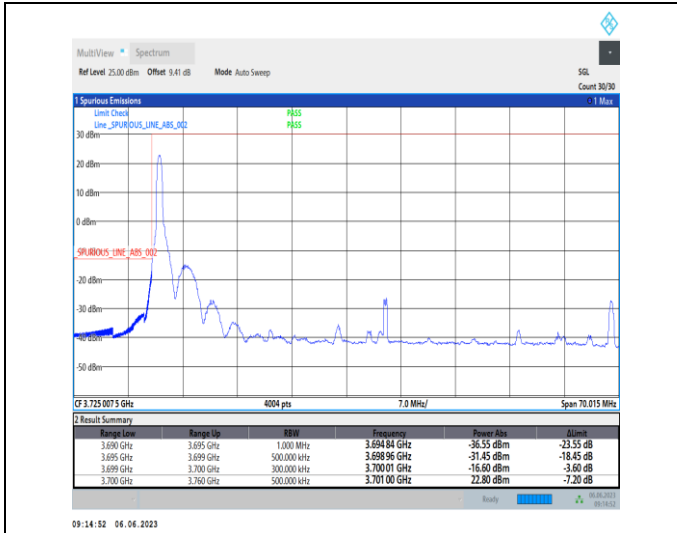
1-N77-3700-3980-PC3-30-60-L-1-DFT-PI2BPSK-Edge_1RB_Left-1@0-Ant1-1--PASS-see graph
