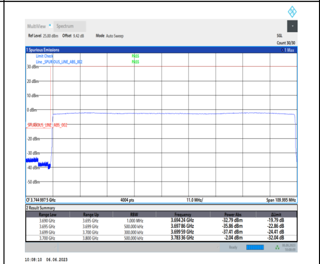
1-N77-3700-3980-PC3-30-100-L-6-CP-QPSK-Outer_Full-273@0-Ant1-1--PASS-see graph
