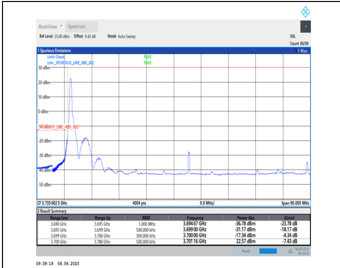
1-N77-3700-3980-PC3-30-80-L-1-DFT-PI2BPSK-Edge_1RB_Left-1@0-Ant1-1--PASS-see graph
