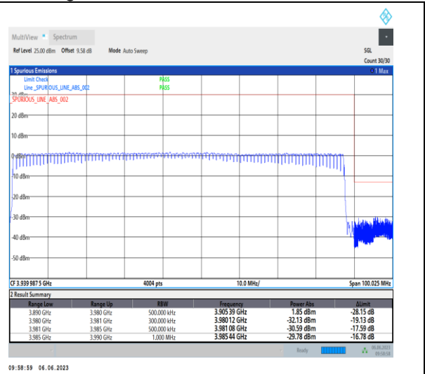
1-N77-3700-3980-PC3-30-90-H-3-DFT-PI2BPSK-Outer_Full-240@0-Ant1-1--PASS-see graph
