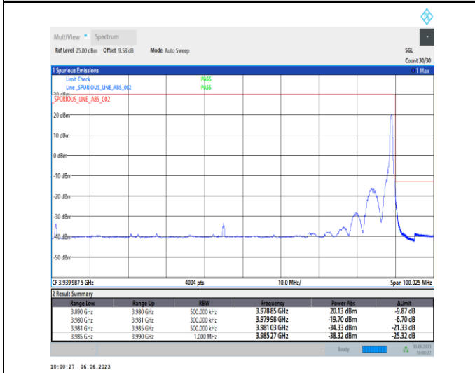
1-N77-3700-3980-PC3-30-90-H-5-CP-QPSK-Edge_1RB_Right-1@244-Ant1-1--PASS-see graph
