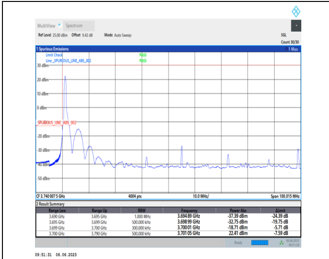
1-N77-3700-3980-PC3-30-90-L-1-DFT-PI2BPSK-Edge_1RB_Left-1@0-Ant1-1--PASS-see graph
