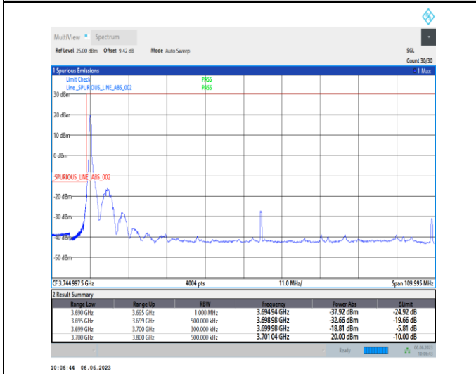
1-N77-3700-3980-PC3-30-100-L-4-CP-QPSK-Edge_1RB_Left-1@0-Ant1-1--PASS-see graph
