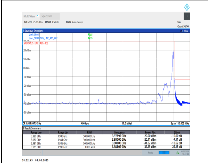
1-N77-3700-3980-PC3-30-100-H-5-CP-QPSK-Edge_1_RB_Right-1@272-Ant1-1--PASS-see graph
