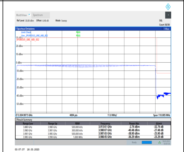
1-N77-3700-3980-PC3-30-100-H-6-CP-QPSK-Outer_Full-273@0-Ant1-1--PASS-see graph
