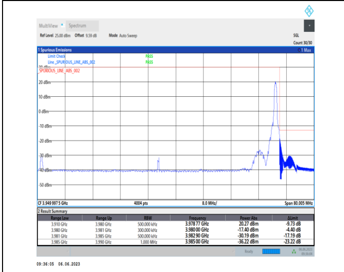
1-N77-3700-3980-PC3-30-70-H-5-CP-QPSK-Edge_1RB_Right-1@188-Ant1-1--PASS-see graph
