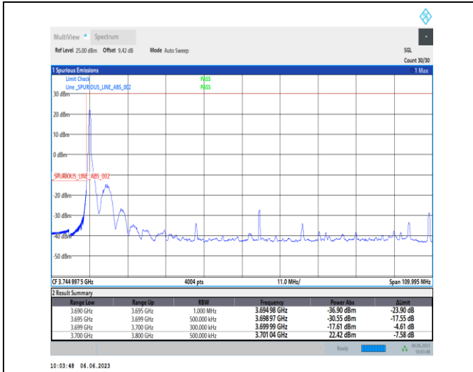
1-N77-3700-3980-PC3-30-100-L-1-DFT-PI2BPSK-Edge_1RB_Left-1@0-Ant1-1--PASS-see graph
