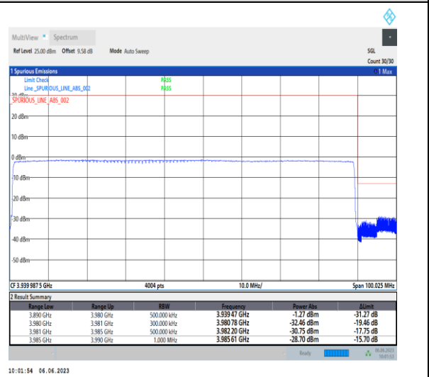
1-N77-3700-3980-PC3-30-90-H-6-CP-QPSK-Outer_Full-245@0-Ant1-1--PASS-see graph
