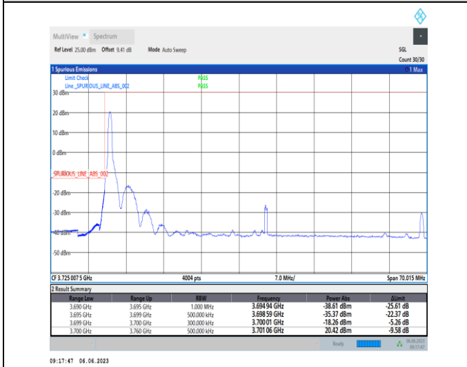
1-N77-3700-3980-PC3-30-60-L-4-CP-QPSK-Edge_1RB_Left-1@0-Ant1-1--PASS-see graph
