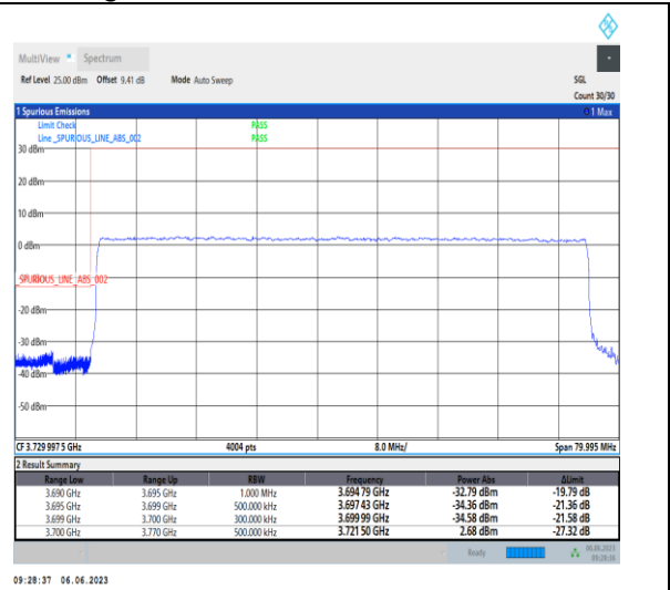
1-N77-3700-3980-PC3-30-70-L-3-DFT-PI2BPSK-Outer_Full-180@0-Ant1-1--PASS-see graph
