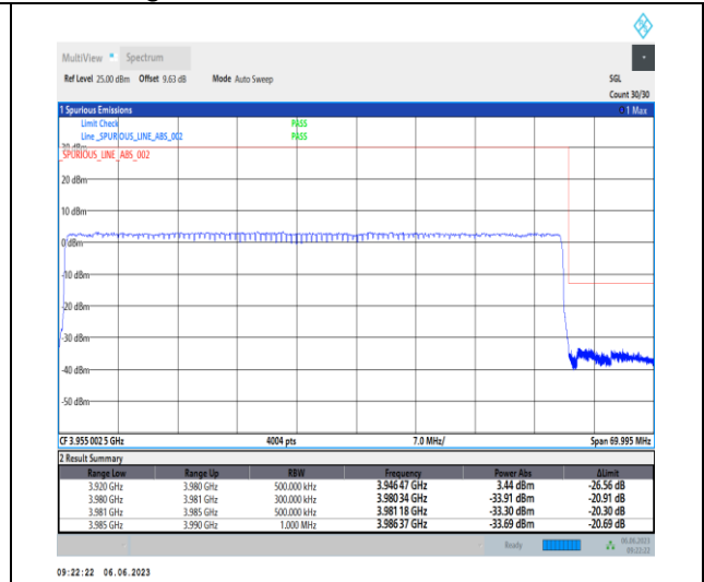
1-N77-3700-3980-PC3-30-60-H-3-DFT-PI2BPSK-Outer_Full-162@0-Ant1-1--PASS-see graph
