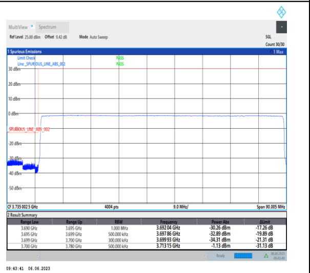
1-N77-3700-3980-PC3-30-80-L-6-CP-QPSK-Outer_Full-217@0-Ant1-1--PASS-see graph
