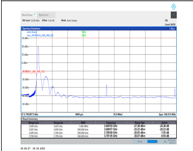
1-N77-3700-3980-PC3-30-90-L-4-CP-QPSK-Edge_1RB_Left-1@0-Ant1-1--PASS-see graph
