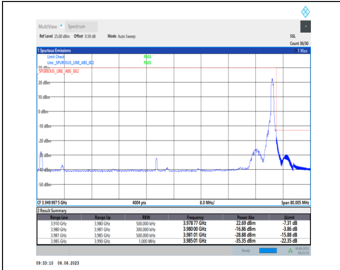
1-N77-3700-3980-PC3-30-70-H-2-DFT-PI2BPSK-Edge_1RB_Right-1@188-Ant1-1--PASS-see graph
