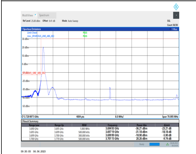
1-N77-3700-3980-PC3-30-70-L-4-CP-QPSK-Edge_1RB_Left-1@0-Ant1-1--PASS-see graph
