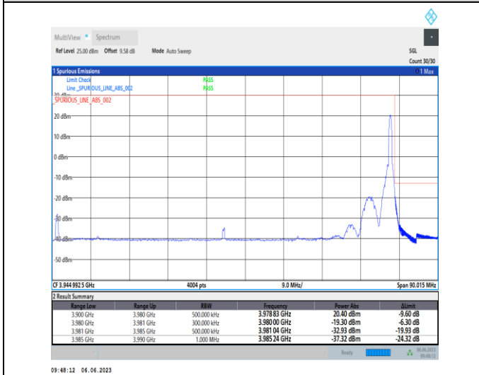
1-N77-3700-3980-PC3-30-80-H-5-CP-QPSK-Edge_1RB_Right-1@216-Ant1-1--PASS-see graph
