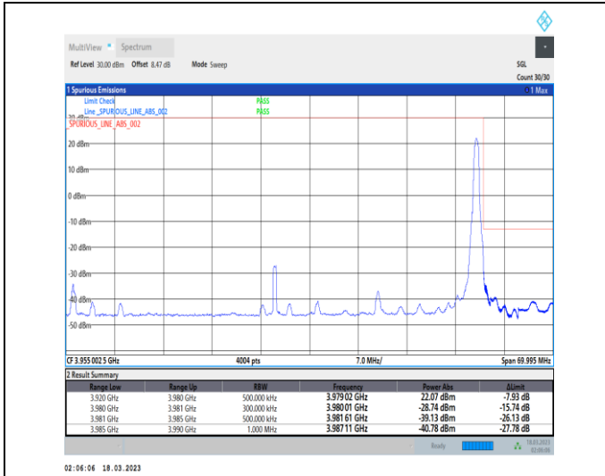
1-N77-3700-3980-PC3-30-60-H-2-DFT-PI2BPSK-Edge_1RB_Right-1@161-Ant1-1--PASS-see graph
