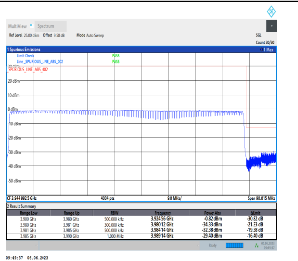
1-N77-3700-3980-PC3-30-80-H-6-CP-QPSK-Outer_Full-217@0-Ant1-1--PASS-see graph
