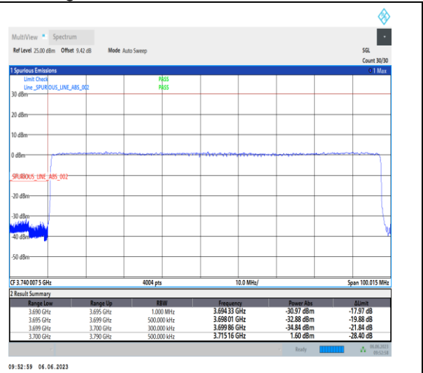
1-N77-3700-3980-PC3-30-90-L-3-DFT-PI2BPSK-Outer_Full-240@0-Ant1-1--PASS-see graph
