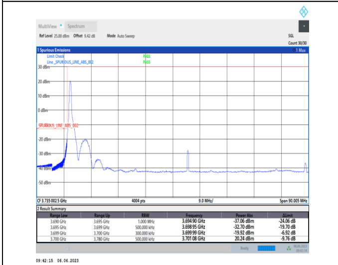
1-N77-3700-3980-PC3-30-80-L-4-CP-QPSK-Edge_1RB_Left-1@0-Ant1-1--PASS-see graph
