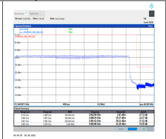
1-N77-3700-3980-PC3-30-70-H-3-DFT-PI2BPSK-Outer_Full-180@0-Ant1-1--PASS-see graph
