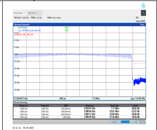
1-N77-3700-3980-PC3-30-100-H-3-DFT-PI2BPSK-Outer_Full-270@0-Ant1-1--PASS-see graph
