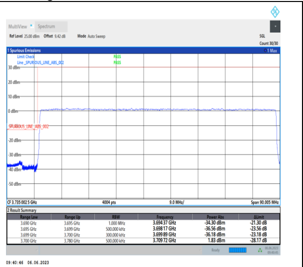
1-N77-3700-3980-PC3-30-80-L-3-DFT-PI2BPSK-Outer_Full-216@0-Ant1-1--PASS-see graph
