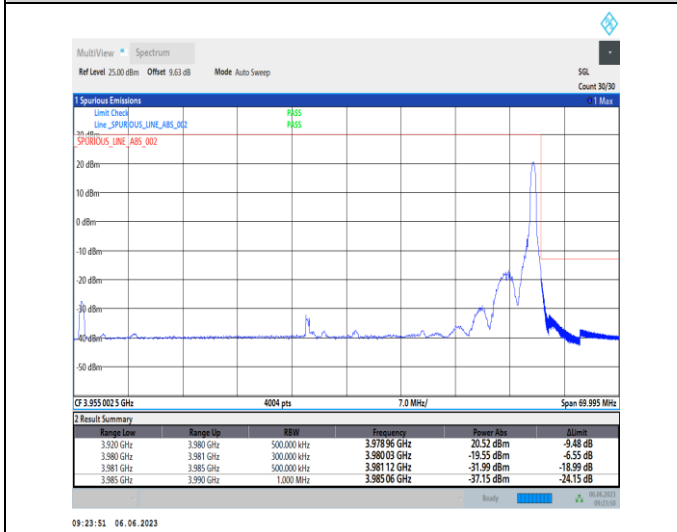
1-N77-3700-3980-PC3-30-60-H-5-CP-QPSK-Edge_1RB_Right-1@161-Ant1-1--PASS-see graph
