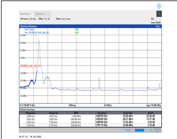
1-N77-3700-3980-PC3-30-70-L-1-DFT-PI2BPSK-Edge_1RB_Left-1@0-Ant1-1--PASS-see graph
