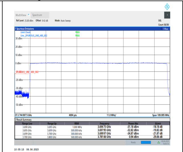
1-N77-3700-3980-PC3-30-100-L-3-DFT-PI2BPSK-Outer_Full-270@0-Ant1-1--PASS-see graph
