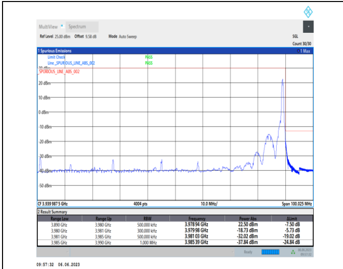
1-N77-3700-3980-PC3-30-90-H-2-DFT-PI2BPSK-Edge_1RB_Right-1@244-Ant1-1--PASS-see graph
