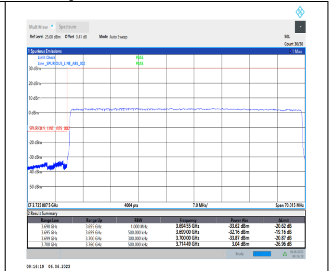
1-N77-3700-3980-PC3-30-60-L-3-DFT-PI2BPSK-Outer_Full-162@0-Ant1-1--PASS-see graph
