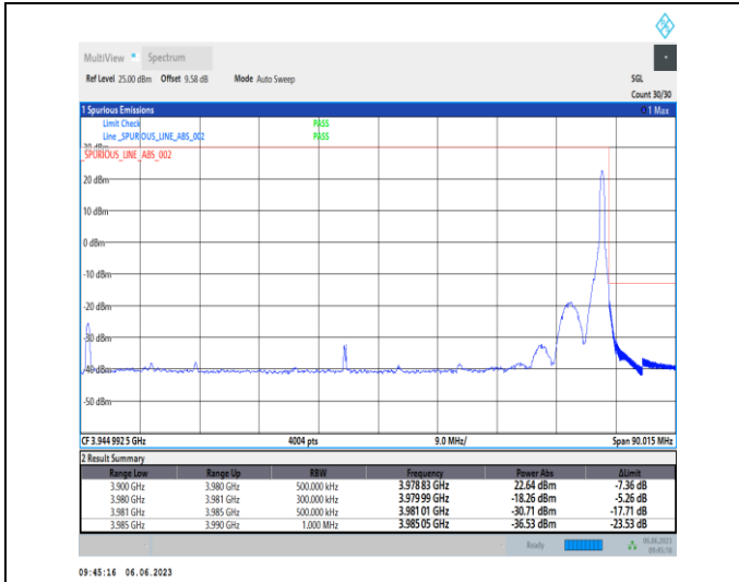
1-N77-3700-3980-PC3-30-80-H-2-DFT-PI2BPSK-Edge_1RB_Right-1@216-Ant1-1--PASS-see graph
