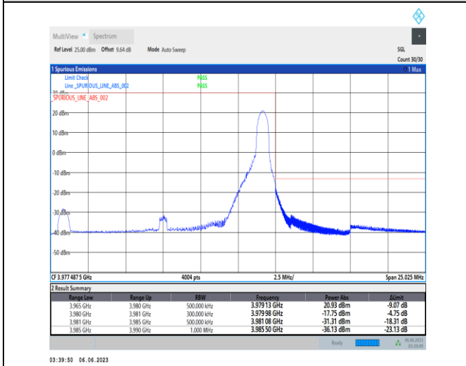
1-N77-3700-3980-PC3-30-15-H-5-CP-QPSK-Edge_1RB_Right-1@37-Ant1-1--PASS-see graph
