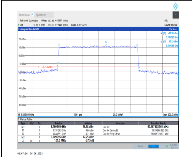
1-N77-3700-3980-PC3-30-100-M-6-CP-QPSK-Outer_Full-273@0-Ant1-97.168-101.000-≤100-PASS
