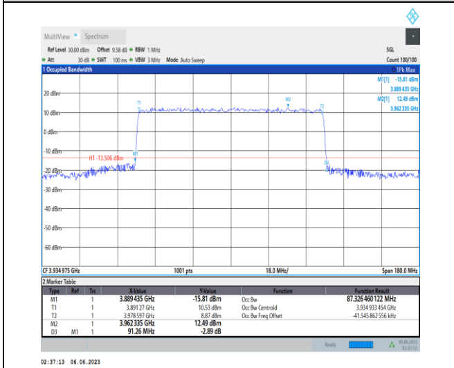
1-N77-3700-3980-PC3-30-90-H-7-CP-16QAM-Outer _Full-245@0-Ant1-87.326-91.260-≤90-PASS
