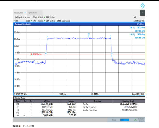
1-N77-3700-3980-PC3-30-100-H-4-DFT-64QAM-Out er_Full-270@0-Ant1-96.066-100.200-≤100-PASS
