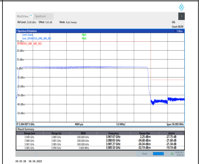
1-N77-3700-3980-PC3-30-40-H-6-CP-QPSK-Outer_Full-106@0-Ant1-1--PASS-see graph
