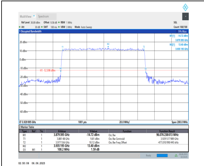
1-N77-3700-3980-PC3-30-100-H-3-DFT-16QAM-Out er_Full-270@0-Ant1-96.076-100.200-≤100-PASS
