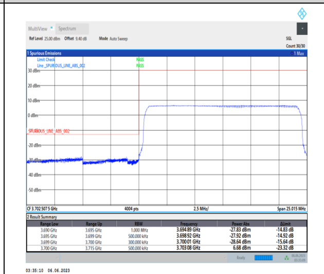
1-N77-3700-3980-PC3-30-15-L-6-CP-QPSK-Outer_Full-38@0-Ant1-1--PASS-see graph
