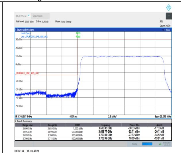
1-N77-3700-3980-PC3-30-15-L-3-DFT-PI2BPSK-Outer_Full-36@0-Ant1-1--PASS-see graph
