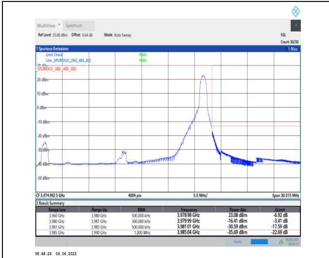
1-N77-3700-3980-PC3-30-20-H-2-DFT-PI2BPSK-Edge_1RB_Right-1@50-Ant1-1--PASS-see graph
