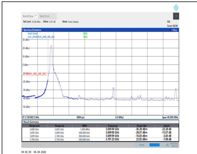
1-N77-3700-3980-PC3-30-50-L-1-DFT-PI2BPSK-Edge_1RB_Left-1@0-Ant1-1--PASS-see graph
