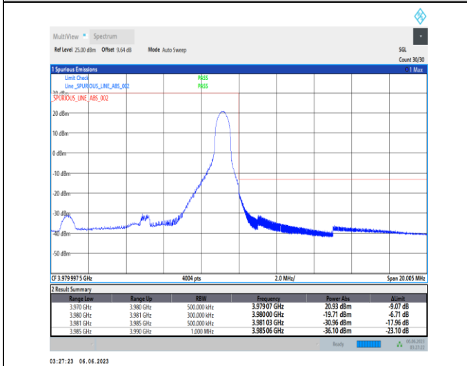
1-N77-3700-3980-PC3-30-10-H-5-CP-QPSK-Edge_1RB_Right-1@23-Ant1-1--PASS-see graph
