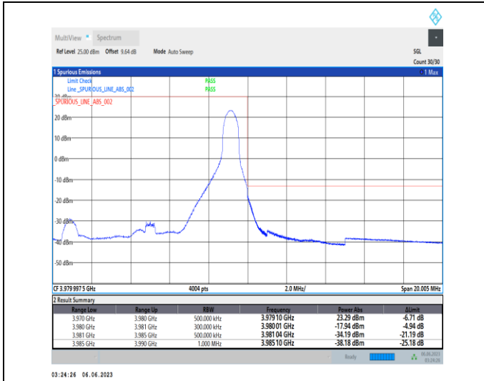
1-N77-3700-3980-PC3-30-10-H-2-DFT-PI2BPSK-Edge_1RB_Right-1@23-Ant1-1--PASS-see graph
