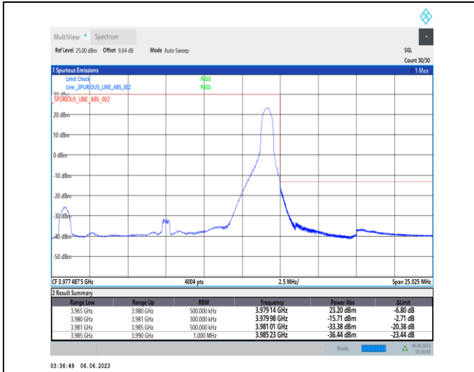
1-N77-3700-3980-PC3-30-15-H-2-DFT-PI2BPSK-Edge_1RB_Right-1@37-Ant1-1--PASS-see graph
