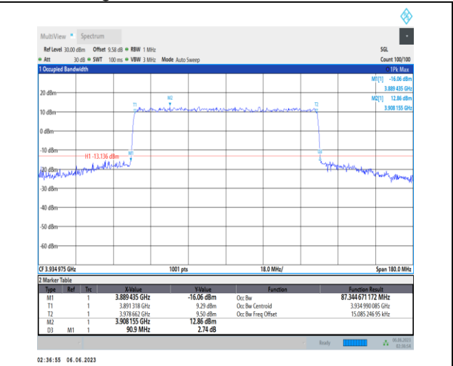
1-N77-3700-3980-PC3-30-90-H-6-CP-QPSK-Outer Full-245@0-Ant1-87.345-90.900-≤90-PASS
