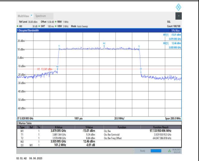
1-N77-3700-3980-PC3-30-100-H-6-CP-QPSK-Outer_Full-273@0-Ant1-97.134-101.200-≤100-PASS
