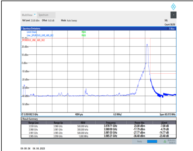
1-N77-3700-3980-PC3-30-50-H-2-DFT-PI2BPSK-Edge_1RB_Right-1@132-Ant1-1--PASS-see graph
