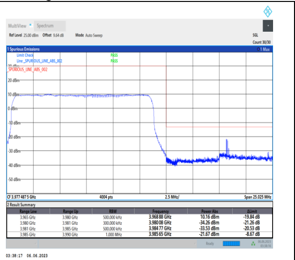
1-N77-3700-3980-PC3-30-15-H-3-DFT-PI2BPSK-Outer_Full-36@0-Ant1-1--PASS-see graph
