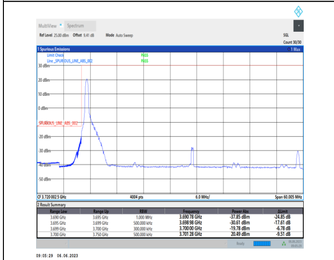
1-N77-3700-3980-PC3-30-50-L-4-CP-QPSK-Edge_1RB_Left-1@0-Ant1-1--PASS-see graph
