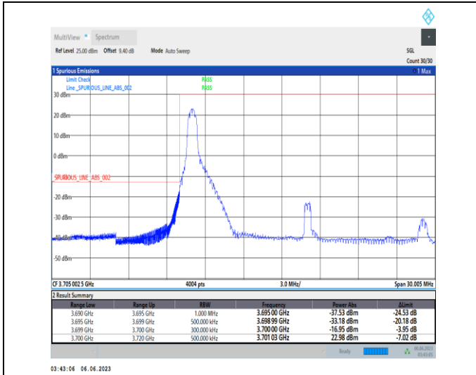
1-N77-3700-3980-PC3-30-20-L-1-DFT-PI2BPSK-Edge_1RB_Left-1@0-Ant1-1--PASS-see graph
