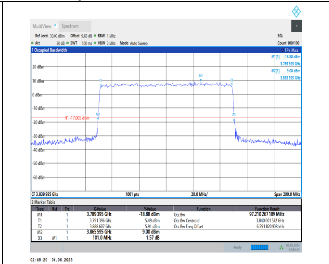
1-N77-3700-3980-PC3-30-100-M-9-CP-256QAM-Out er_Full-273@0-Ant1-97.21-101.000-≤100-PASS
