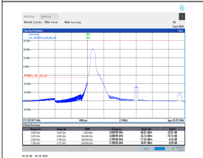
1-N77-3700-3980-PC3-30-15-L-4-CP-QPSK-Edge_1RB_Left-1@0-Ant1-1--PASS-see graph
