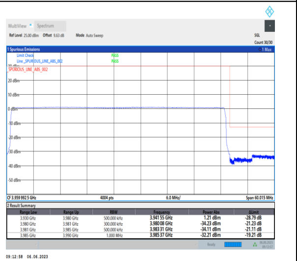
1-N77-3700-3980-PC3-30-50-H-6-CP-QPSK-Outer_Full-133@0-Ant1-1--PASS-see graph
