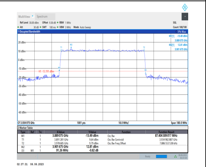
1-N77-3700-3980-PC3-30-90-H-8-CP-64QAM-Outer _Full-245@0-Ant1-87.404-91.260-≤90-PASS
