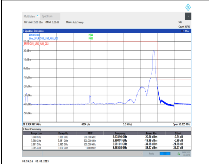
1-N77-3700-3980-PC3-30-40-H-5-CP-QPSK-Edge_1RB_Right-1@105-Ant1-1--PASS-see graph
