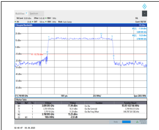
1-N77-3700-3980-PC3-30-100-L-1-DFT-QPSK-Outer_Full-270@0-Ant1-95.951-100.400-≤100-PASS
