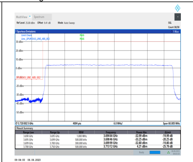
1-N77-3700-3980-PC3-30-50-L-3-DFT-PI2BPSK-Outer_Full-128@0-Ant1-1--PASS-see graph
