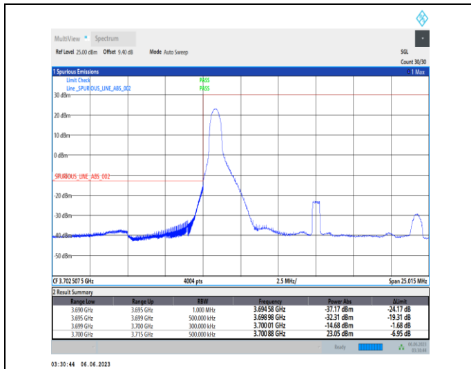
1-N77-3700-3980-PC3-30-15-L-1-DFT-PI2BPSK-Edge_1RB_Left-1@0-Ant1-1--PASS-see graph
