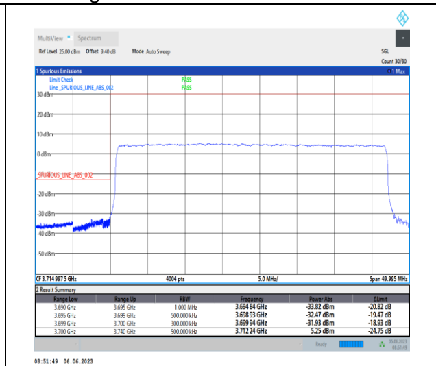
1-N77-3700-3980-PC3-30-40-L-3-DFT-PI2BPSK-Outer_Full-100@0-Ant1-1--PASS-see graph
