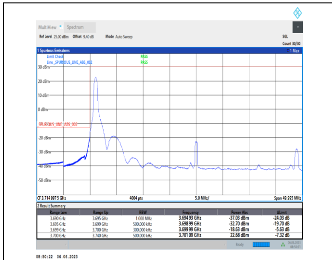
1-N77-3700-3980-PC3-30-40-L-1-DFT-PI2BPSK-Edge_1RB_Left-1@0-Ant1-1--PASS-see graph
