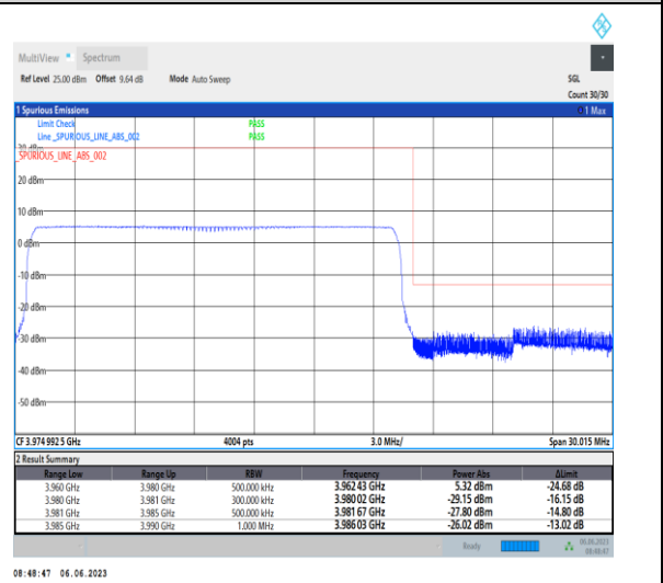
1-N77-3700-3980-PC3-30-20-H-6-CP-QPSK-Outer_Full-51@0-Ant1-1--PASS-see graph
