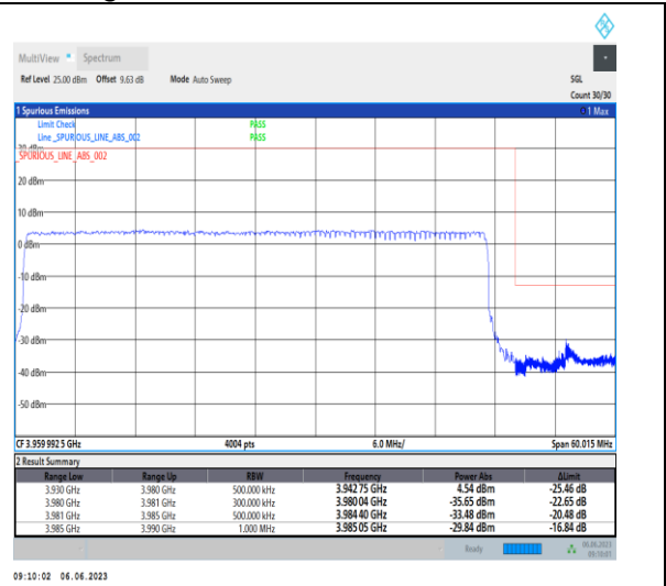
1-N77-3700-3980-PC3-30-50-H-3-DFT-PI2BPSK-Outer_Full-128@0-Ant1-1--PASS-see graph
