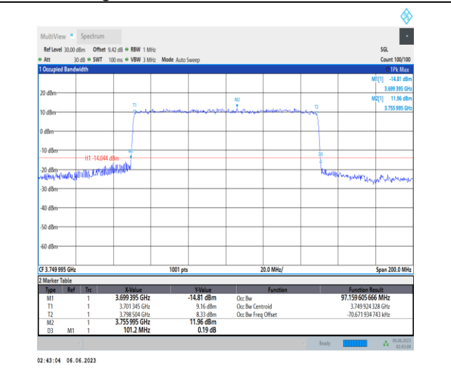
1-N77-3700-3980-PC3-30-100-L-6-CP-QPSK-Outer_Full-273@0-Ant1-97.16-101.200-≤100-PASS
