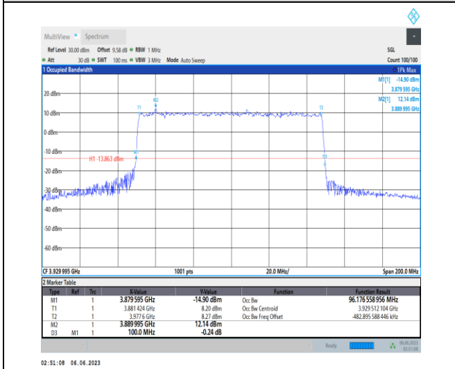
1-N77-3700-3980-PC3-30-100-H-5-DFT-256QAM-Outer_Full-270@0-Ant1-96.177-100.000-≤100-PASS
