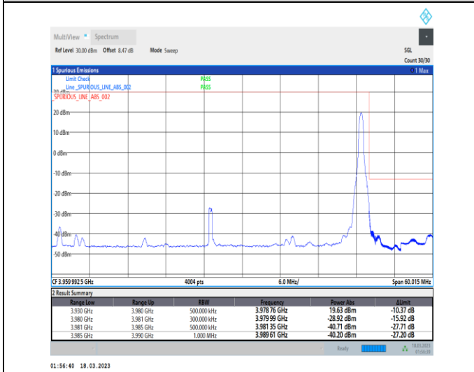
1-N77-3700-3980-PC3-30-50-H-5-CP-QPSK-Edge_1RB_Right-1@132-Ant1-1--PASS-see graph
