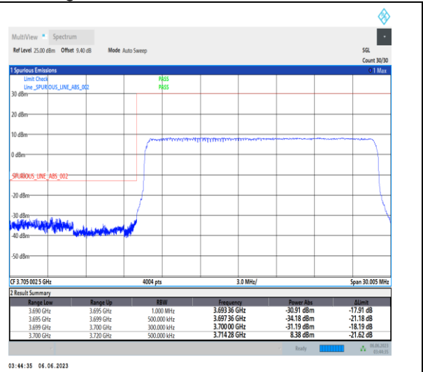
1-N77-3700-3980-PC3-30-20-L-3-DFT-PI2BPSK-Outer_Full-50@0-Ant1-1--PASS-see graph
