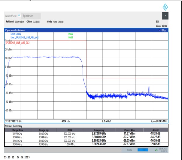
1-N77-3700-3980-PC3-30-10-H-3-DFT-PI2BPSK-Outer_Full-24@0-Ant1-1--PASS-see graph
