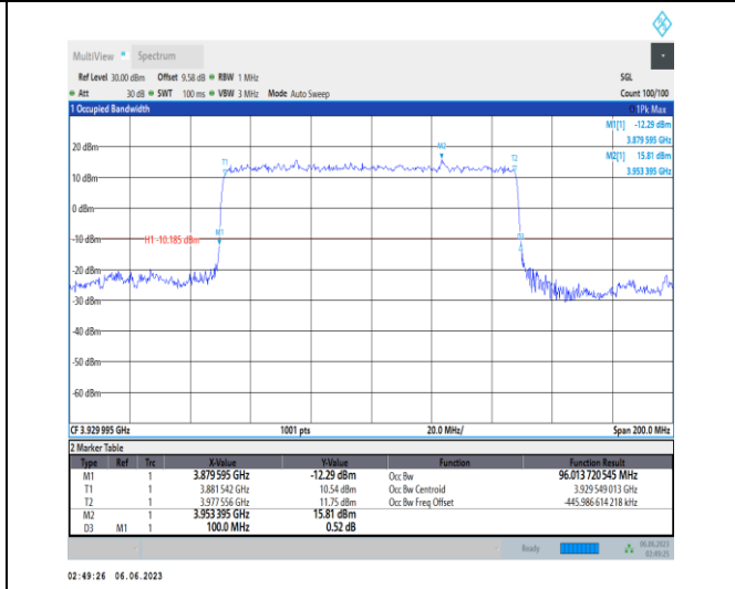
1-N77-3700-3980-PC3-30-100-H-2-DFT-PI2BPSK-Out er_Full-270@0-Ant1-96.014-100.000-≤100-PASS
