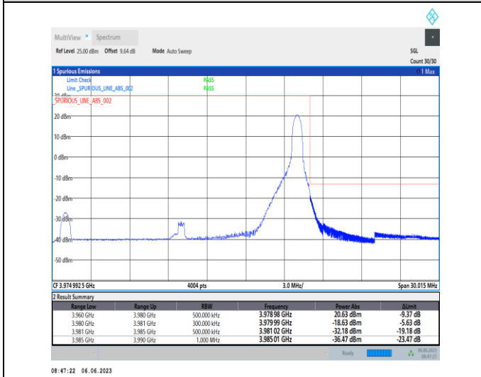
1-N77-3700-3980-PC3-30-20-H-5-CP-QPSK-Edge_1RB_Right-1@50-Ant1-1--PASS-see graph
