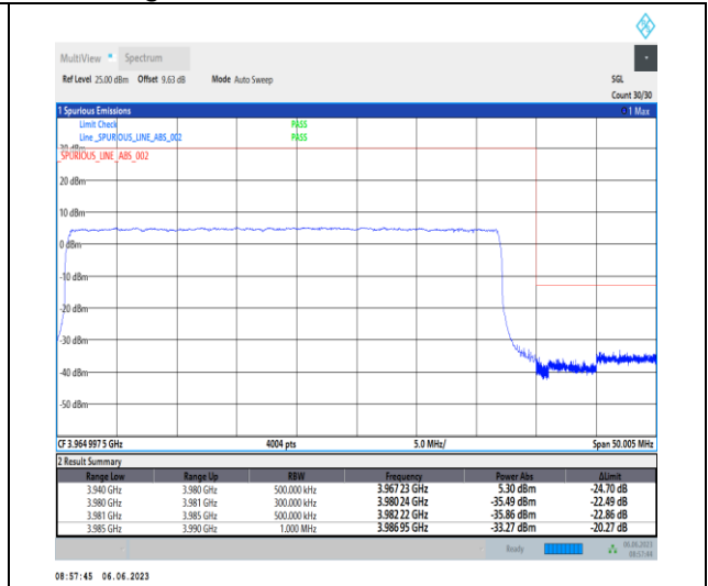
1-N77-3700-3980-PC3-30-40-H-3-DFT-PI2BPSK-Outer_Full-100@0-Ant1-1--PASS-see graph
