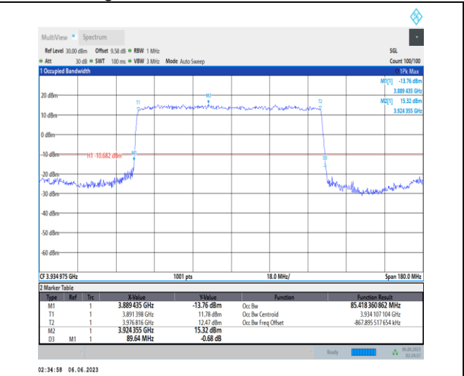
1-N77-3700-3980-PC3-30-90-H-2-DFT-PI2BPSK-Outer_Full-240@0-Ant1-85.418-89.640-≤90-PASS
