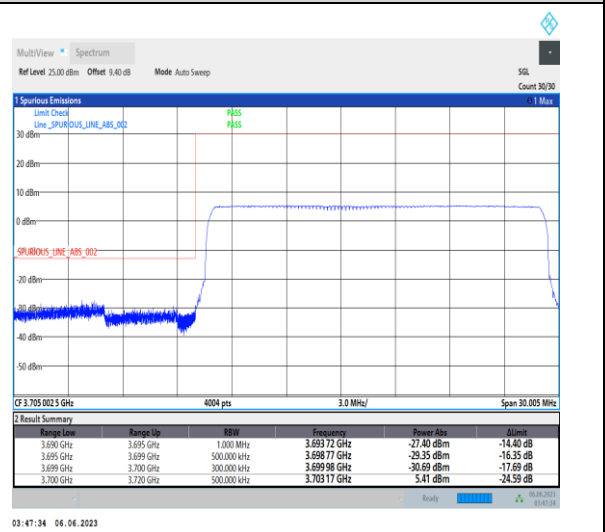
1-N77-3700-3980-PC3-30-20-L-6-CP-QPSK-Outer_Full-51@0-Ant1-1--PASS-see graph
