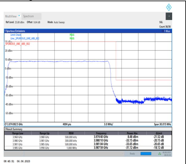
1-N77-3700-3980-PC3-30-20-H-3-DFT-PI2BPSK-Outer_Full-50@0-Ant1-1--PASS-see graph
