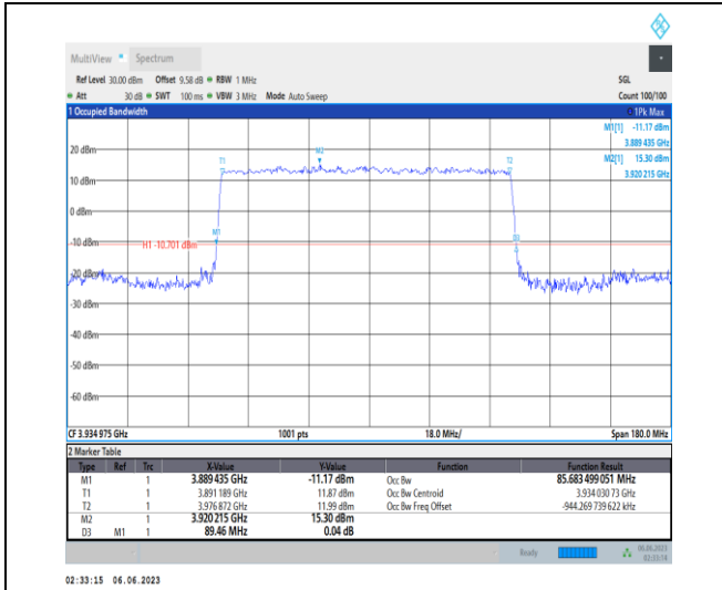
1-N77-3700-3980-PC3-30-90-H-1-DFT-QPSK-Outer_Full-240@0-Ant1-85.683-89.460-≤90-PASS
