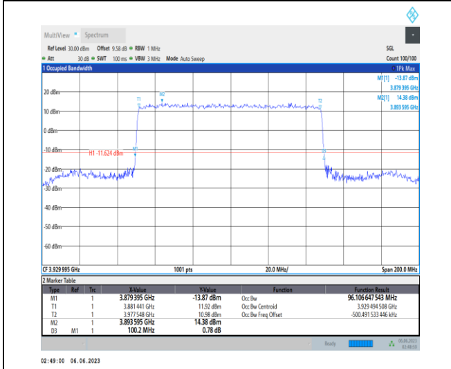
1-N77-3700-3980-PC3-30-100-H-1-DFT-QPSK-Out er_Full-270@0-Ant1-96.107-100.200-≤100-PASS
