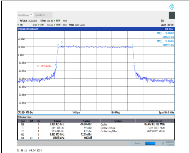
1-N77-3700-3980-PC3-30-90-H-5-DFT-256QAM-Out er_Full-240@0-Ant1-85.478-89.640-≤90-PASS
