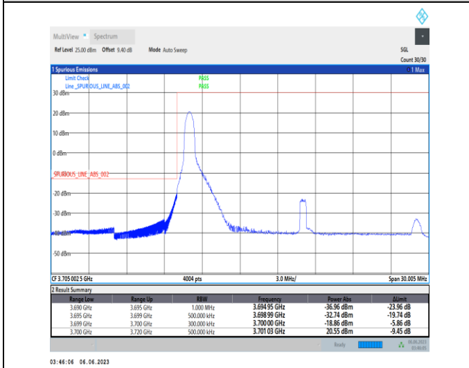
1-N77-3700-3980-PC3-30-20-L-4-CP-QPSK-Edge_1RB_Left-1@0-Ant1-1--PASS-see graph
