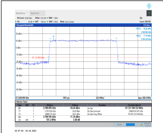
1-N77-3700-3980-PC3-30-100-M-8-CP-64QAM-Out er_Full-273@0-Ant1-97.121-101.200-≤100-PASS
