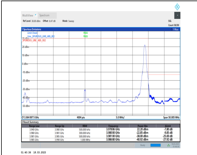
1-N77-3700-3980-PC3-30-40-H-2-DFT-PI2BPSK-Edge_1RB_Right-1@105-Ant1-1--PASS-see graph
