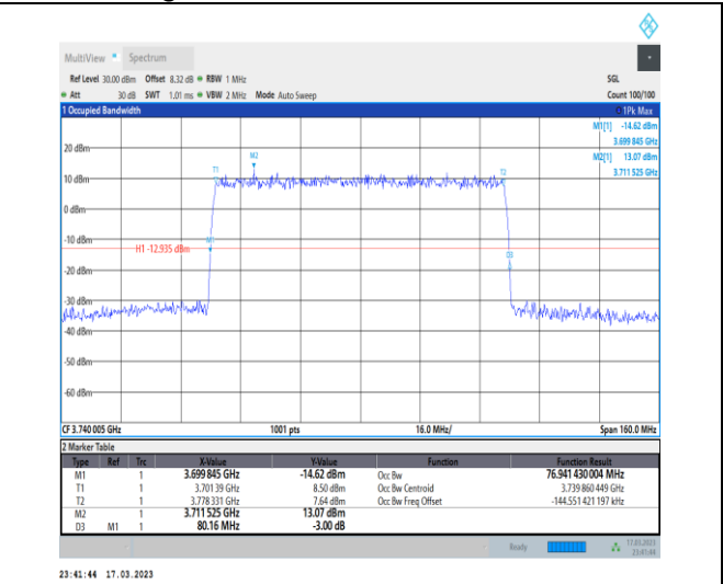
1-N77-3700-3980-30-80-L-3-DFT-16QAM-Outer_Full -216@0-Ant1-76.941-80.160-<=80-PASS
