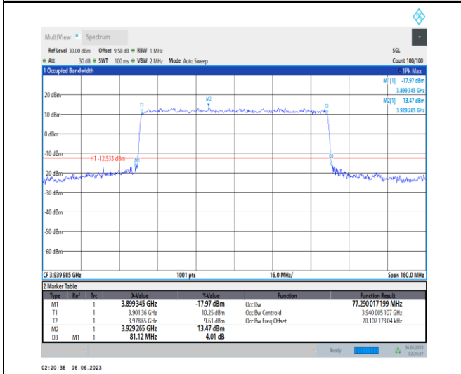
1-N77-3700-3980-PC3-30-80-H-6-CP-QPSK-Outer_Full-217@0-Ant1-77.29-81.120-≤80-PASS
