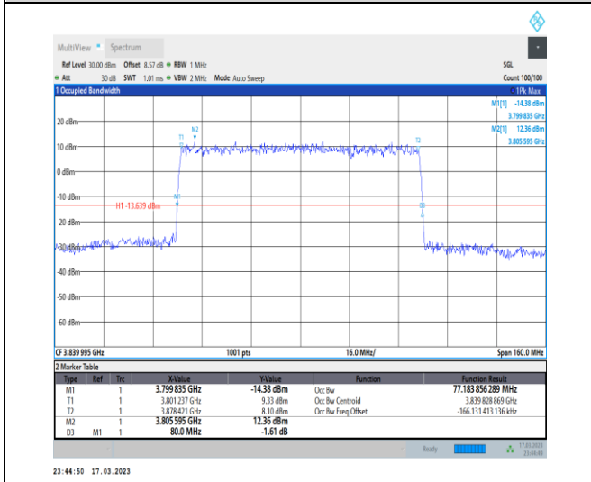
1-N77-3700-3980-30-80-M-3-DFT-16QAM-Outer_Full-216@0-Ant1-77.184-80.000-≤80-PASS
