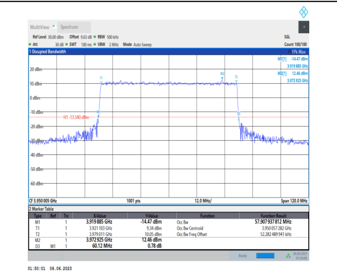
1-N77-3700-3980-PC3-30-60-H-4-DFT-64QAM-Oute r_Full-162@0-Ant1-57.908-60.120-≤60-PASS
