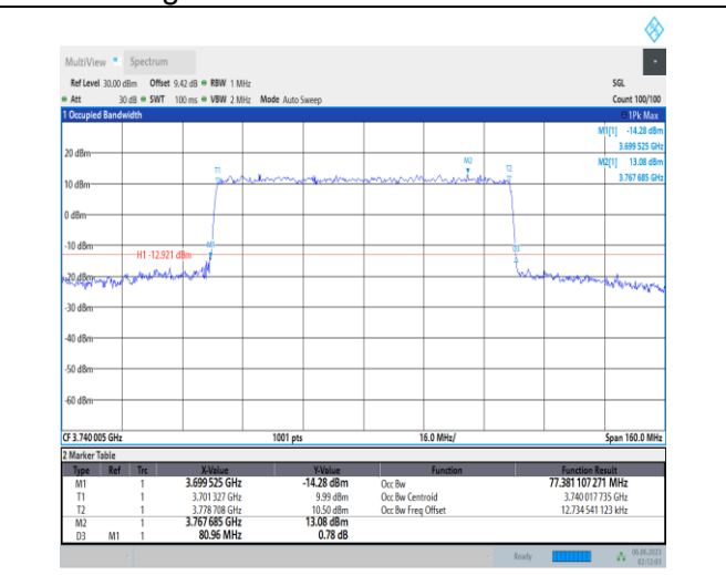
1-N77-3700-3980-PC3-30-80-L-7-CP-16QAM-Outer_Full-217@0-Ant1-77.381-80.960-≤80-PASS
