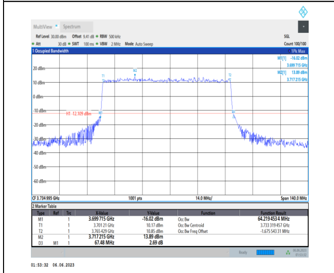
1-N77-3700-3980-PC3-30-70-L-2-DFT-PI2BPSK-Outer_Full-180@0-Ant1-64.219-67.480-<=70-PASS
