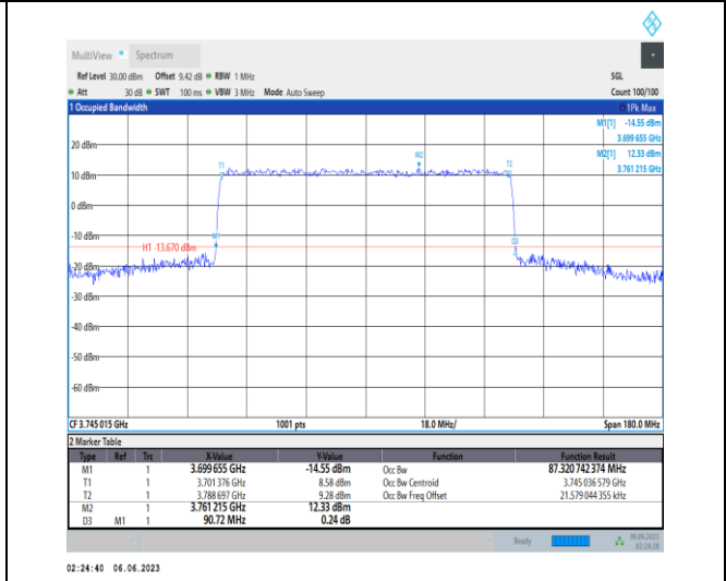
1-N77-3700-3980-PC3-30-90-L-6-CP-QPSK-Outer_Full-245@0-Ant1-87.321-90.720-≤90-PASS
