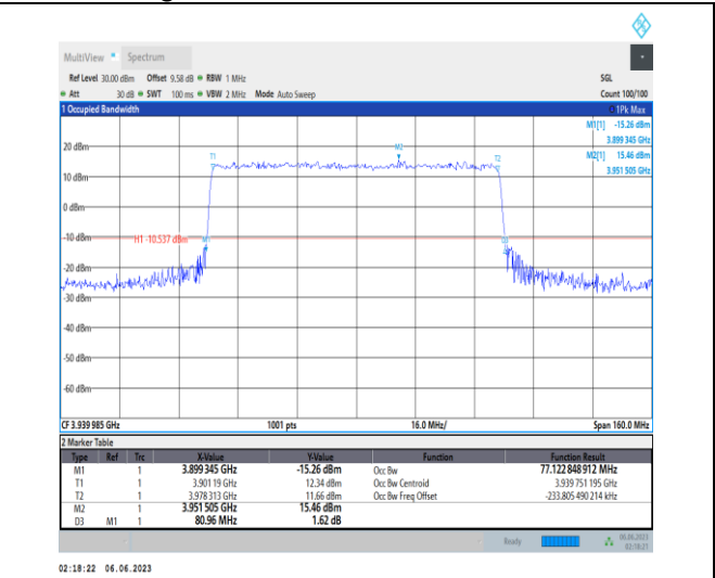
1-N77-3700-3980-PC3-30-80-H-1-DFT-QPSK-Outer_Full-216@0-Ant1-77.123-80.960-≤80-PASS
