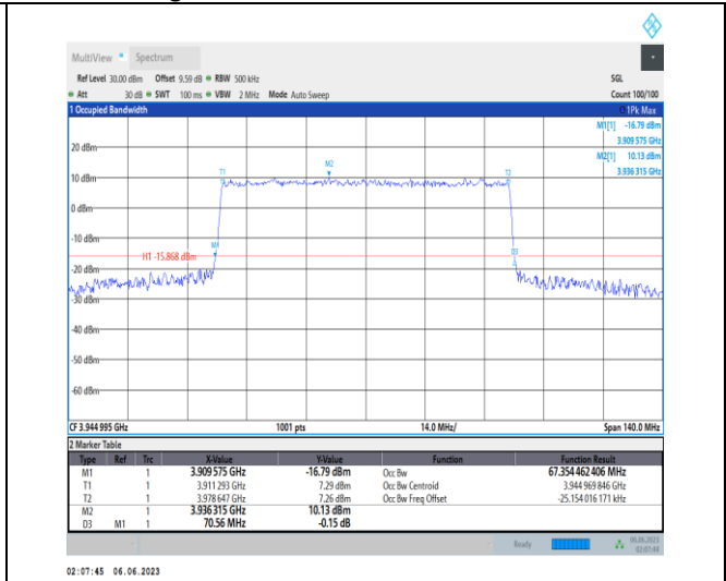
1-N77-3700-3980-PC3-30-70-H-8-CP-64QAM-Outer_Full-189@0-Ant1-67.354-70.560-≤70-PASS
