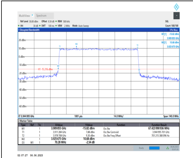
1-N77-3700-3980-PC3-30-70-H-7-CP-16QAM-Outer_Full-189@0-Ant1-67.424-70.280-≤70-PASS
