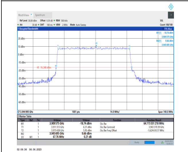
1-N77-3700-3980-PC3-30-70-H-5-DFT-256QAM-Outer_Full-180@0-Ant1-64.116-67.760-≤70-PASS
