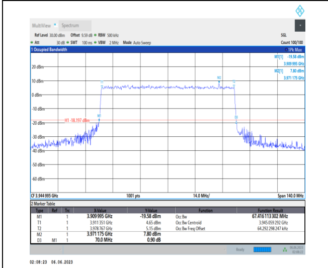
1-N77-3700-3980-PC3-30-70-H-9-CP-256QAM-Outer_Full-189@0-Ant1-67.416-70.000-≤70-PASS
