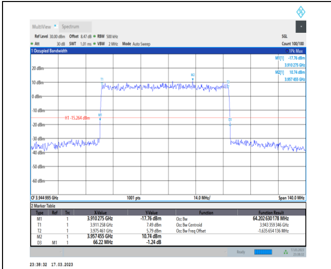
1-N77-3700-3980-30-70-H-3-DFT-16QAM-Outer_Ful I-180@0-Ant1-64.203-66.220-≤70-PASS
