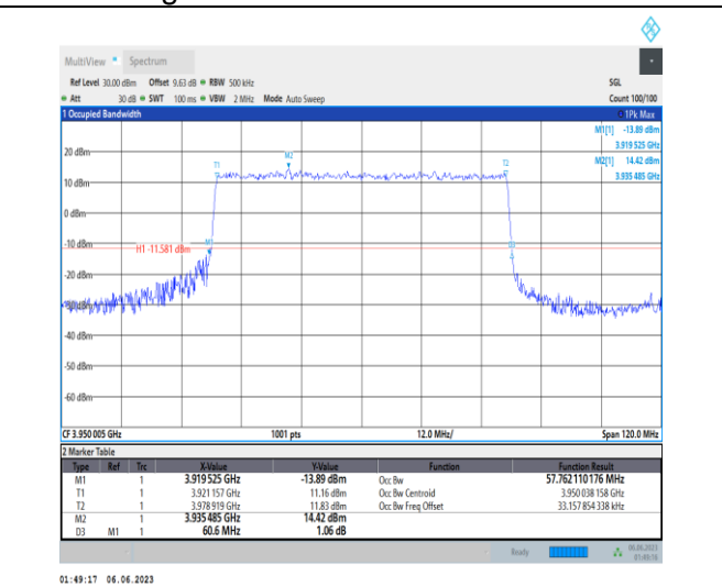
1-N77-3700-3980-PC3-30-60-H-2-DFT-PI2BPSK-Ou ter_Full-162@0-Ant1-57.762-60.600-≤60-PASS
