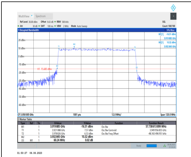
1-N77-3700-3980-PC3-30-60-H-5-DFT-256QAM-Out er_Full-162@0-Ant1-57.739-60.240-≤60-PASS
