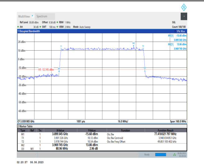
1-N77-3700-3980-PC3-30-80-H-7-CP-16QAM-Outer_Full-217@0-Ant1-77.418-80.960-≤80-PASS
