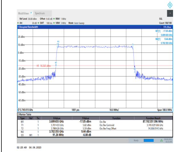
1-N77-3700-3980-PC3-30-90-L-9-CP-256QAM-Outer_Full-245@0-Ant1-87.192-91.260-≤90-PASS
