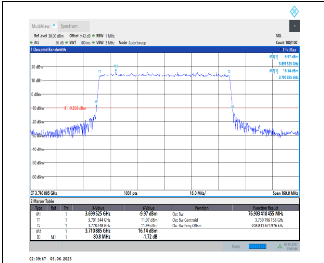
1-N77-3700-3980-PC3-30-80-L-2-DFT-PI2BPSK-Out er_Full-216@0-Ant1-76.903-80.800-<=80-PASS
