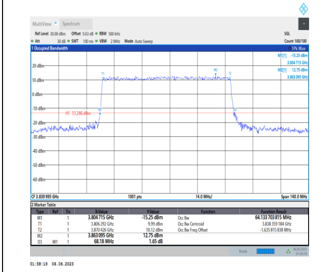
1-N77-3700-3980-PC3-30-70-M-1-DFT-QPSK-Outer_Full-180@0-Ant1-64.134-68.180-≤70-PASS
