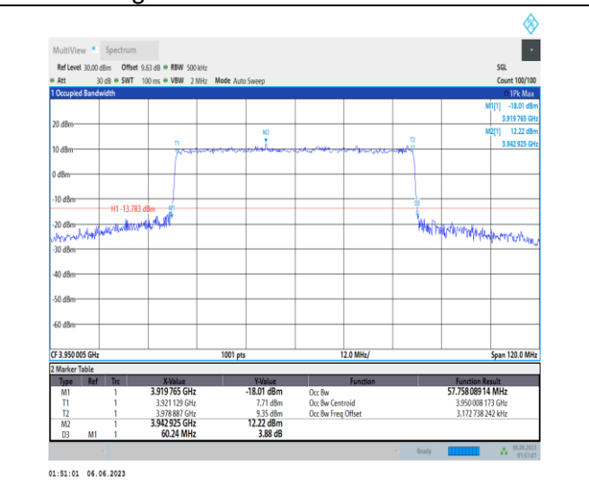
1-N77-3700-3980-PC3-30-60-H-6-CP-QPSK-Outer_Full-162@0-Ant1-57.758-60.240-≤60-PASS
