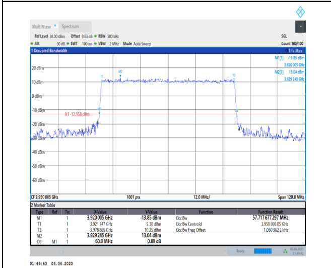
1-N77-3700-3980-PC3-30-60-H-3-DFT-16QAM-Oute r_Full-162@0-Ant1-57.718-60.000-≤60-PASS
