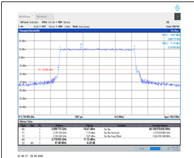
1-N77-3700-3980-PC3-30-70-L-4-DFT-64QAM-Outer_Full-180@0-Ant1-64.15-67.480-≤70-PASS
