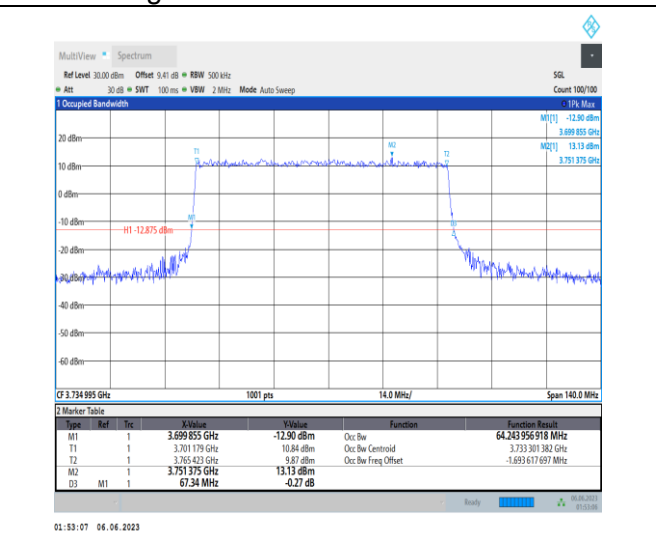
1-N77-3700-3980-PC3-30-70-L-1-DFT-QPSK-Outer_Full-180@0-Ant1-64.244-67.340-<=70-PASS
