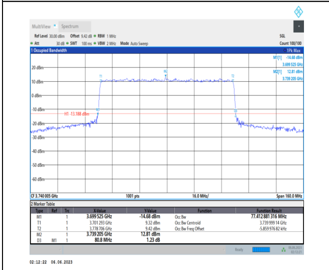
1-N77-3700-3980-PC3-30-80-L-8-CP-64QAM-Outer_Full-217@0-Ant1-77.413-80.800-≤80-PASS
