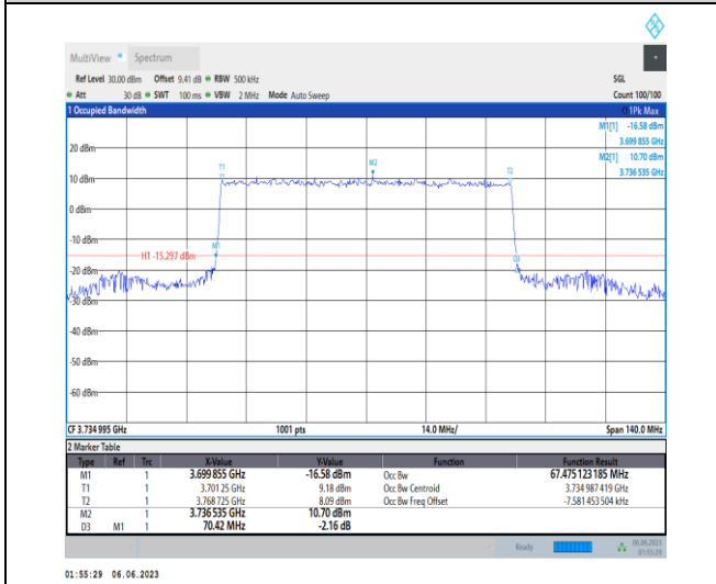
1-N77-3700-3980-PC3-30-70-L-6-CP-QPSK-Outer_Full-189@0-Ant1-67.475-70.420-≤70-PASS
