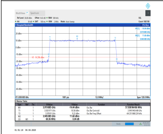
1-N77-3700-3980-PC3-30-60-H-7-CP-16QAM-Outer_Full-162@0-Ant1-57.939-60.360-≤60-PASS
