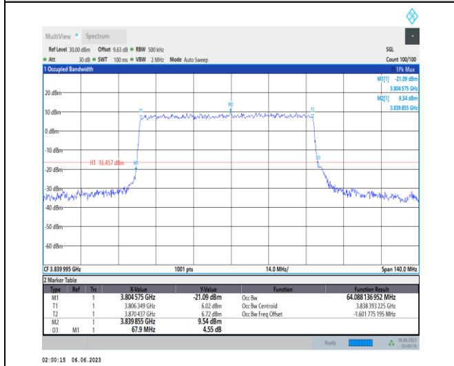
1-N77-3700-3980-PC3-30-70-M-5-DFT-256QAM-Outer_Full-180@0-Ant1-64.088-67.900-≤70-PASS
