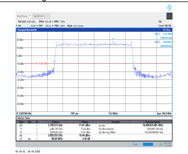
1-N77-3700-3980-PC3-30-80-M-2-DFT-PI2BPSK-Outer_Full-216@0-Ant1-76.901-80.640-≤80-PASS
