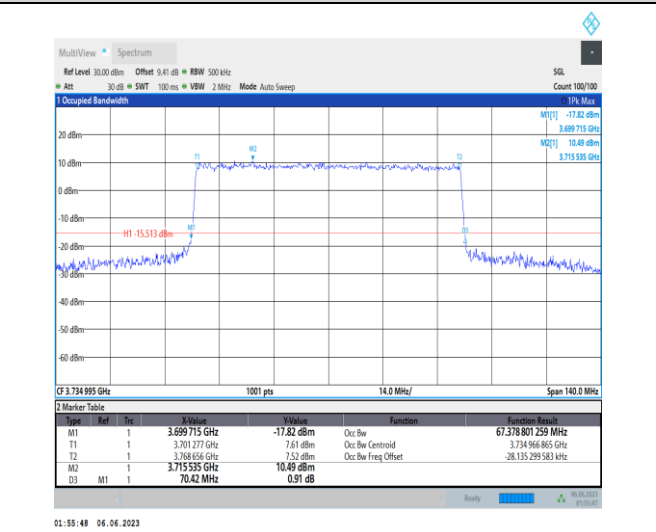
1-N77-3700-3980-PC3-30-70-L-7-CP-16QAM-Outer_Full-189@0-Ant1-67.379-70.420-≤70-PASS
