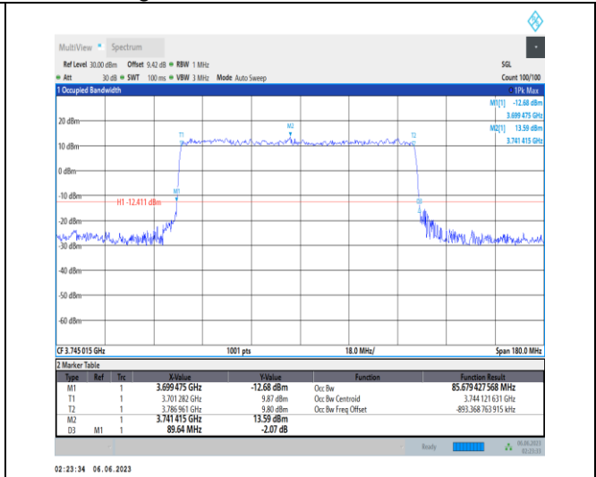
1-N77-3700-3980-PC3-30-90-L-4-DFT-64QAM-Outer_Full-240@0-Ant1-85.679-89.640-≤90-PASS
