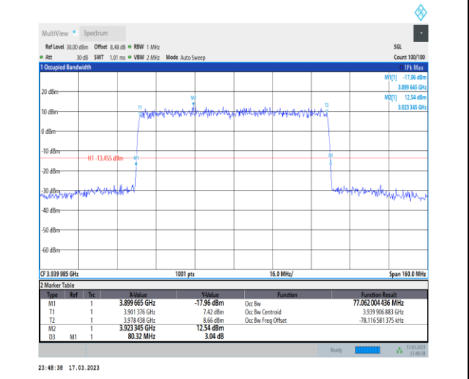
1-N77-3700-3980-30-80-H-3-DFT-16QAM-Outer_Full-216@0-Ant1-77.062-80.320-≤80-PASS
