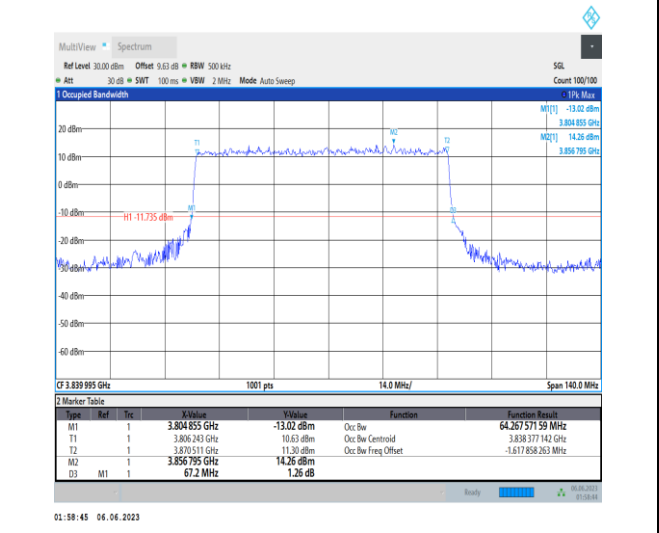
1-N77-3700-3980-PC3-30-70-M-2-DFT-PI2BPSK-Outer_Full-180@0-Ant1-64.268-67.200-≤70-PASS
