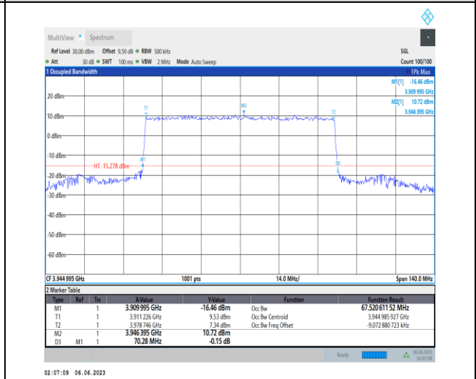
1-N77-3700-3980-PC3-30-70-H-6-CP-QPSK-Outer_Full-189@0-Ant1-67.521-70.280-≤70-PASS
