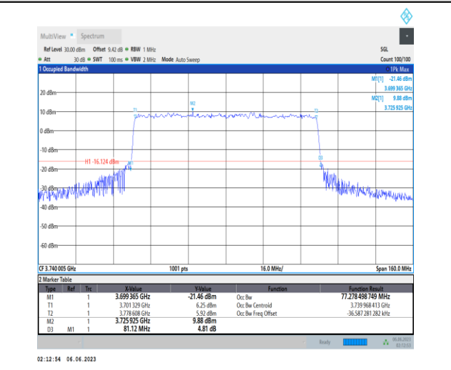
1-N77-3700-3980-PC3-30-80-L-9-CP-256QAM-Outer_Full-217@0-Ant1-77.278-81.120-≤80-PASS
