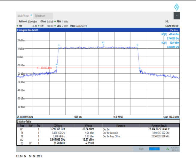
1-N77-3700-3980-PC3-30-80-M-8-CP-64QAM-Outer_Full-217@0-Ant1-77.324-81.280-≤80-PASS
