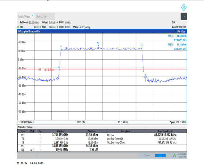
1-N77-3700-3980-PC3-30-90-M-3-DFT-16QAM-Outer_Full-240@0-Ant1-85.526-89.460-≤90-PASS
