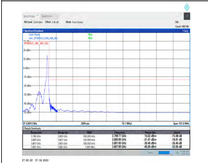
1-N78-3700-3800-PC3-30-80-H-5-CP-QPSK-Edge_1RB_Right-1@216-Ant1-1--PASS-see graph
