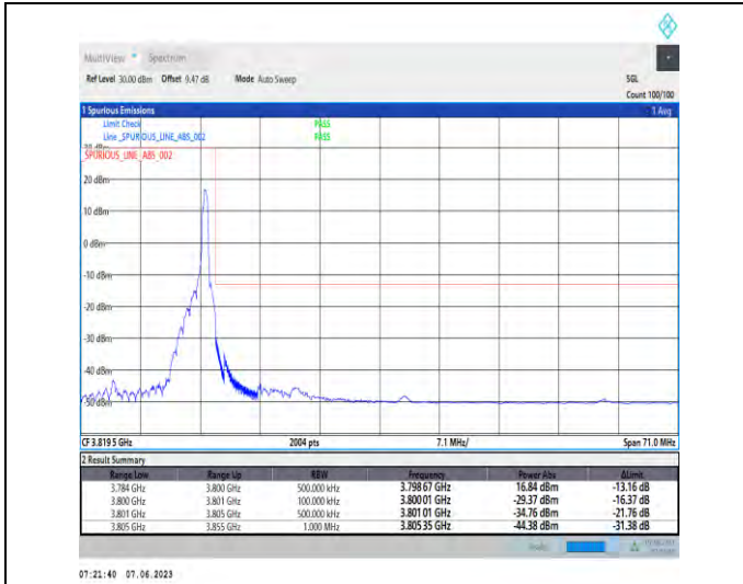
1-N78-3700-3800-PC3-30-50-H-2-DFT-PI2BPSK-Edge_1RB_Right-1@132-Ant1-1--PASS-see graph
