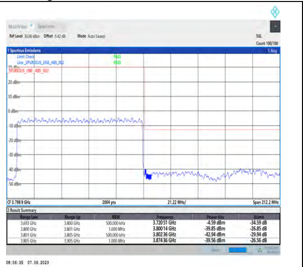
1-N78-3700-3800-PC3-30-100-H-3-DFT-PI2BPSK-Outer_Full-270@0-Ant1-1--PASS-see graph
