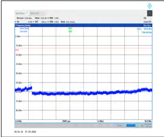
1-N78-3700-3800-PC3-30-100-L-1-N/A-DFT-PI2BP SK-Inner_1RB_Left-1@1-6000-18000-Ant1-7384.32 --53.34--13-PASS
