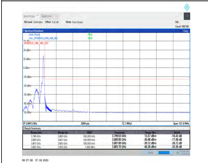
1-N78-3700-3800-PC3-30-100-H-5-CP-QPSK-Edge_1_RB_Right-1@272-Ant1-1--PASS-see graph
