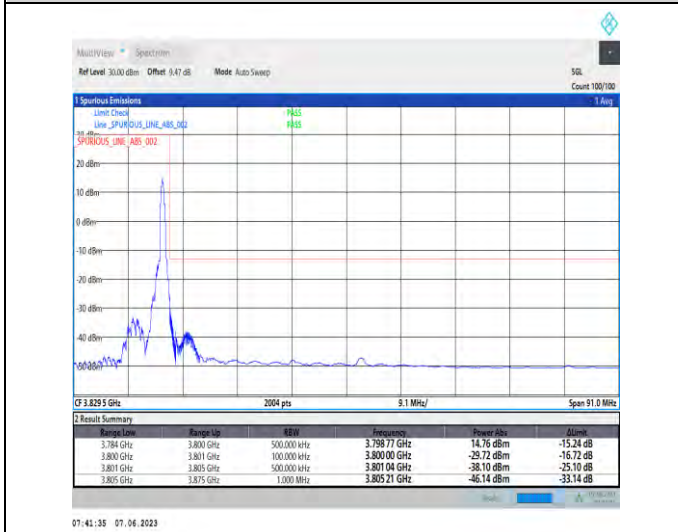
1-N78-3700-3800-PC3-30-70-H-5-CP-QPSK-Edge_1RB_Right-1@188-Ant1-1--PASS-see graph
