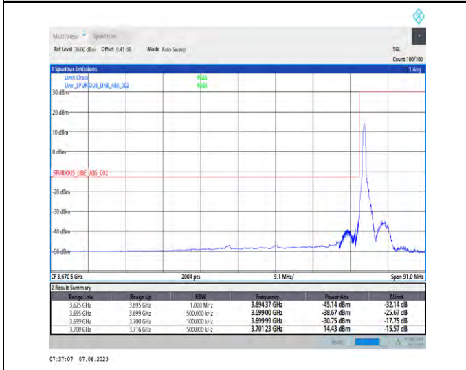
1-N78-3700-3800-PC3-30-70-L-4-CP-QPSK-Edge_1RB_Left-1@0-Ant1-1--PASS-see graph
