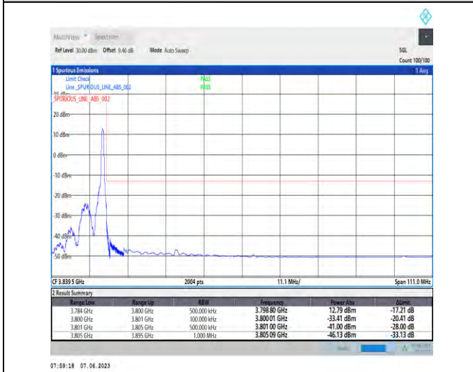
1-N78-3700-3800-PC3-30-90-H-5-CP-QPSK-Edge_1RB_Right-1@244-Ant1-1--PASS-see graph
