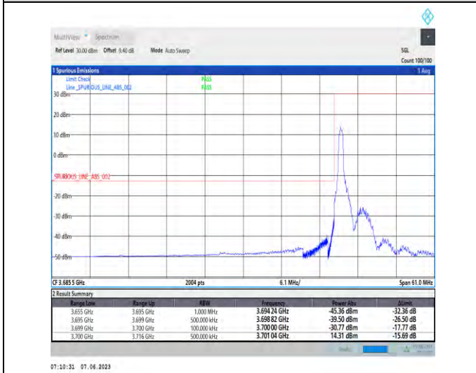
1-N78-3700-3800-PC3-30-40-L-4-CP-QPSK-Edge_1RB_Left-1@0-Ant1-1--PASS-see graph
