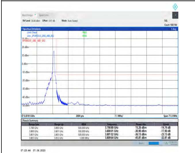
1-N78-3700-3800-PC3-30-50-H-5-CP-QPSK-Edge_1RB_Right-1@132-Ant1-1--PASS-see graph
