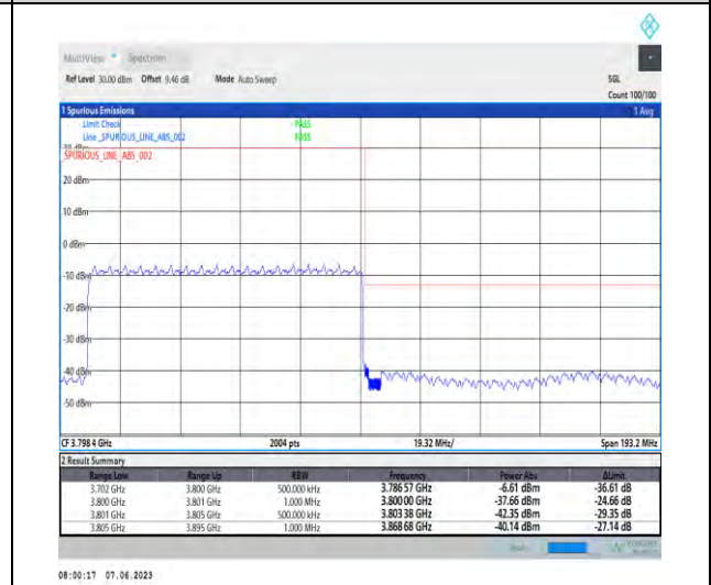
1-N78-3700-3800-PC3-30-90-H-6-CP-QPSK-Outer_Full-245@0-Ant1-1--PASS-see graph
