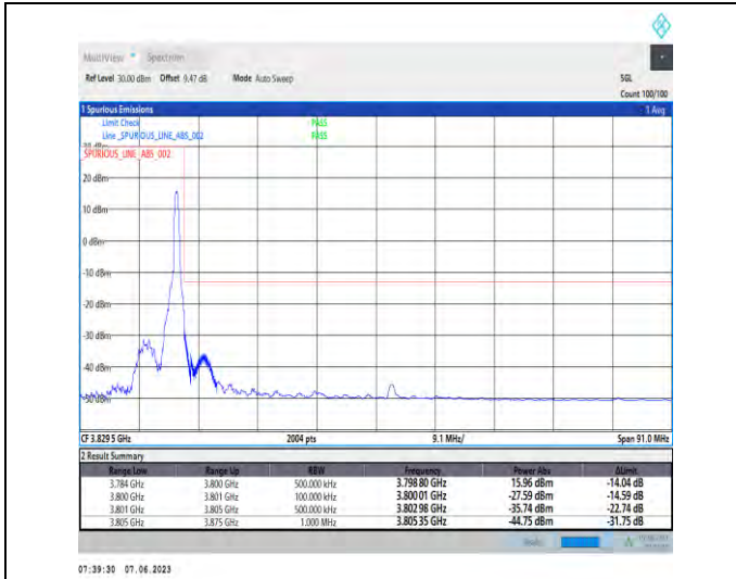
1-N78-3700-3800-PC3-30-70-H-2-DFT-PI2BPSK-Edge_1RB_Right-1@188-Ant1-1--PASS-see graph
