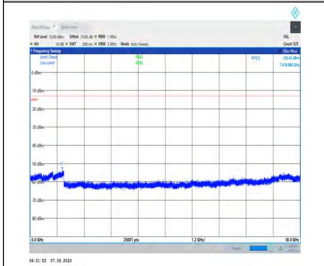
1-N78-3700-3800-PC3-30-100-M-1-N/A-DFT-PI2BP SK-Inner_1RB_Left-1@1-6000-18000-Ant1-7418.88 --53.42--13-PASS
