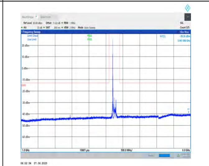
1-N78-3700-3800-PC3-30-100-H-1-N/A-DFT-PI2BPS K-Inner_1RB_Left-1@1-1000-6000-Ant1-5941.00--39 .26--13-PASS
