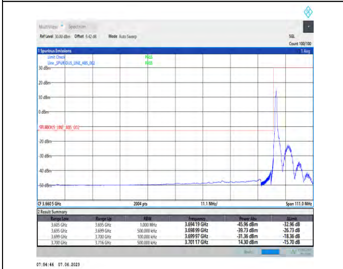
1-N78-3700-3800-PC3-30-90-L-4-CP-QPSK-Edge_1RB_Left-1@0-Ant1-1--PASS-see graph
