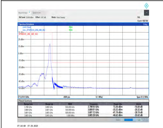
1-N78-3700-3800-PC3-30-40-H-5-CP-QPSK-Edge_1RB_Right-1@105-Ant1-1--PASS-see graph
