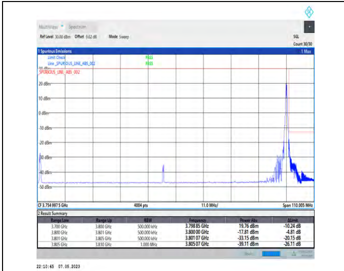
1-N78-3700-3800-PC3-30-100-H-1-DFT-PI2BPSK-Edge_1_RB_Right-1@272-Ant1-1--PASS-see graph
