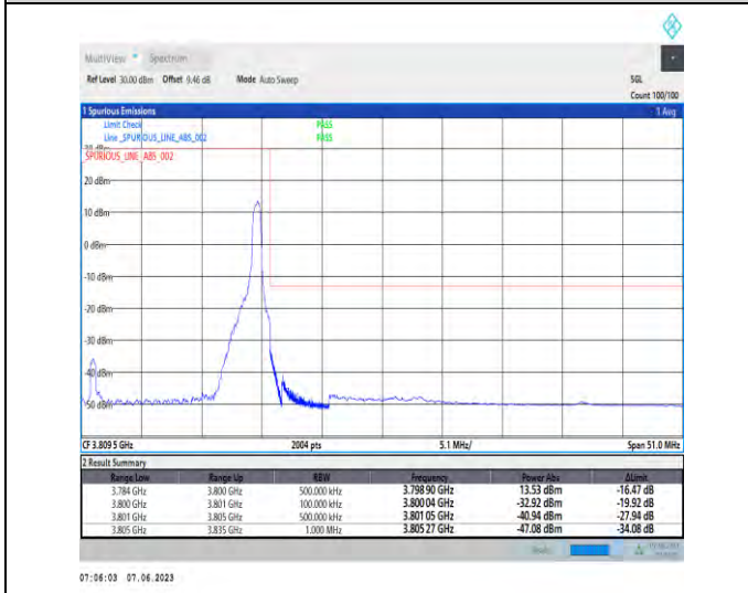
1-N78-3700-3800-PC3-30-30-H-5-CP-QPSK-Edge_1RB_Right-1@77-Ant1-1--PASS-see graph
