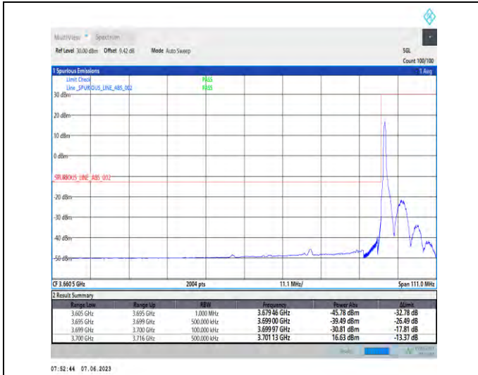
1-N78-3700-3800-PC3-30-90-L-1-DFT-PI2BPSK-Edge_1RB_Left-1@0-Ant1-1--PASS-see graph
