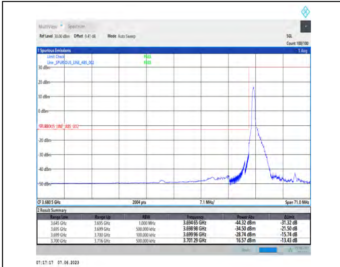
1-N78-3700-3800-PC3-30-50-L-1-DFT-PI2BPSK-Edge_1RB_Left-1@0-Ant1-1--PASS-see graph
