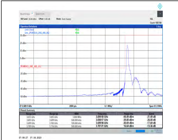
1-N78-3700-3800-PC3-30-40-L-1-DFT-PI2BPSK-Edge_1RB_Left-1@0-Ant1-1--PASS-see graph
