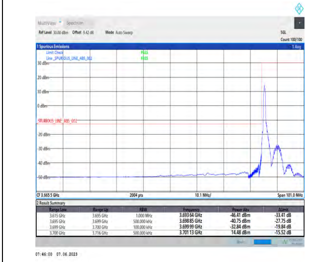
1-N78-3700-3800-PC3-30-80-L-4-CP-QPSK-Edge_1RB_Left-1@0-Ant1-1--PASS-see graph
