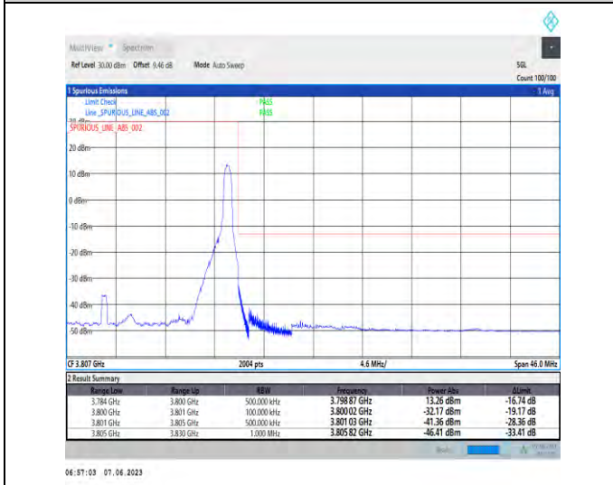
1-N78-3700-3800-PC3-30-25-H-5-CP-QPSK-Edge_1RB_Right-1@64-Ant1-1--PASS-see graph
