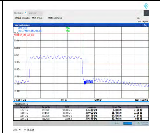
1-N78-3700-3800-PC3-30-30-H-6-CP-QPSK-Outer_Full-78@0-Ant1-1--PASS-see graph
