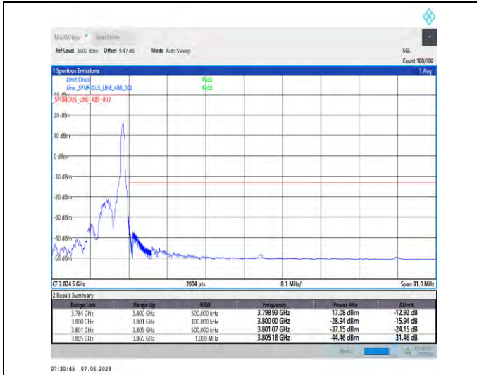
1-N78-3700-3800-PC3-30-60-H-2-DFT-PI2BPSK-Edge_1RB_Right-1@161-Ant1-1--PASS-see graph
