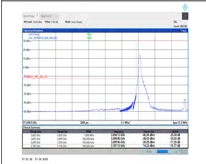
1-N78-3700-3800-PC3-30-30-L-4-CP-QPSK-Edge_1RB_Left-1@0-Ant1-1--PASS-see graph
