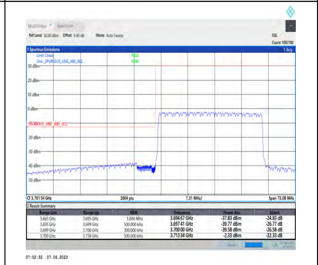
1-N78-3700-3800-PC3-30-30-L-6-CP-QPSK-Outer_Full-78@0-Ant1-1--PASS-see graph
