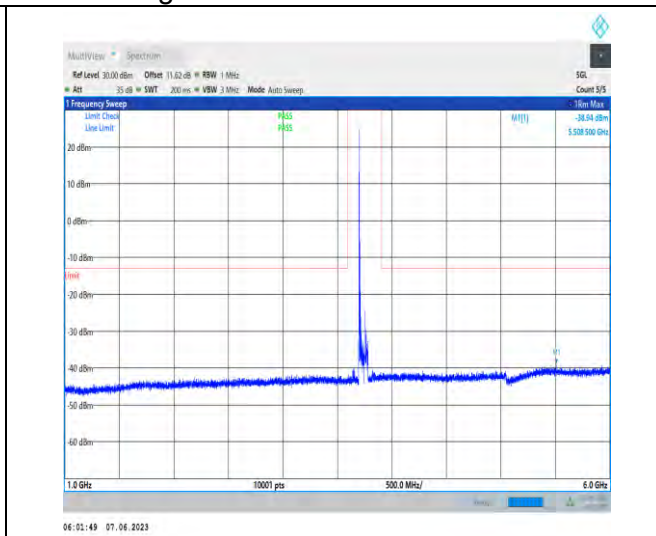
1-N78-3700-3800-PC3-30-100-M-1-N/A-DFT-PI2BPS K-Inner_1RB_Left-1@1-1000-6000-Ant1-5508.50--38 .94--13-PASS
