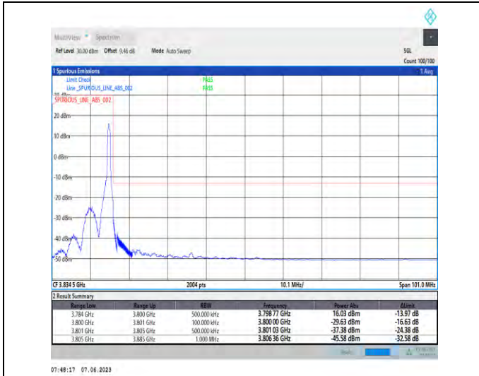
1-N78-3700-3800-PC3-30-80-H-2-DFT-PI2BPSK-Edge_1RB_Right-1@216-Ant1-1--PASS-see graph
