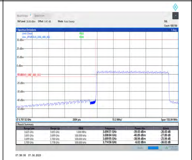
1-N78-3700-3800-PC3-30-70-L-6-CP-QPSK-Outer_Full-189@0-Ant1-1--PASS-see graph
