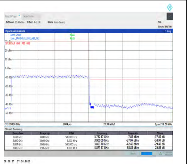
1-N78-3700-3800-PC3-30-100-H-6-CP-QPSK-Outer_Full-273@0-Ant1-1--PASS-see graph
