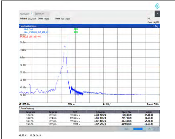
1-N78-3700-3800-PC3-30-25-H-2-DFT-PI2BPSK-Edge_1RB_Right-1@64-Ant1-1--PASS-see graph
