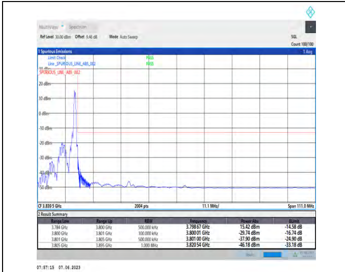
1-N78-3700-3800-PC3-30-90-H-2-DFT-PI2BPSK-Edge_1RB_Right-1@244-Ant1-1--PASS-see graph
